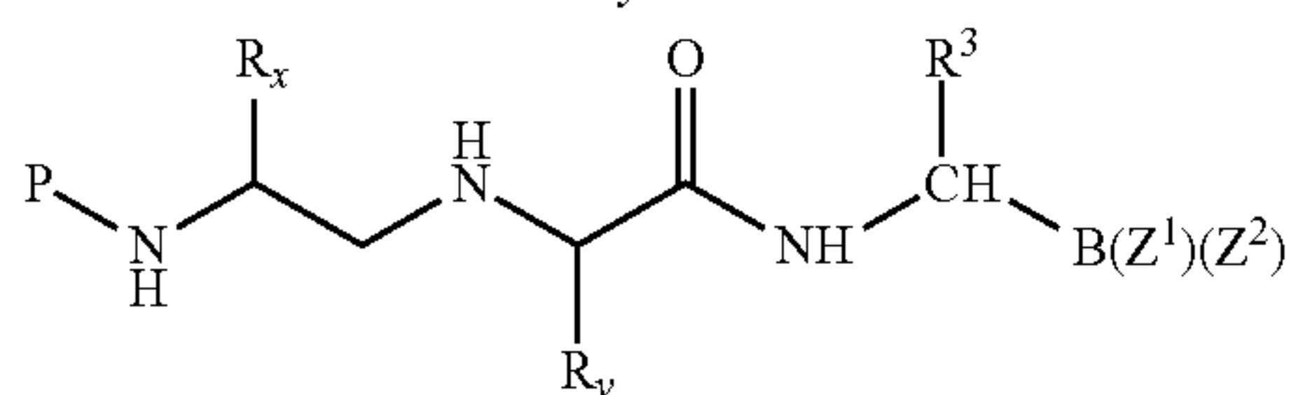
reduced peptide bond
