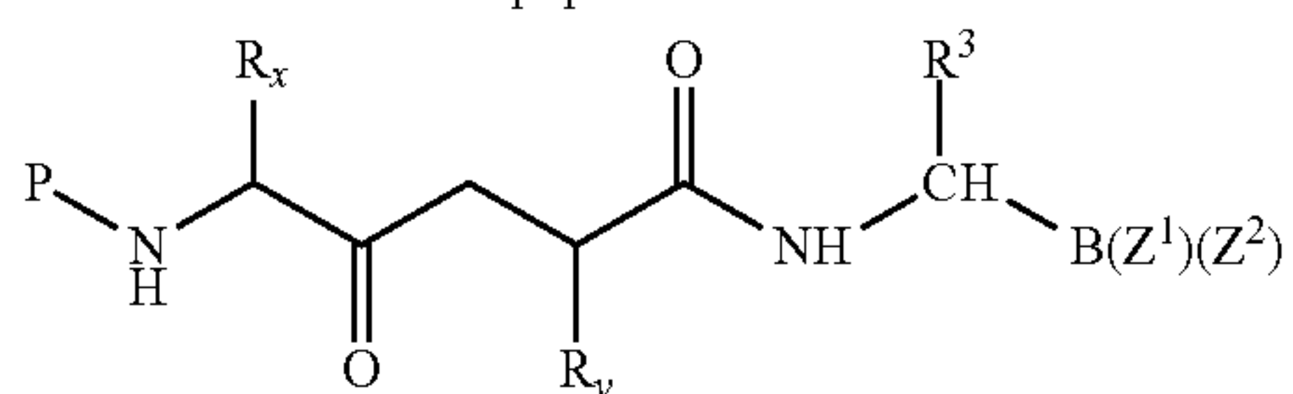
keto methylene isostere
