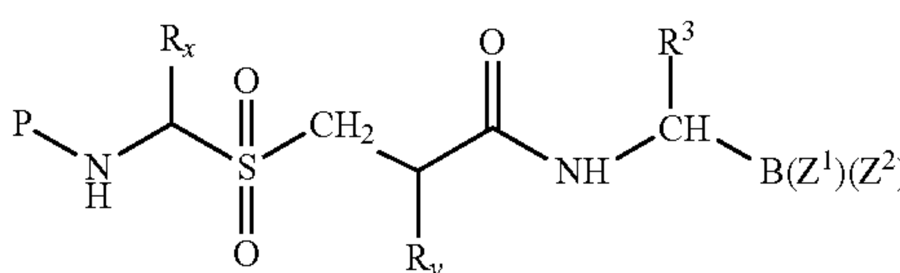
sulfone methylene isostere
