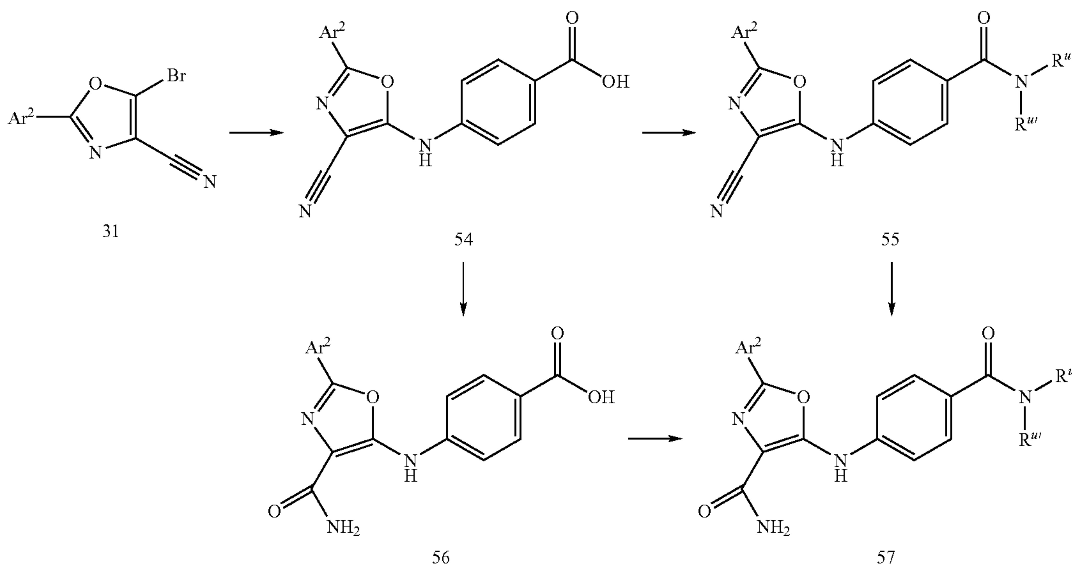
Scheme 15
