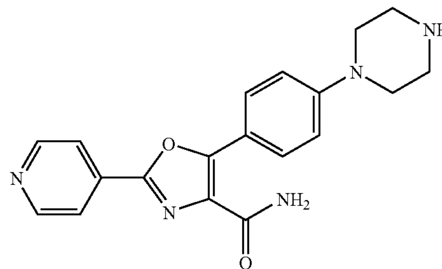
5-(4-(piperazin-1-yl)phenyl)-2-(pyridin-4-yl)oxazole-4-carboxamide
