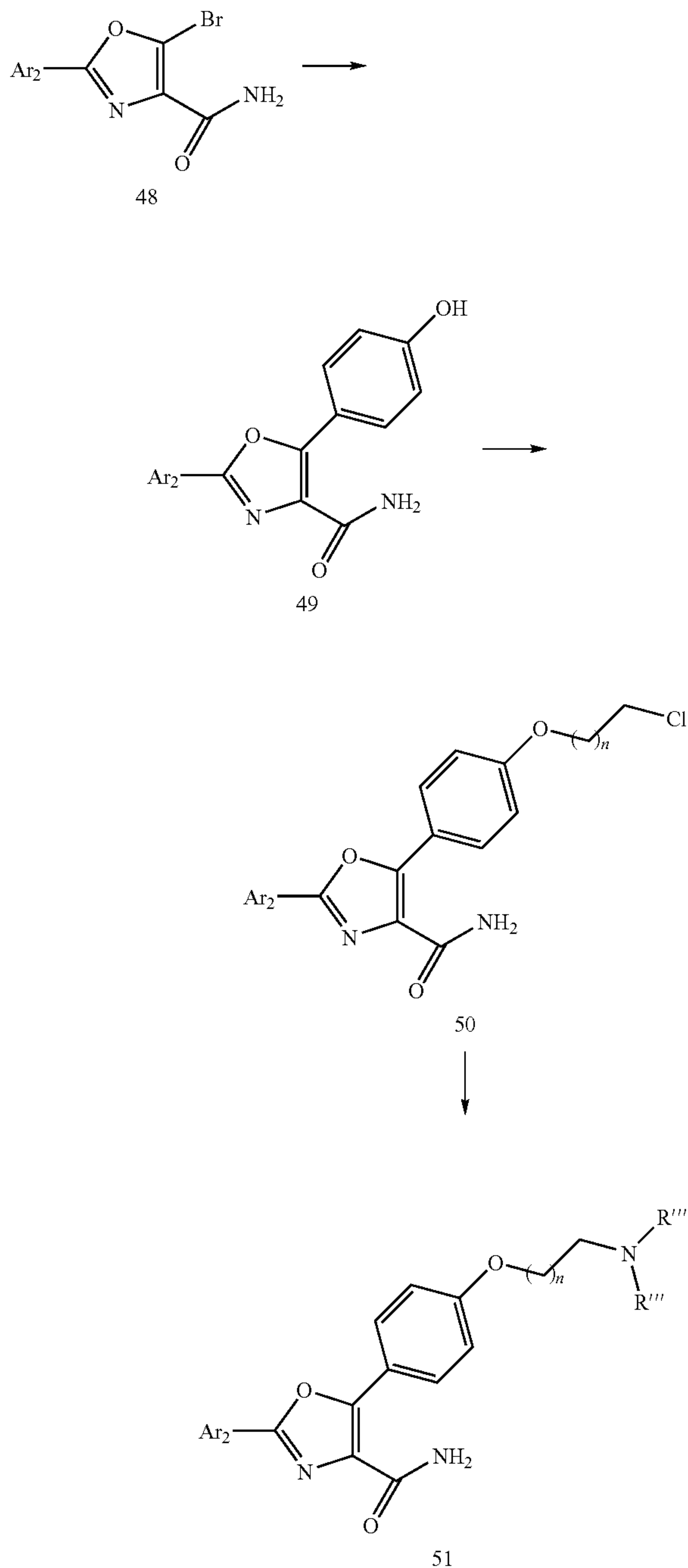
Scheme 13
