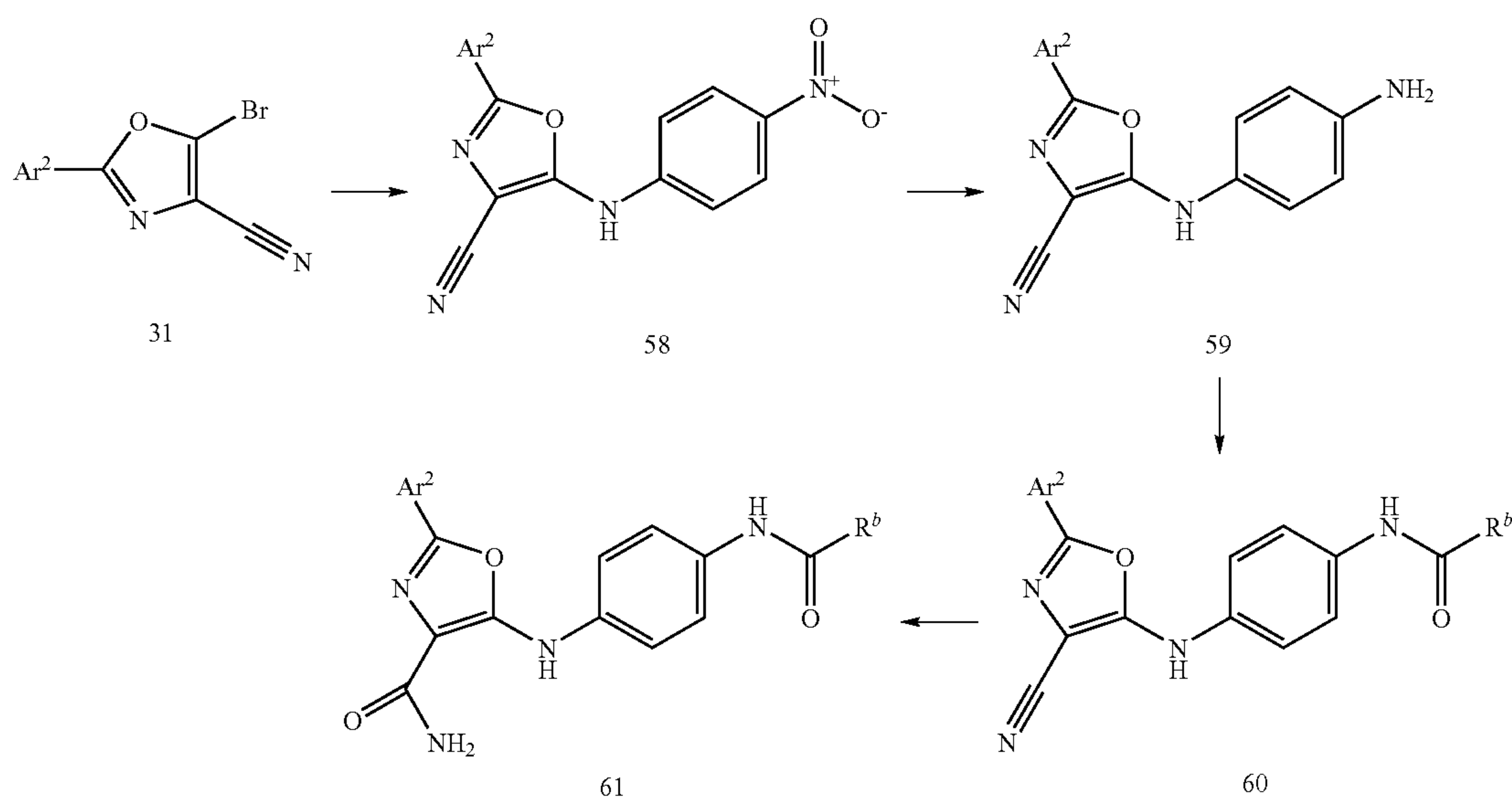
Scheme 16
