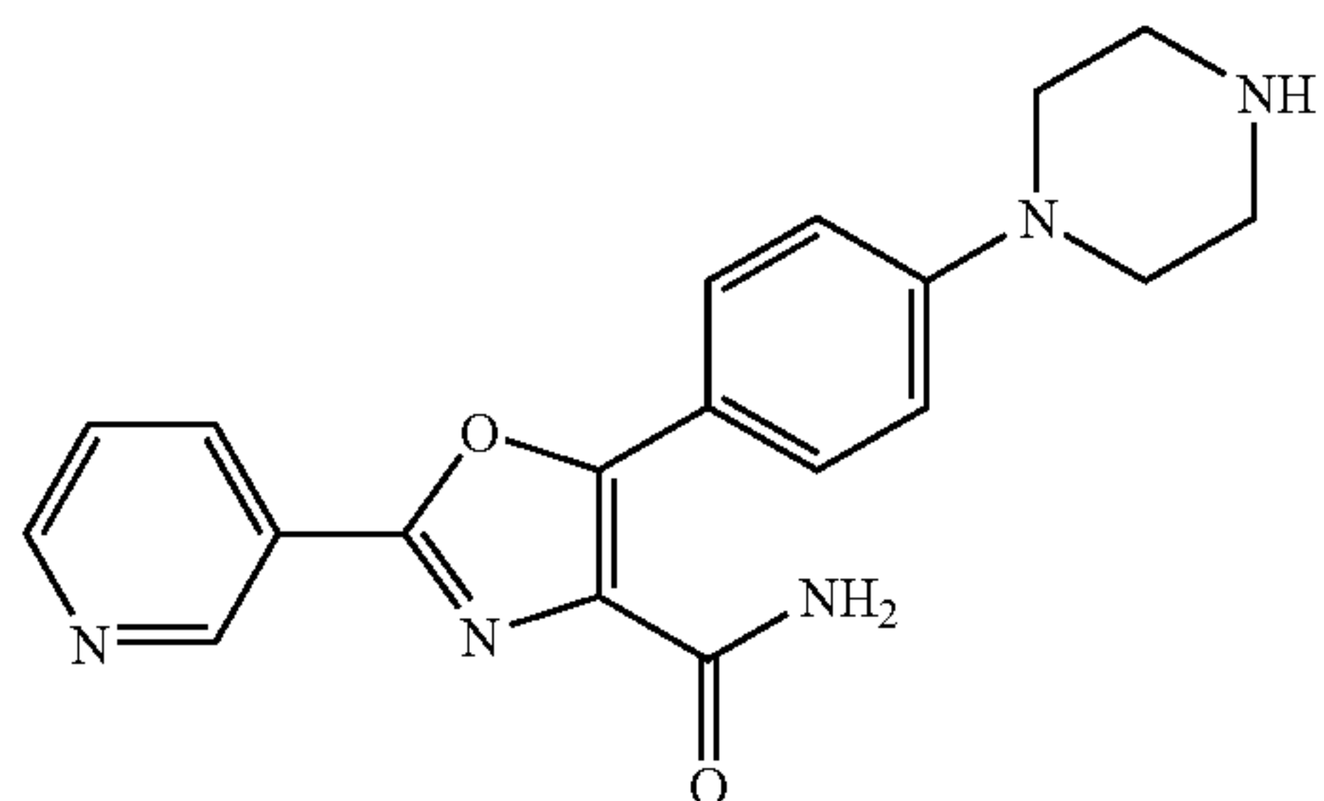
5-(4-(piperazin-1-yl)phenyl)-2-(pyridin-3-yl)oxazole-4-carboxamide
