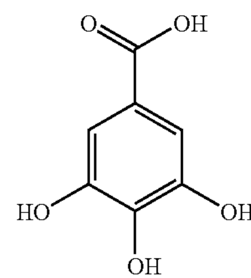
Gallic acid
