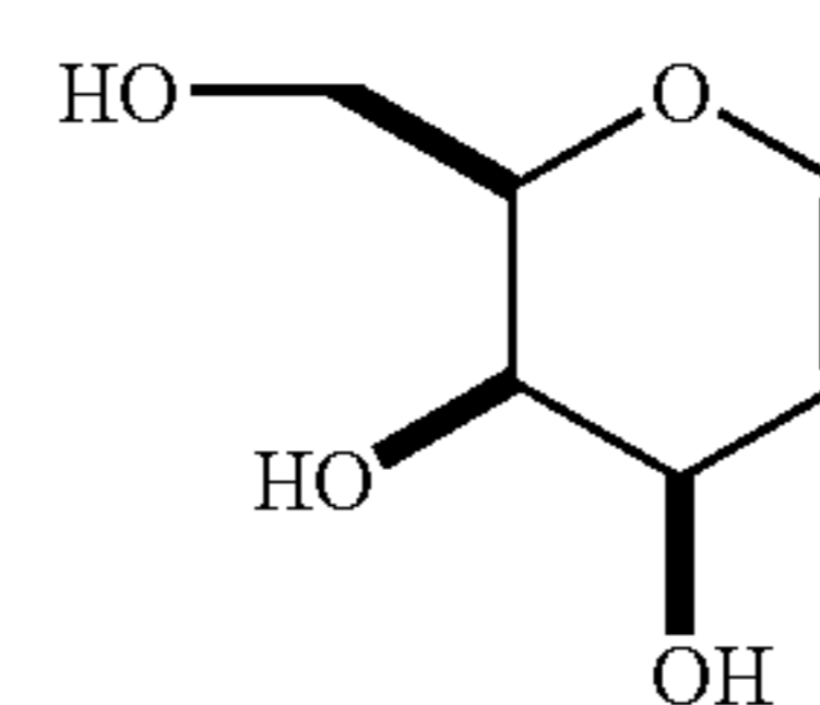
D-Galactal
