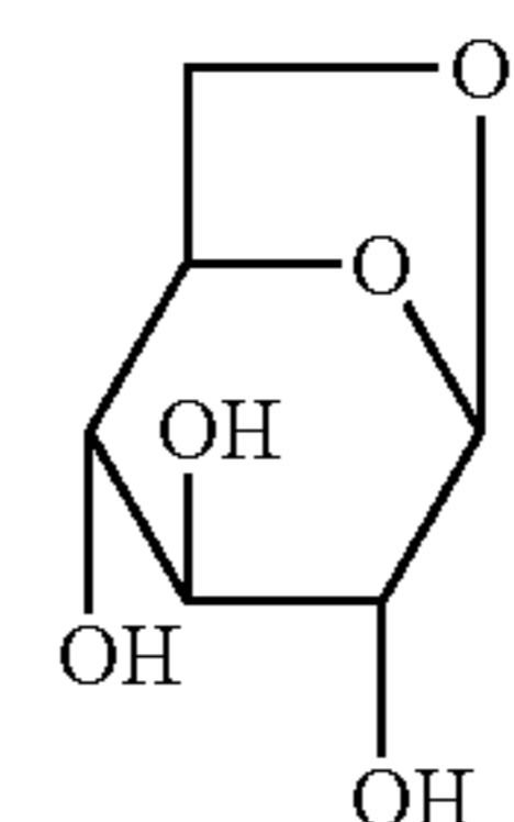
1,6-anhydro- \beta -D-Glucose
