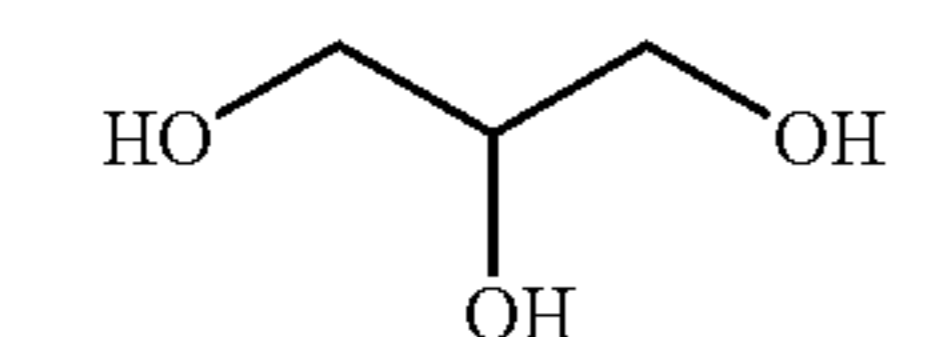
Glycerol (1,2,3-Propanetriol)
