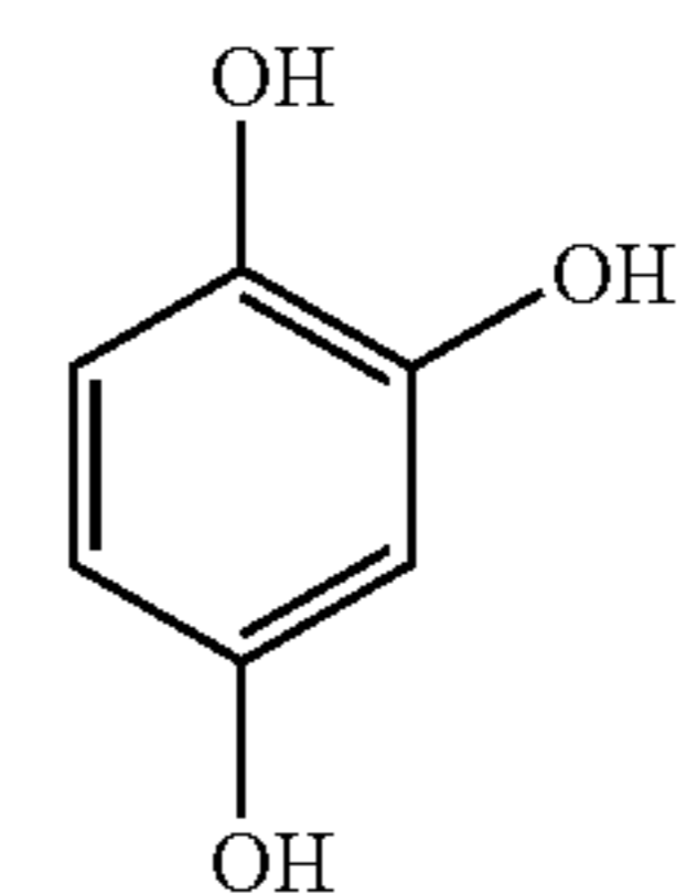
1,2,4-Trihydroxyl-benzene
