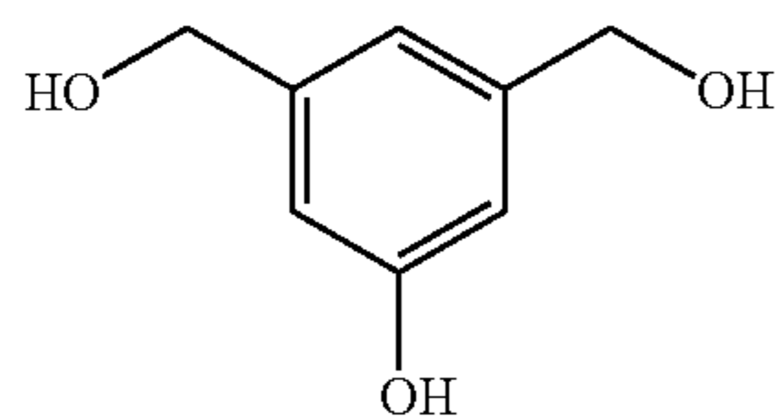
3,5-Di(hydroxymethyl)phenol
