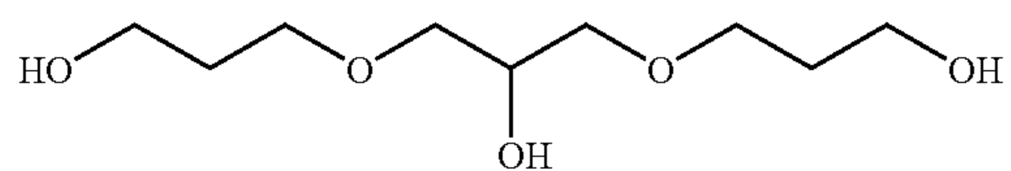
1,3-Di(hydroxypropoxy)-2-hydroxyl-propane
