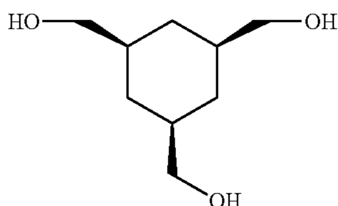
cis-1,3,5-Tri(hydroxymethyl)cyclohexane
