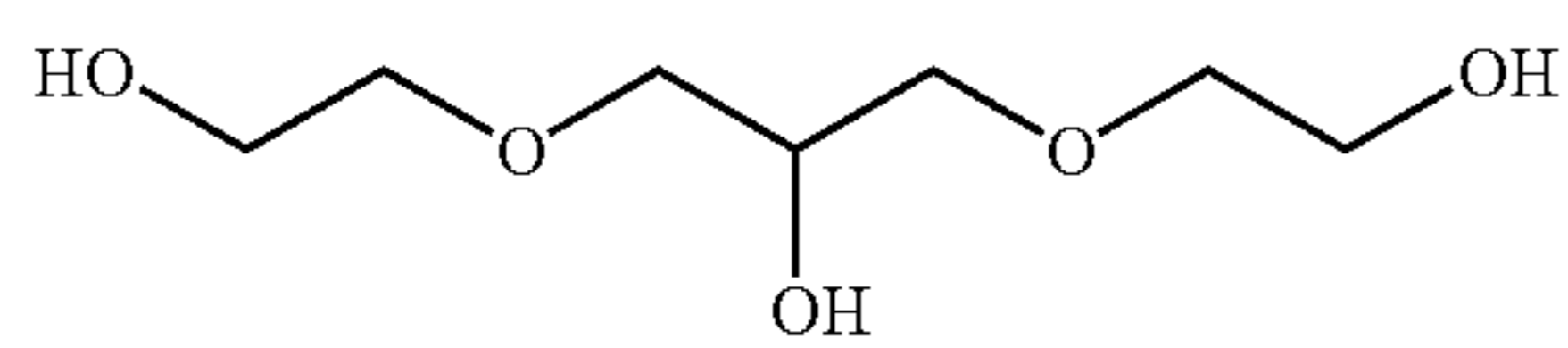
1,3-Di(hydroxyethoxy)-2-hydroxyl-propane
