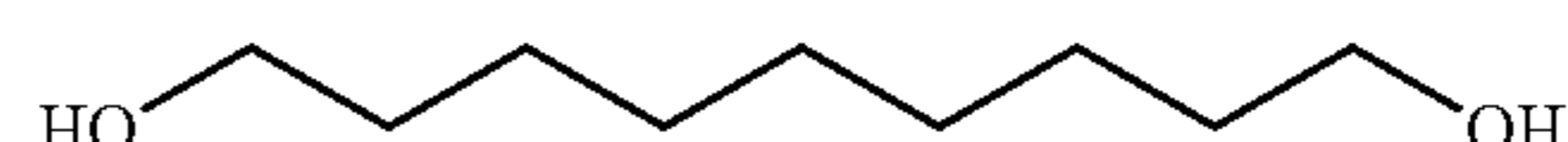
1,9-Nonanediol
