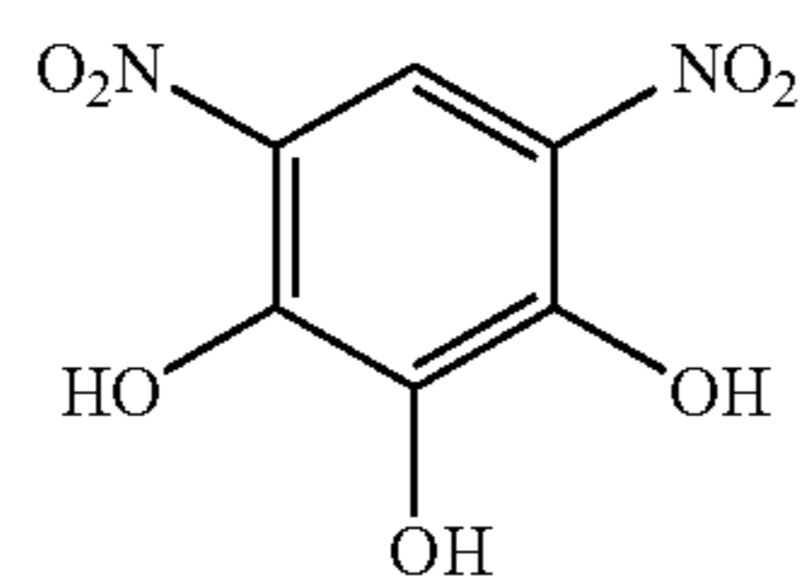
4,6-Nitropyrogallol
