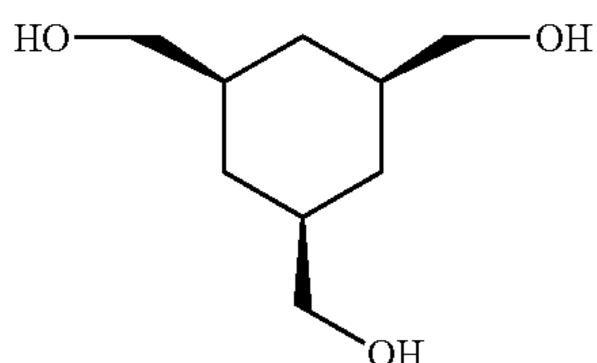
cis-1,3,5-Tri(hydroxymethyl)cyclohexane
