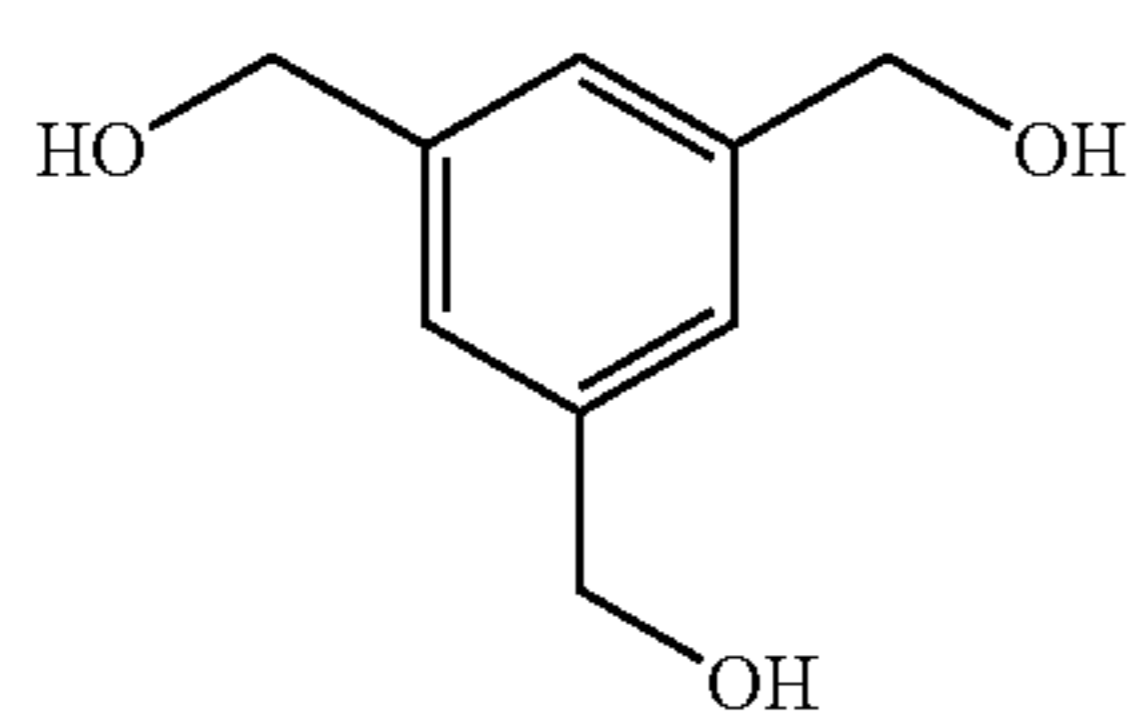
1,3,5-Tri(hydroxymethyl)benzene
