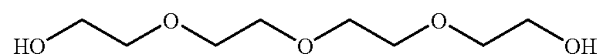
Tetraethylene glycol
