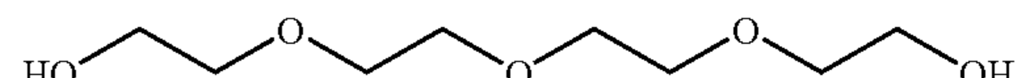
Tetraethylene glycol
