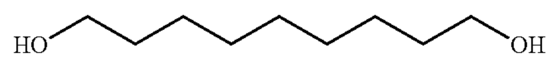
1,9-Nonanediol
