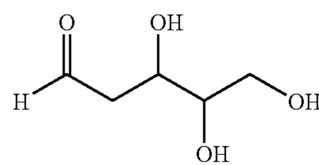
2-Deoxy-D-ribose
