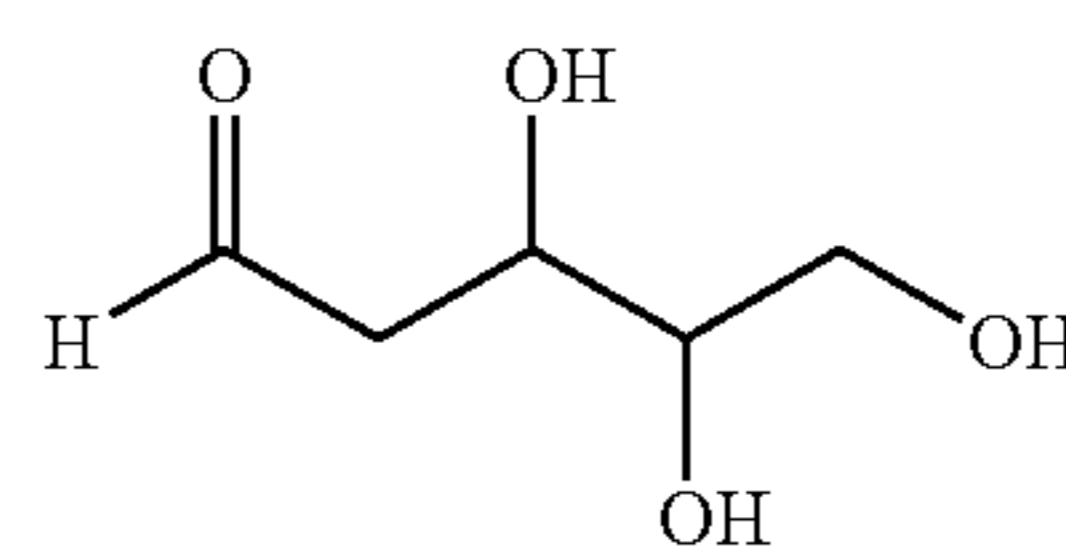
2-Deoxy-D-ribose
