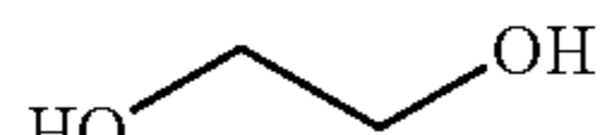
Ethylene glycol
