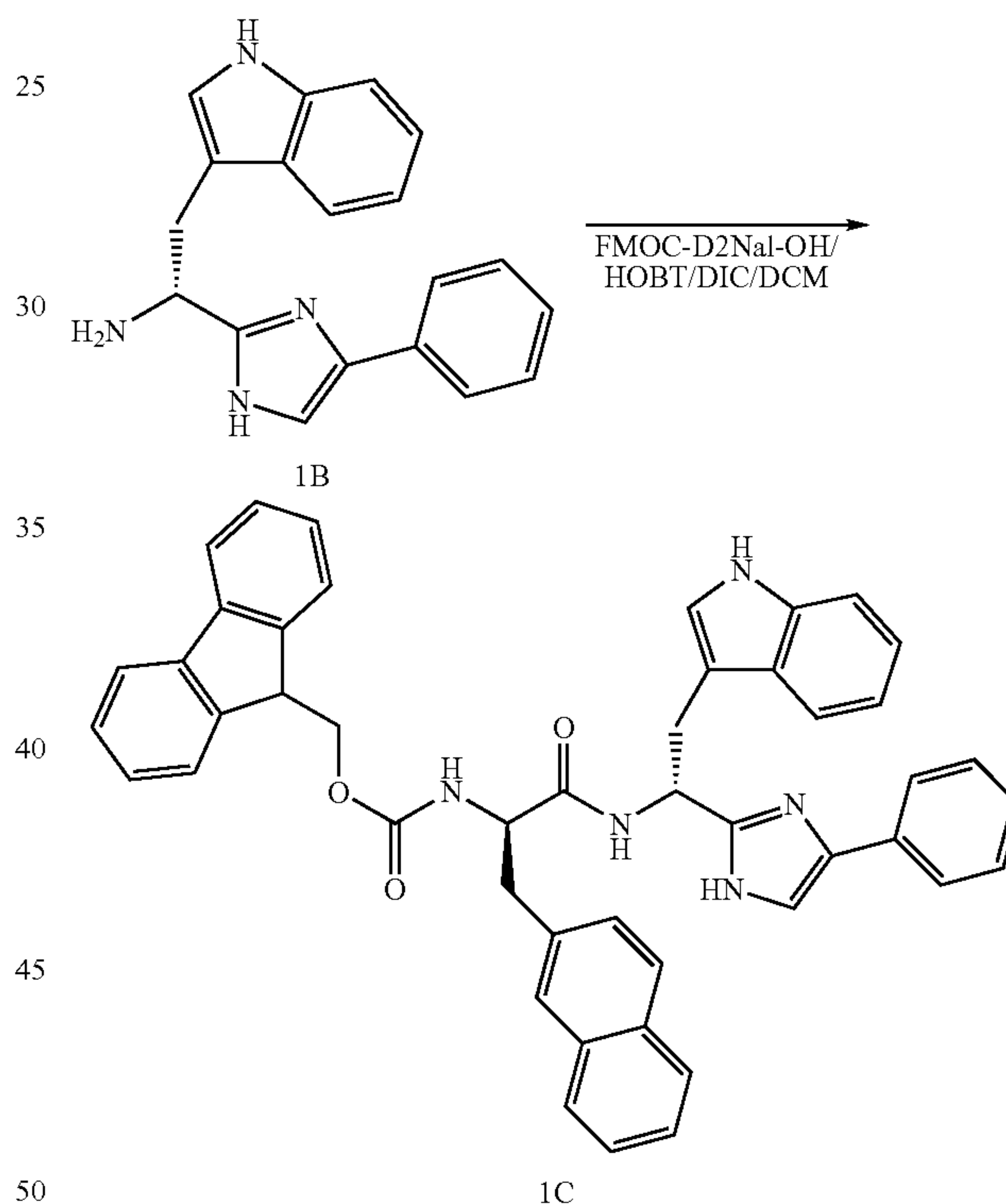
Scheme 1C
