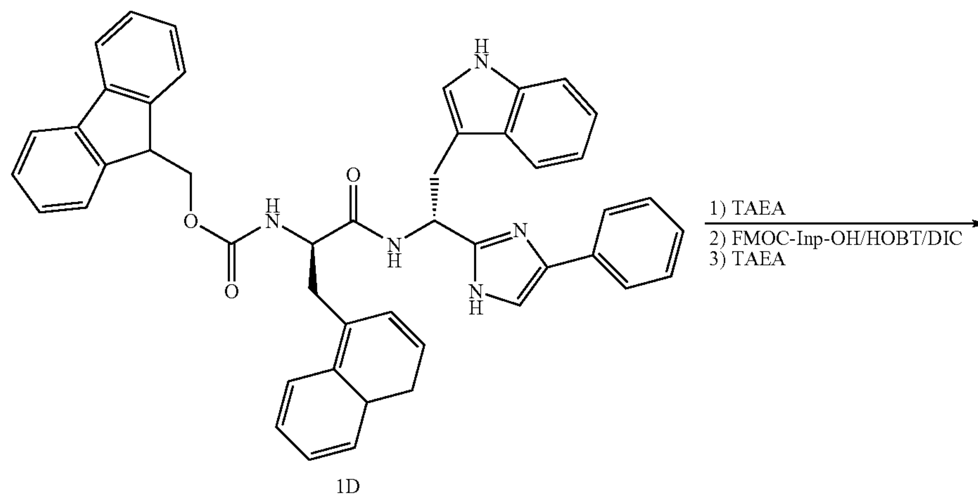
Scheme 1H
