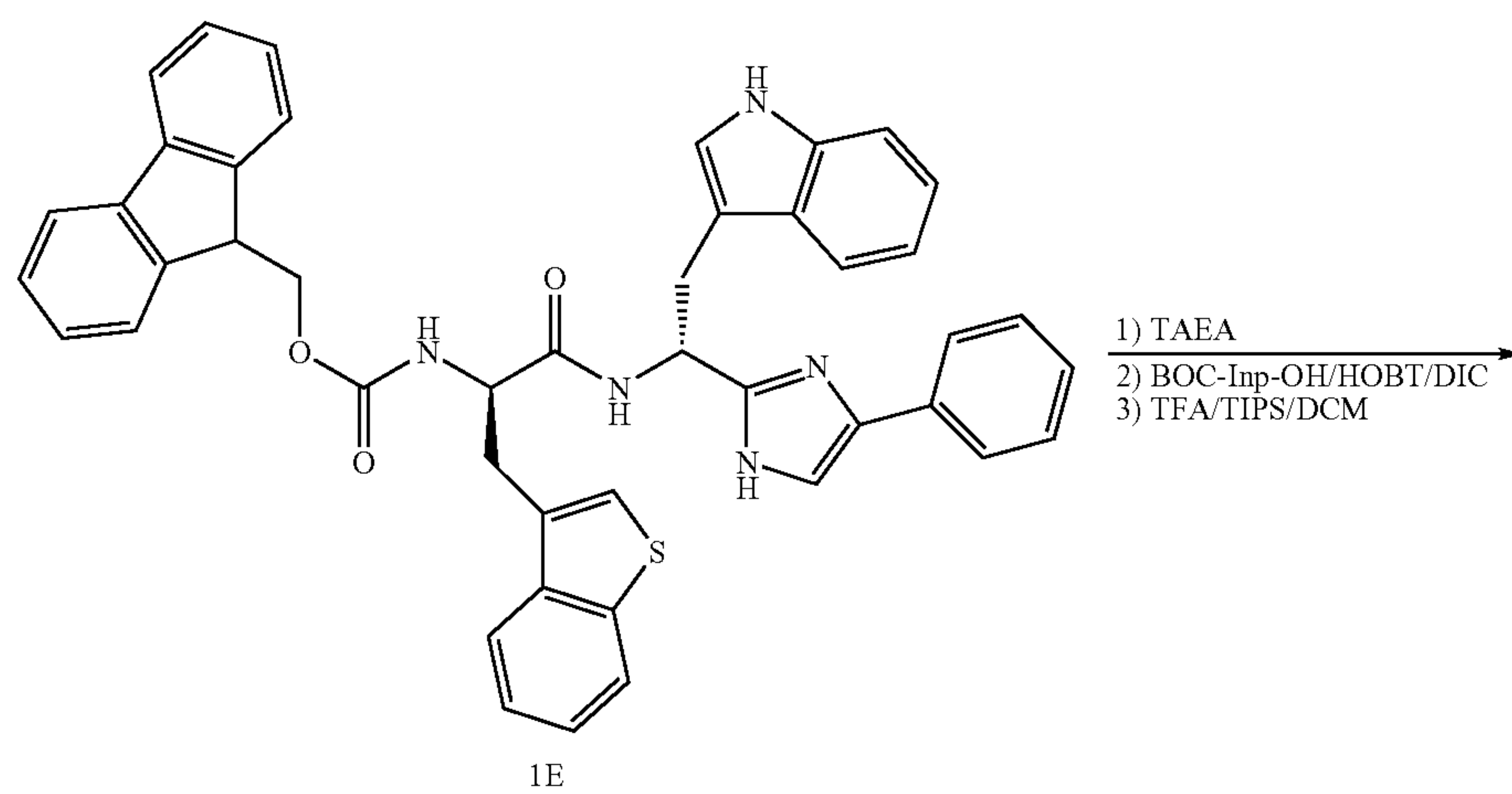
Scheme II
