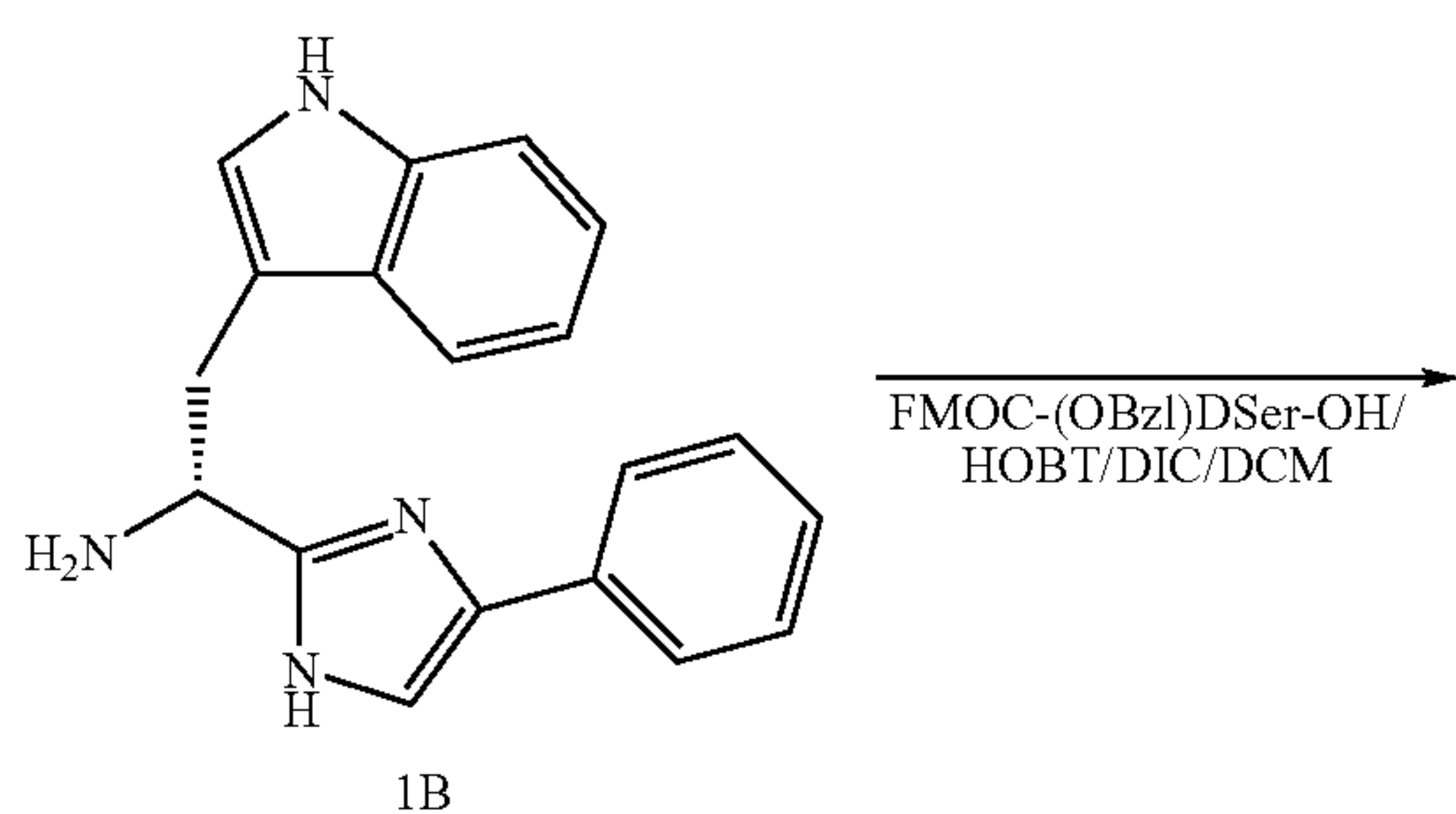
Scheme 1F
