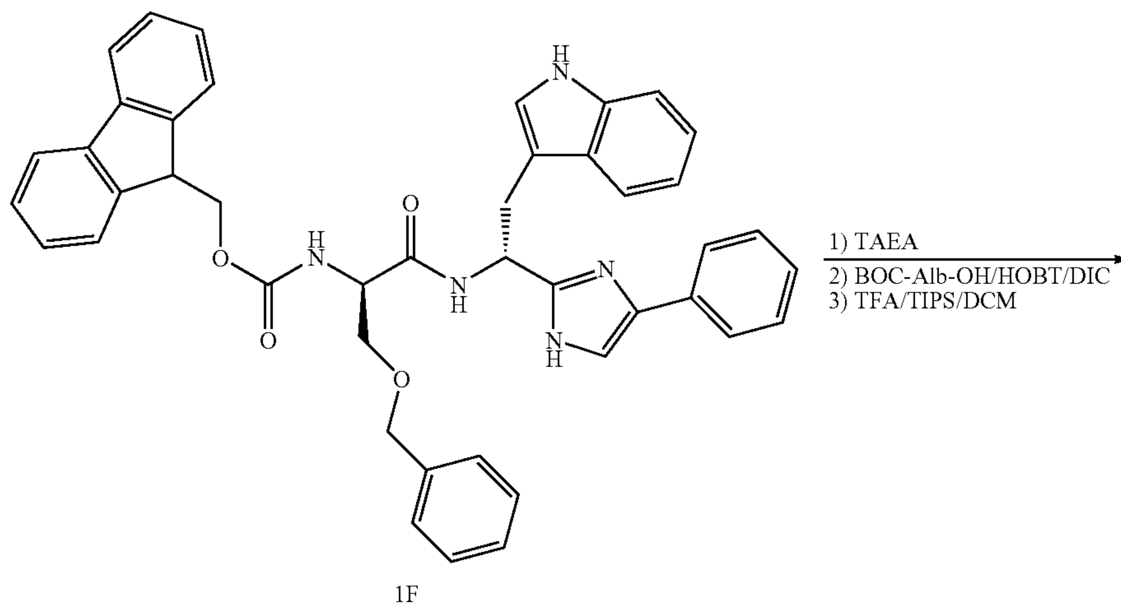
Scheme 1J
