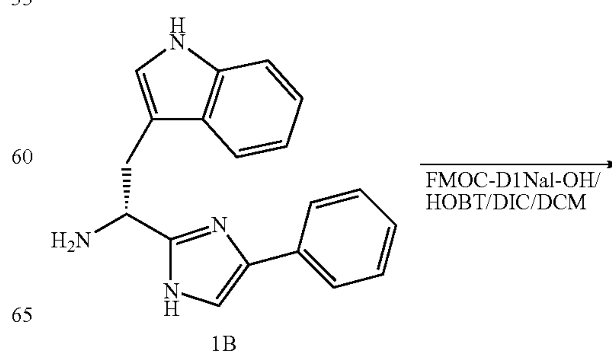
Scheme 1D
