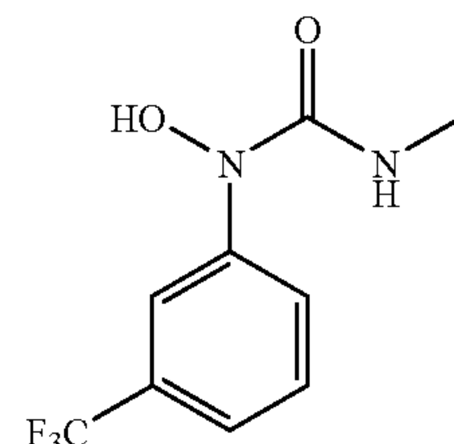
Formula (I)
