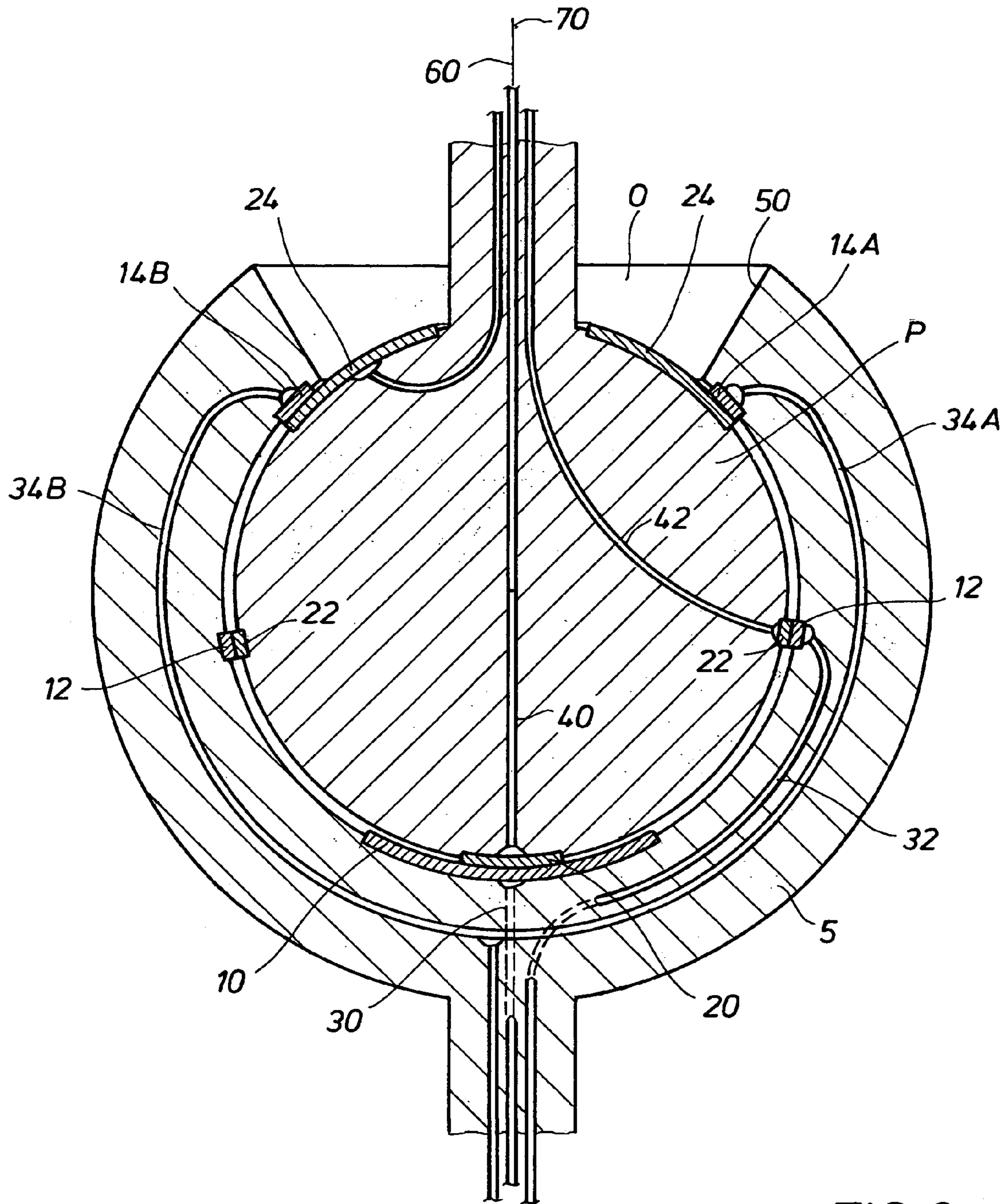
FIG. 2 (PRIOR ART)
