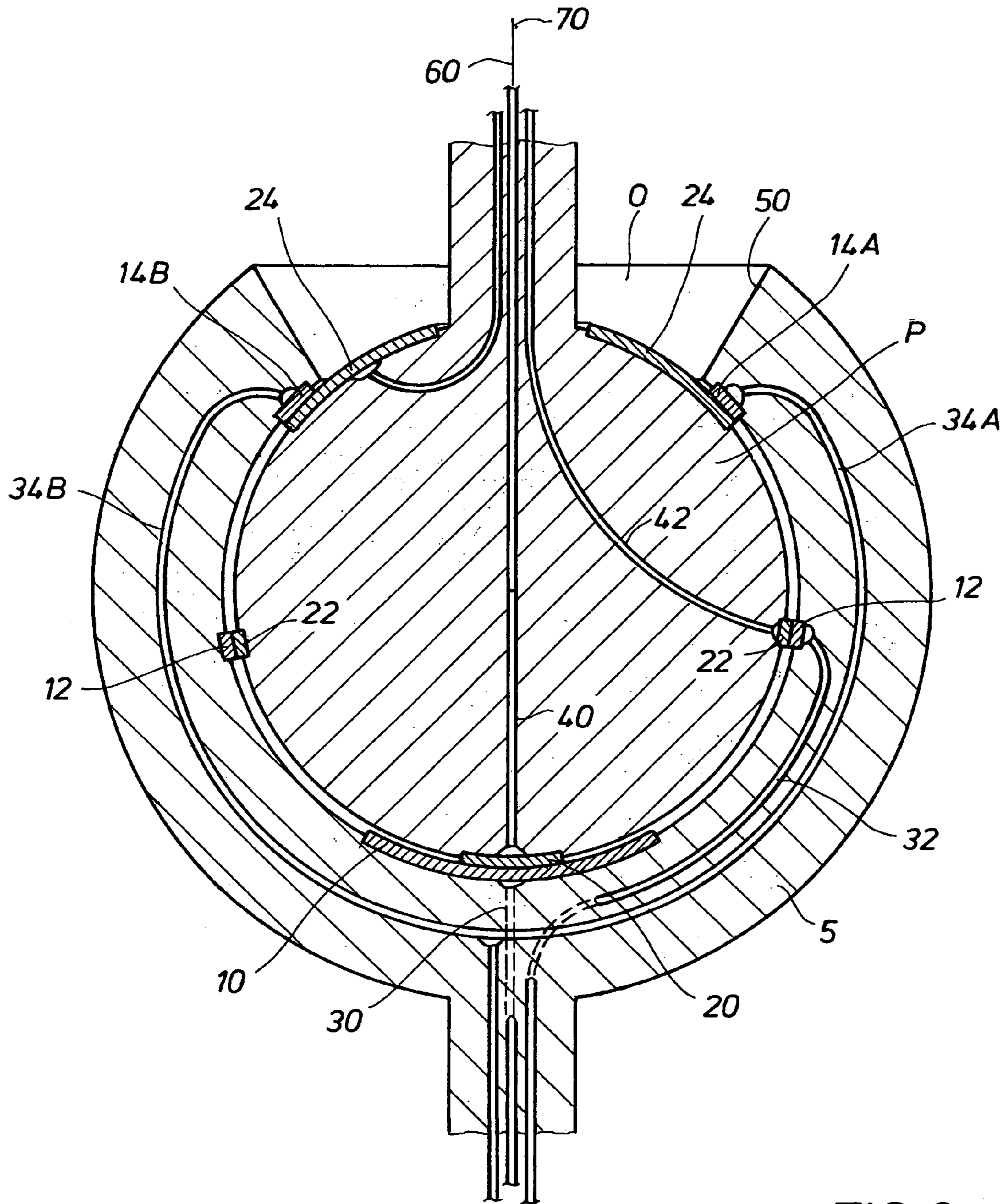
FIG. 2 (PRIOR ART)
