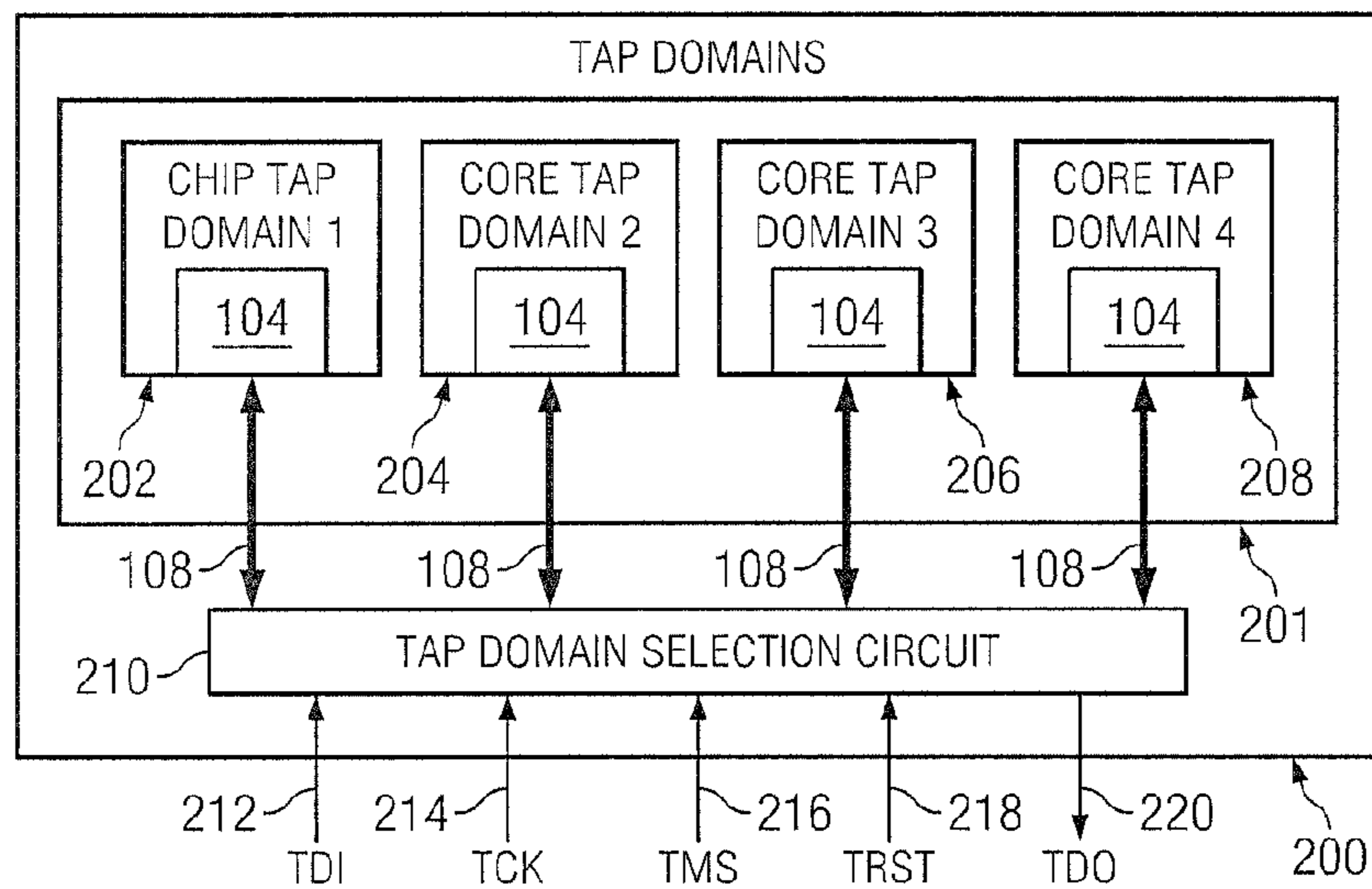
FIG. 2 (PRIOR ART)
