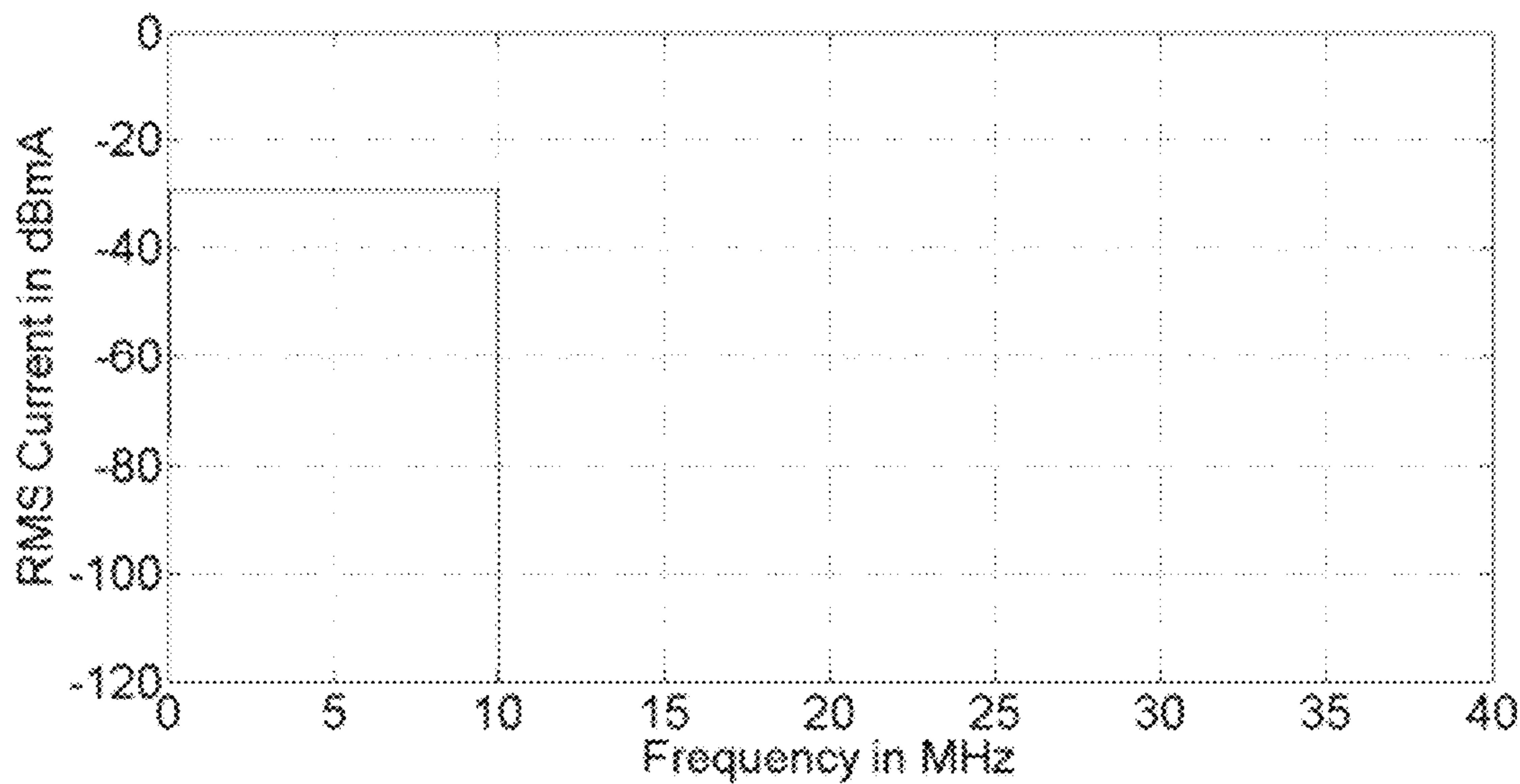
Frequency Response of an OFDM sequence of a flat 10 MHz bandwidth and sampled at 80 MHz
