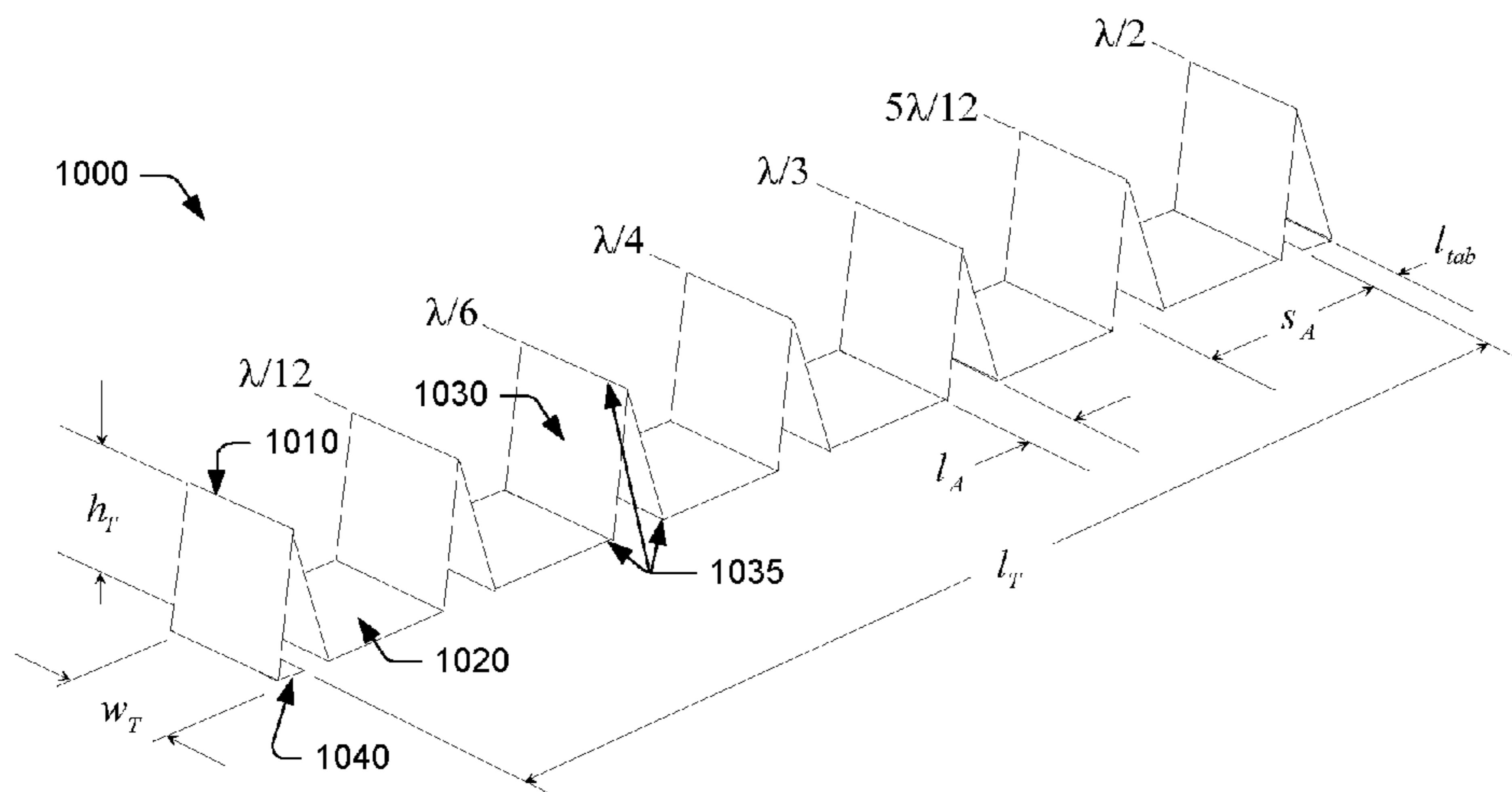
FIG. 10B FOLDED PATTERN
