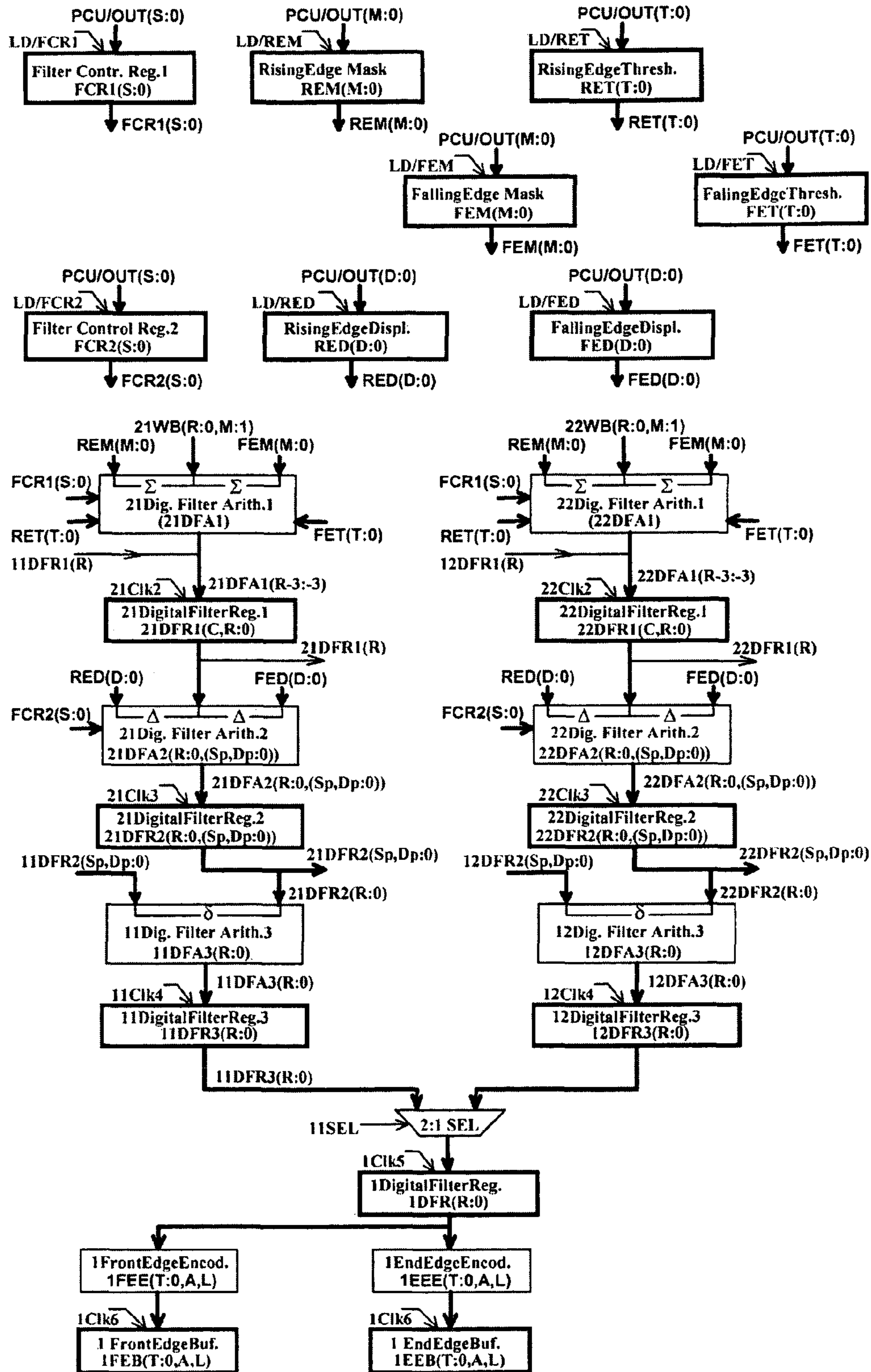
FIG.10 Noise Filtering Edge Detectors (NFED)
