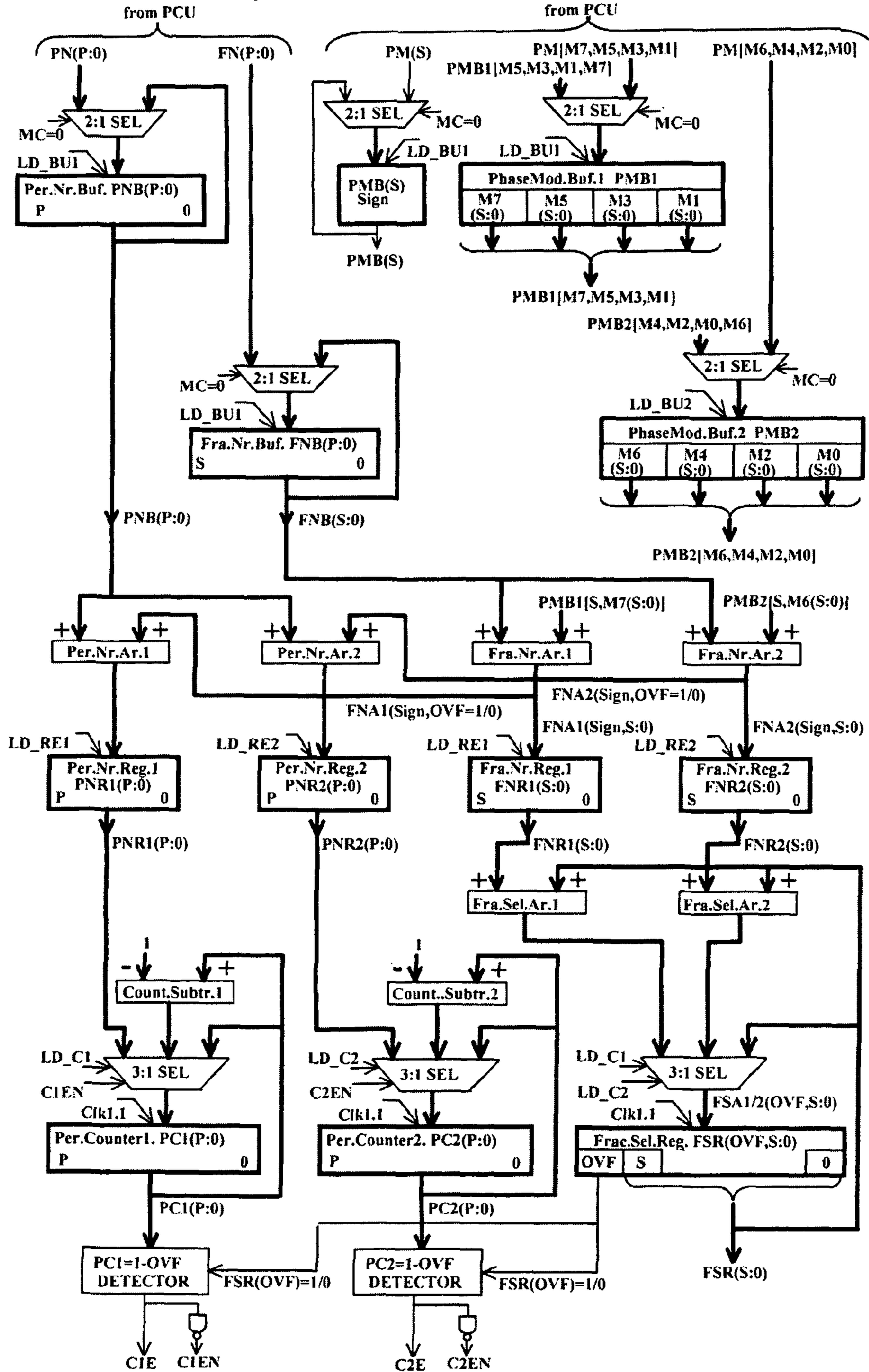
FIG.6 Synchronous Sequential Phase Processor (SSPP)
