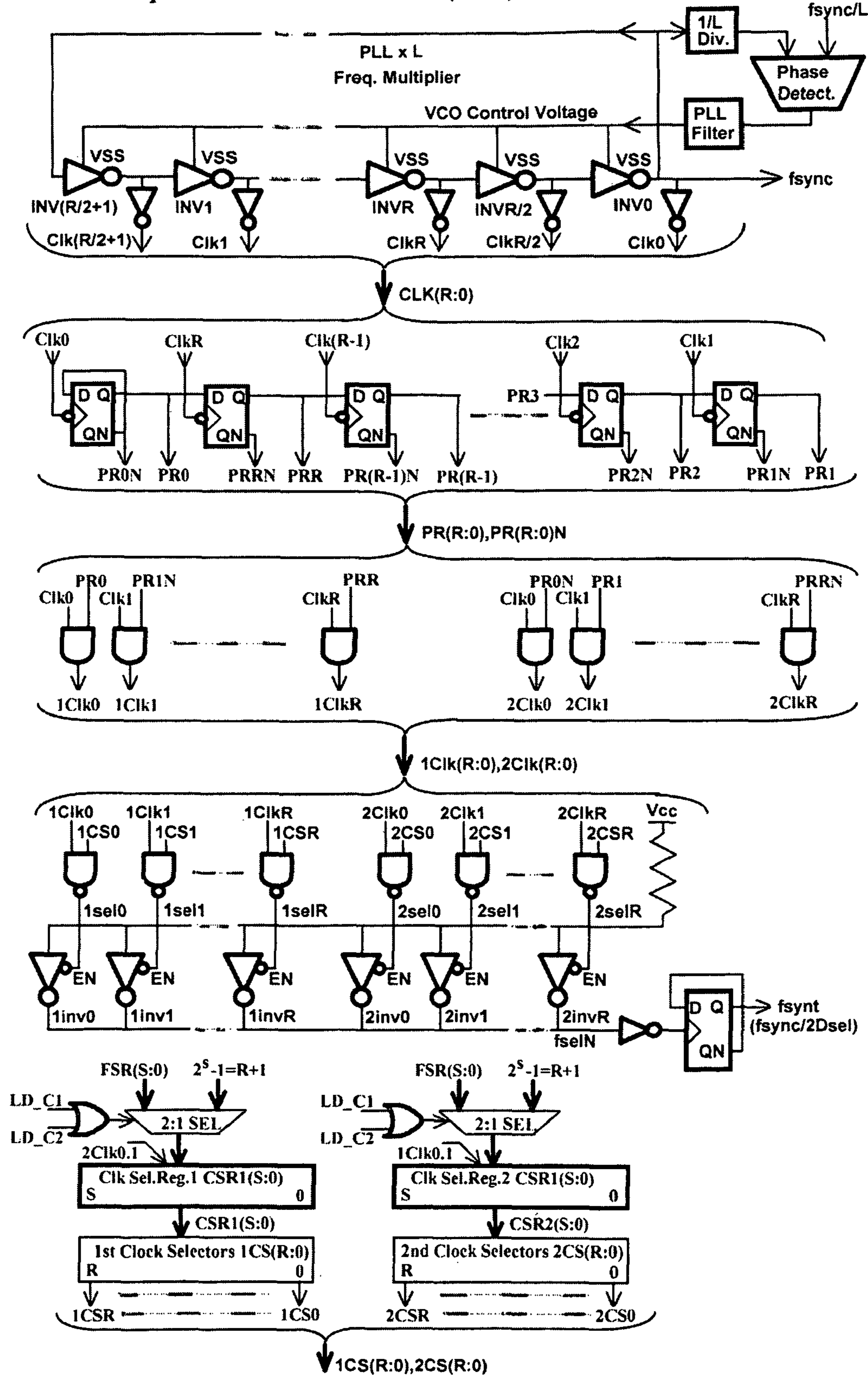
FIG.4 Sequential Clocks Generator (SCG) and Output Selection Circuits (OSC)
