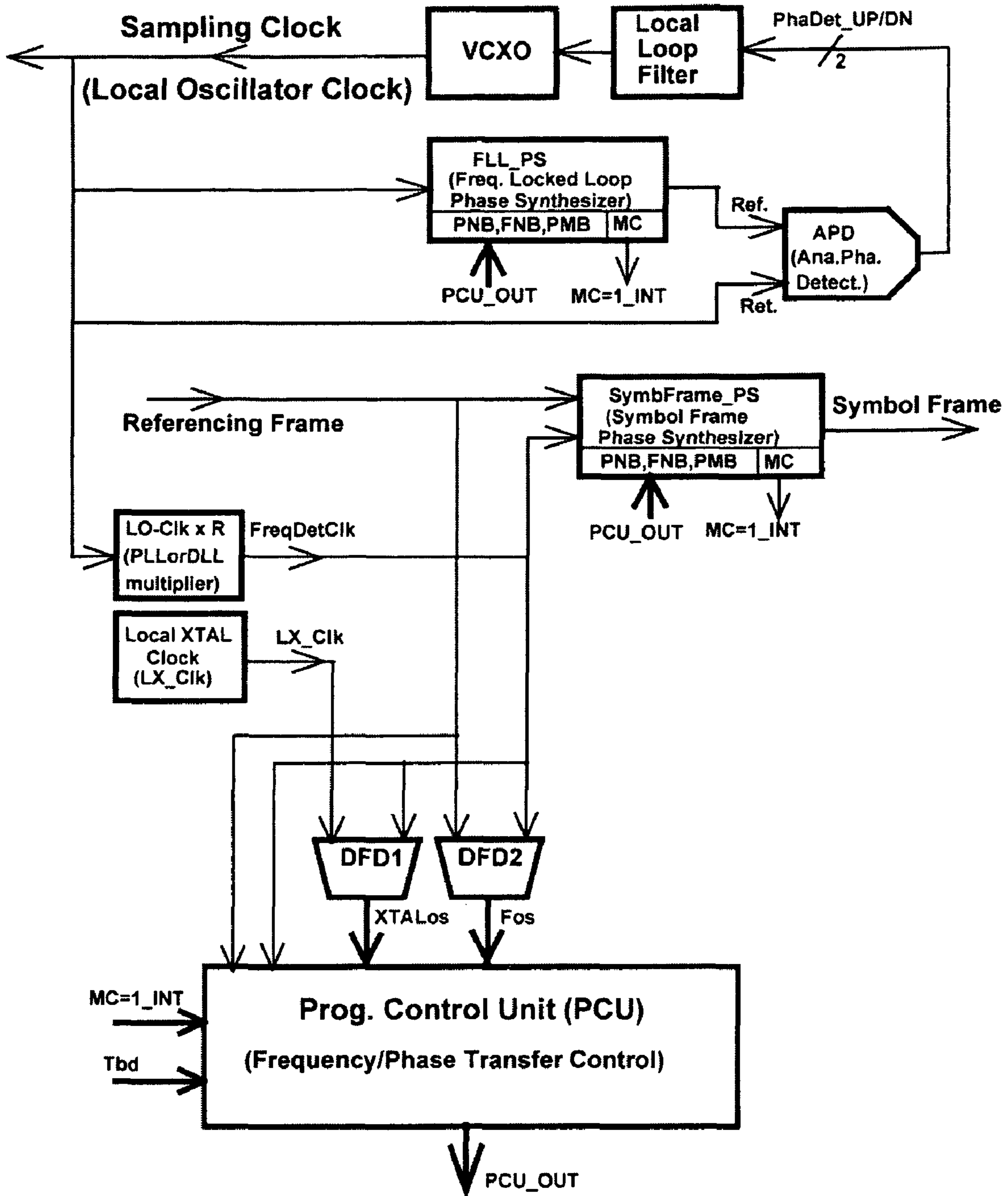
FIG.18 High Accuracy FLPS
