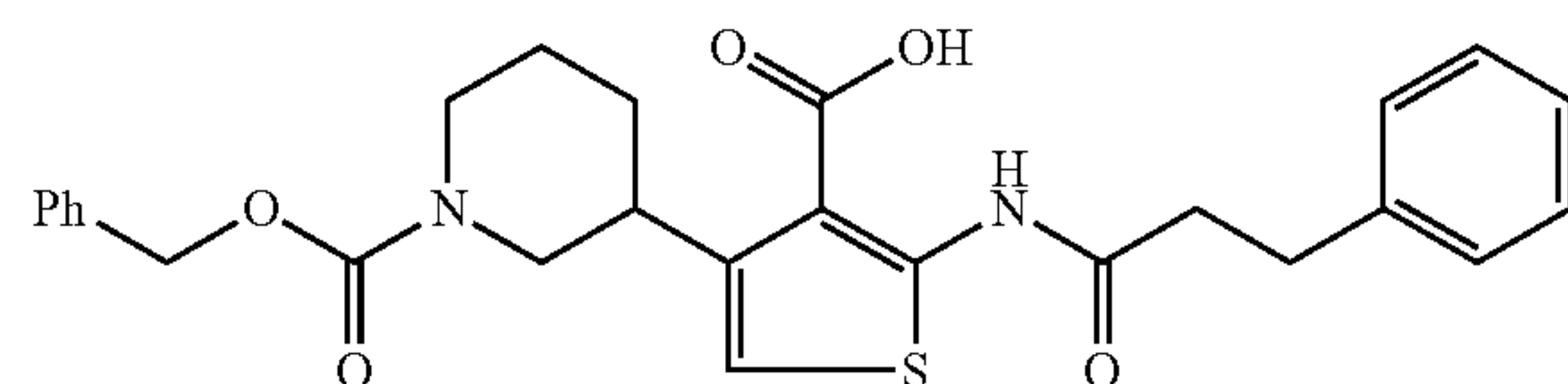
4-(1-(benzyloxycarbonyl)piperidin-3-yl)-2-(3-phenylpropanamido)thiophene-3-carboxylic acid (58)
