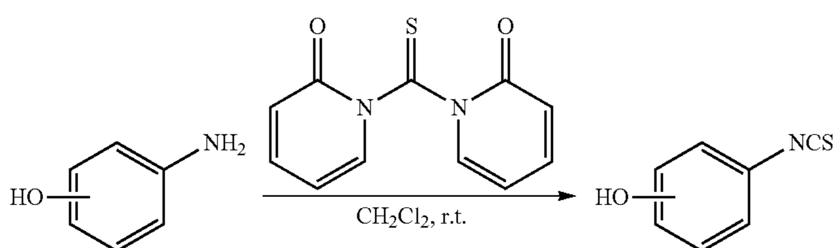
Scheme XIV
