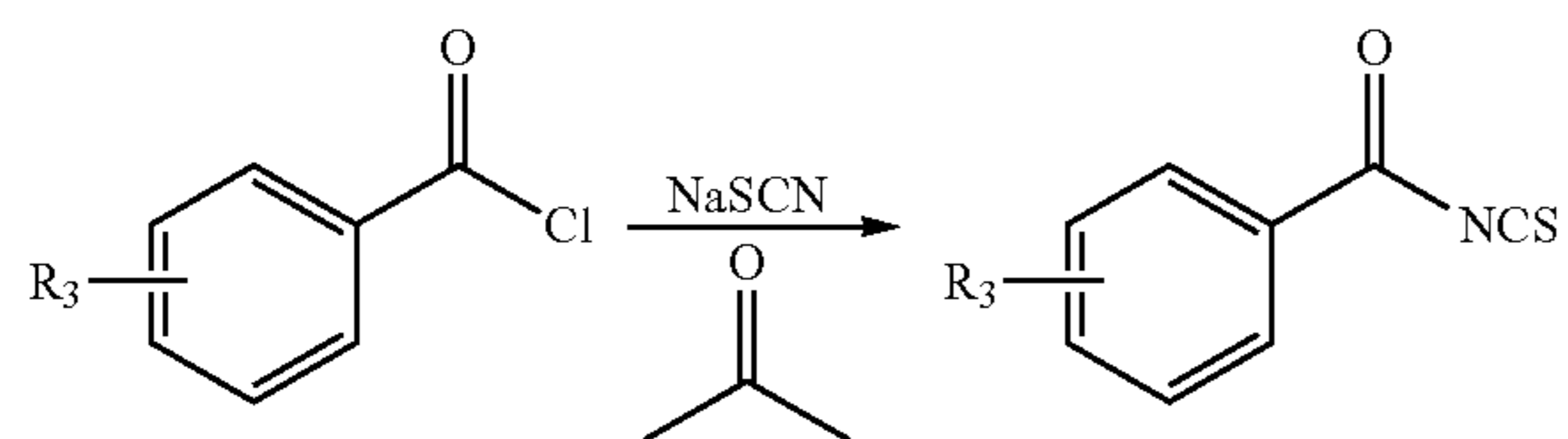
Scheme IX
