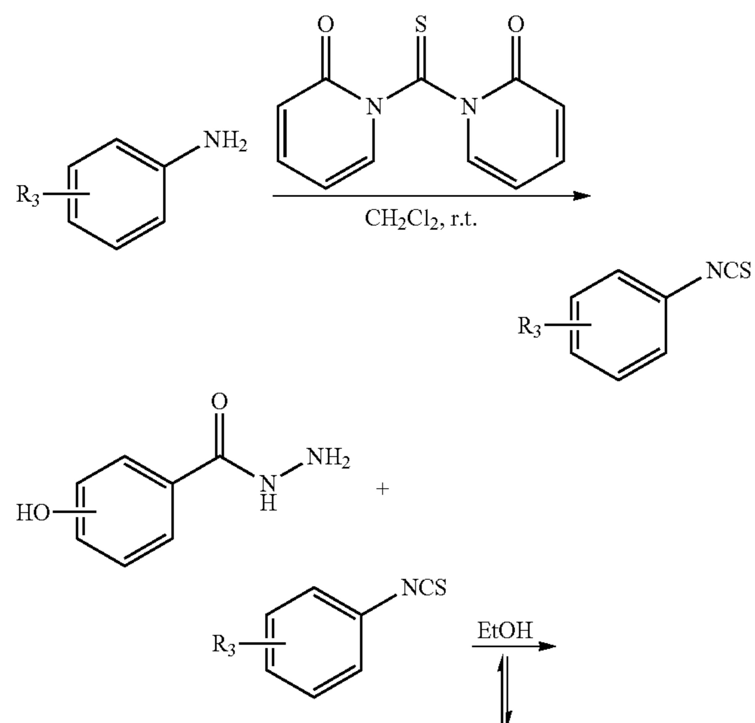
Scheme XI
