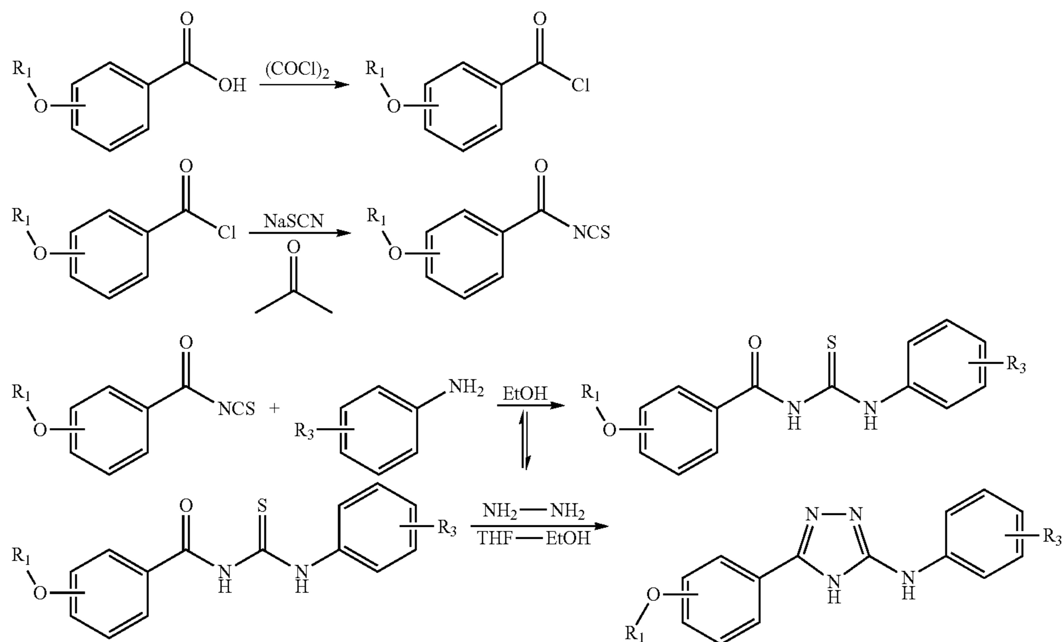
Scheme VII
