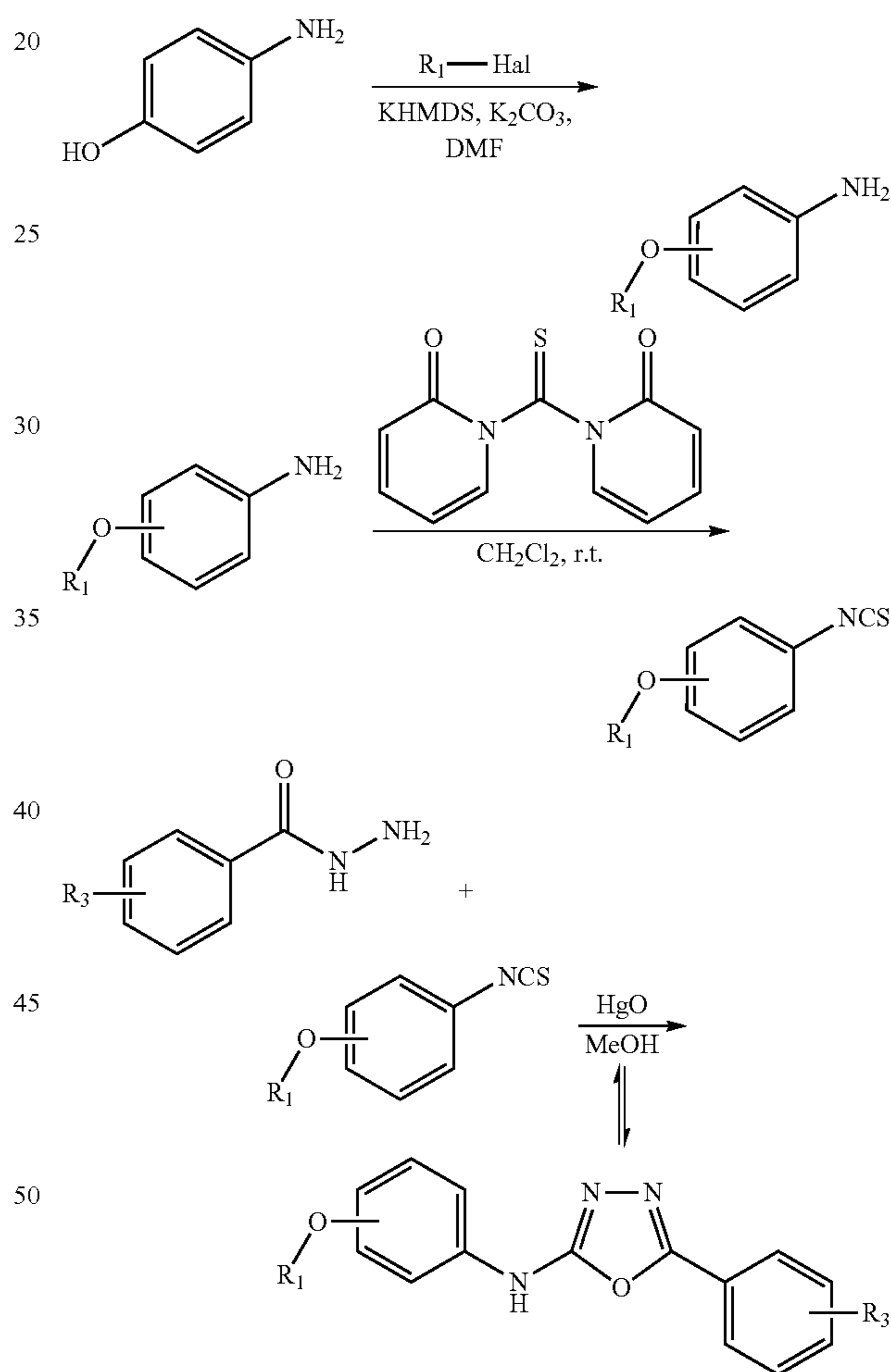
Scheme XIII
