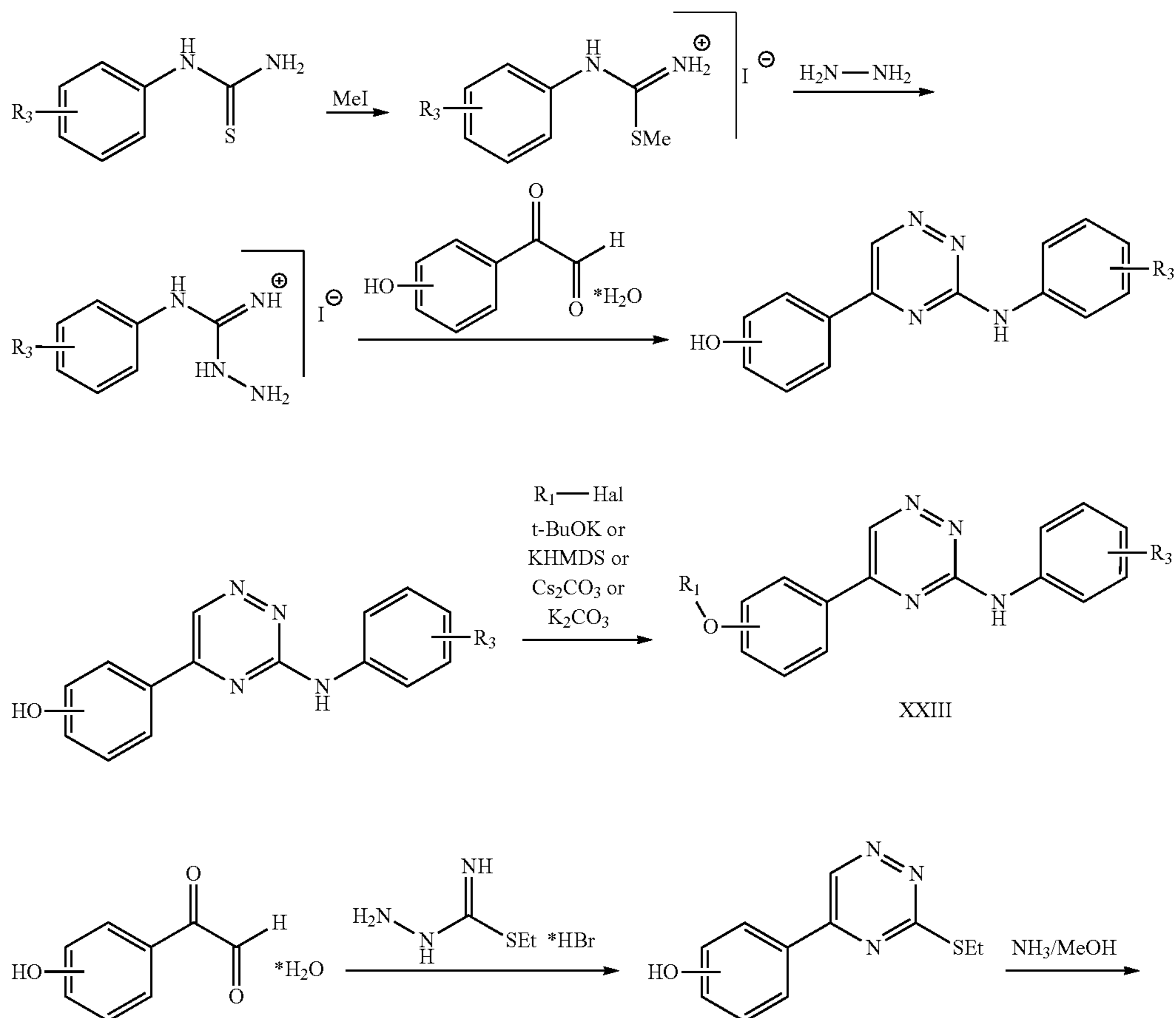
Scheme XVII
