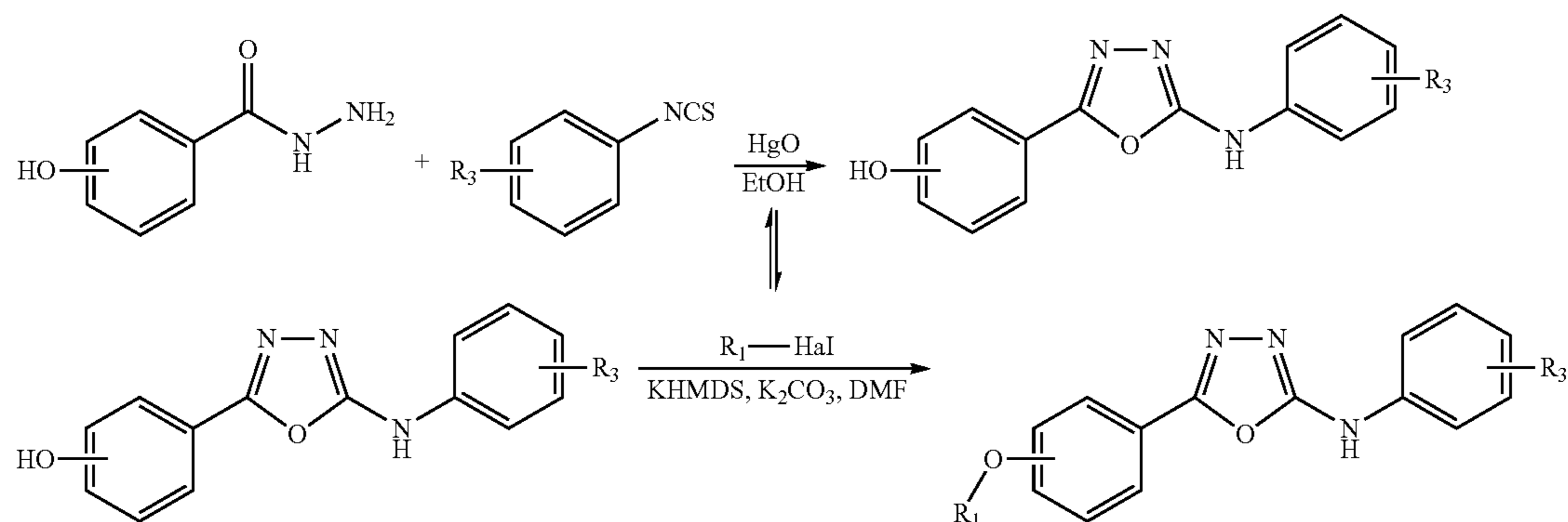
Scheme X
