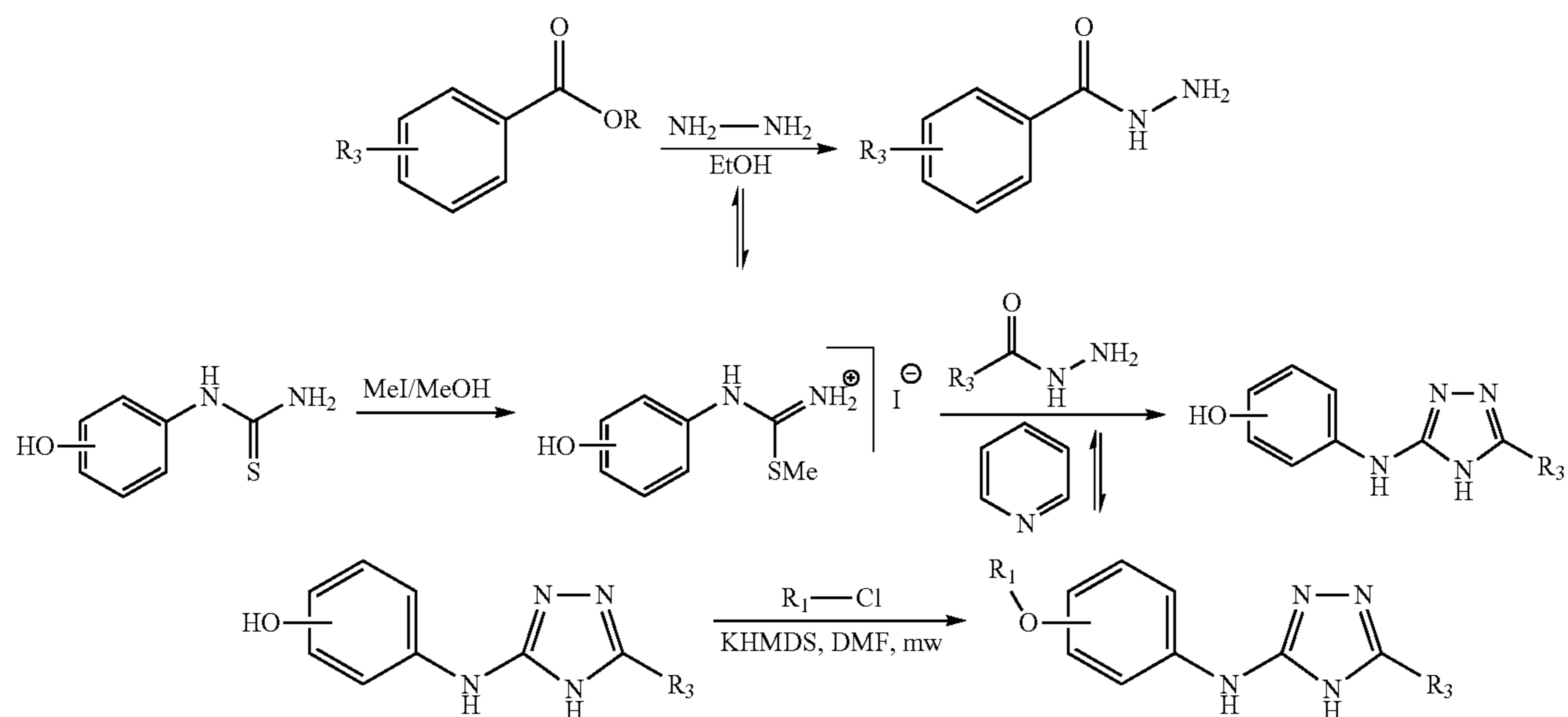
Scheme VIII
