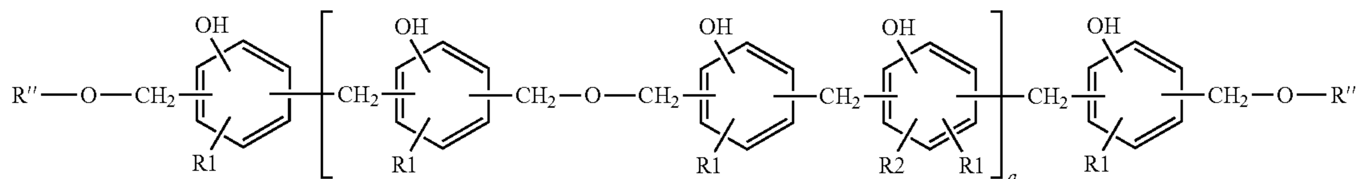
Formula (VIIIa)
