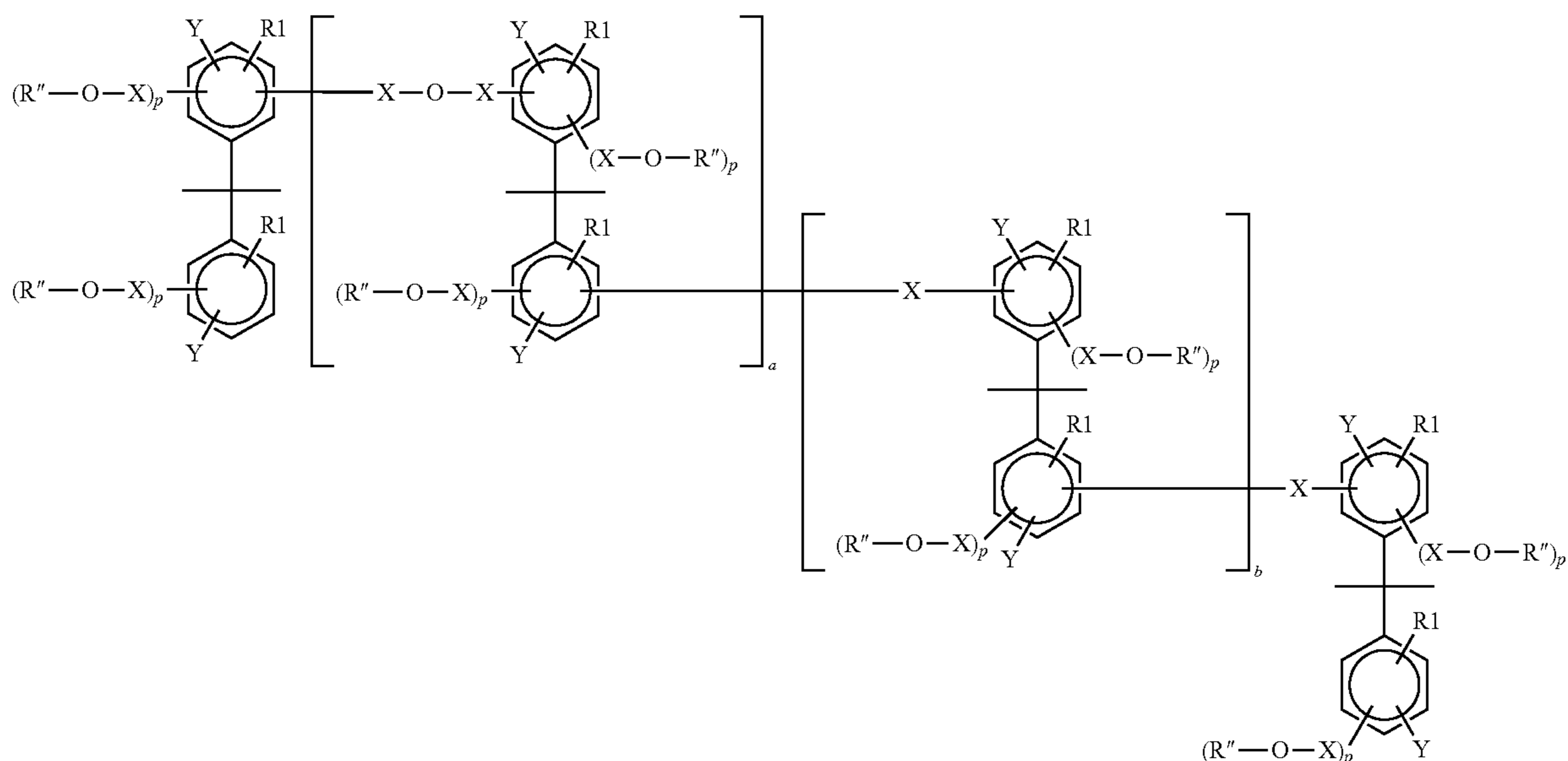
Formula (VI)
