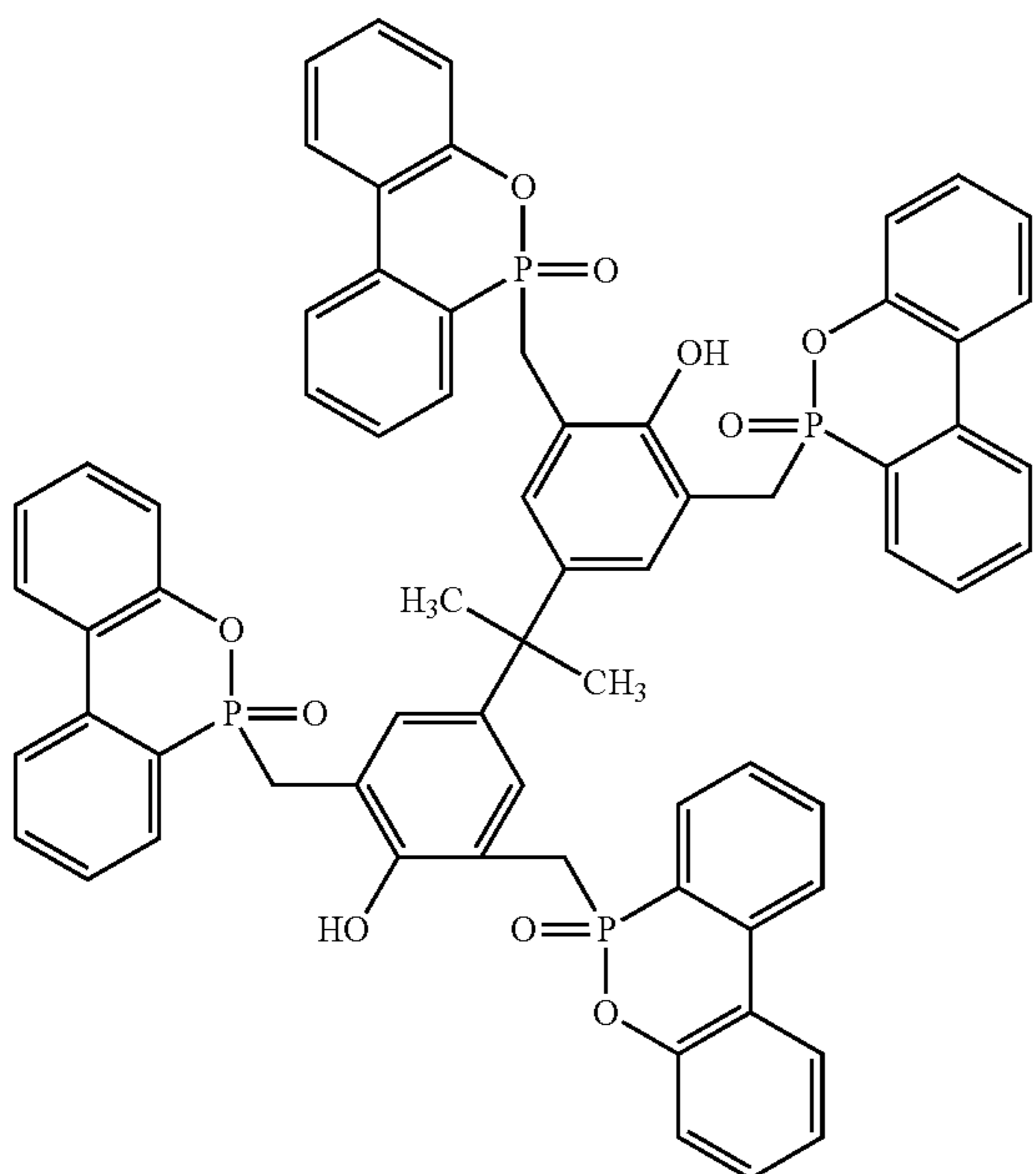
Example 9
