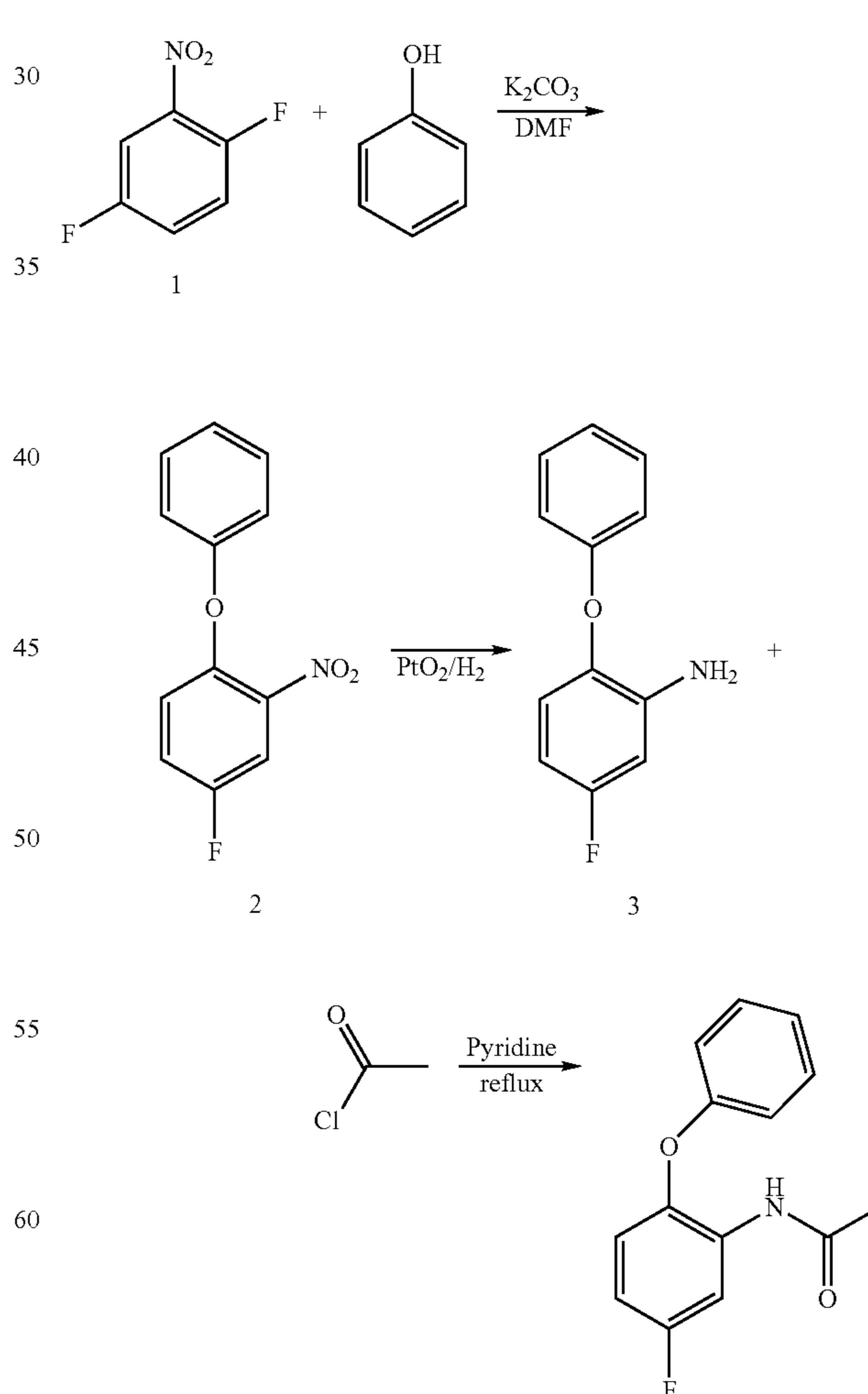
Scheme 4 - Synthesis of conjugatable DAA1106
