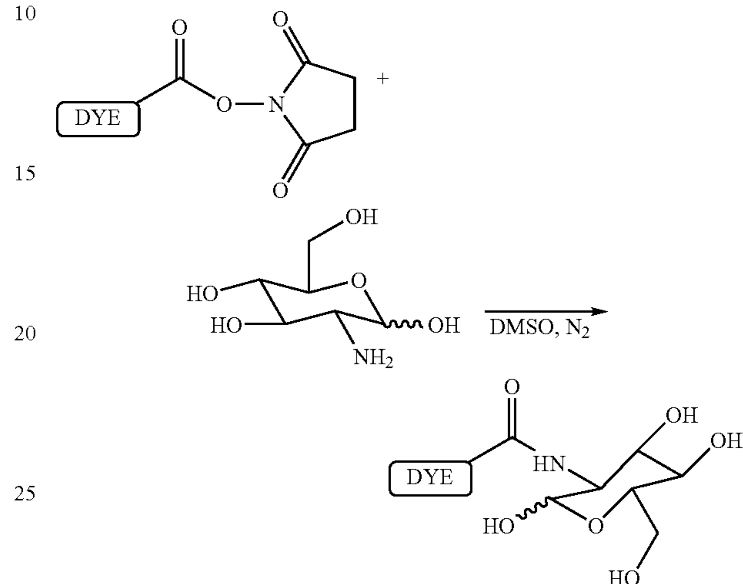
Scheme 2- Conjugation of Succinimidyl Dye to glucosamine
