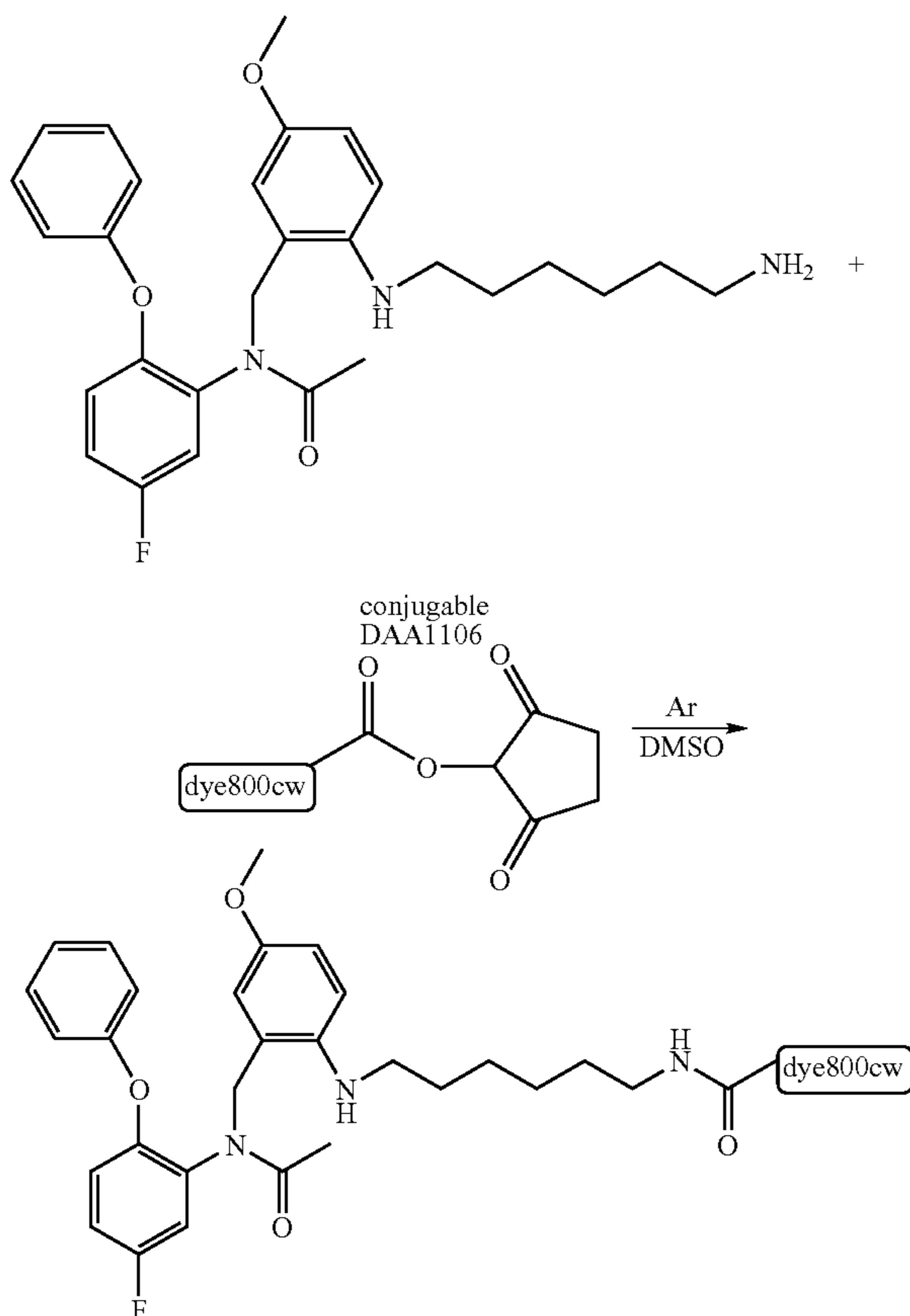
Scheme 5. Reaction scheme for dye800CW-DAA1106
