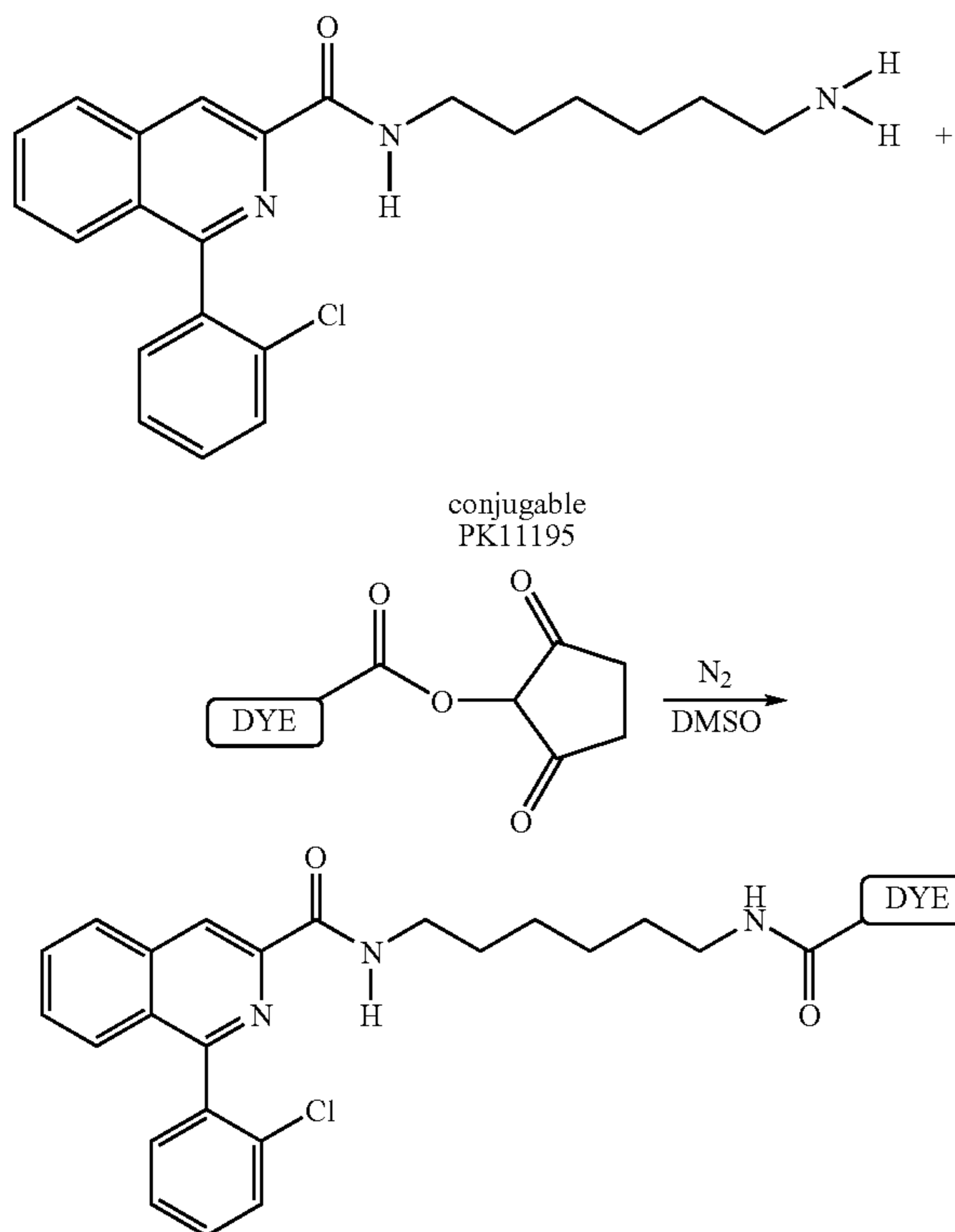
Scheme 1 - Conjugation of Succinimidyl Dye to conjugable PK11195
