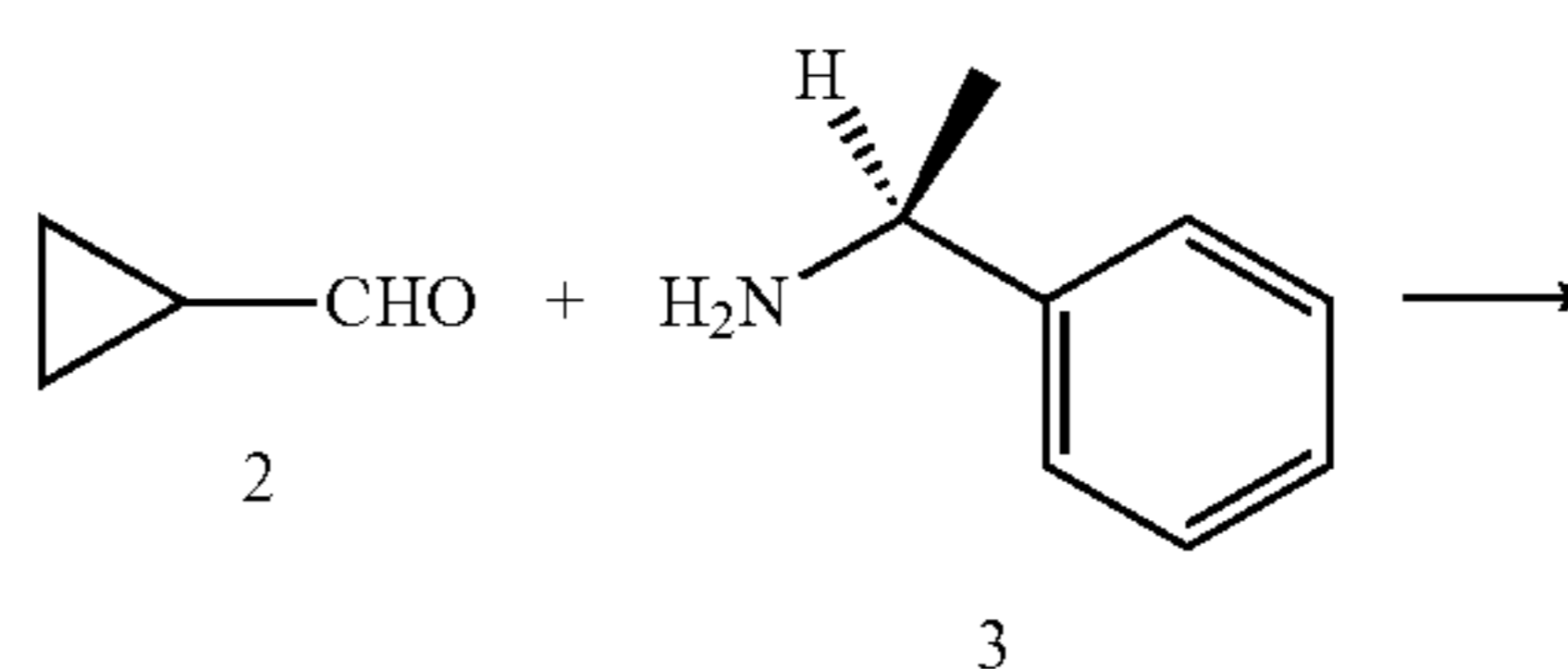
Scheme 1.
