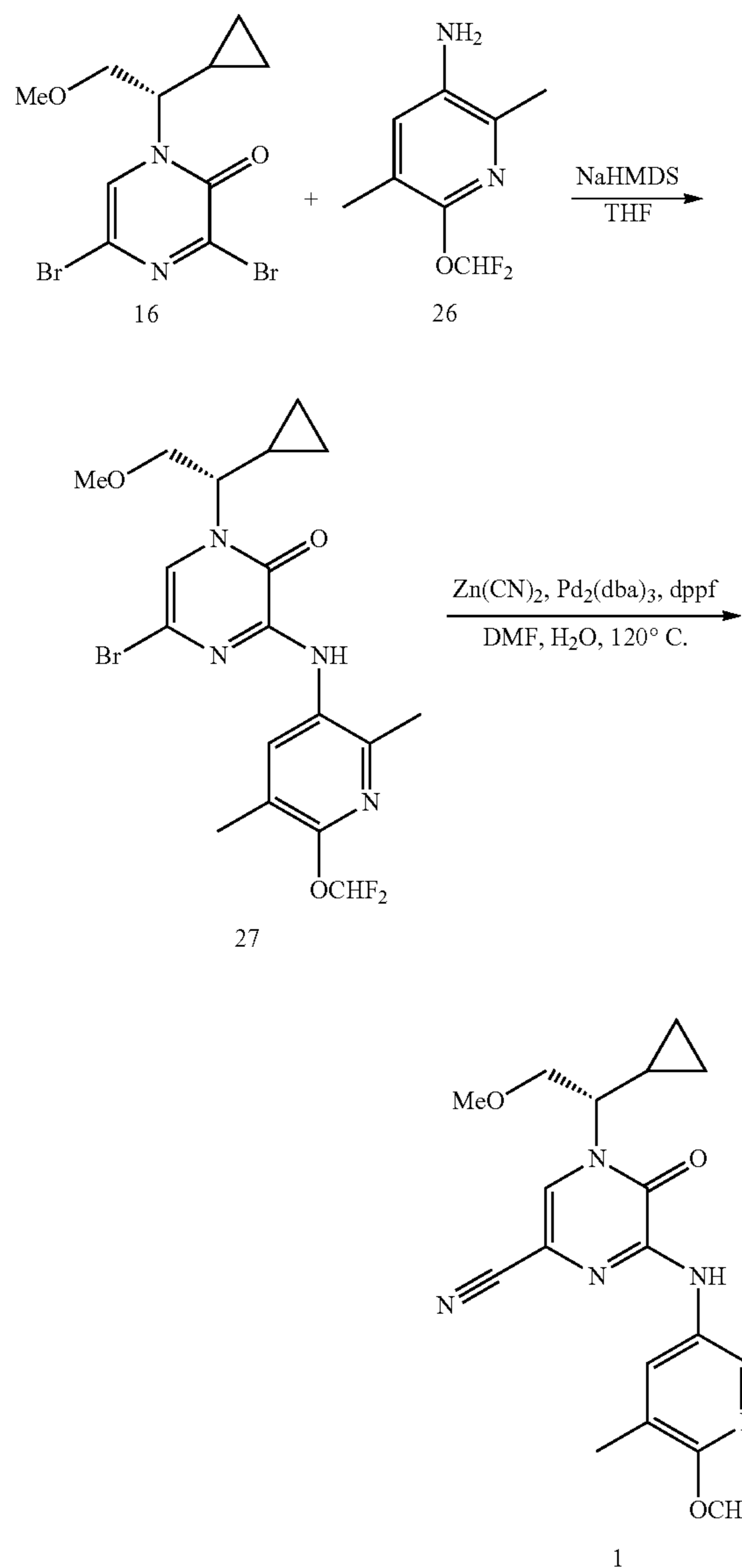
Scheme 6.
