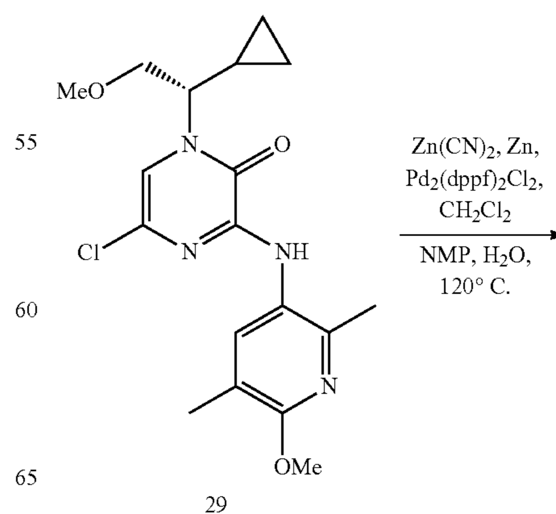
Scheme 8.
