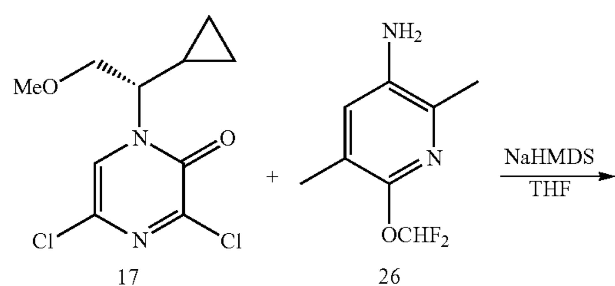
Scheme 7.
