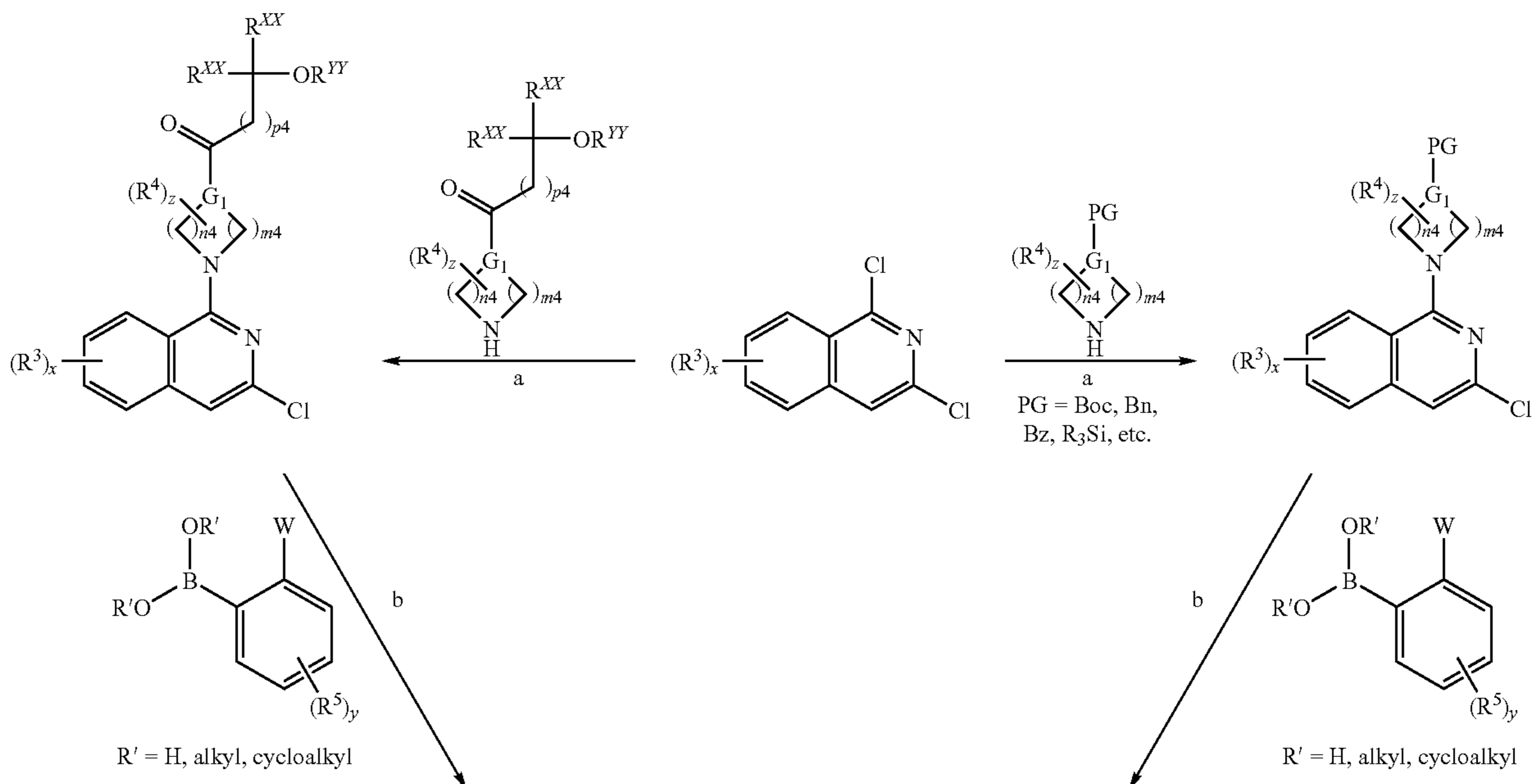
Scheme 15: Compounds of formula IA(nn)
