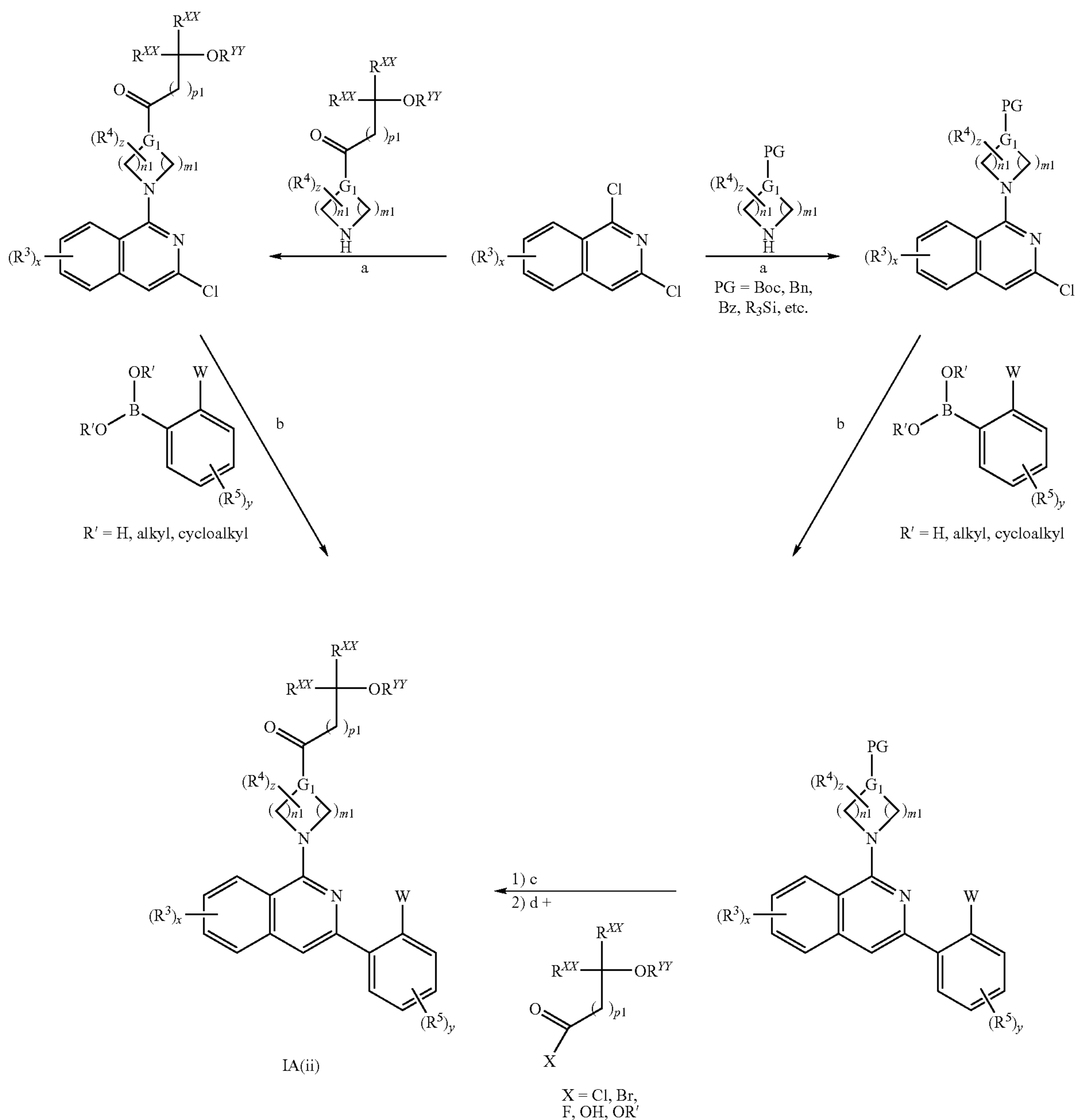
Scheme 10: Compounds of formula IA(ii)
