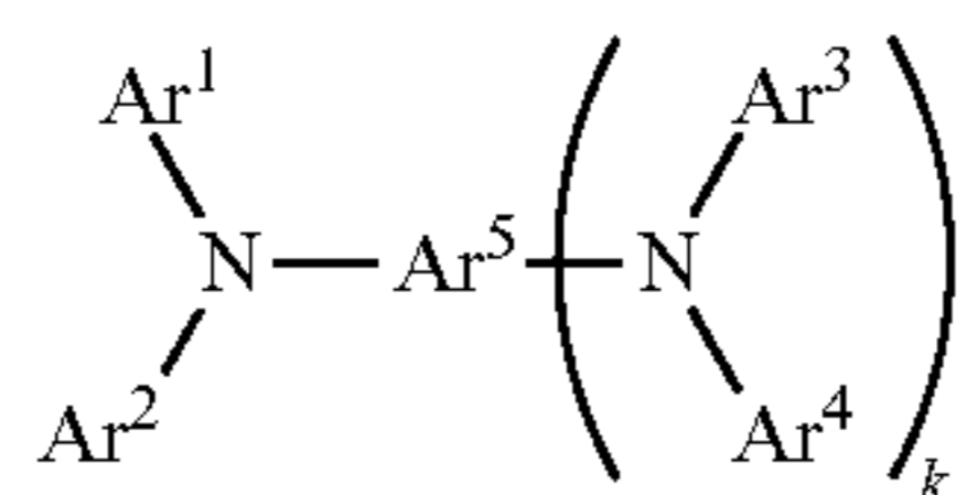
triarylamine
