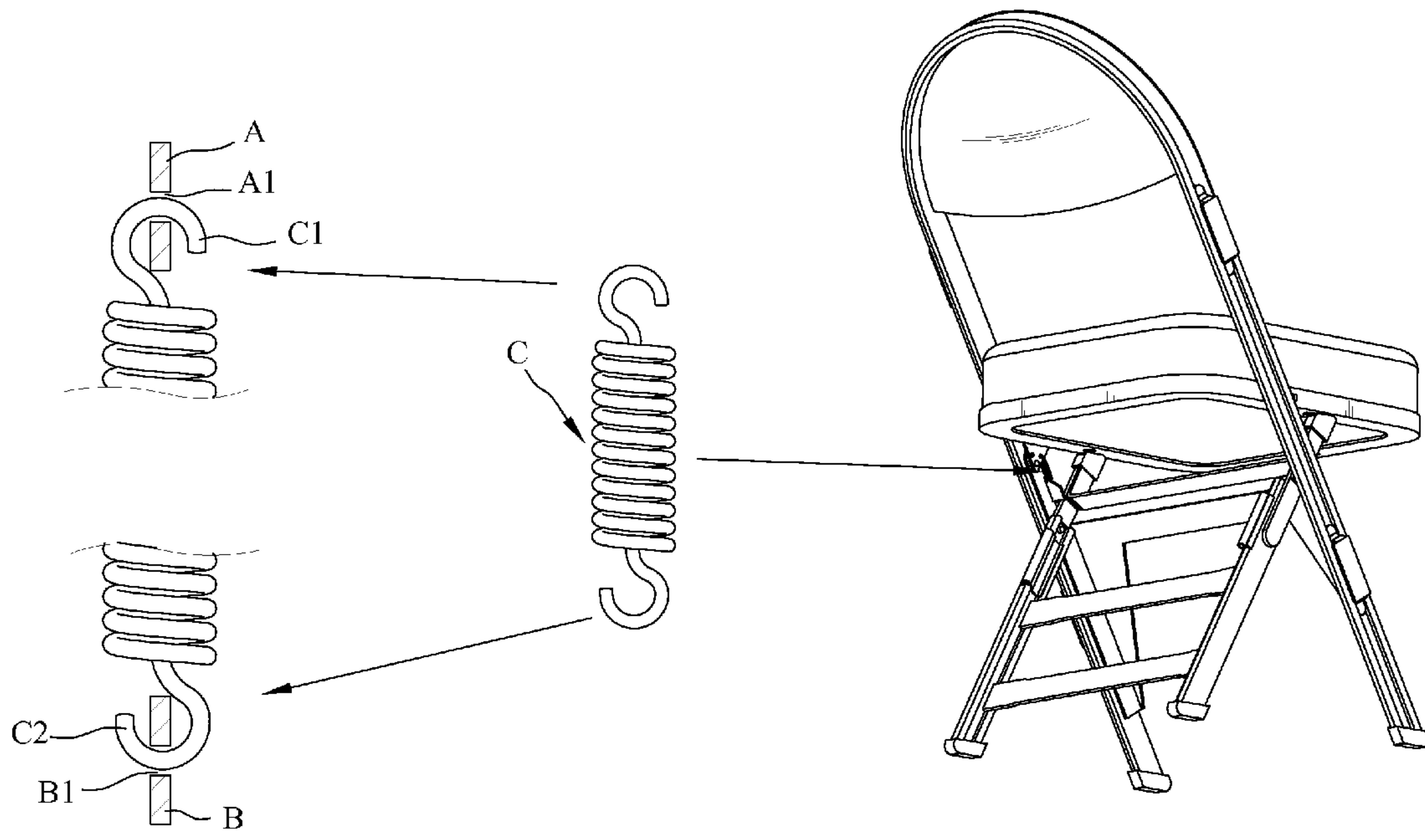
FIG. 8 (PRIOR ART)
