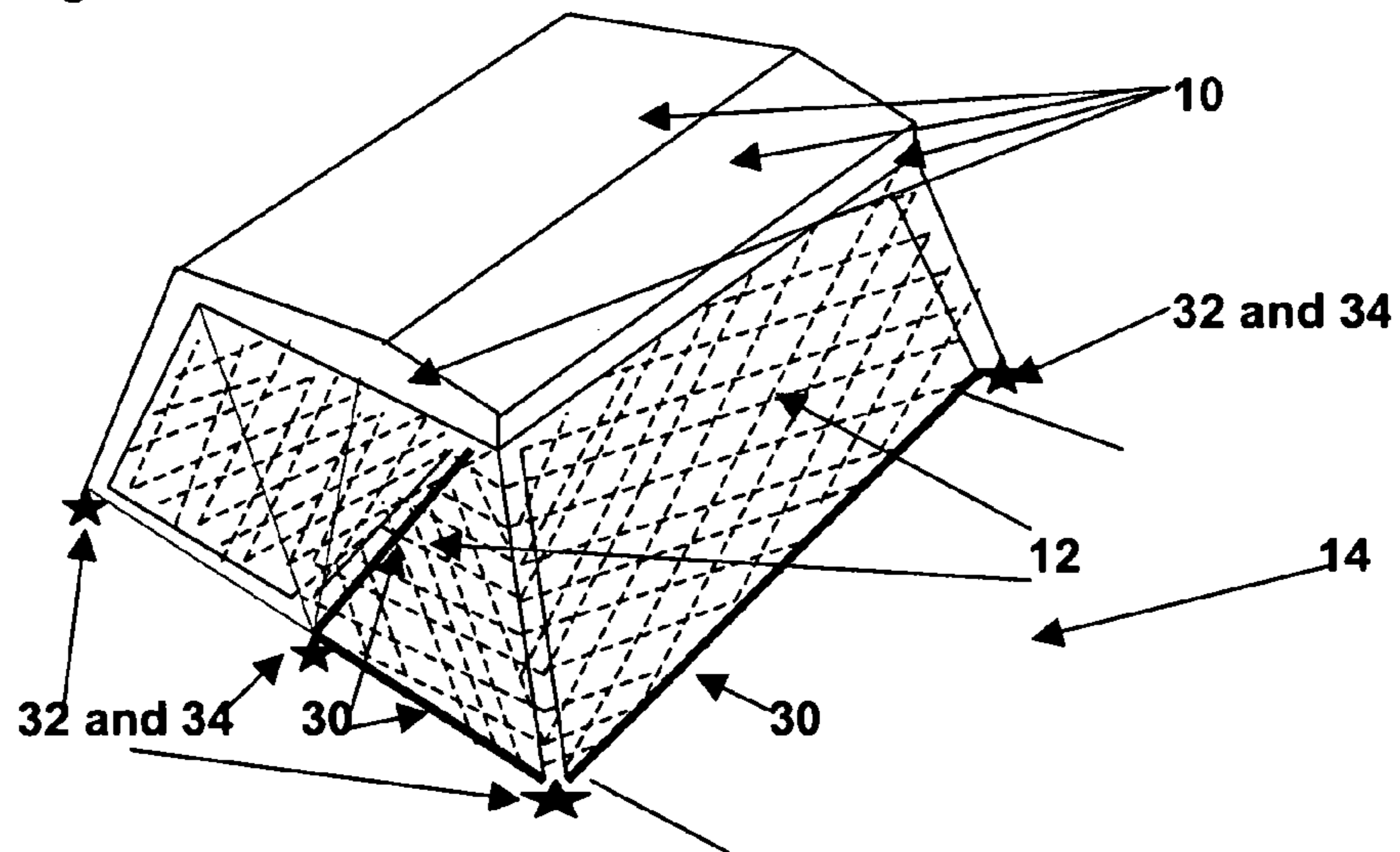
Fig. 8C Front and Left Side with Mesh Enclosure
