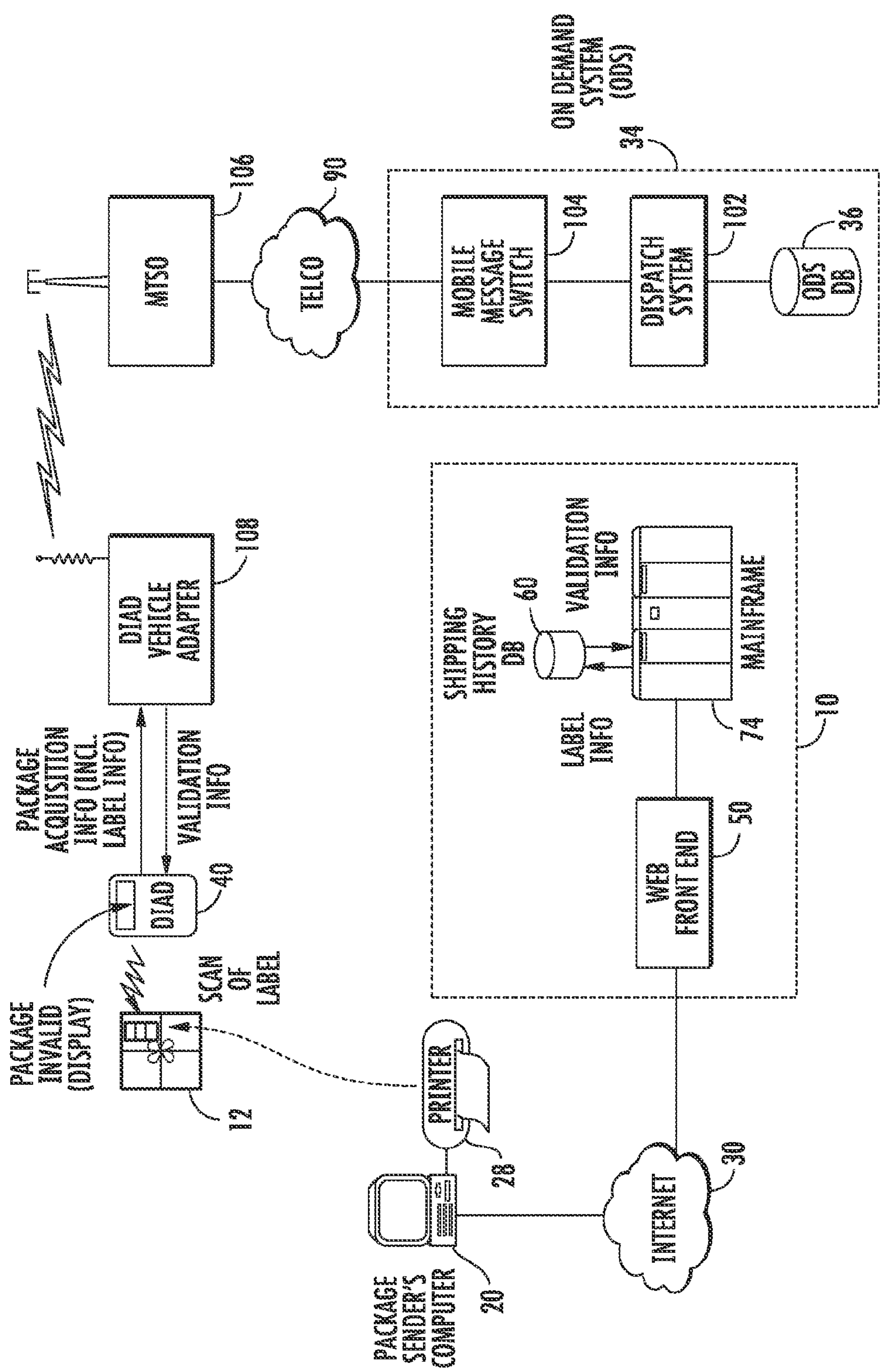
FIG. 3 DISPATCH ARCHITECTURE
