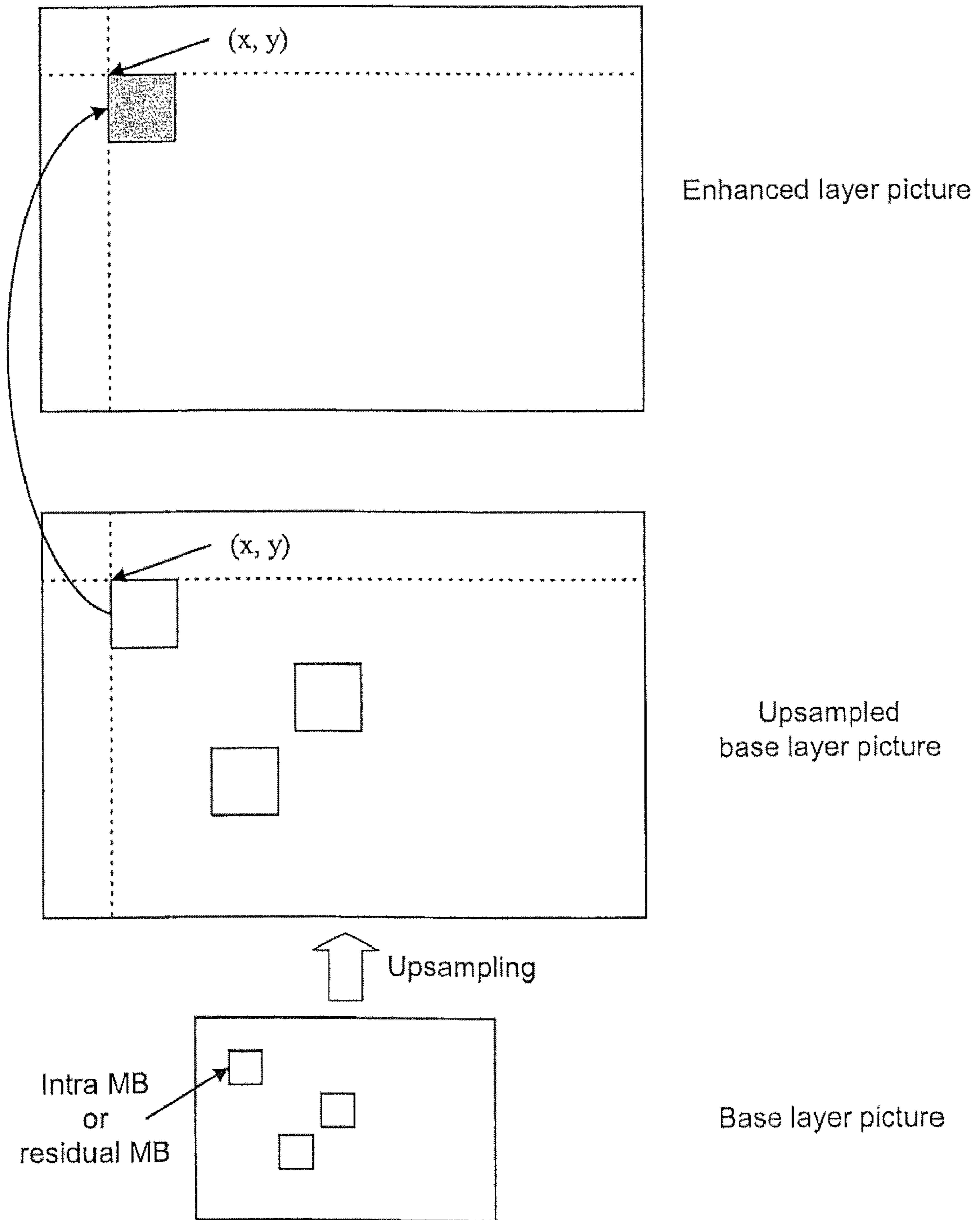
FIG. 1 (PRIOR ART)
