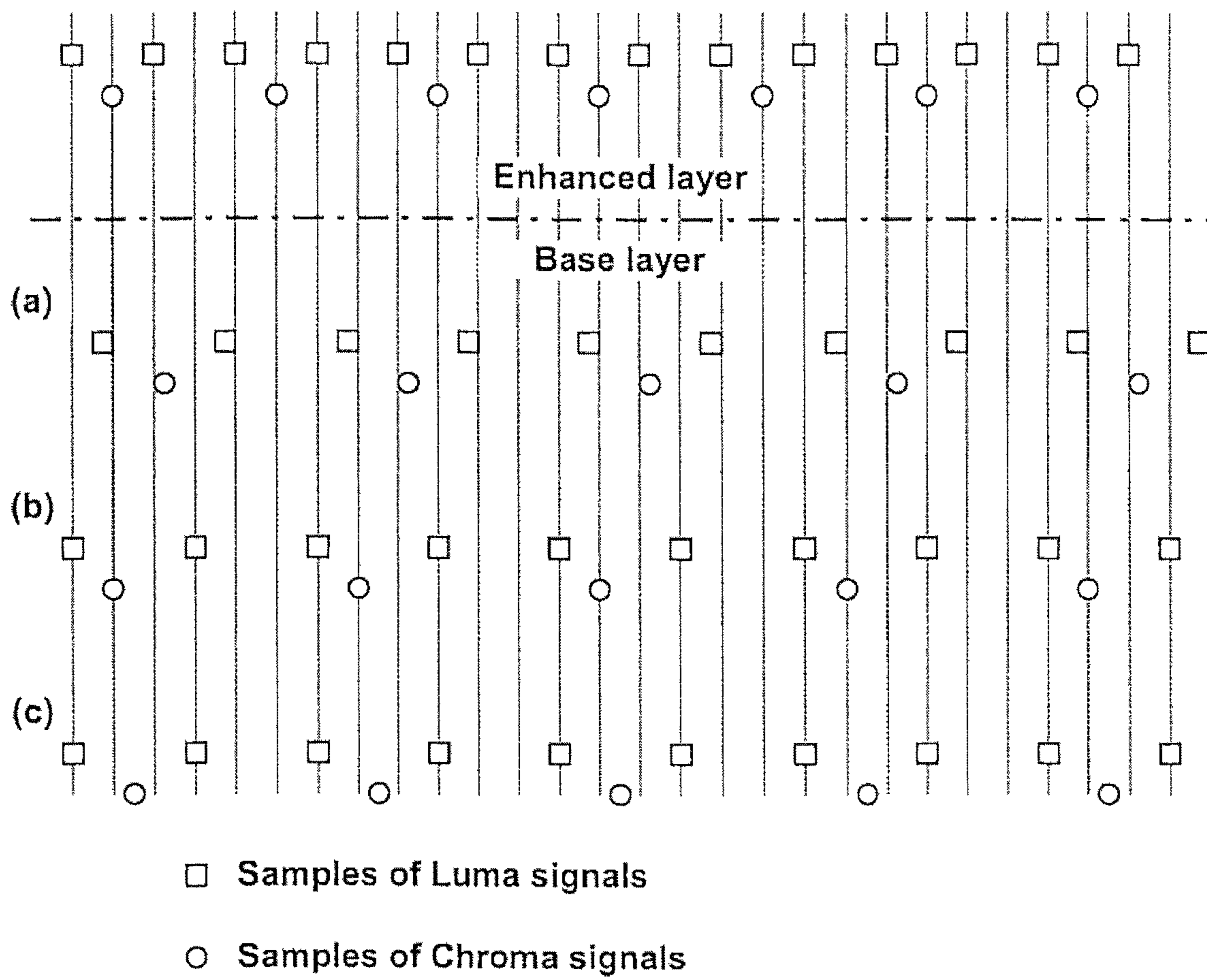
FIG. 2 (PRIOR ART)
