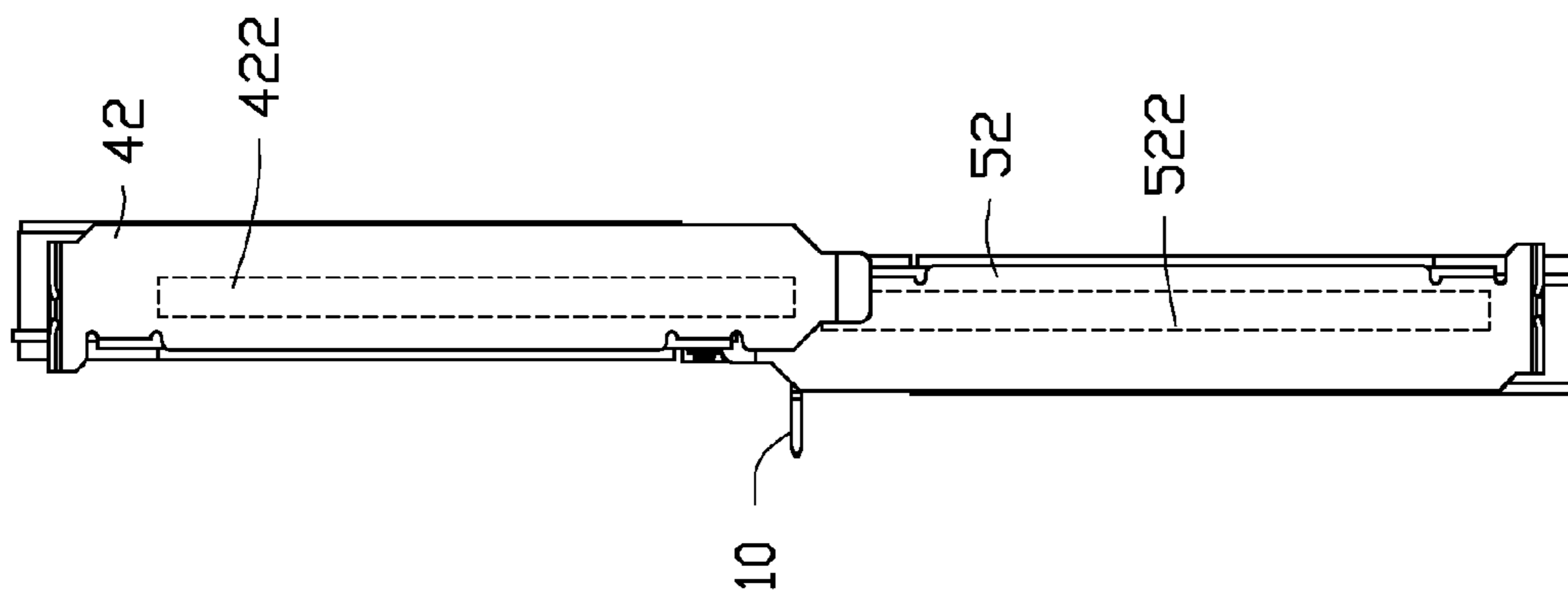
FIG. 10 (Prior Art)
