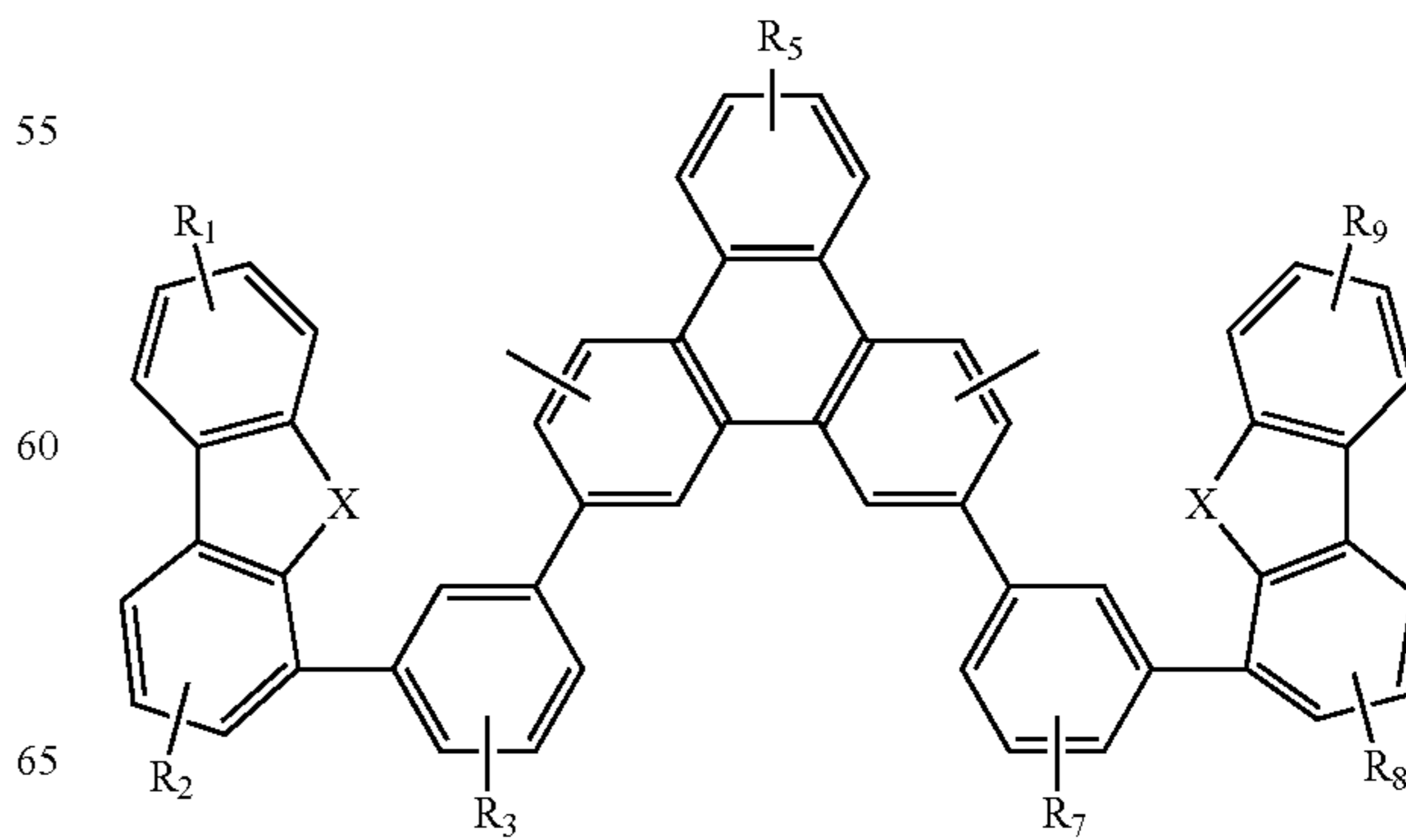
Compound 4G
