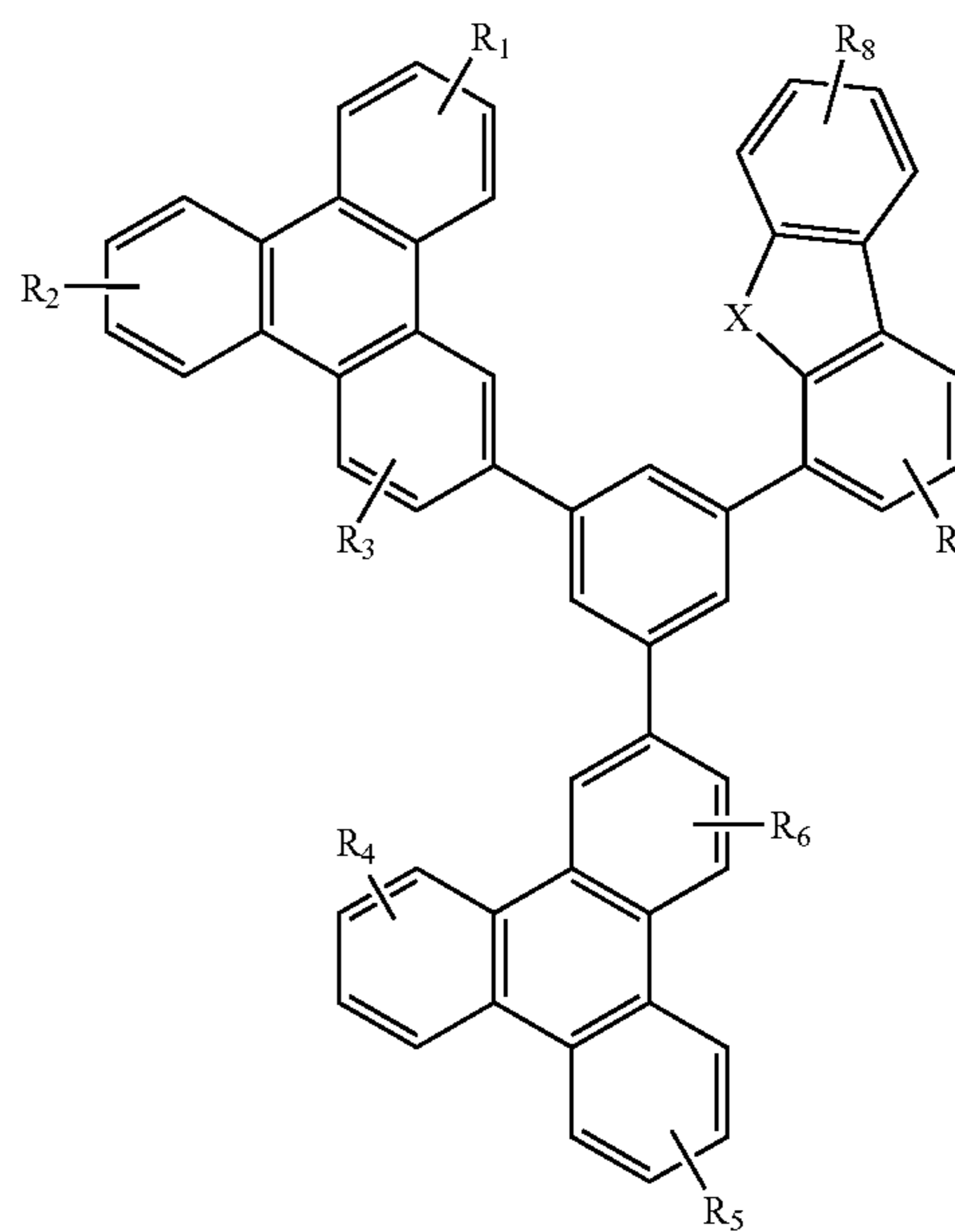
Compound 38
