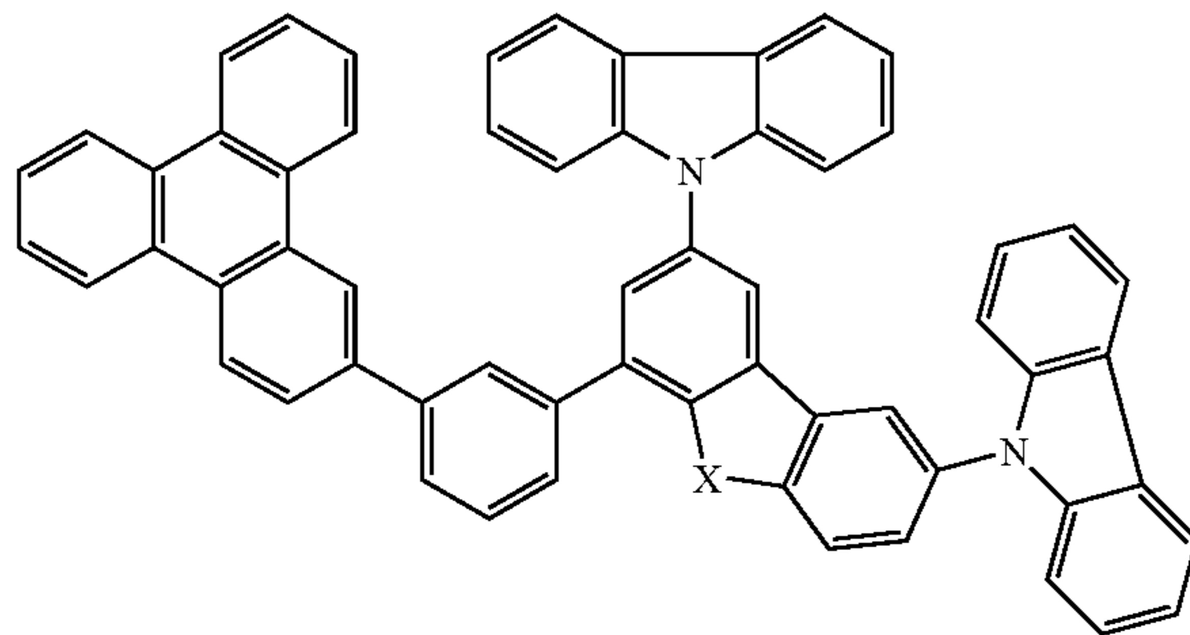
Compound 27
