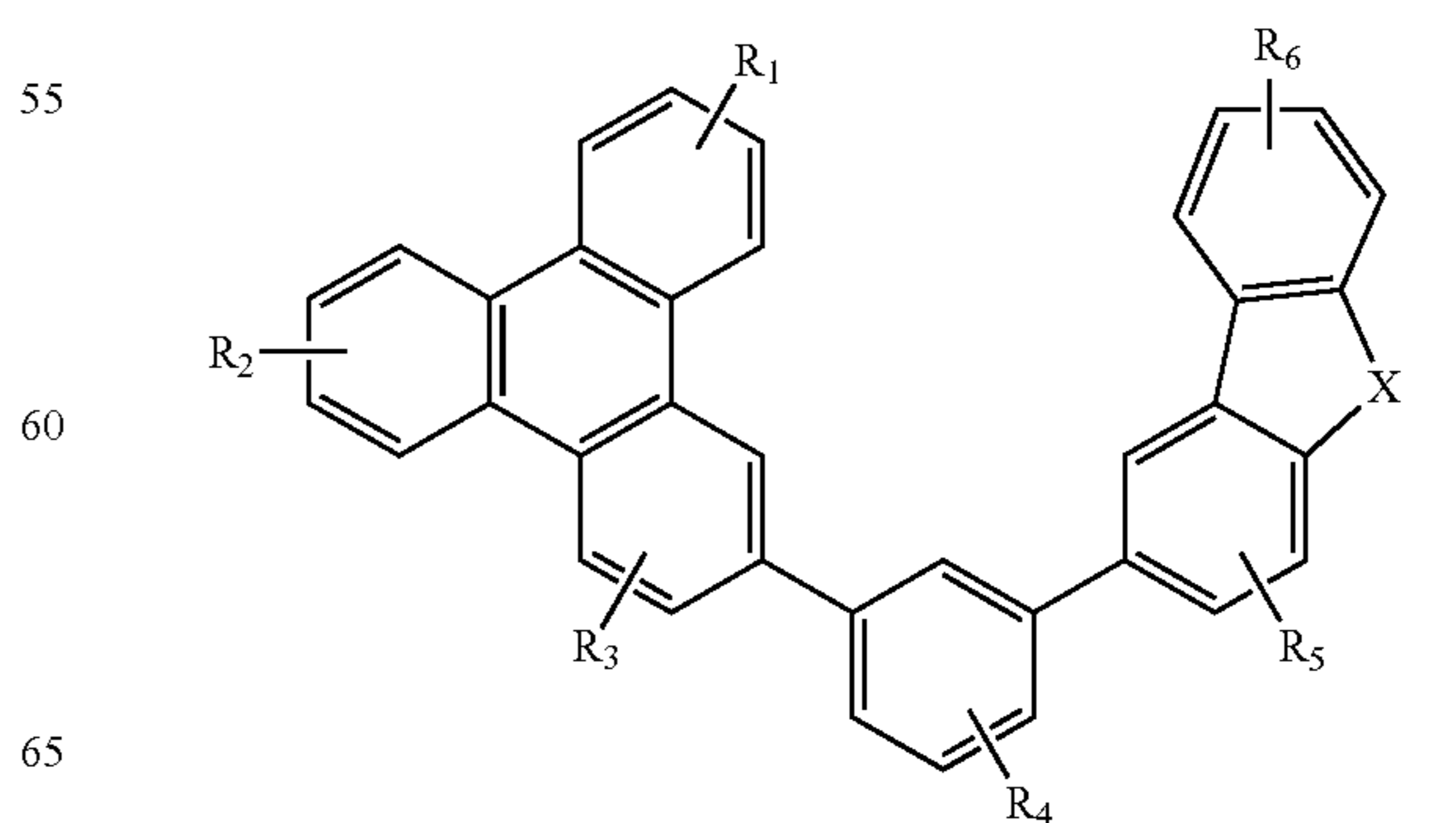
Compound 20 G
