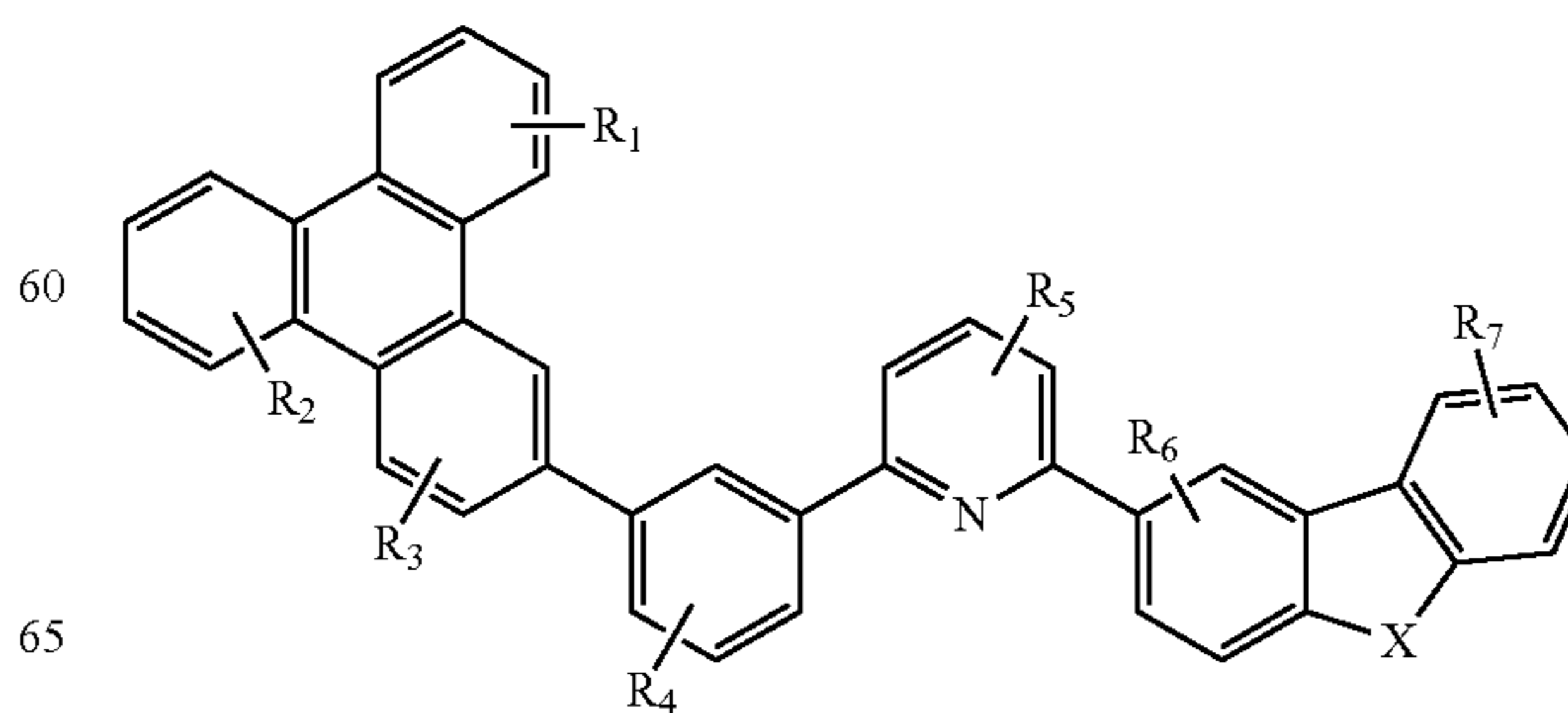
Compound 44 G
