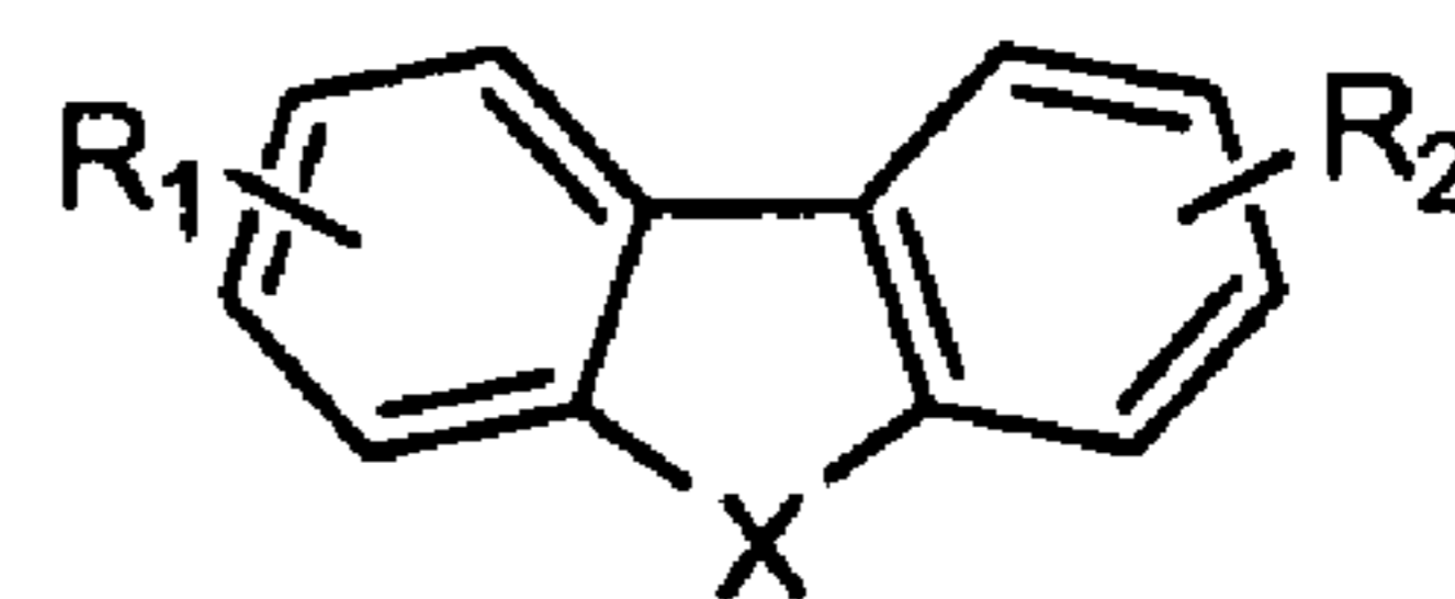
Formula (VI)
