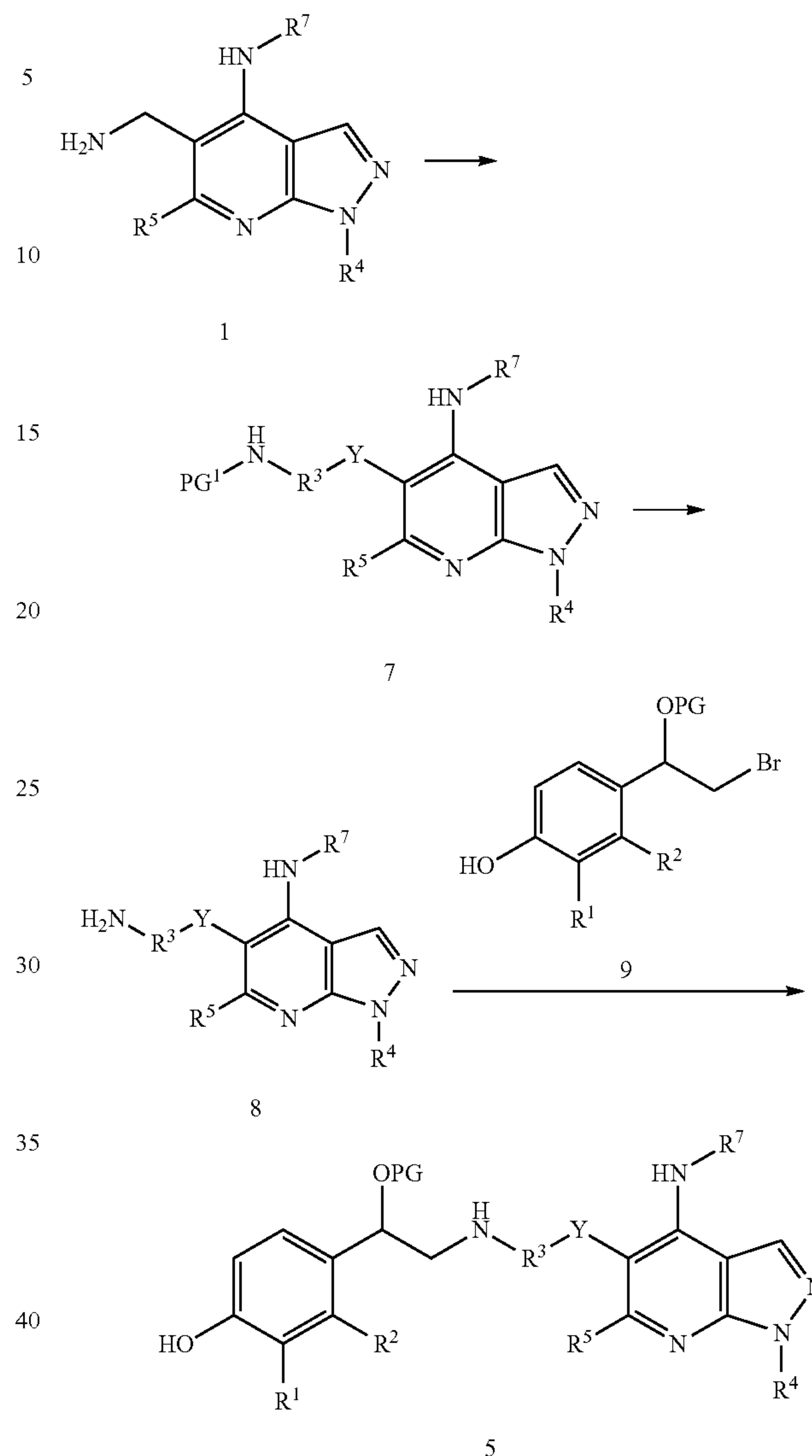
Scheme 3
