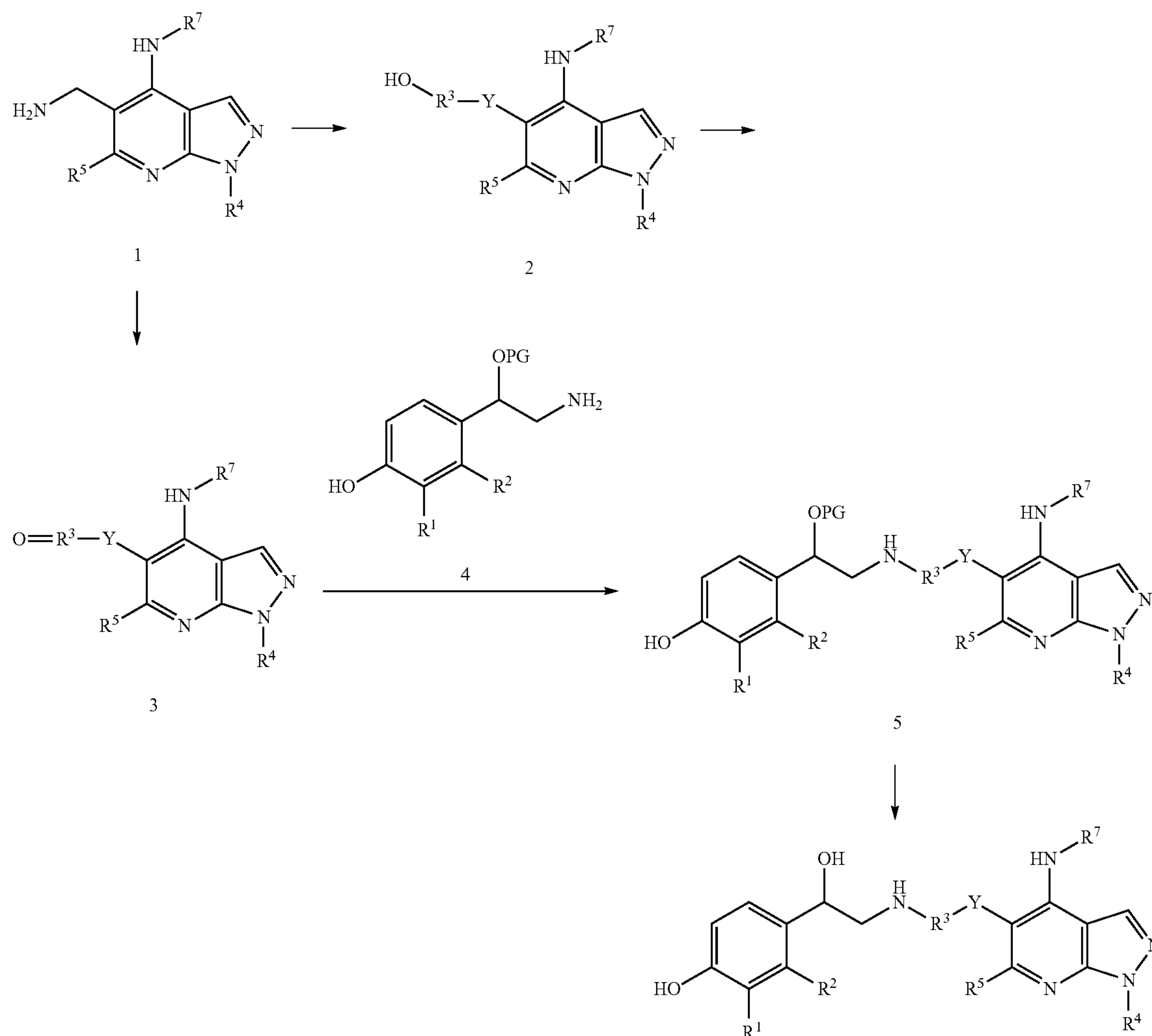
Scheme 1
