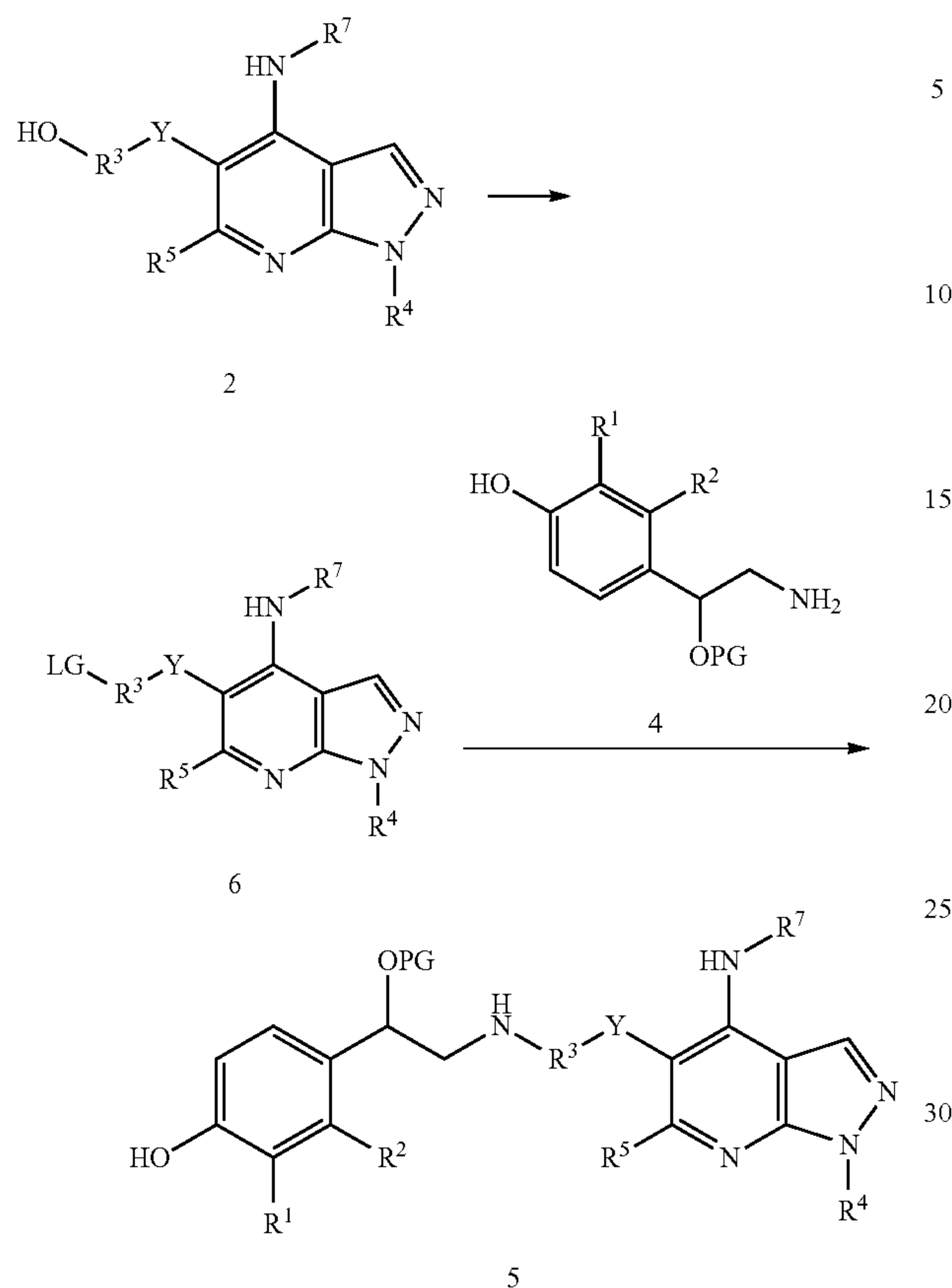
Scheme 2
