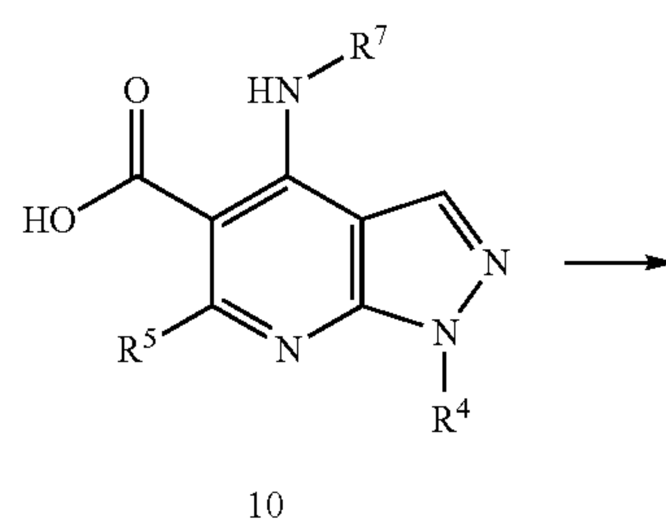
Scheme 5
