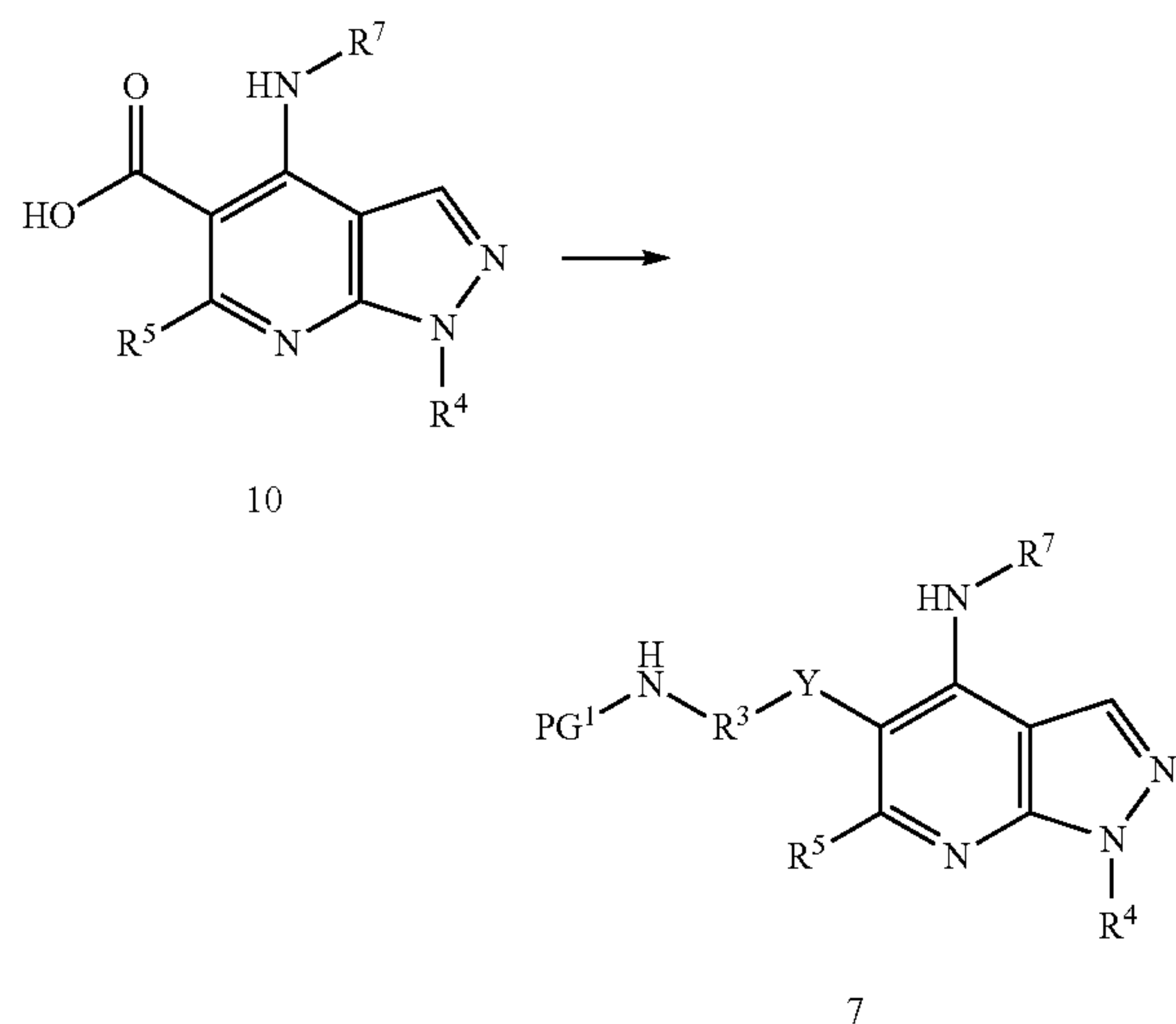
Scheme 4
