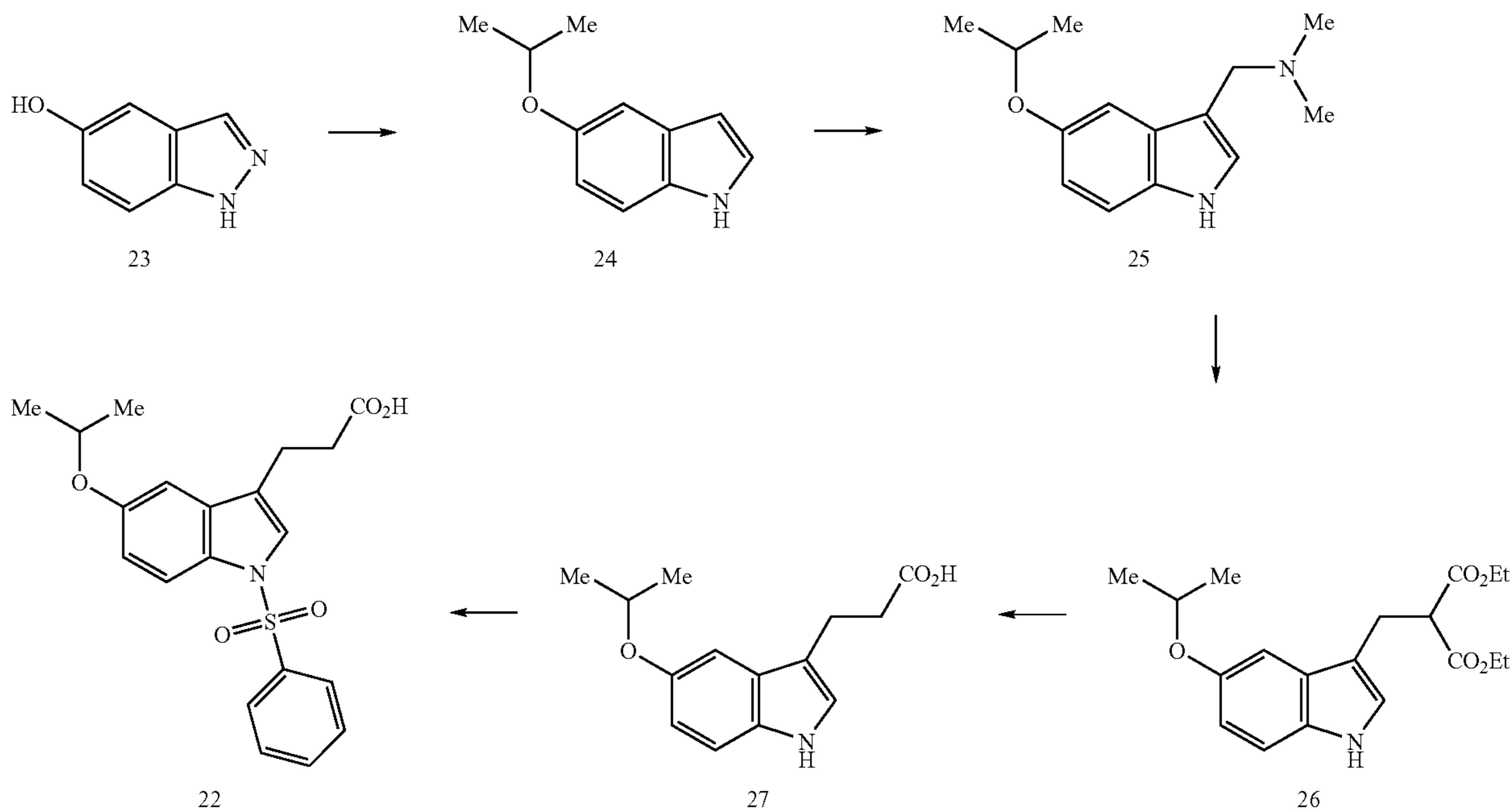
Scheme 10
