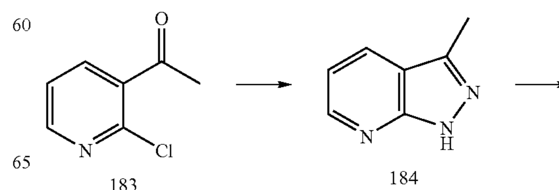
Scheme 30
