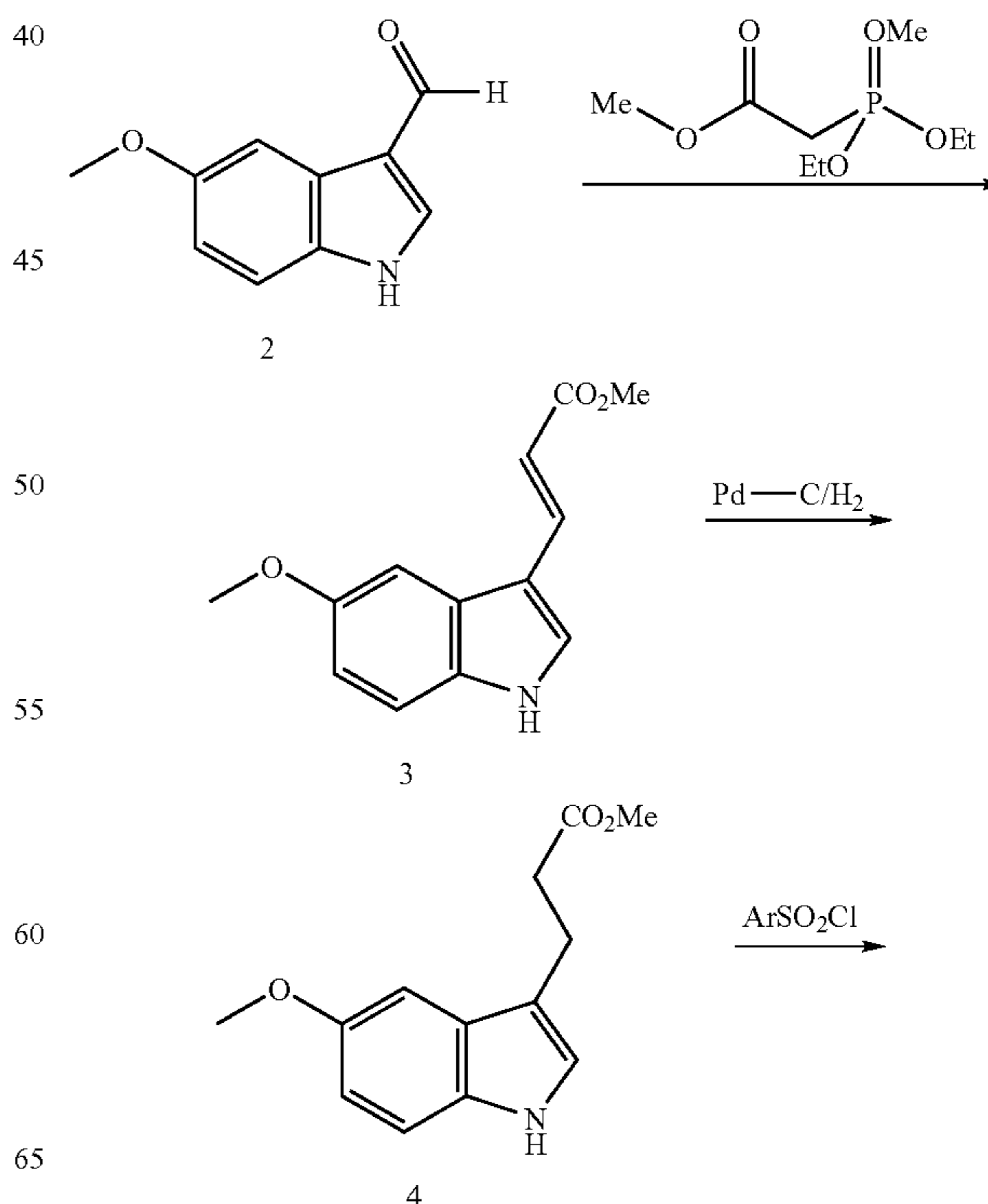
Scheme 7
