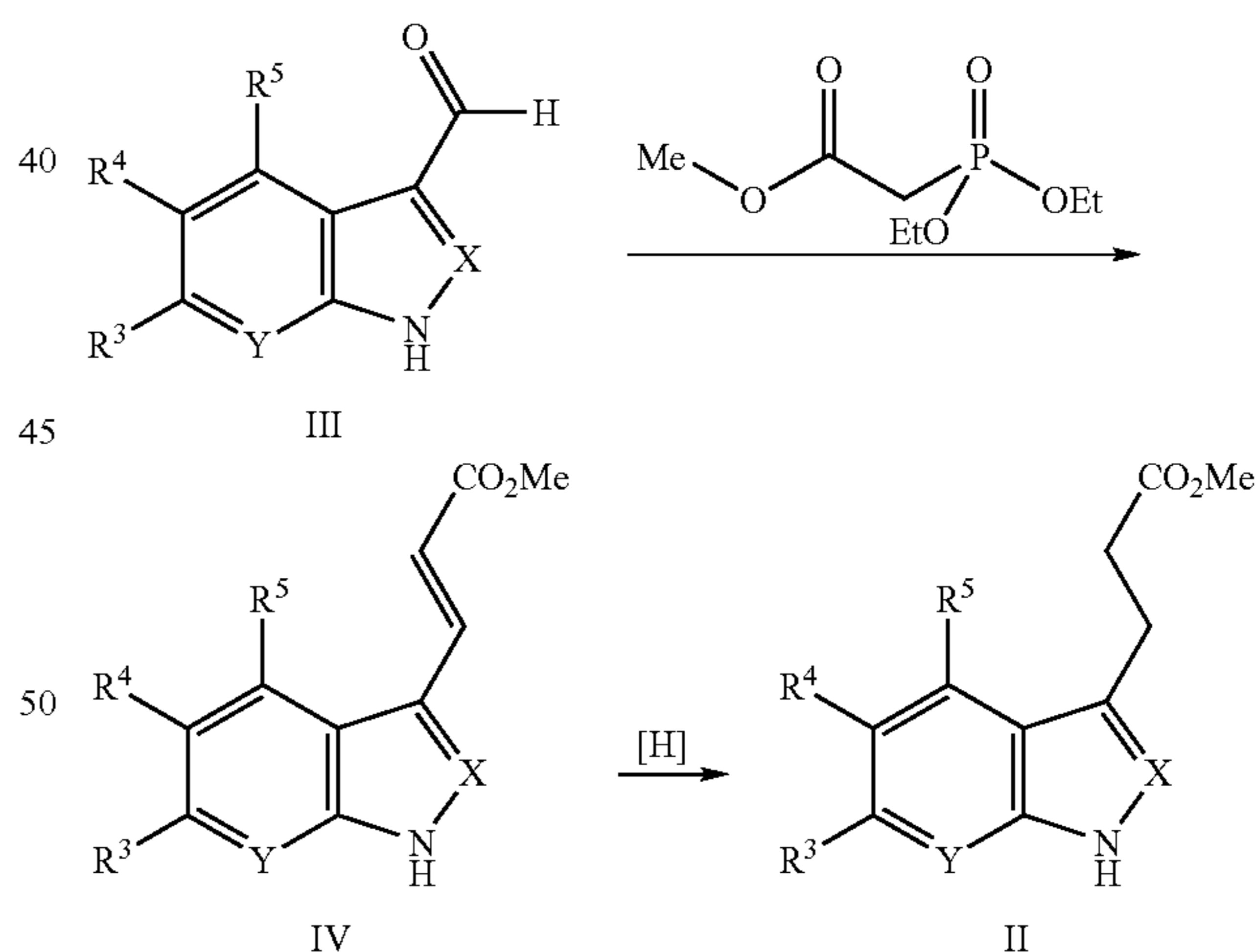
Scheme 1a:
