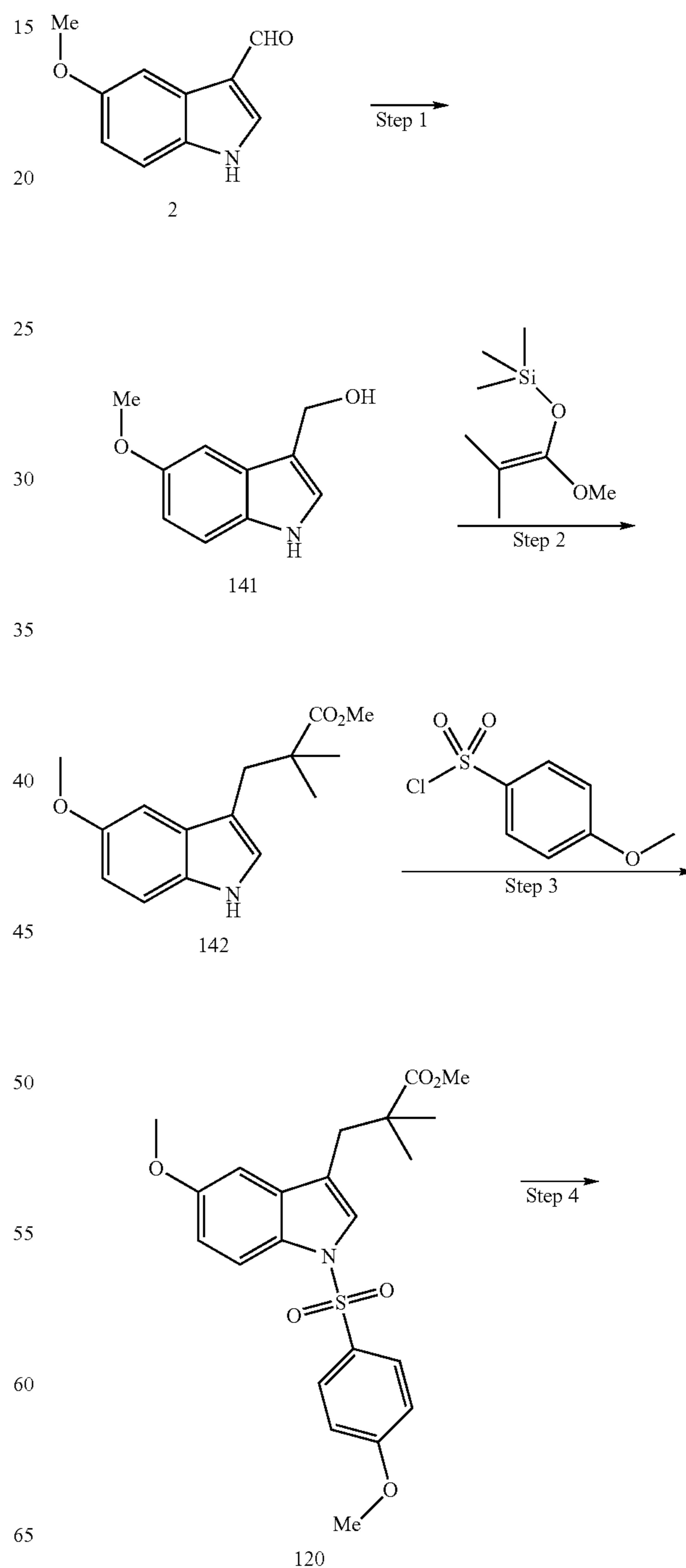
Scheme 13
