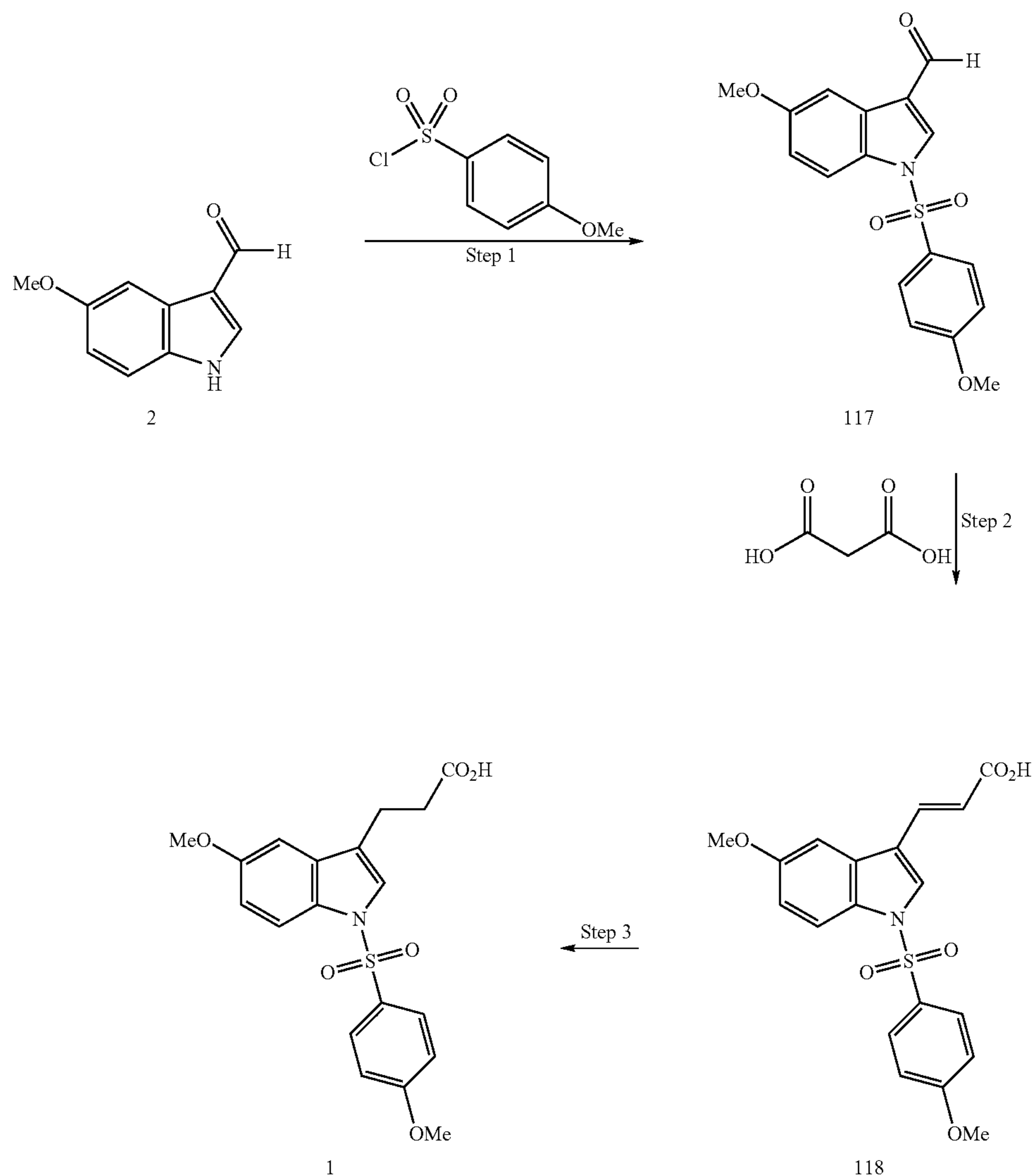
Scheme 12
