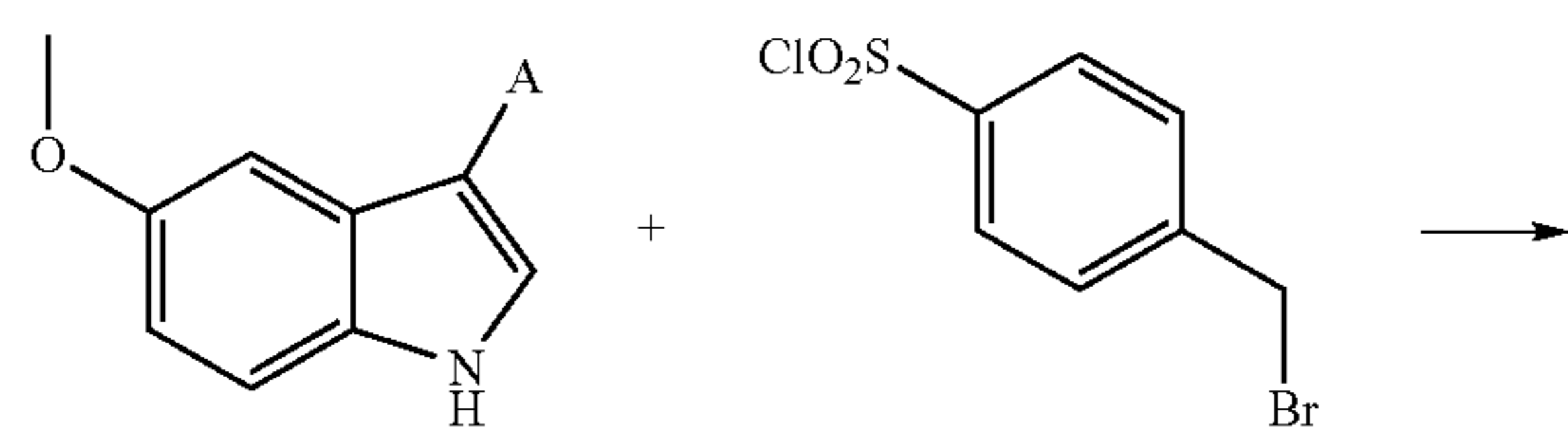
Scheme 24
