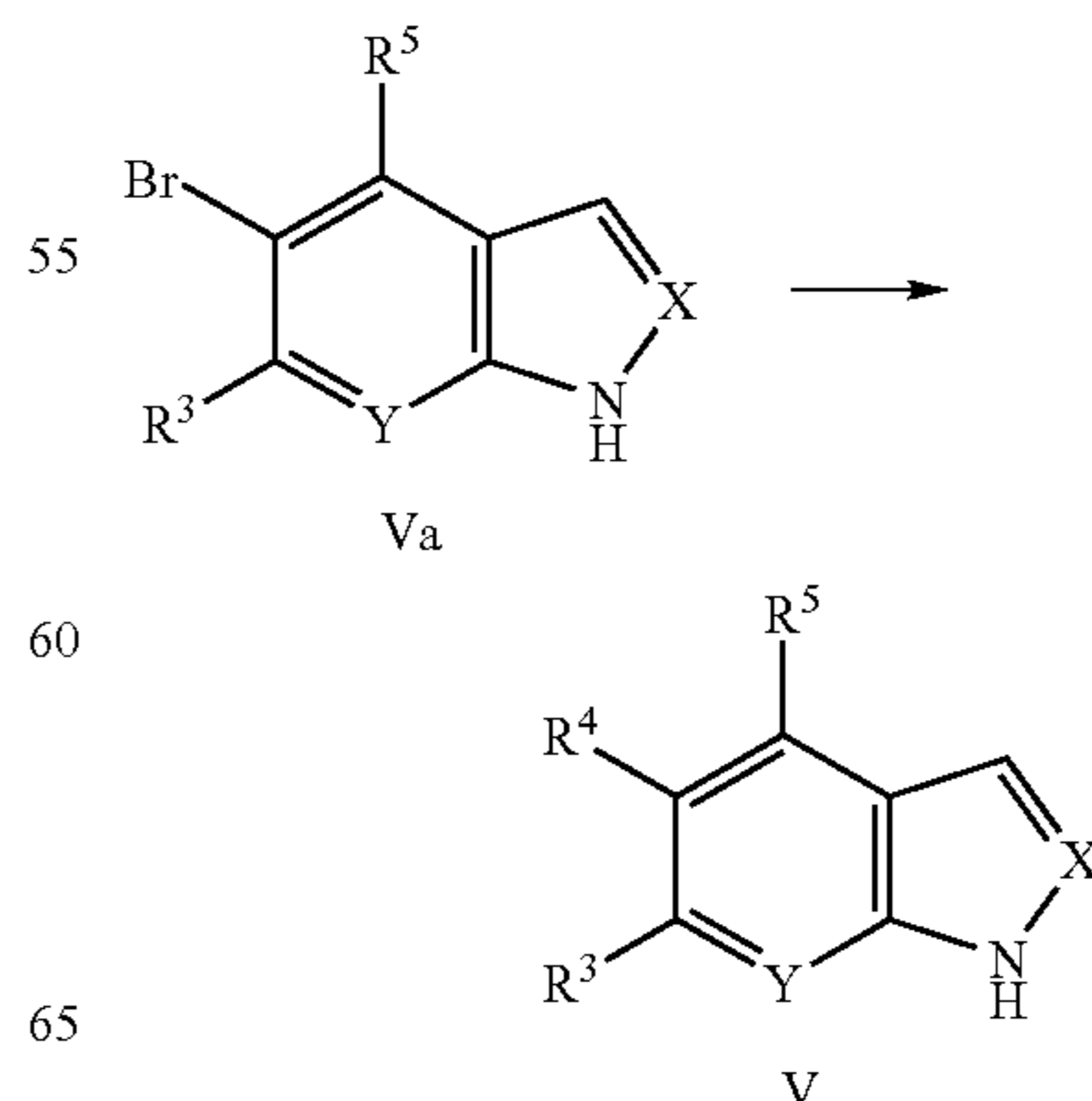
Scheme 5b
