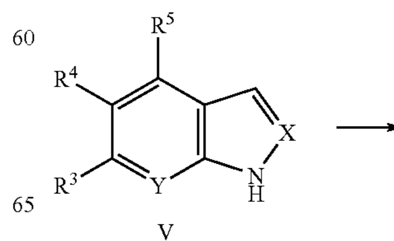
Scheme 6
