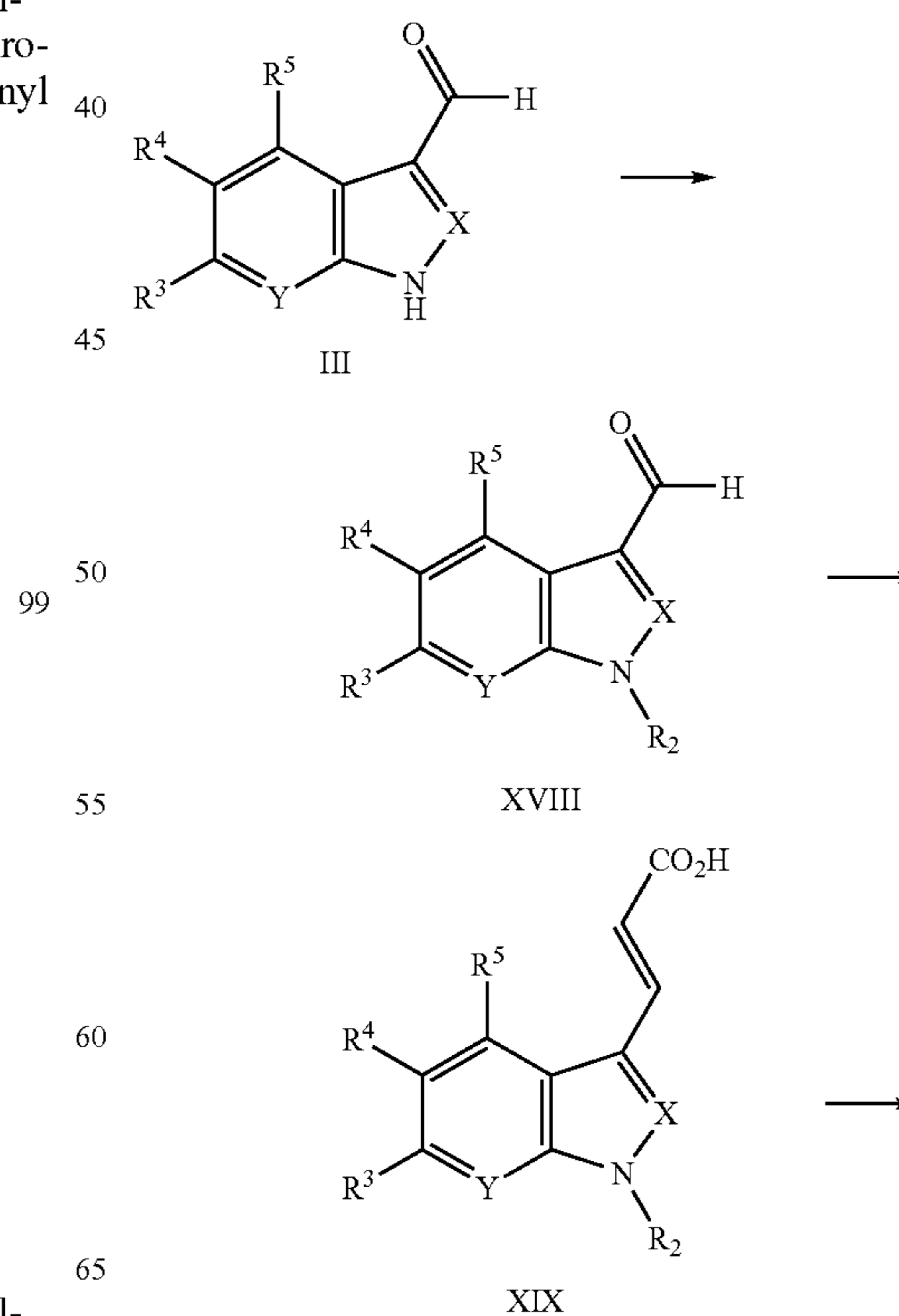
Scheme 11: Alternative synthesis methodology for Compounds of Formula Ib
