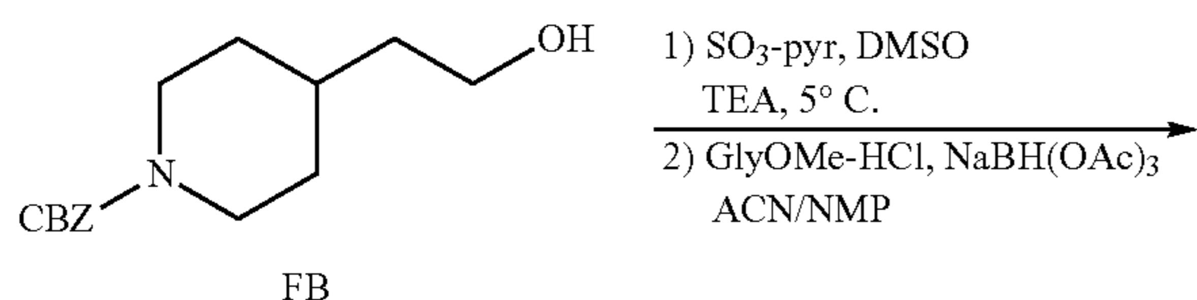
Scheme 91
