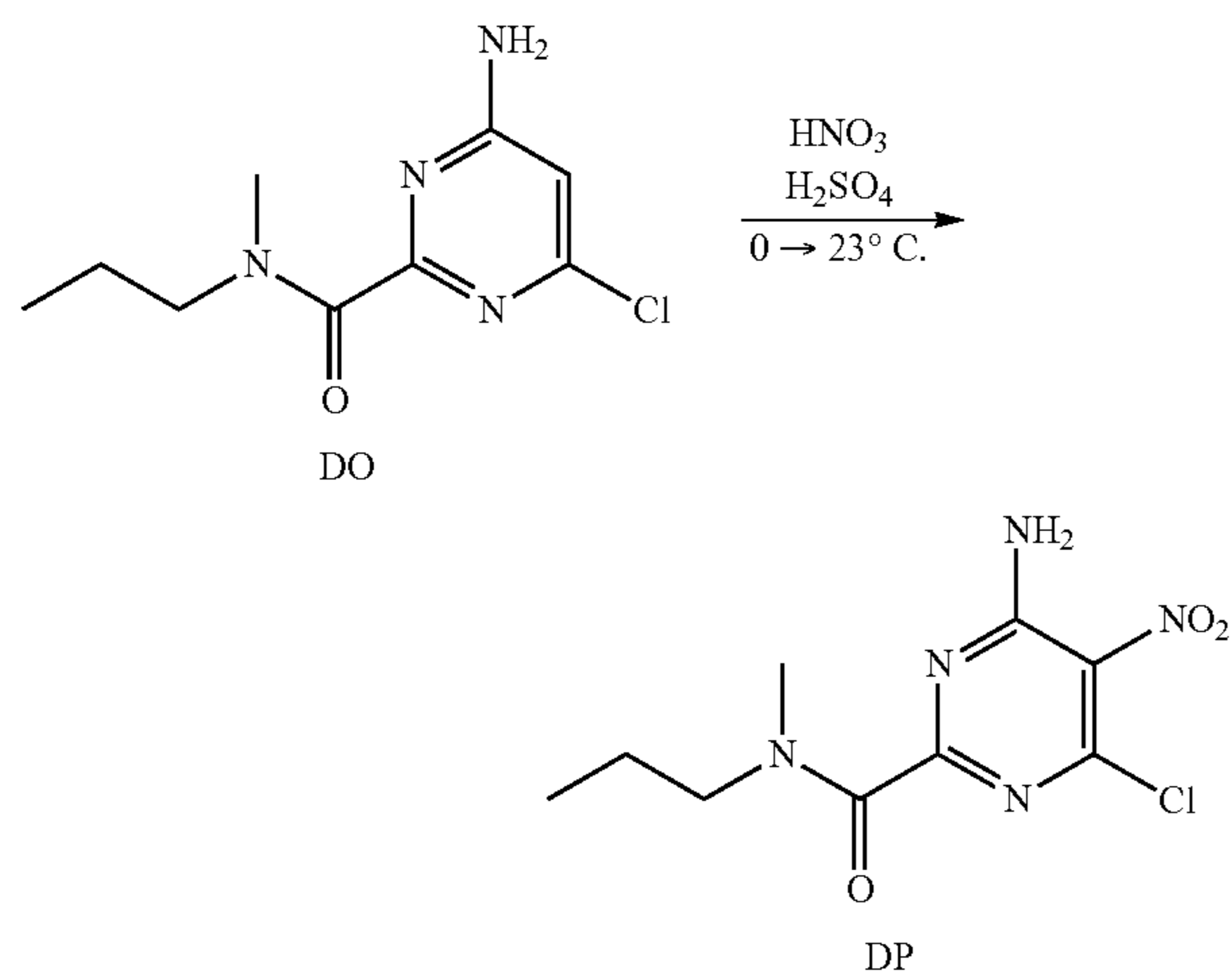
Scheme 82
