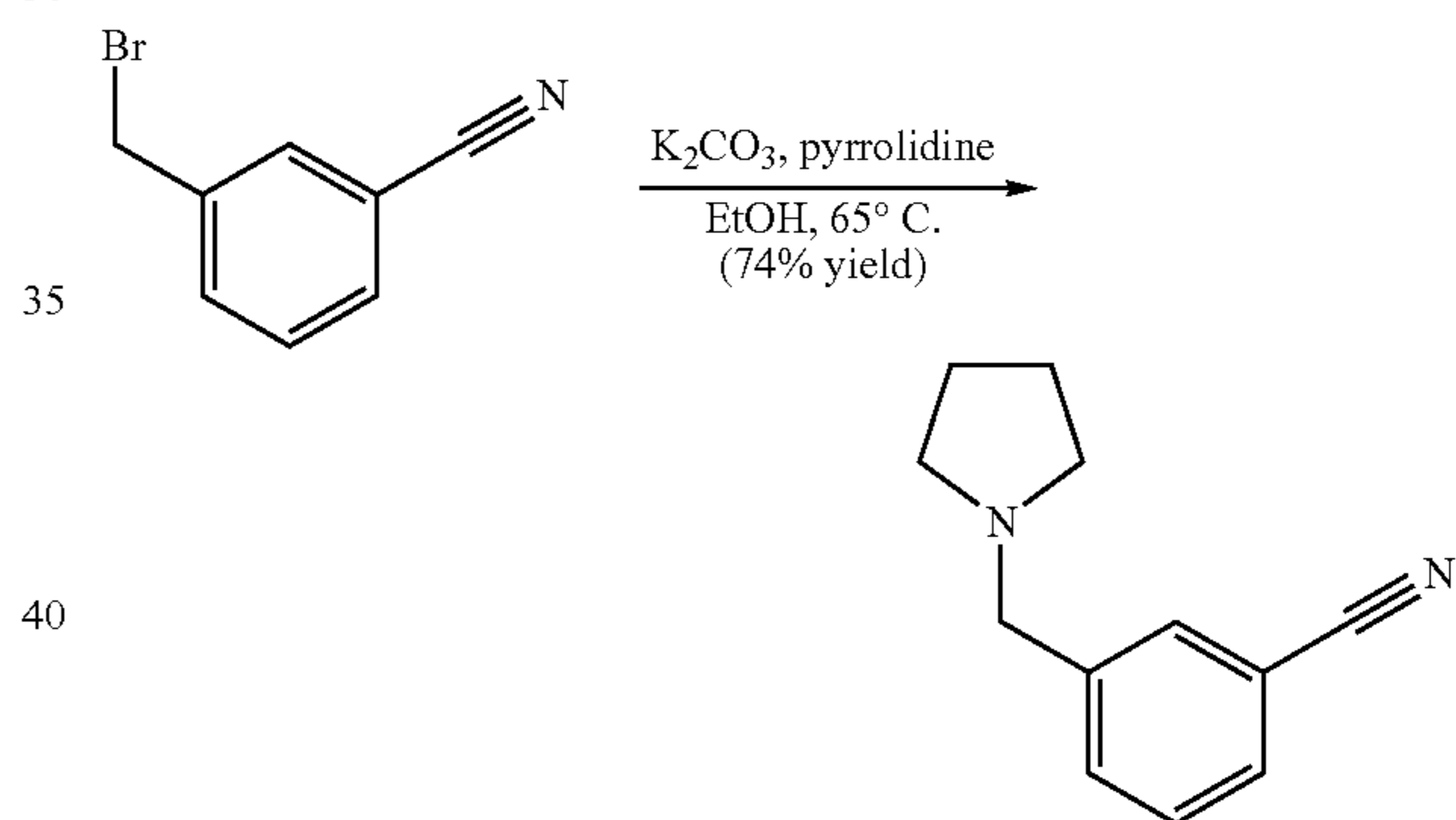
Scheme 3
