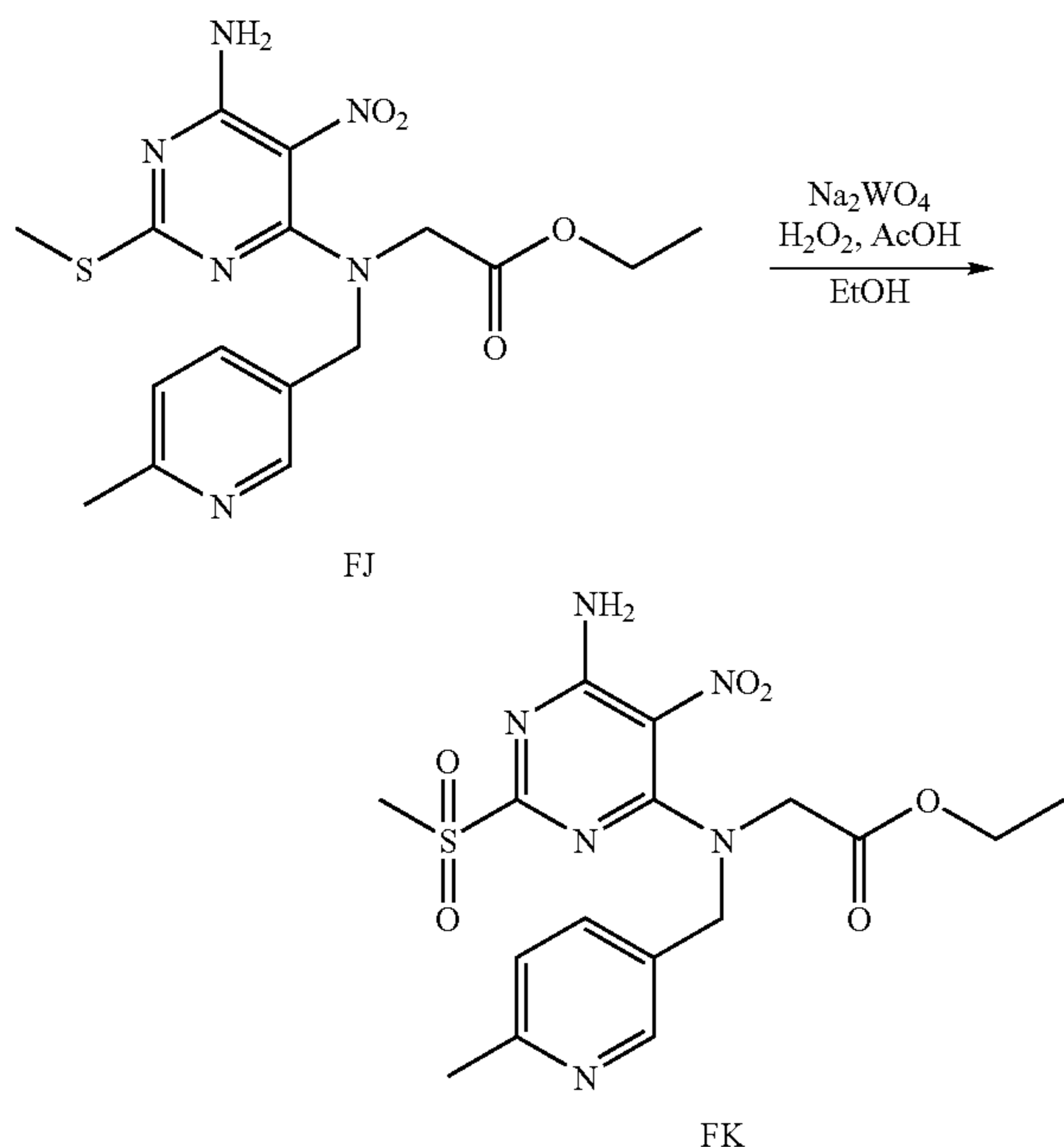
Scheme 99:
