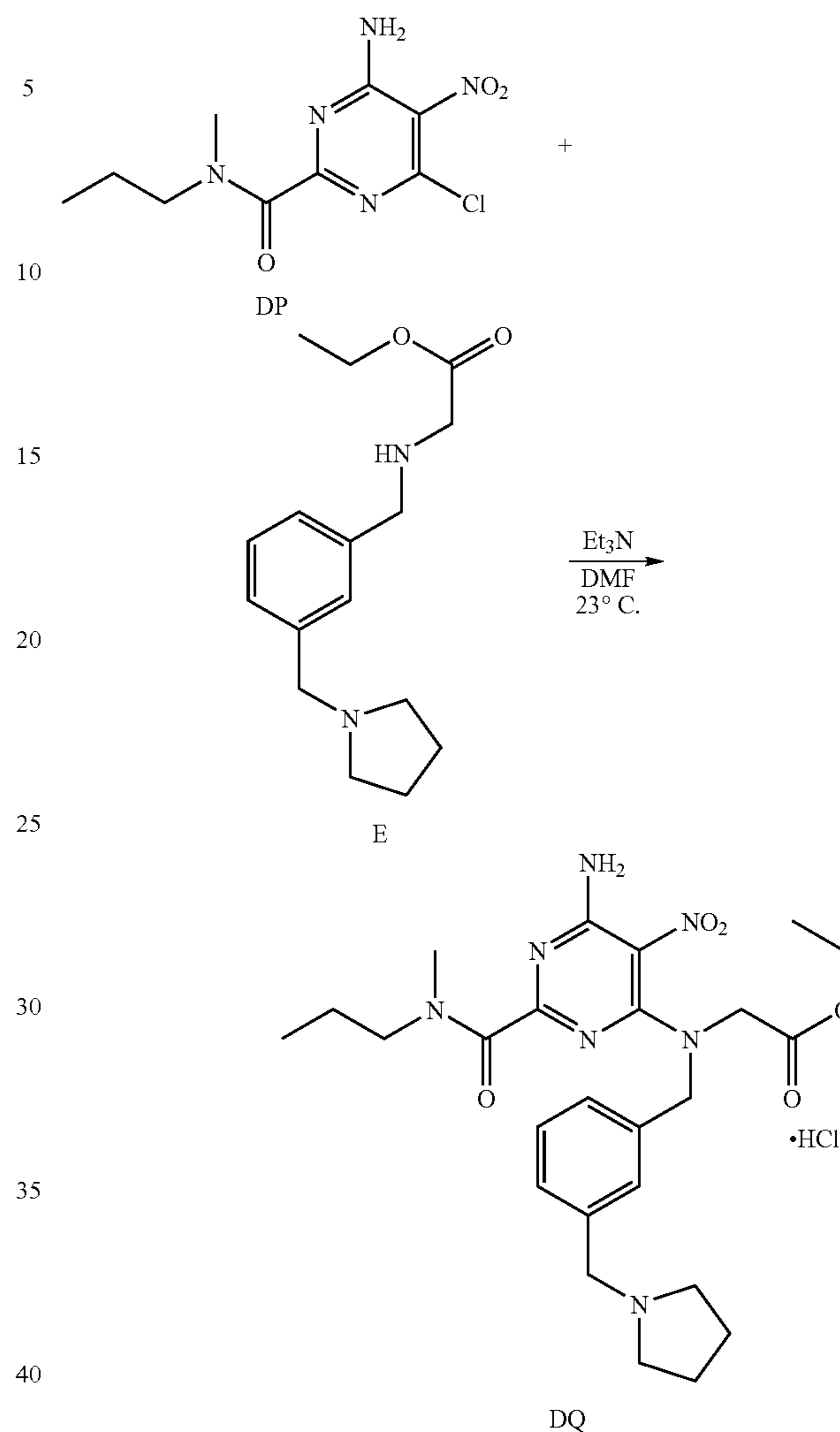
Scheme 83:
