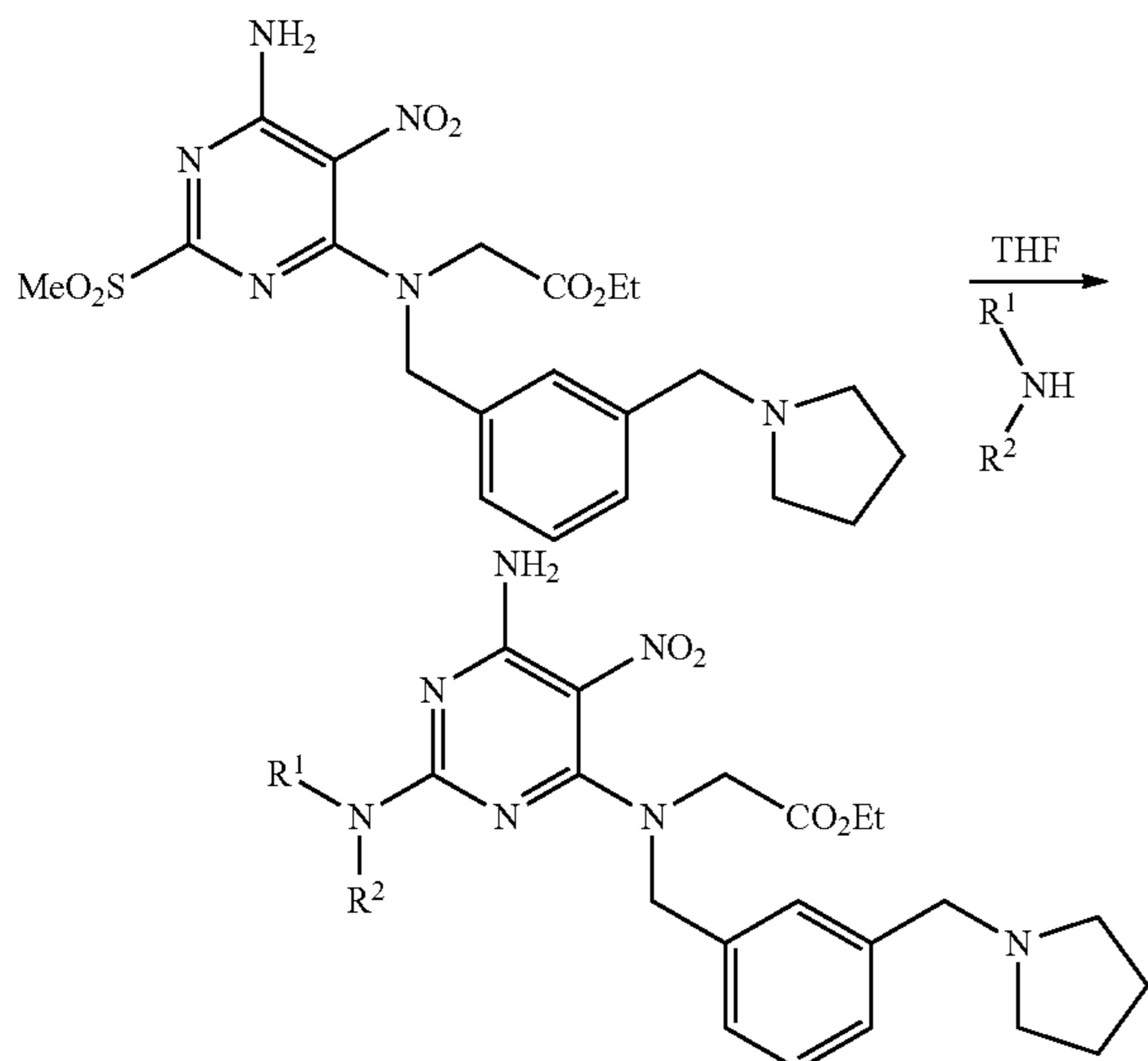
Scheme 16
