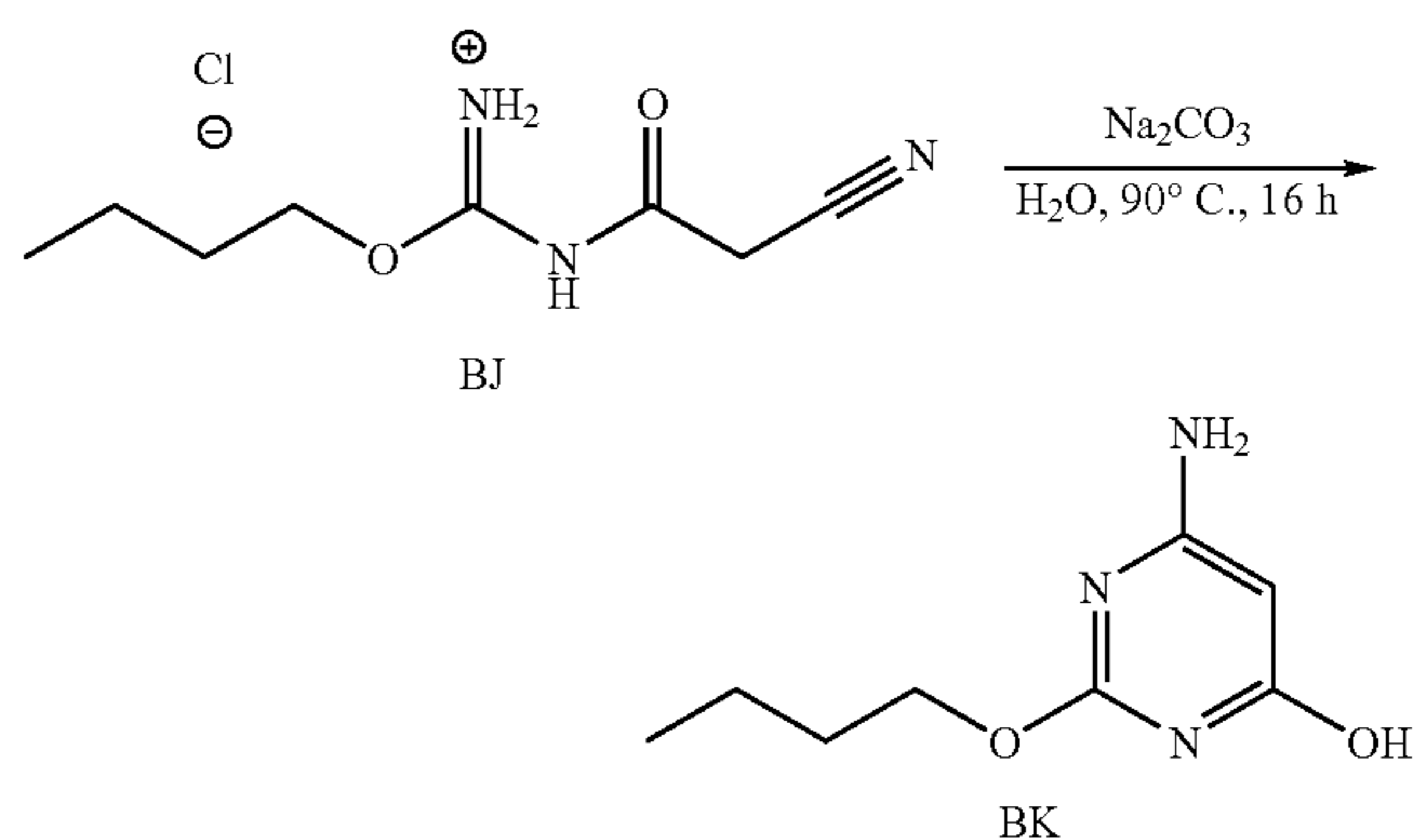
Scheme 29
