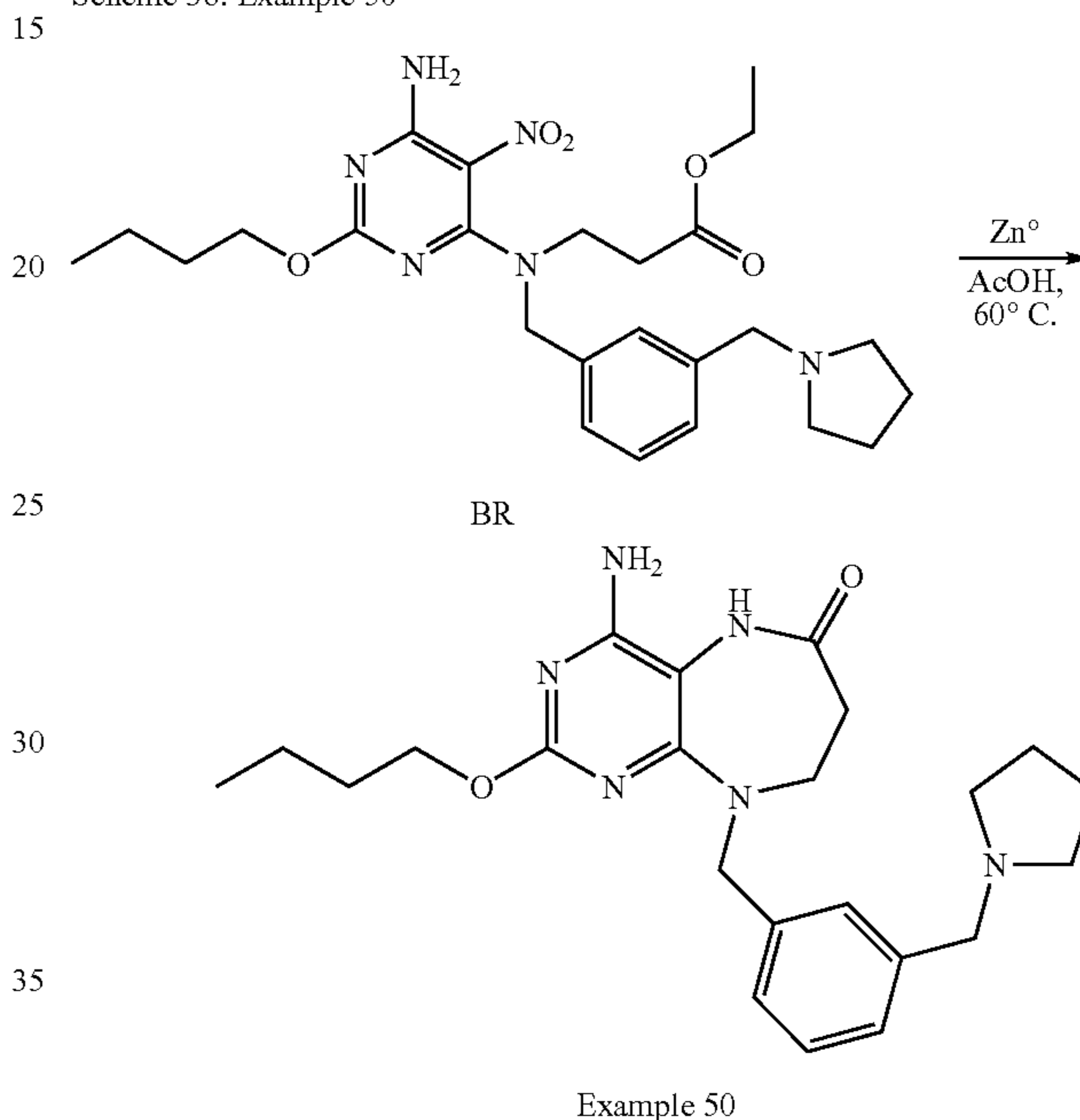
Scheme 38: Example 50
