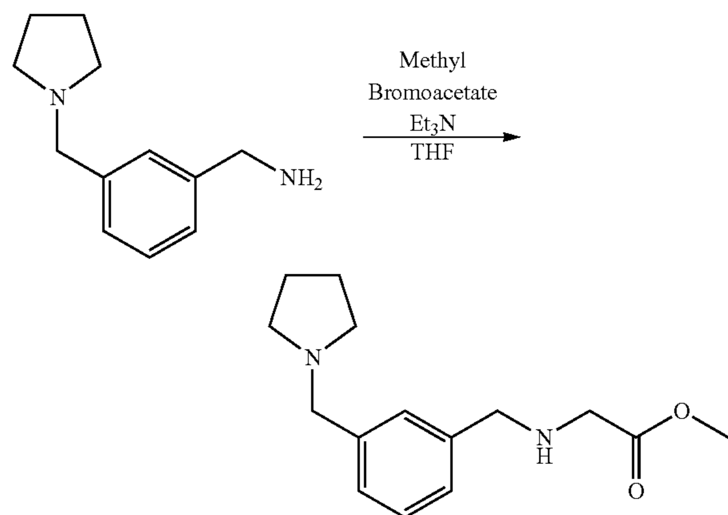
Scheme 20
