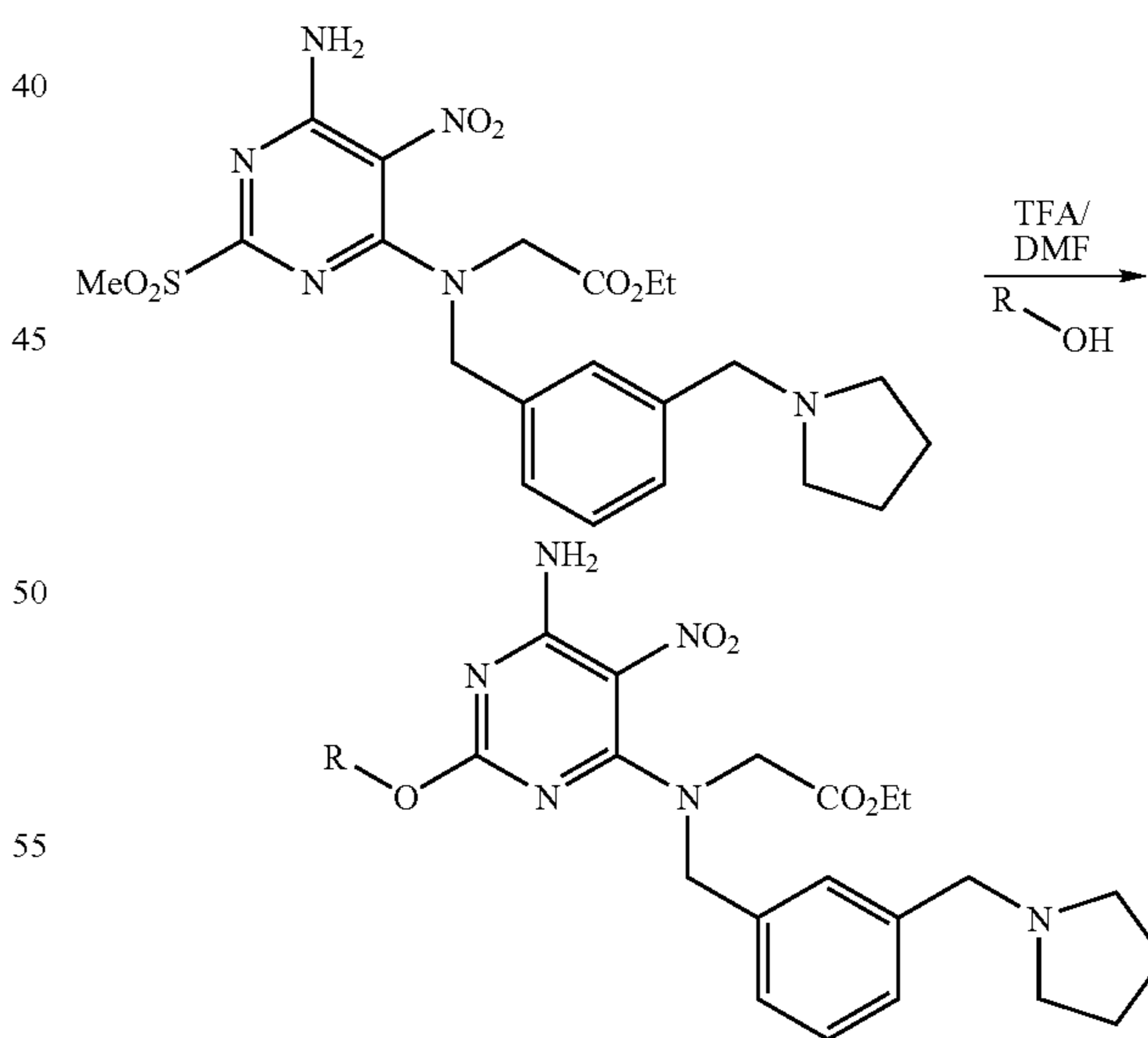
Scheme 14
