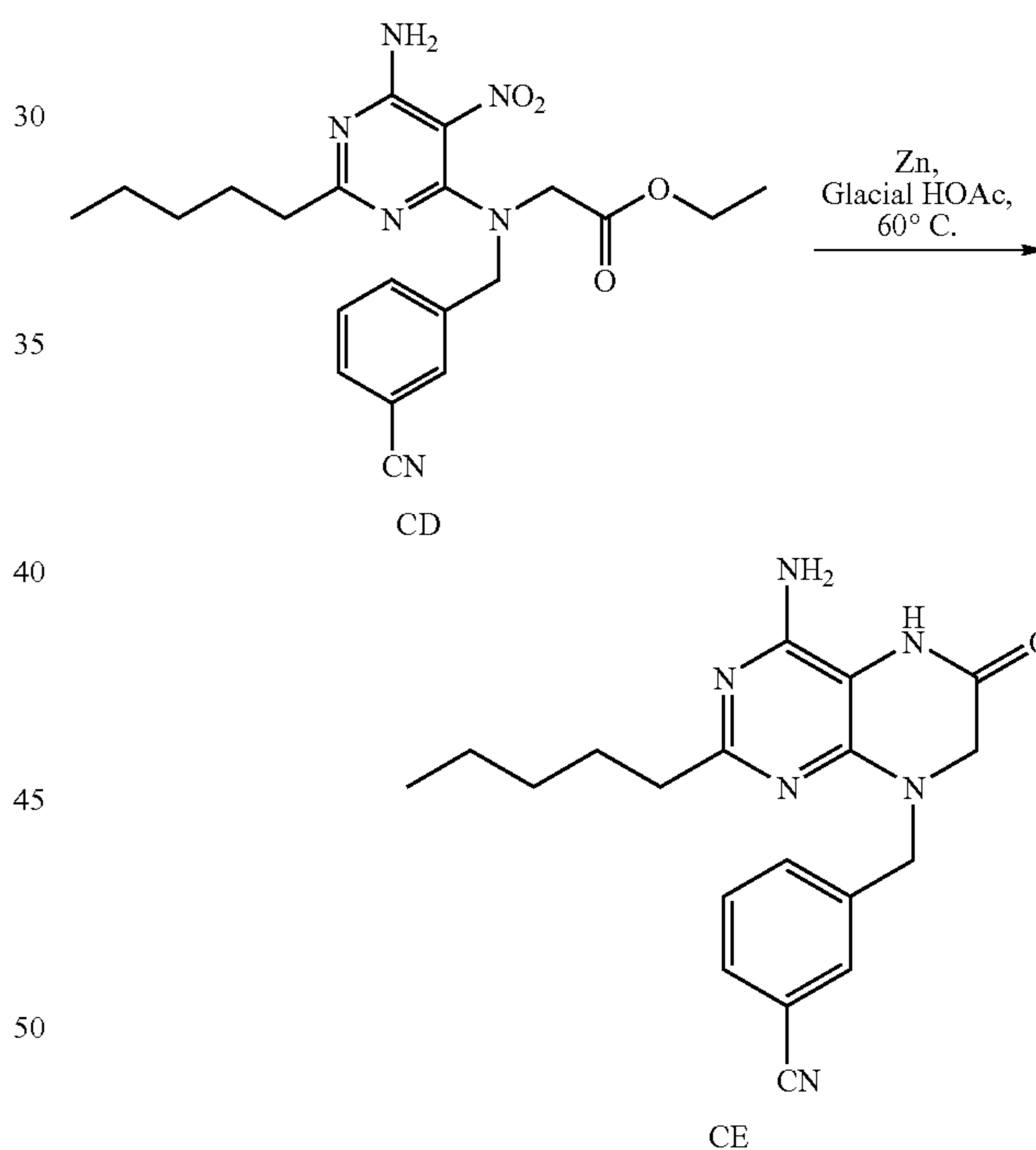
Scheme 52
