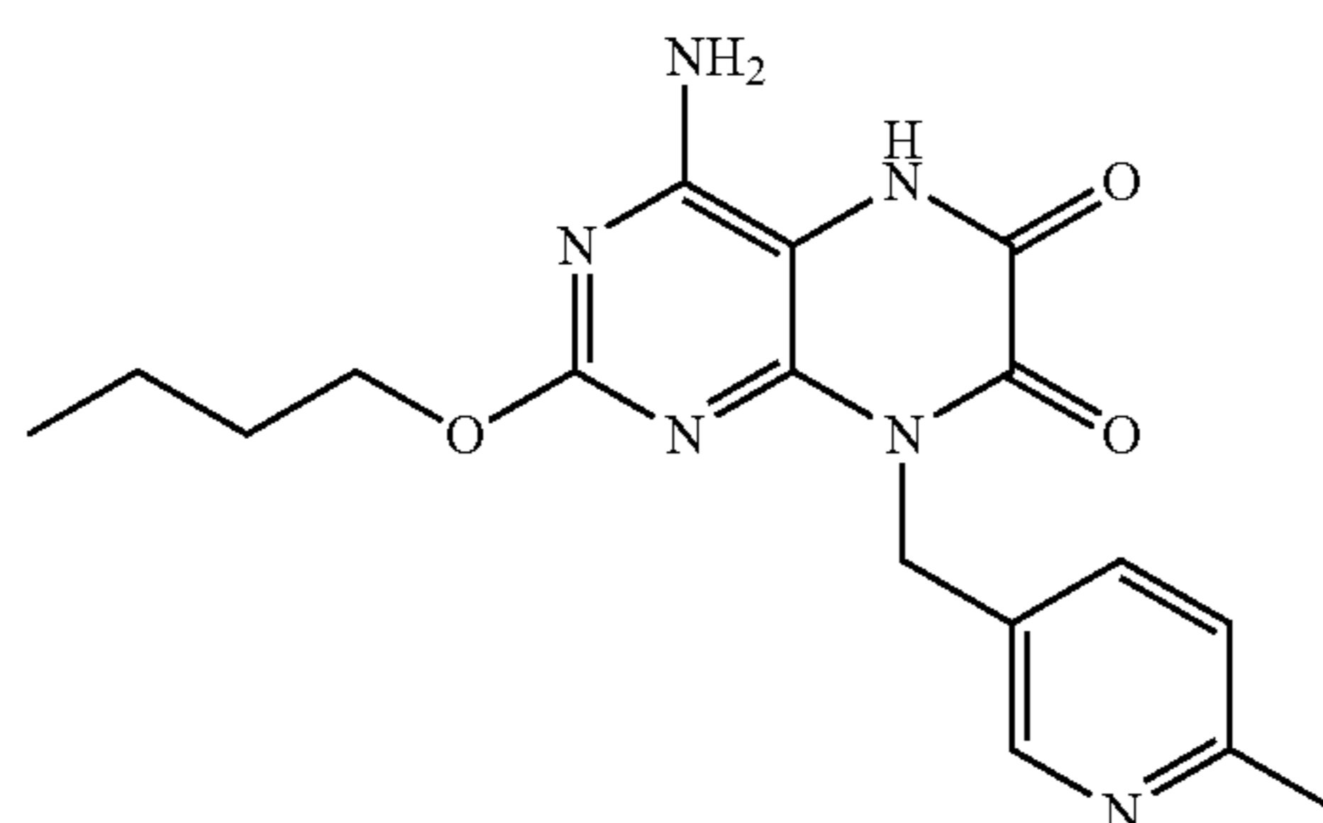
Example 112
