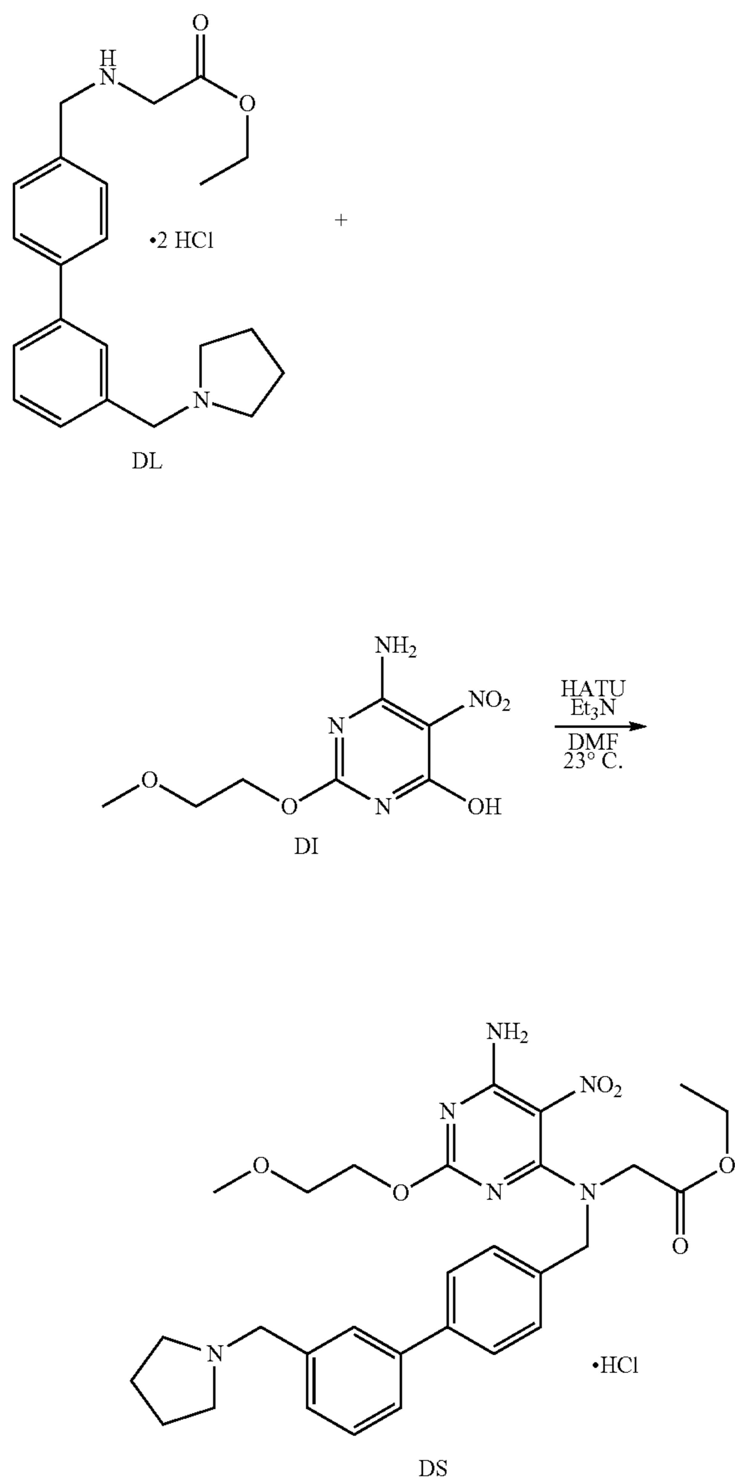
Scheme 86
