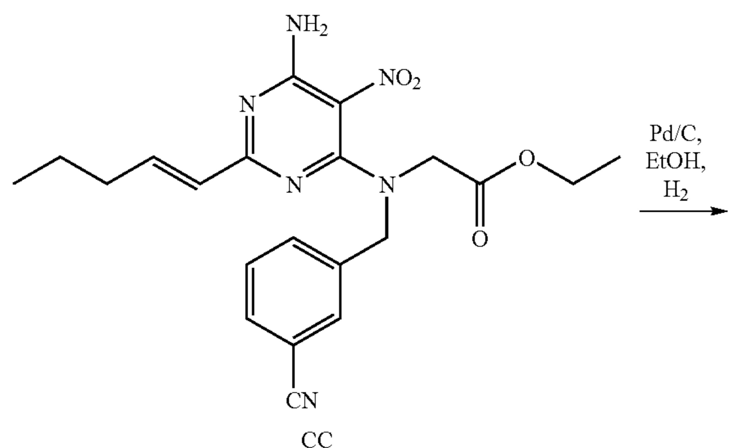
Scheme 51
