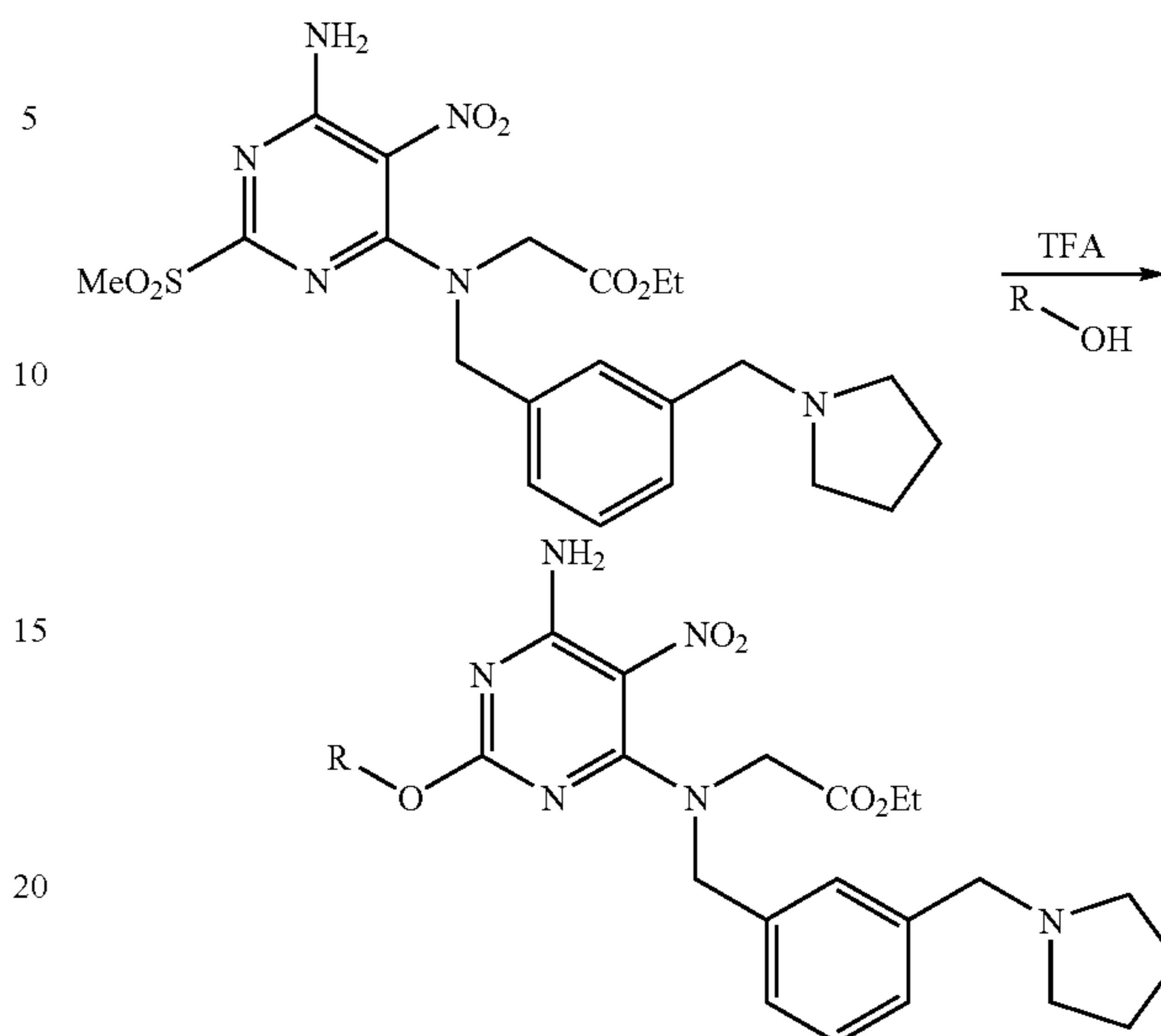
Scheme 13
