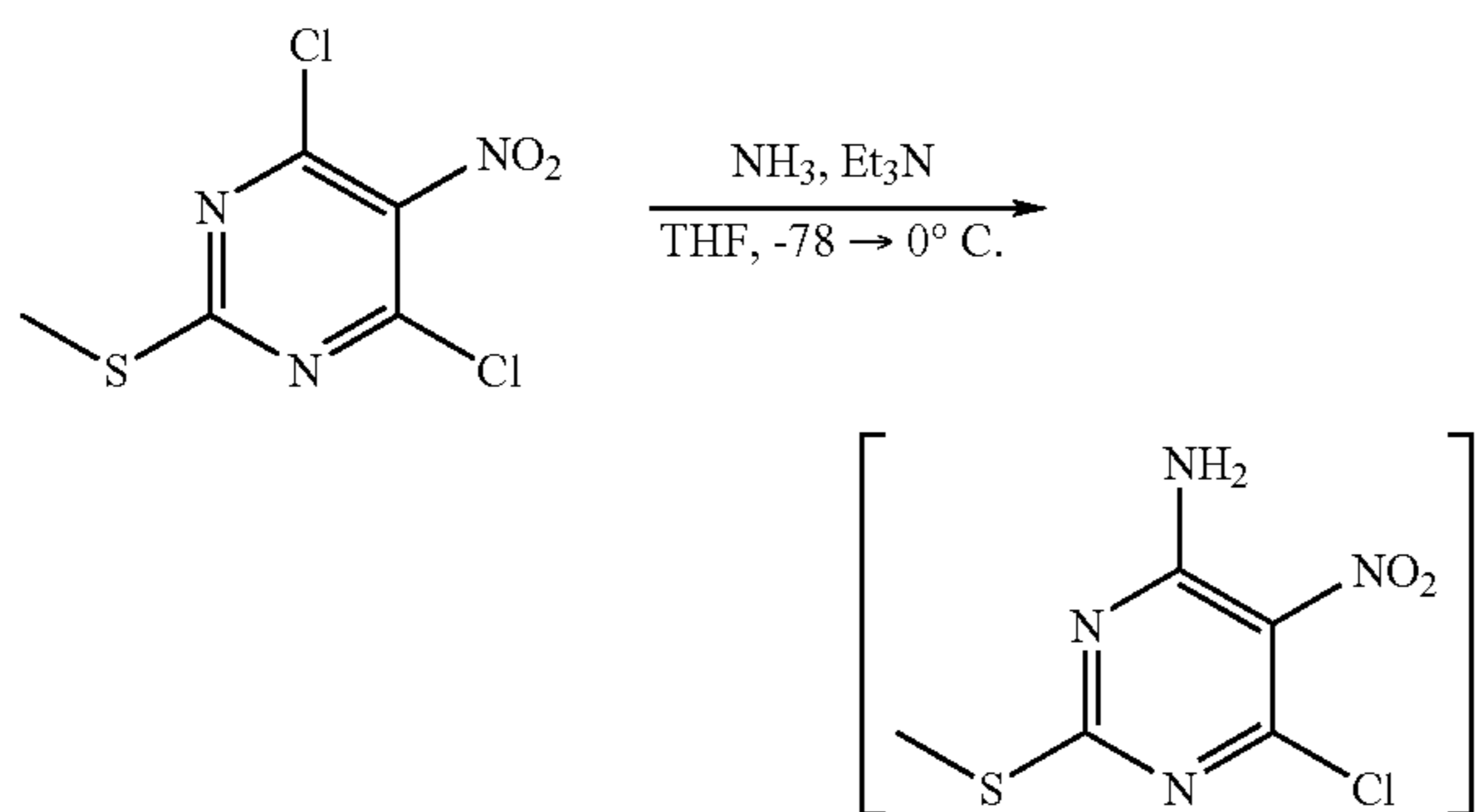
Scheme 34
