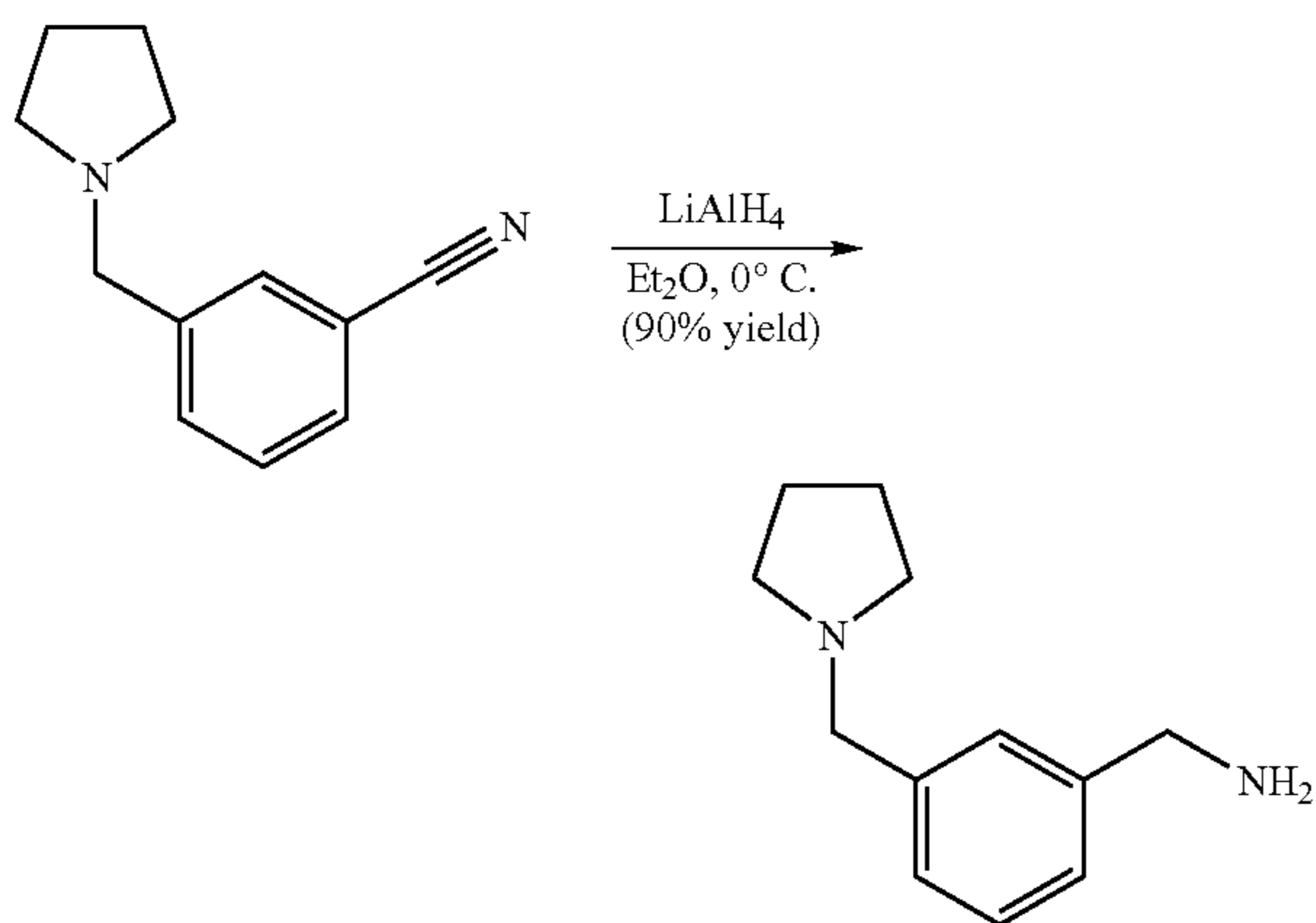
Scheme 5
