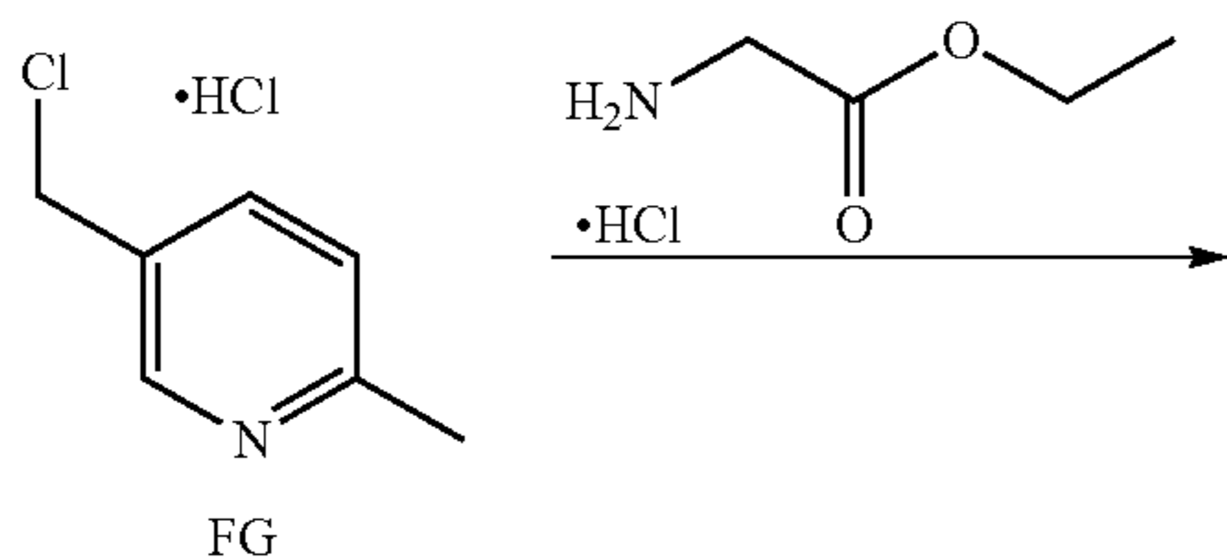
Scheme 97
