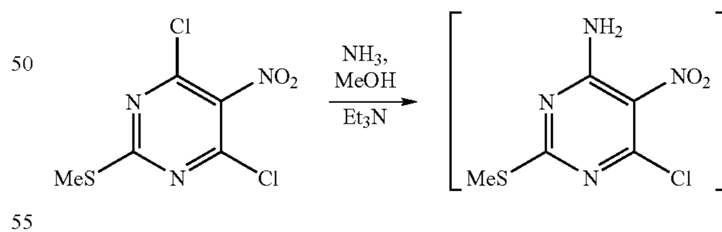
Scheme 18
