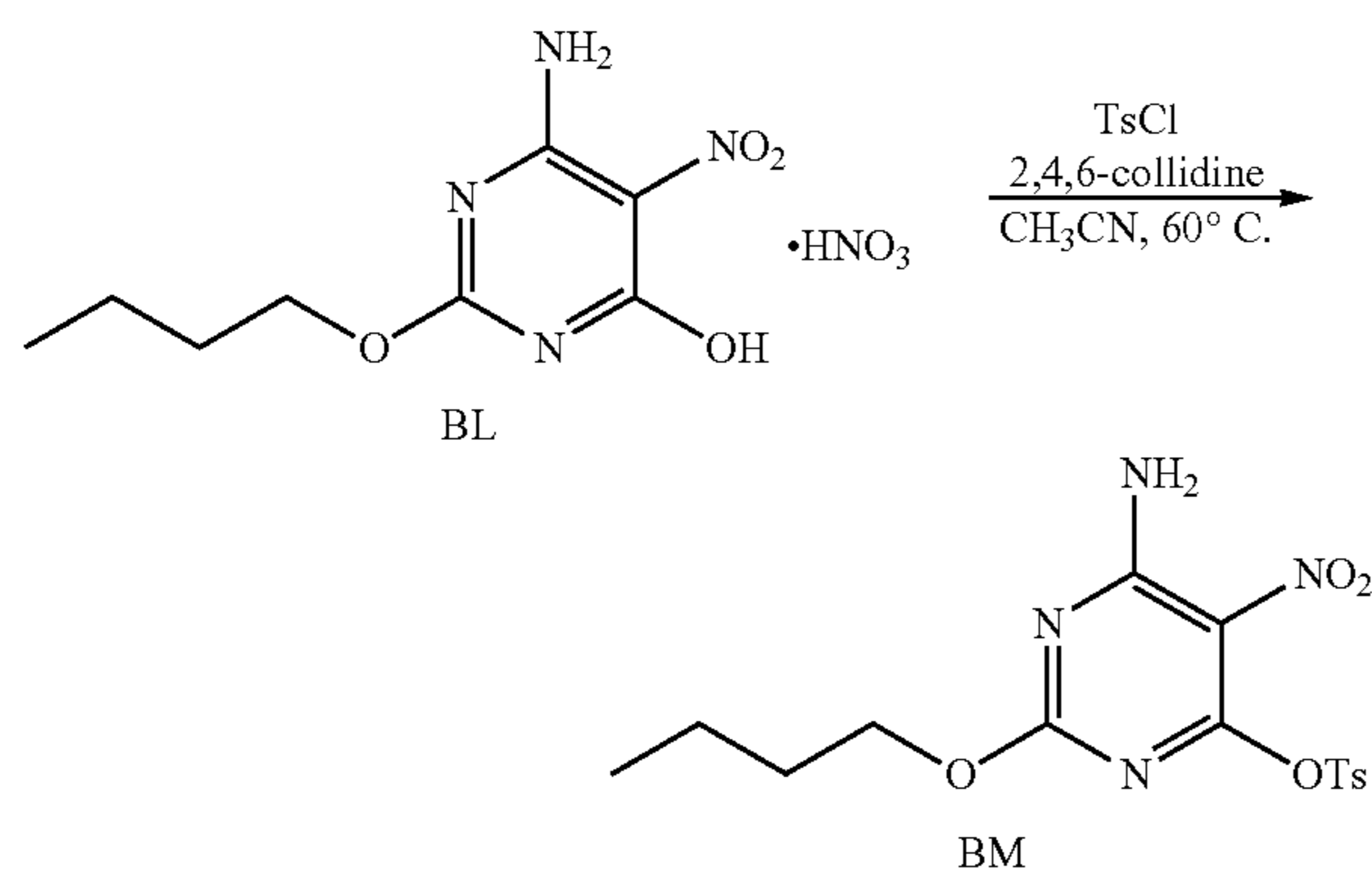
Scheme 31
