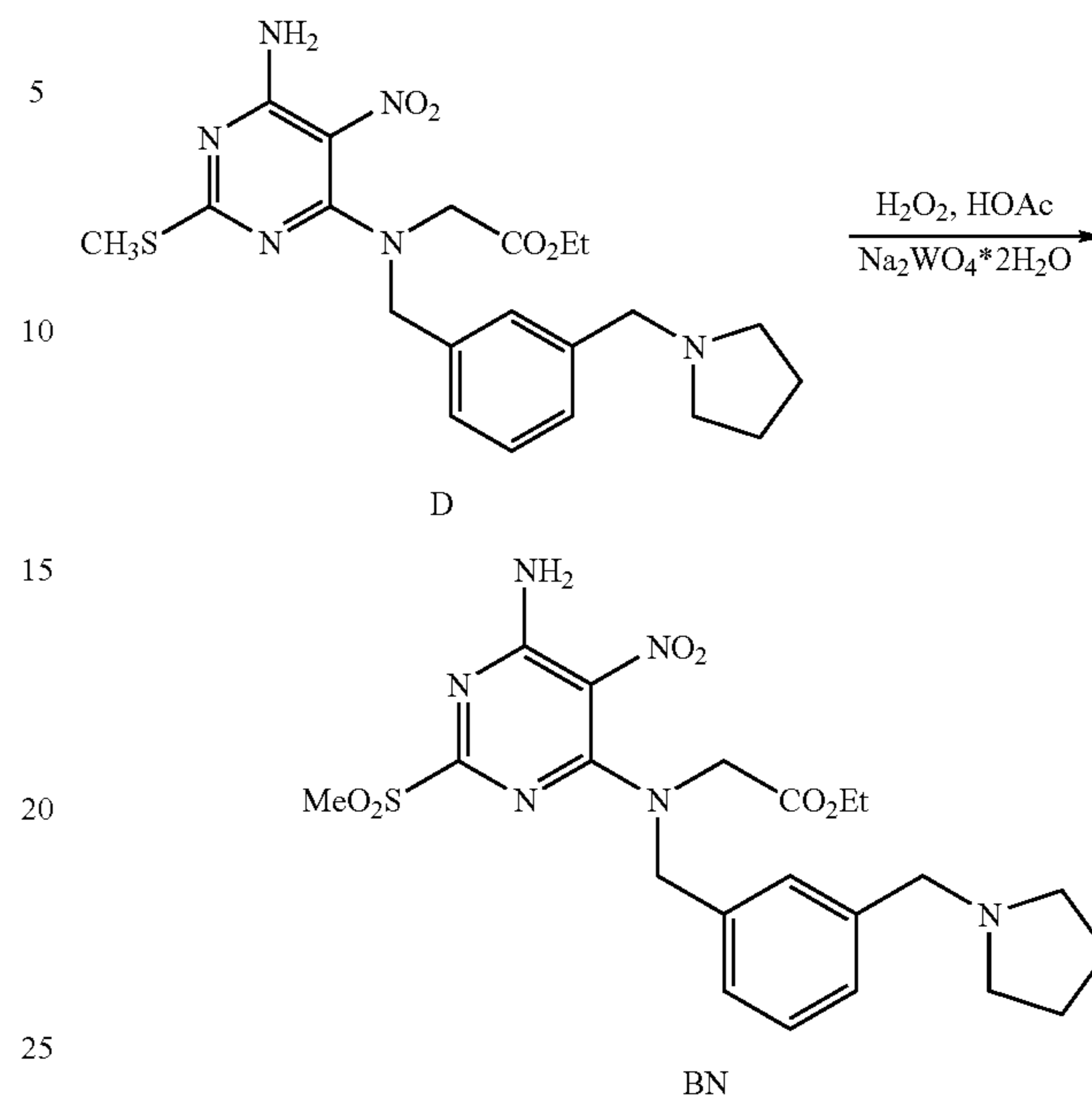
Scheme 32
