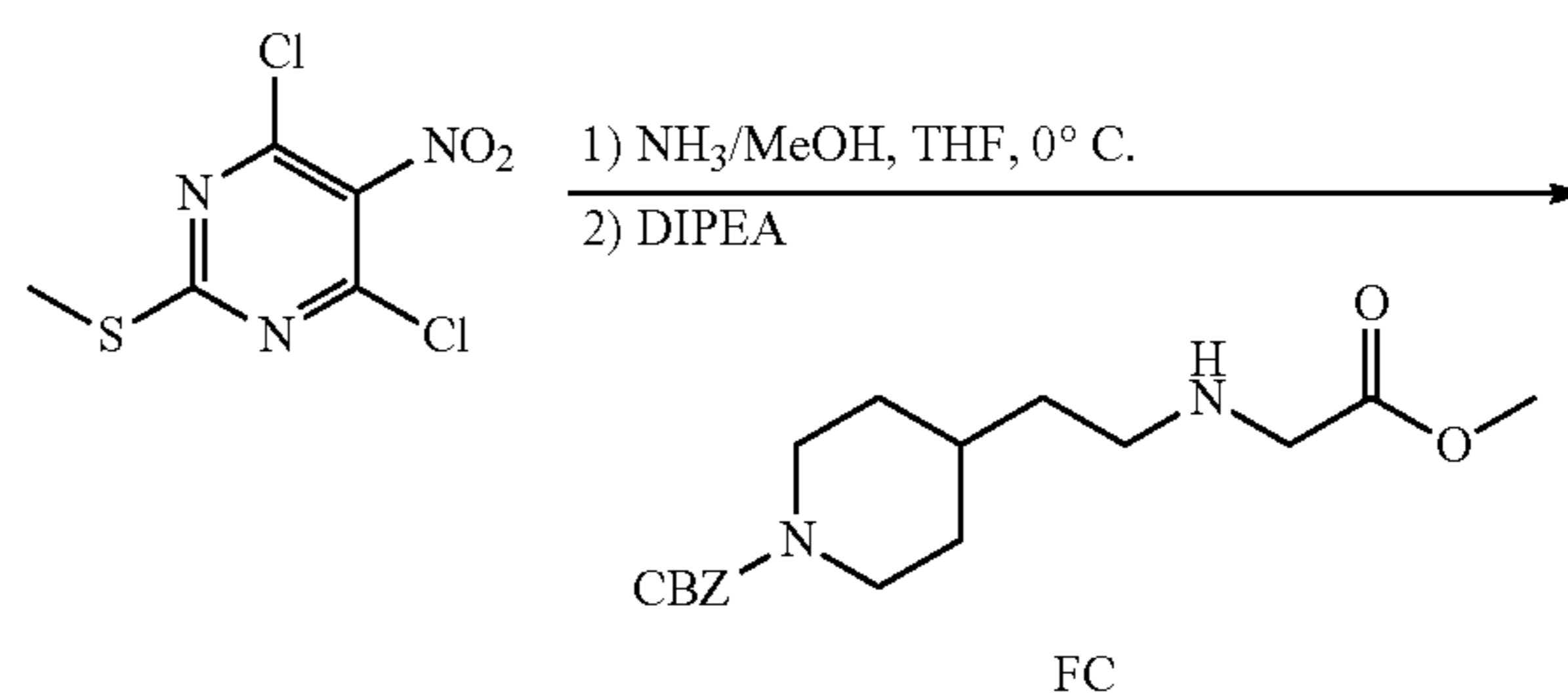
Scheme 92
