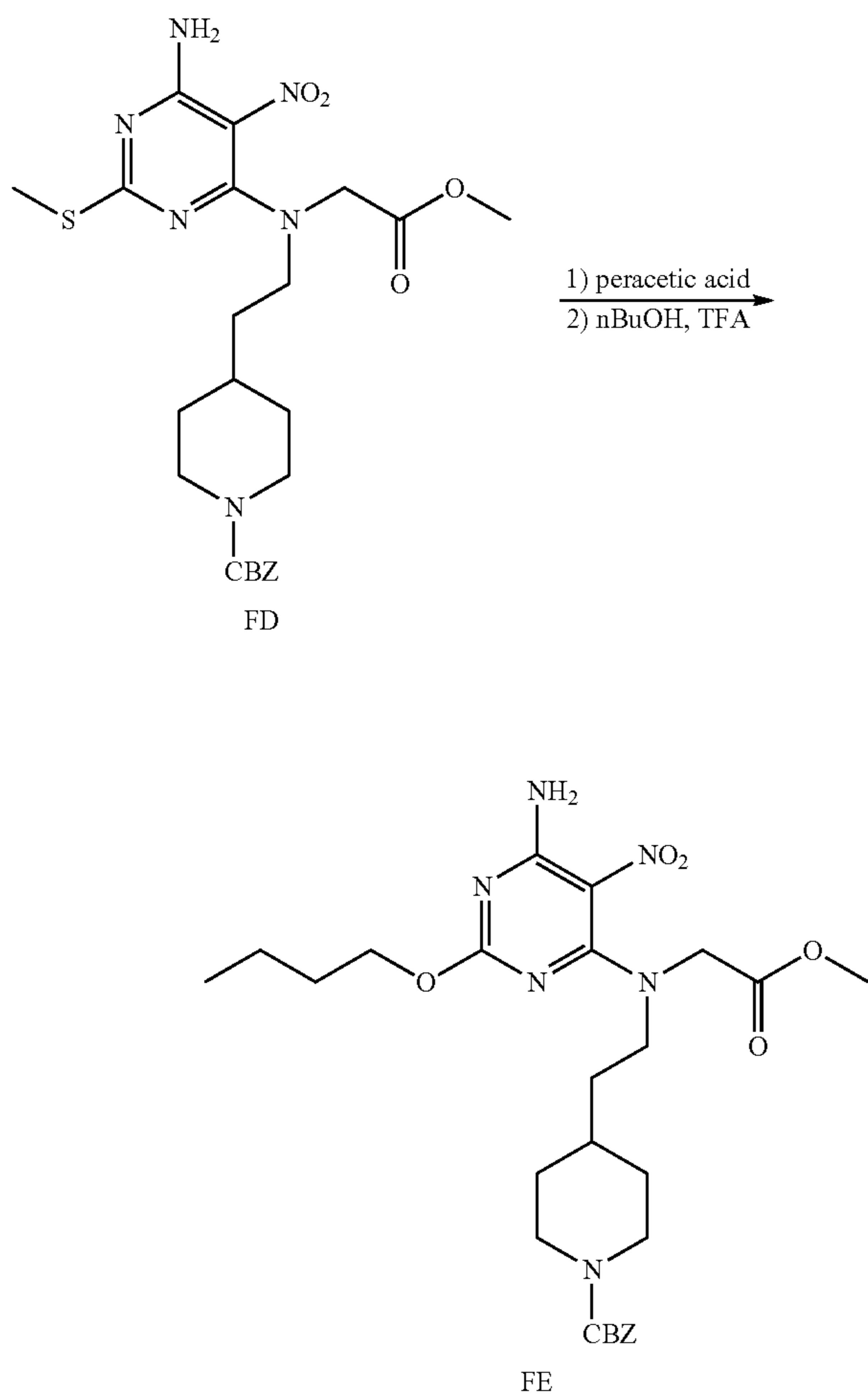
Scheme 93
