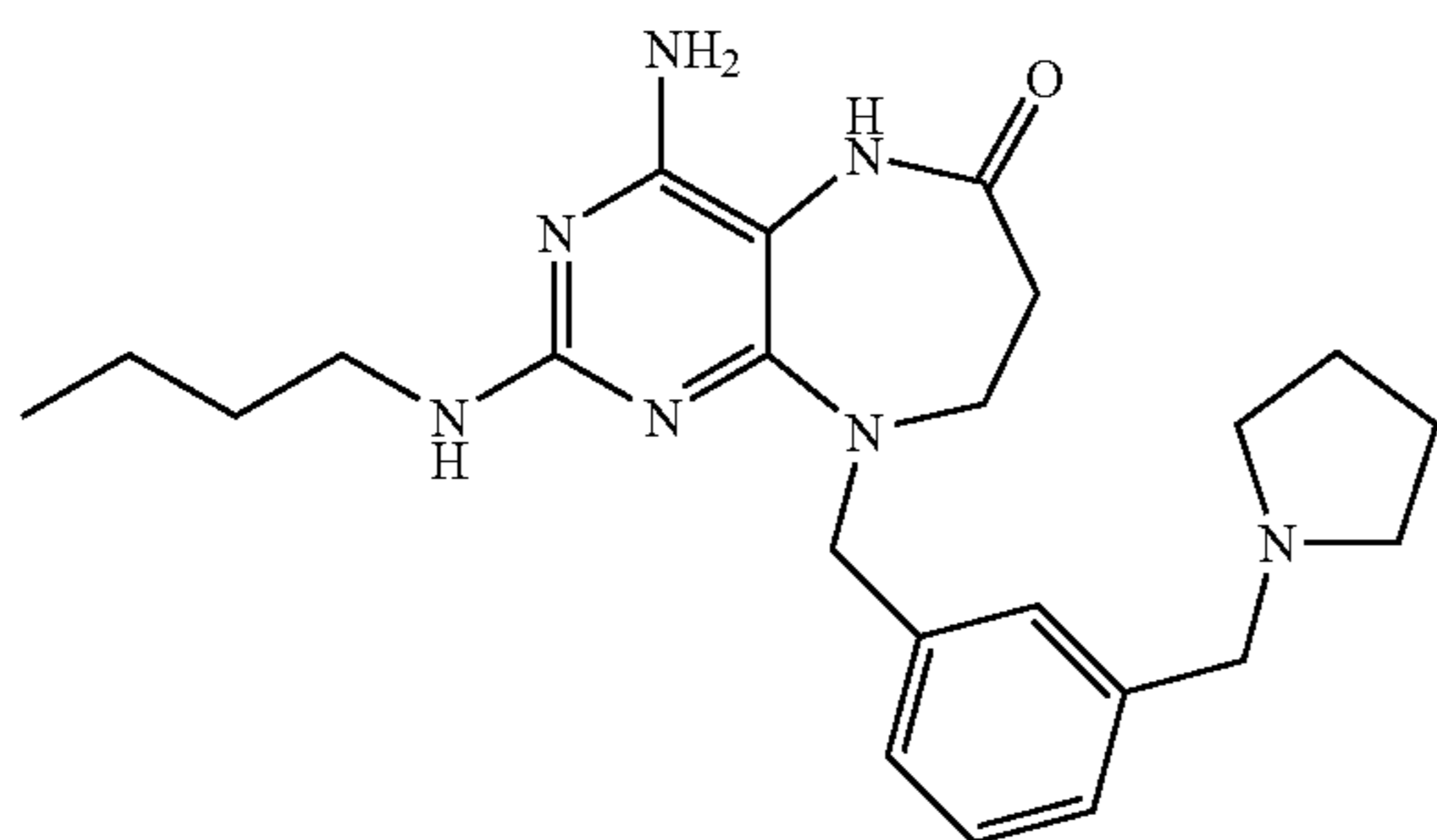
Example 76
