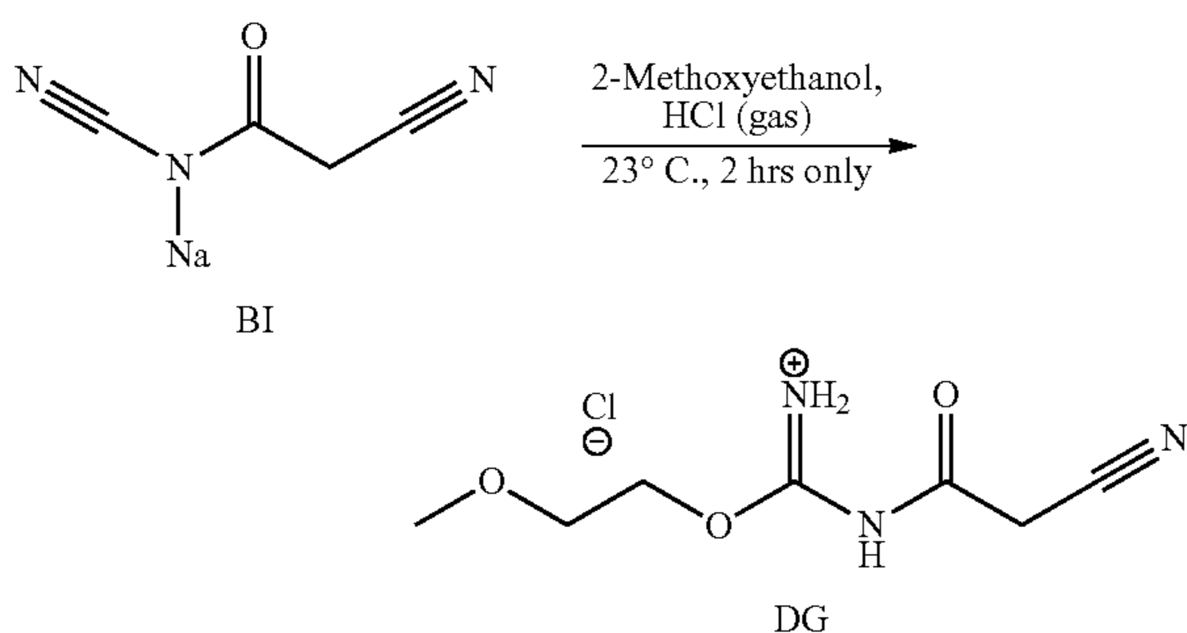
Scheme 74
