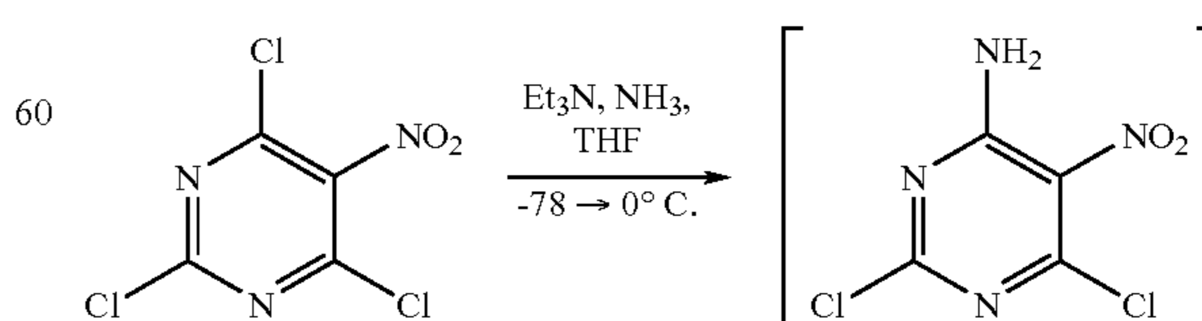
Scheme 39
