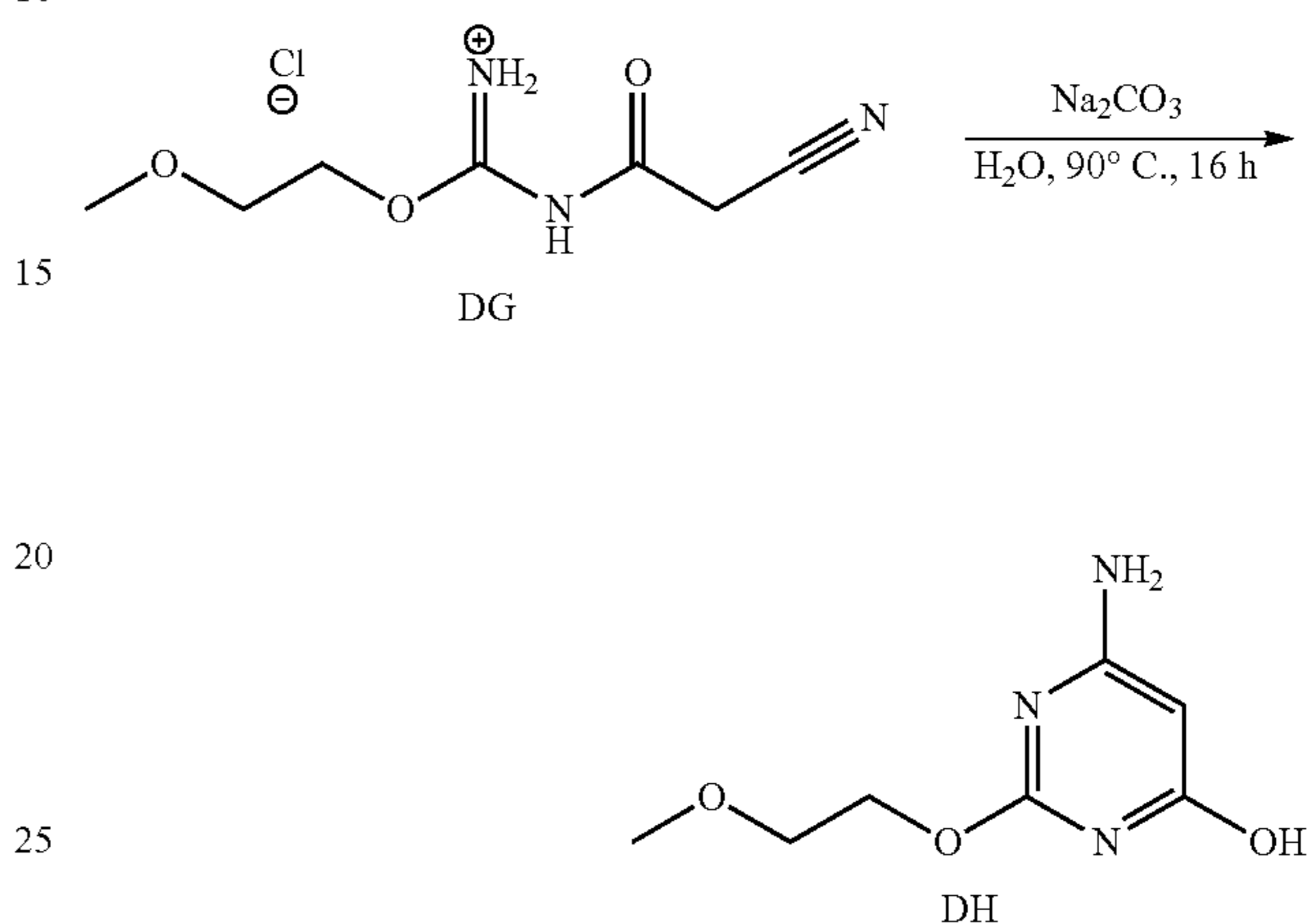
Scheme 75
