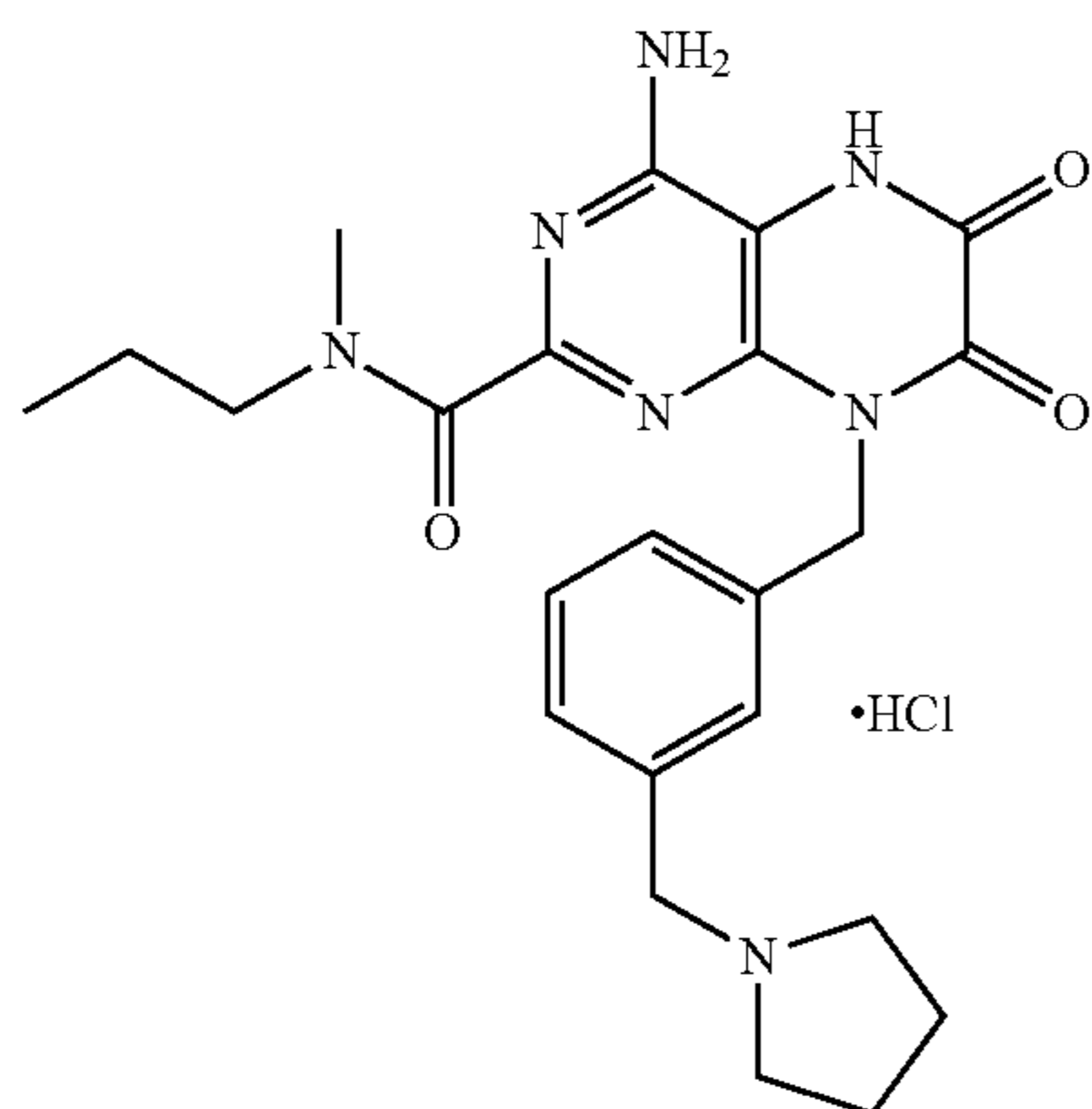
Example 92
