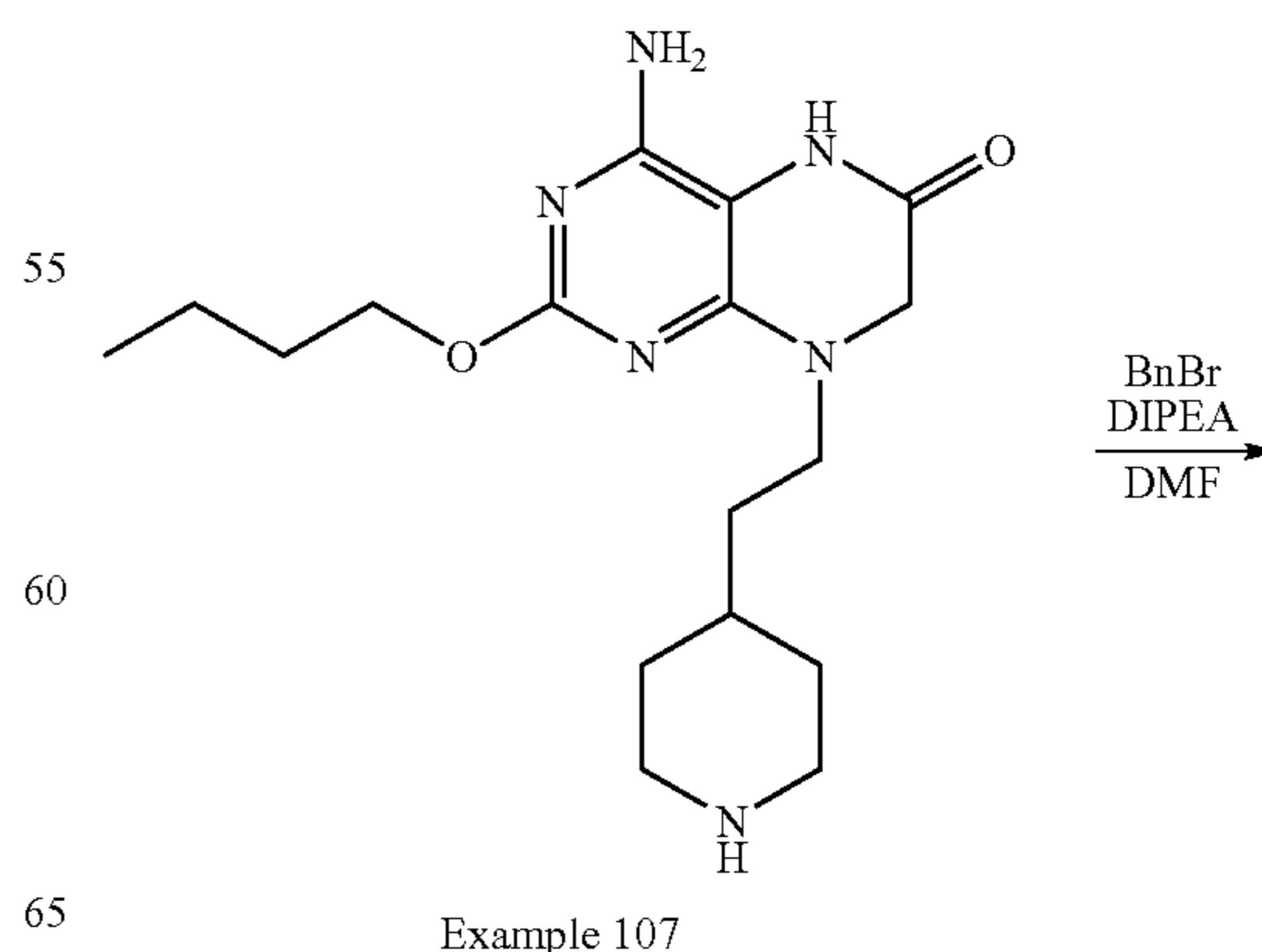
Scheme 95: Example 108
