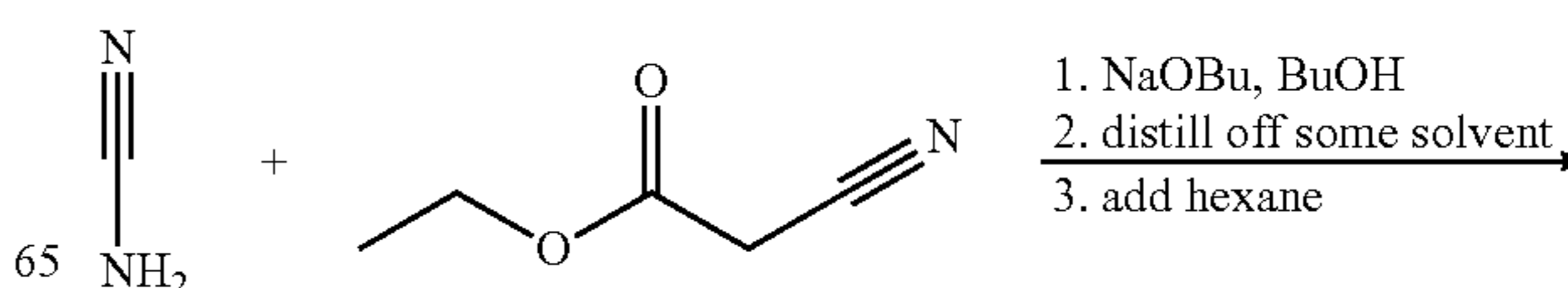
Scheme 27
