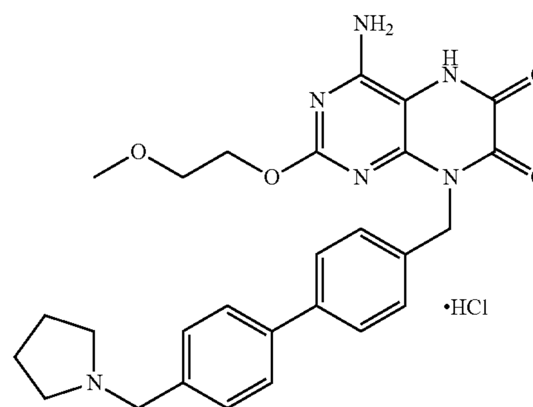
Example 99
