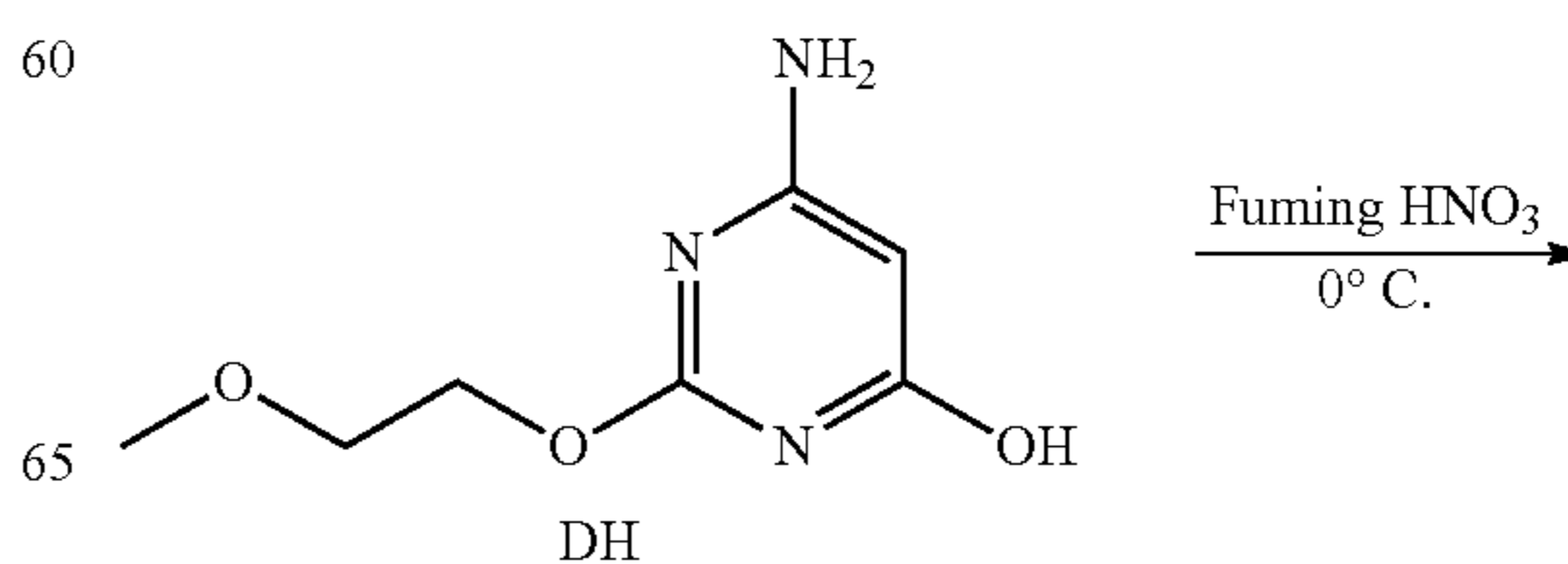
Scheme 76
