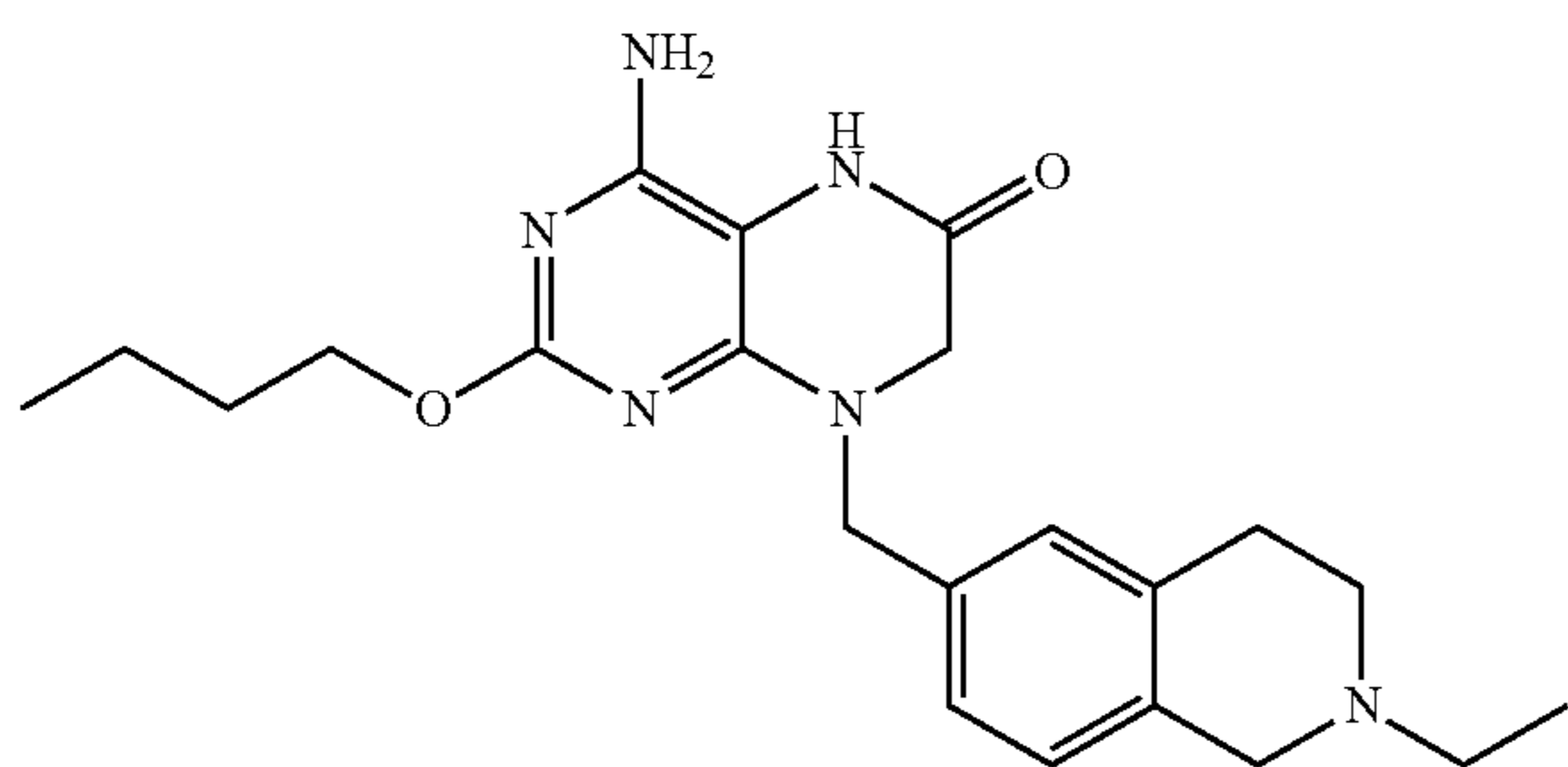
Example 104
