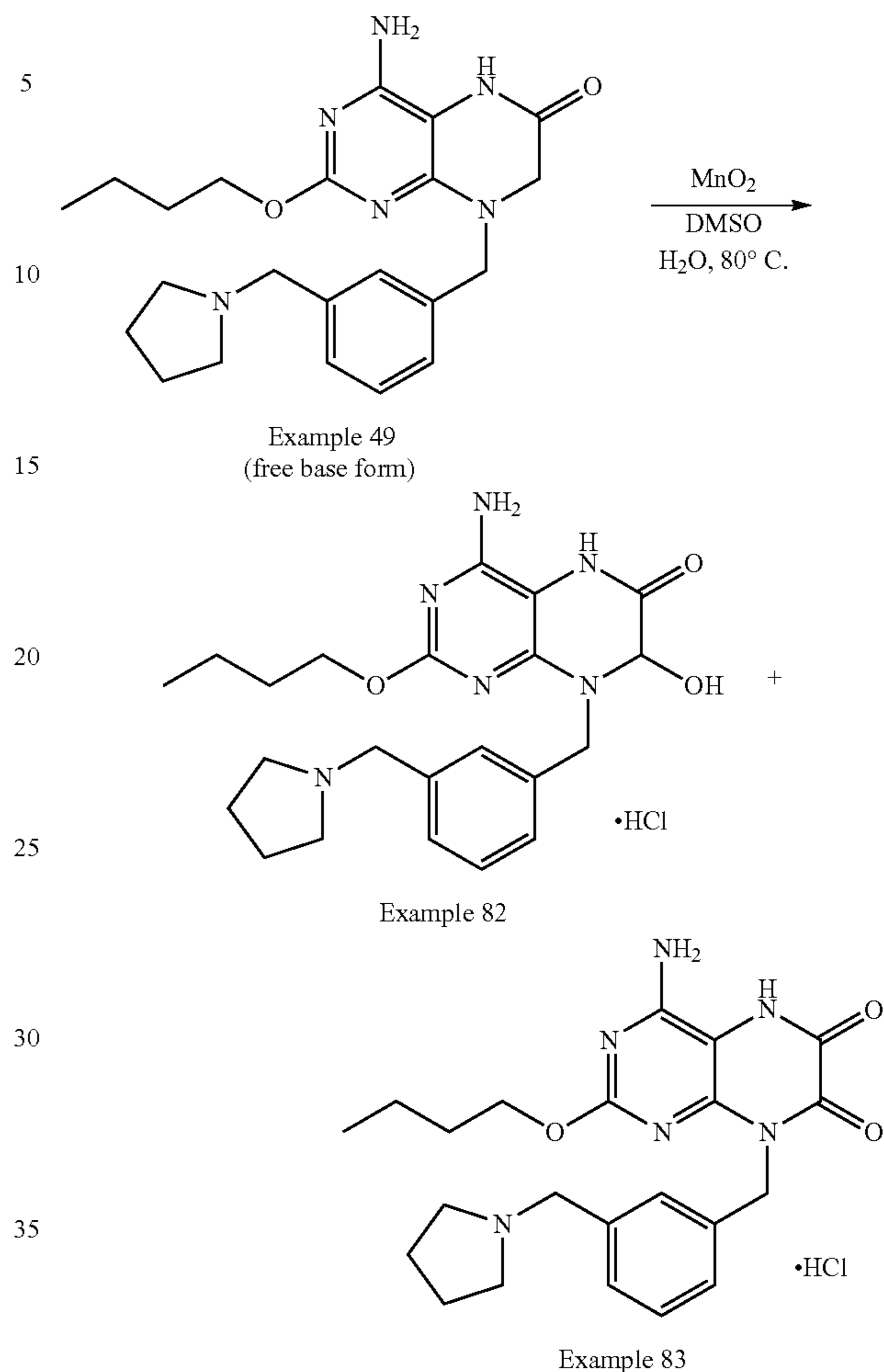
Scheme 87
