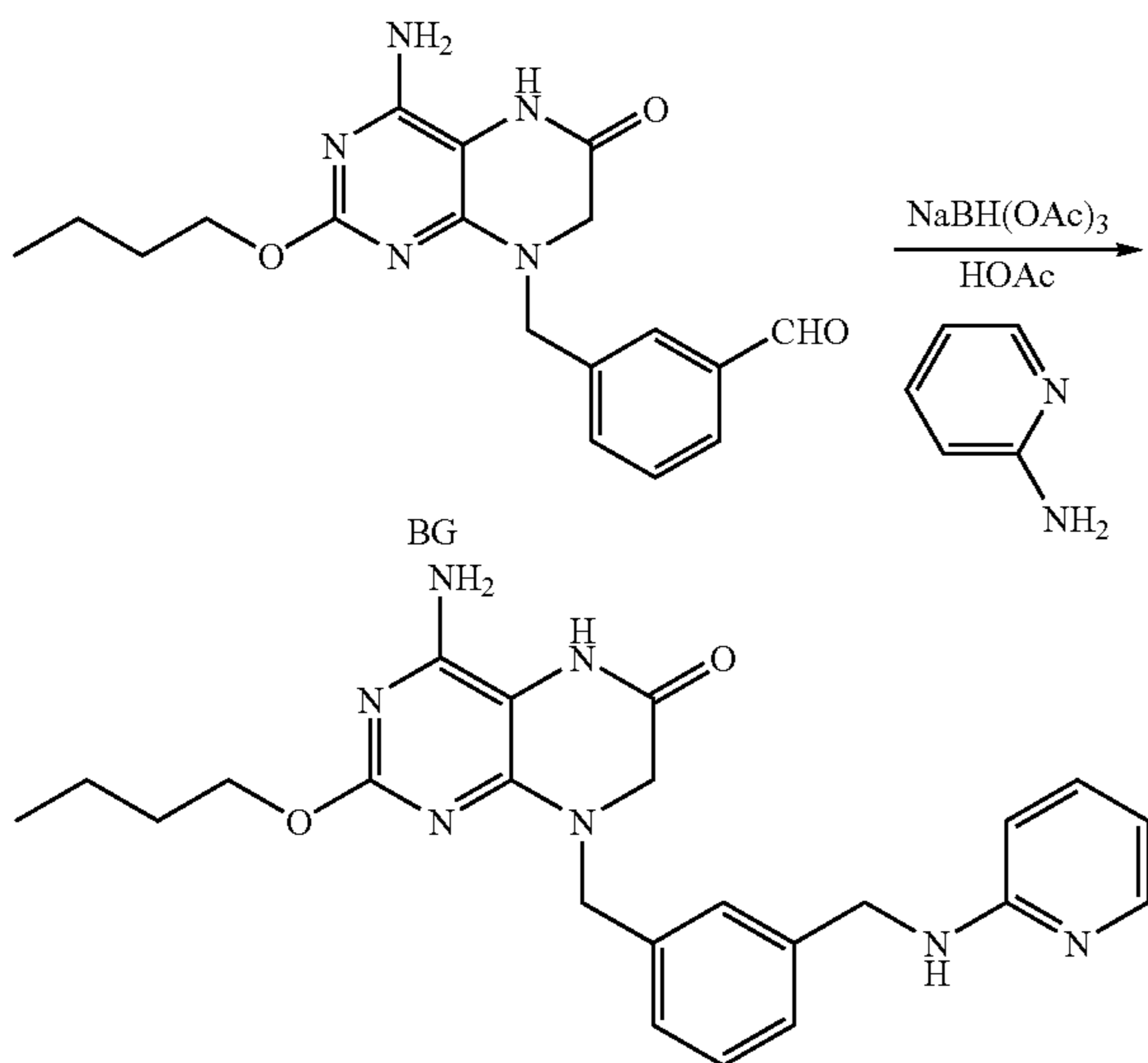
Example 80
