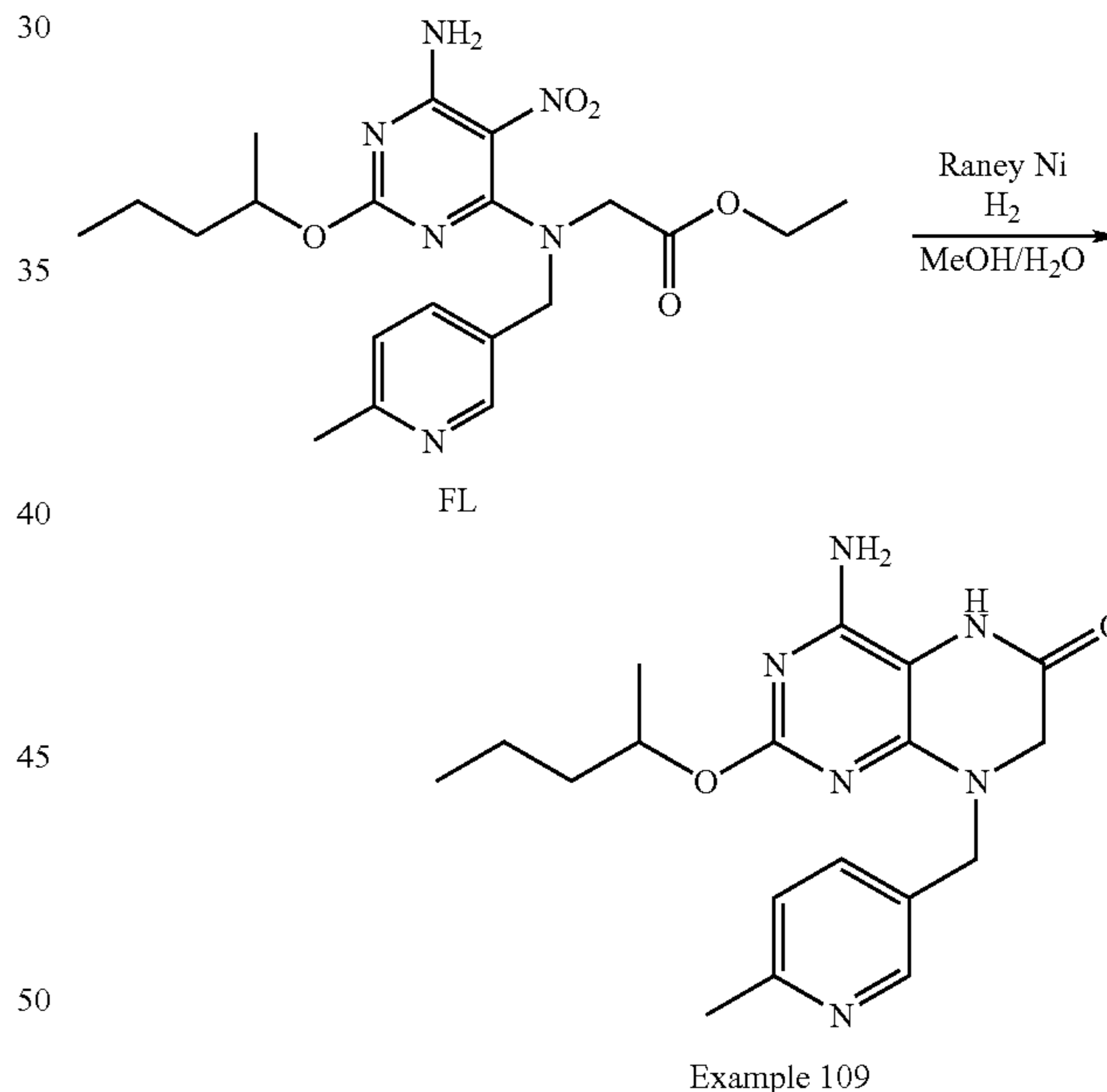
Scheme 101:
