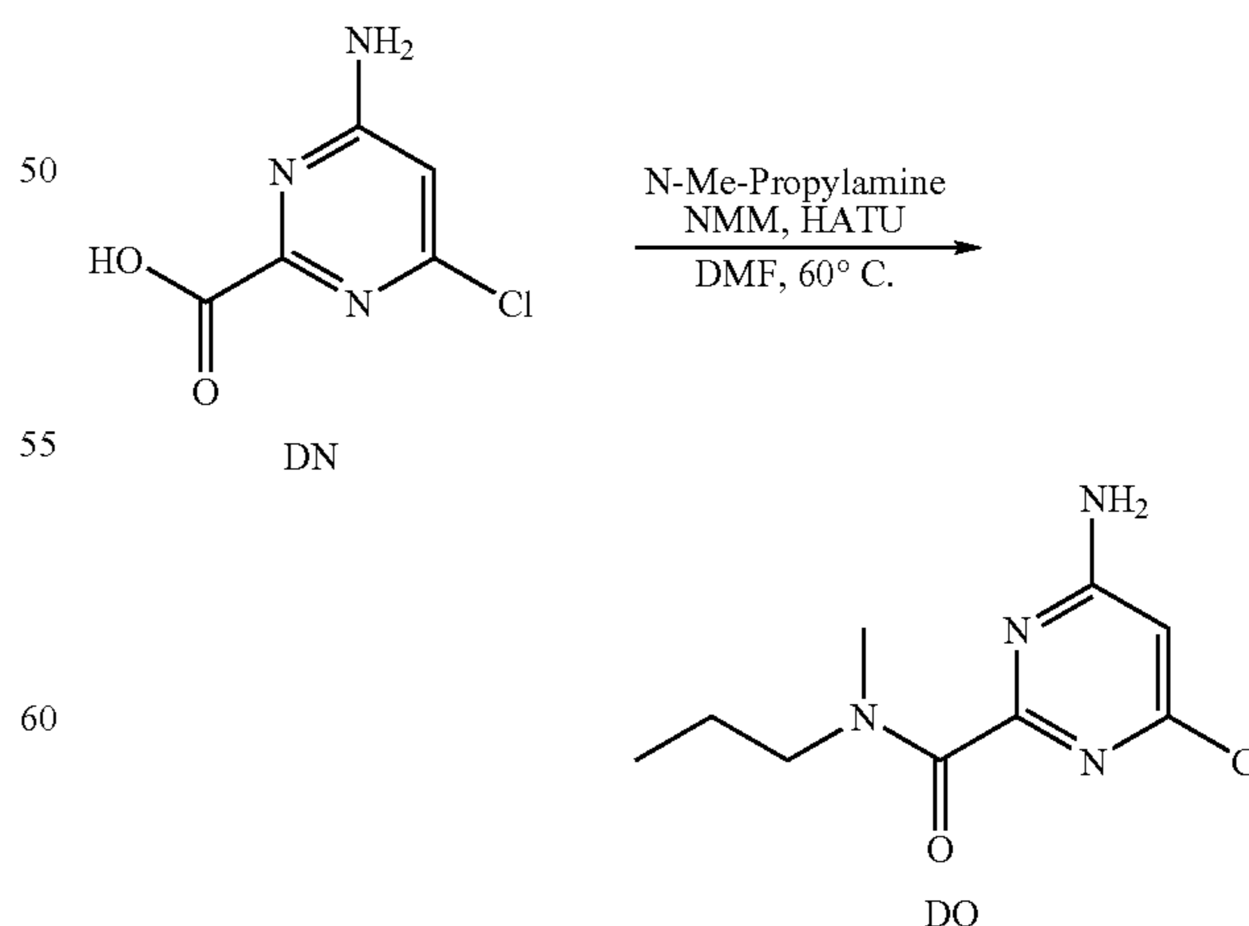
Scheme 81:
