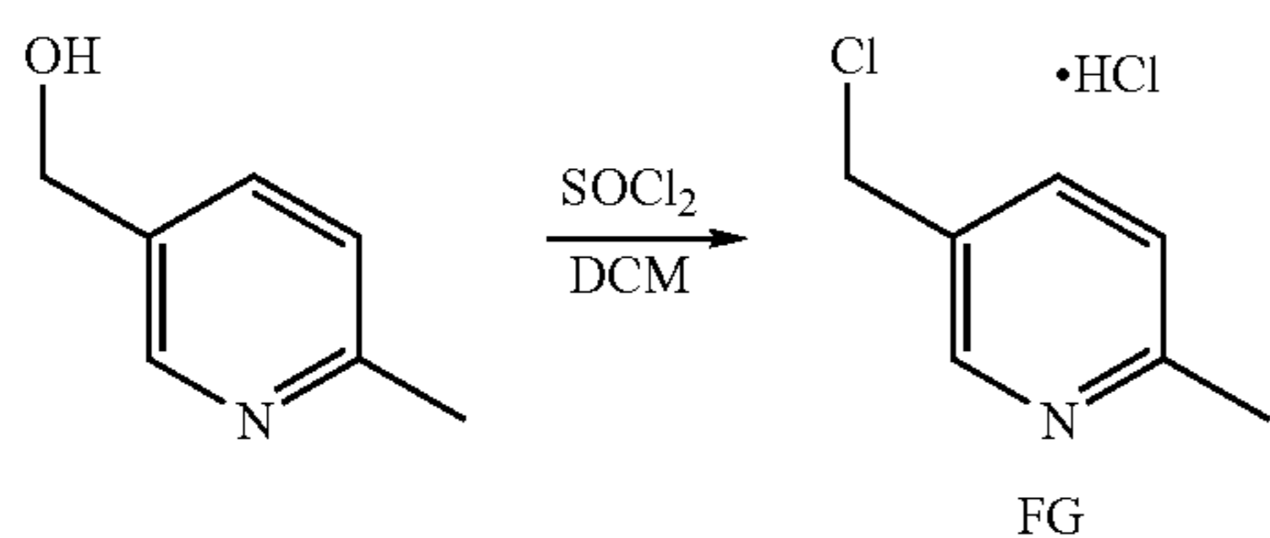
Scheme 96:
