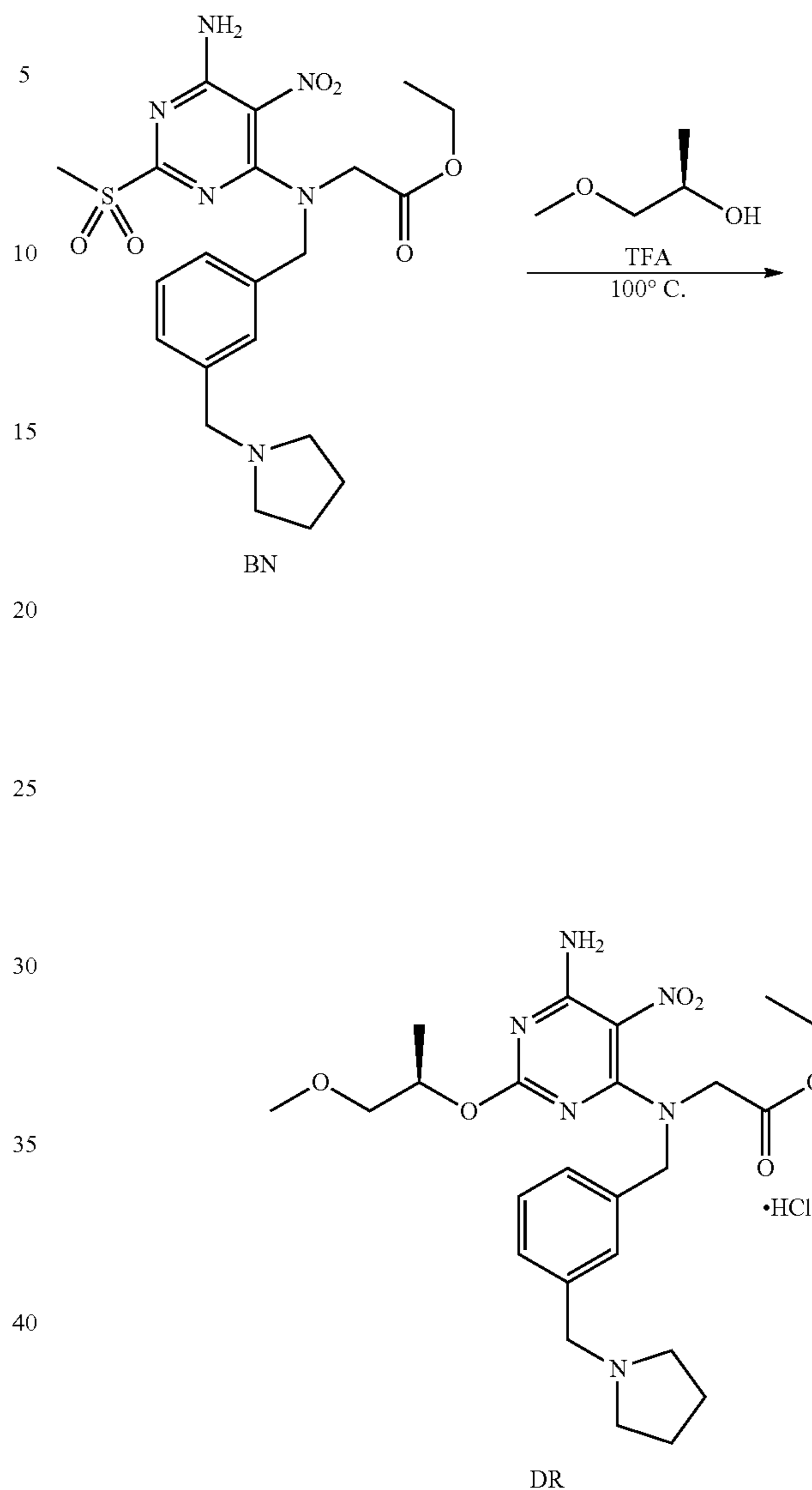
Scheme 85
