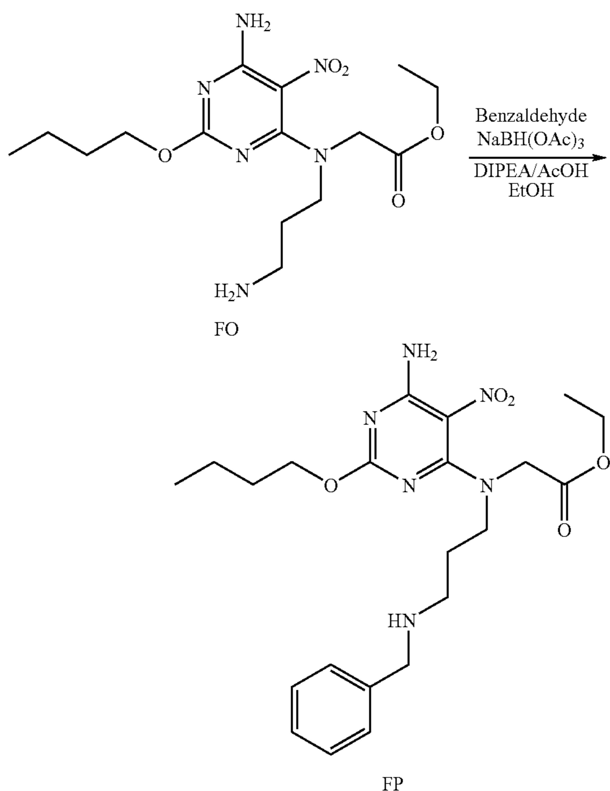
Scheme 106:
