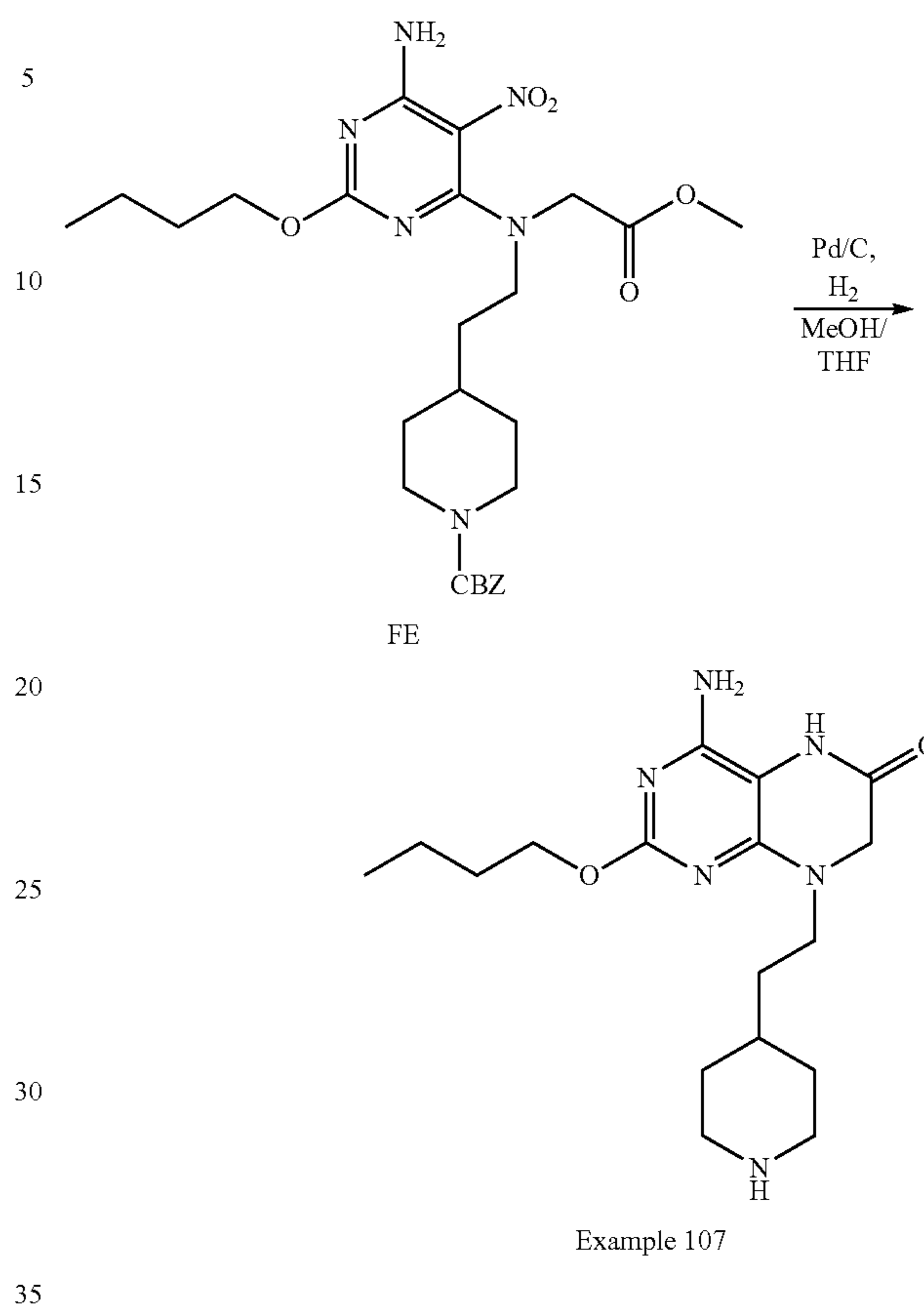
Scheme 94
