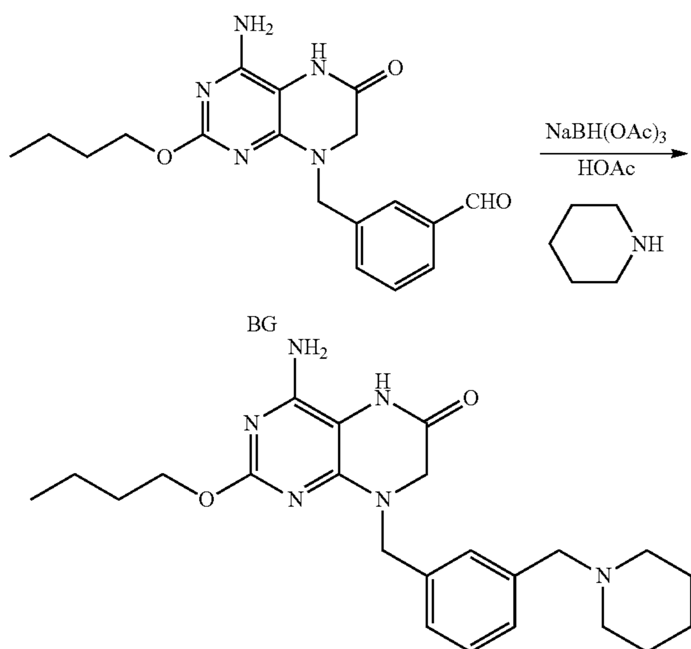
Example 48
