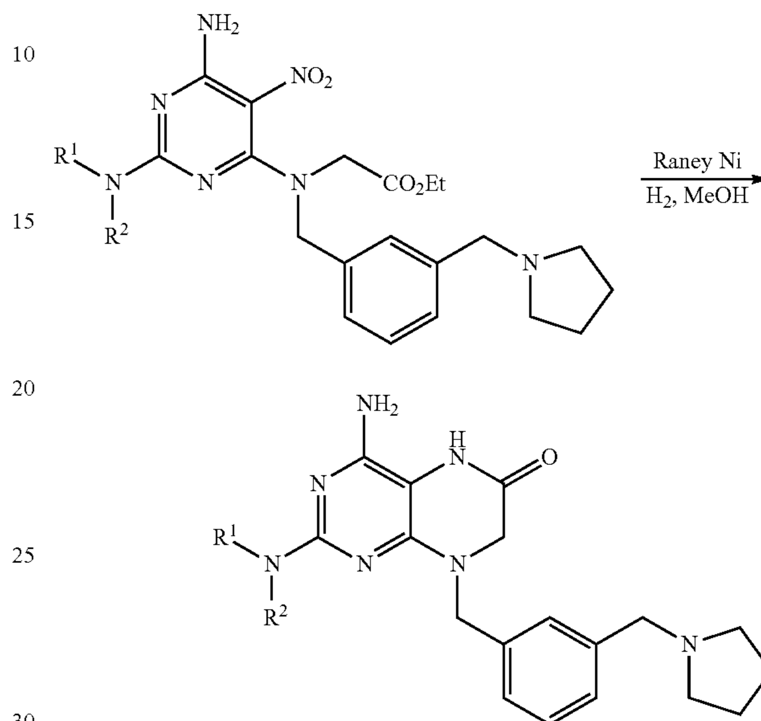
Scheme 17
