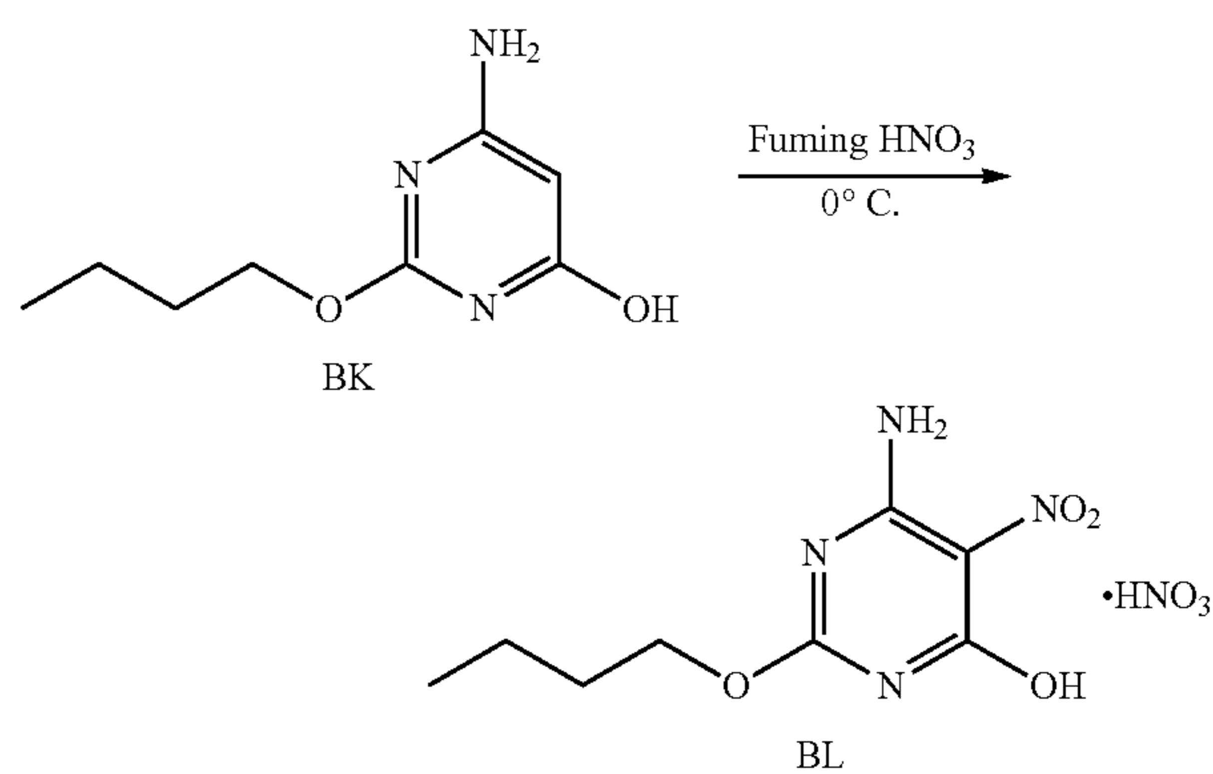
Scheme 30
