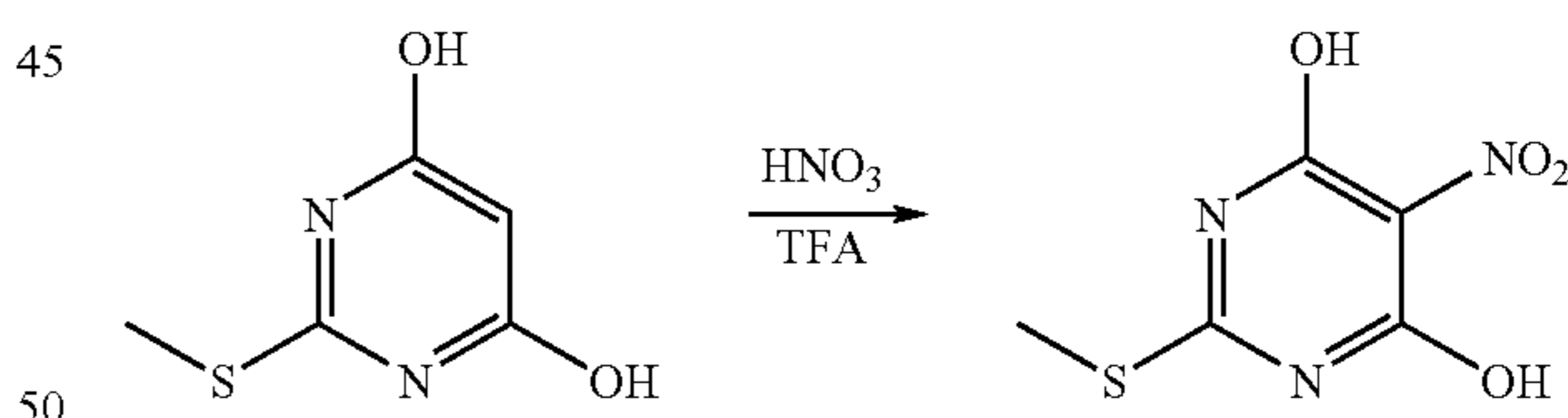
Scheme 7
