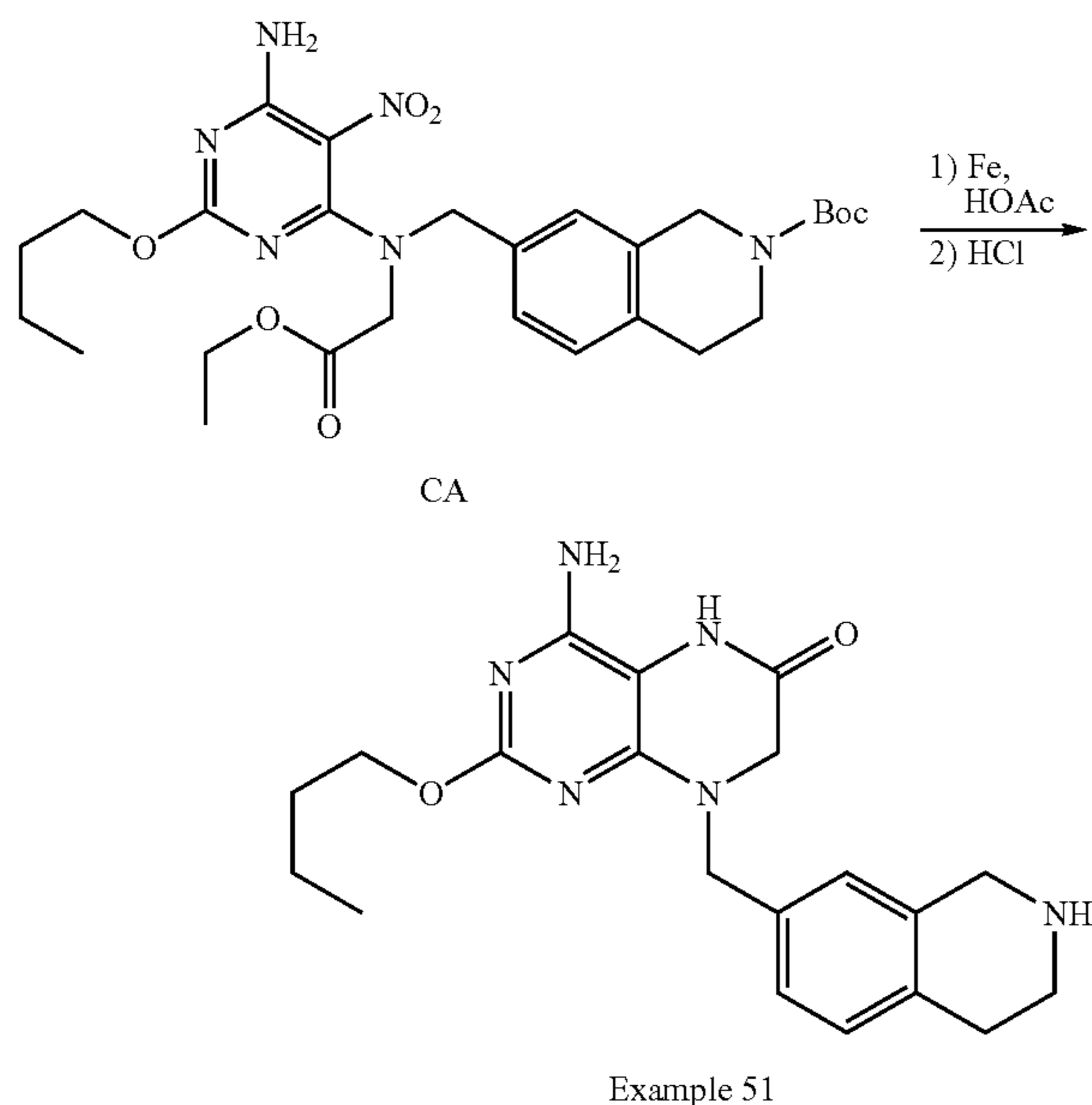
Scheme 47: Example 51
