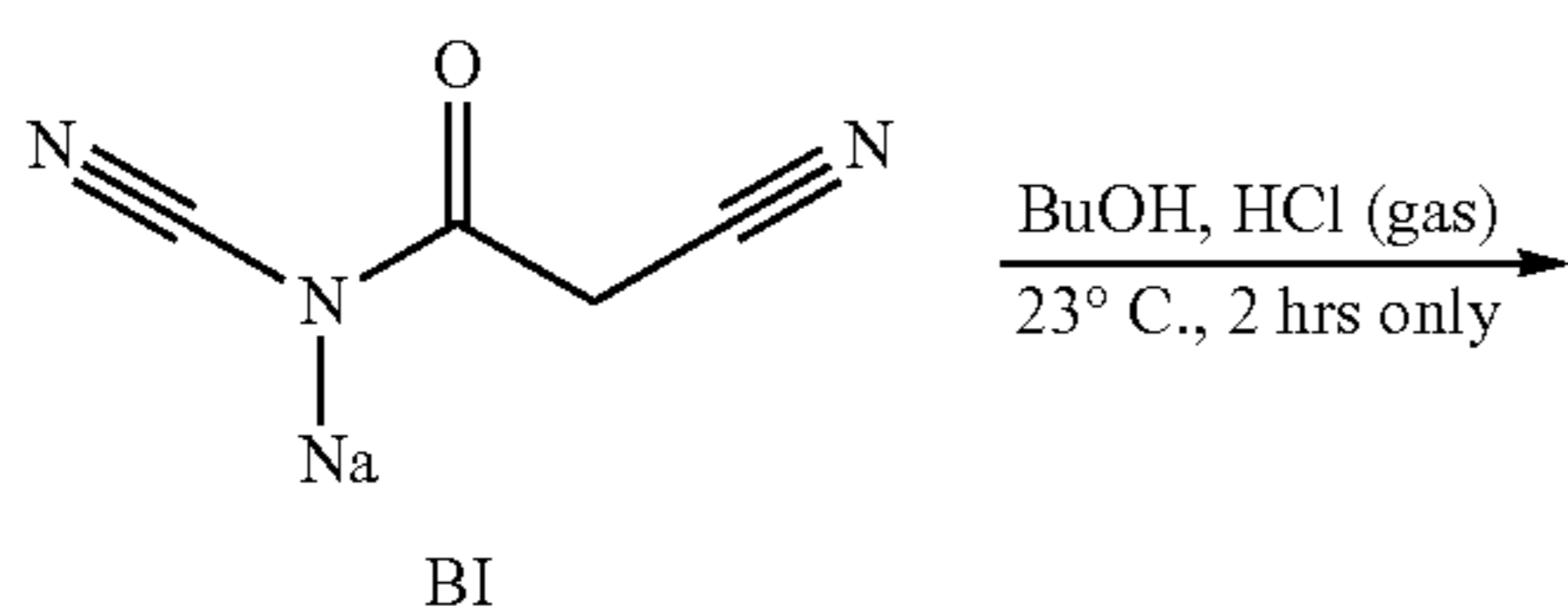
Scheme 28
