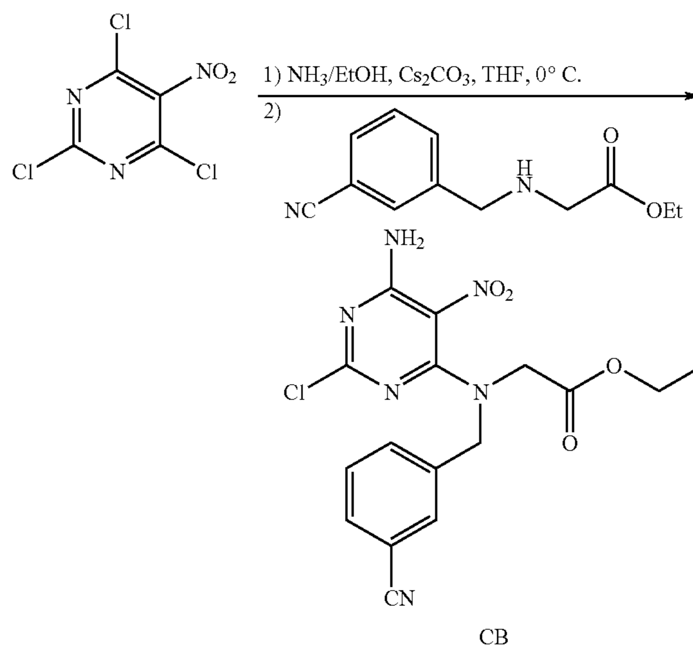
Scheme 49
