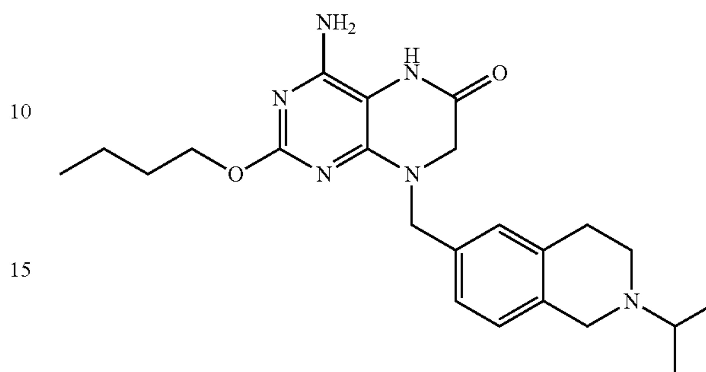
Example 105
