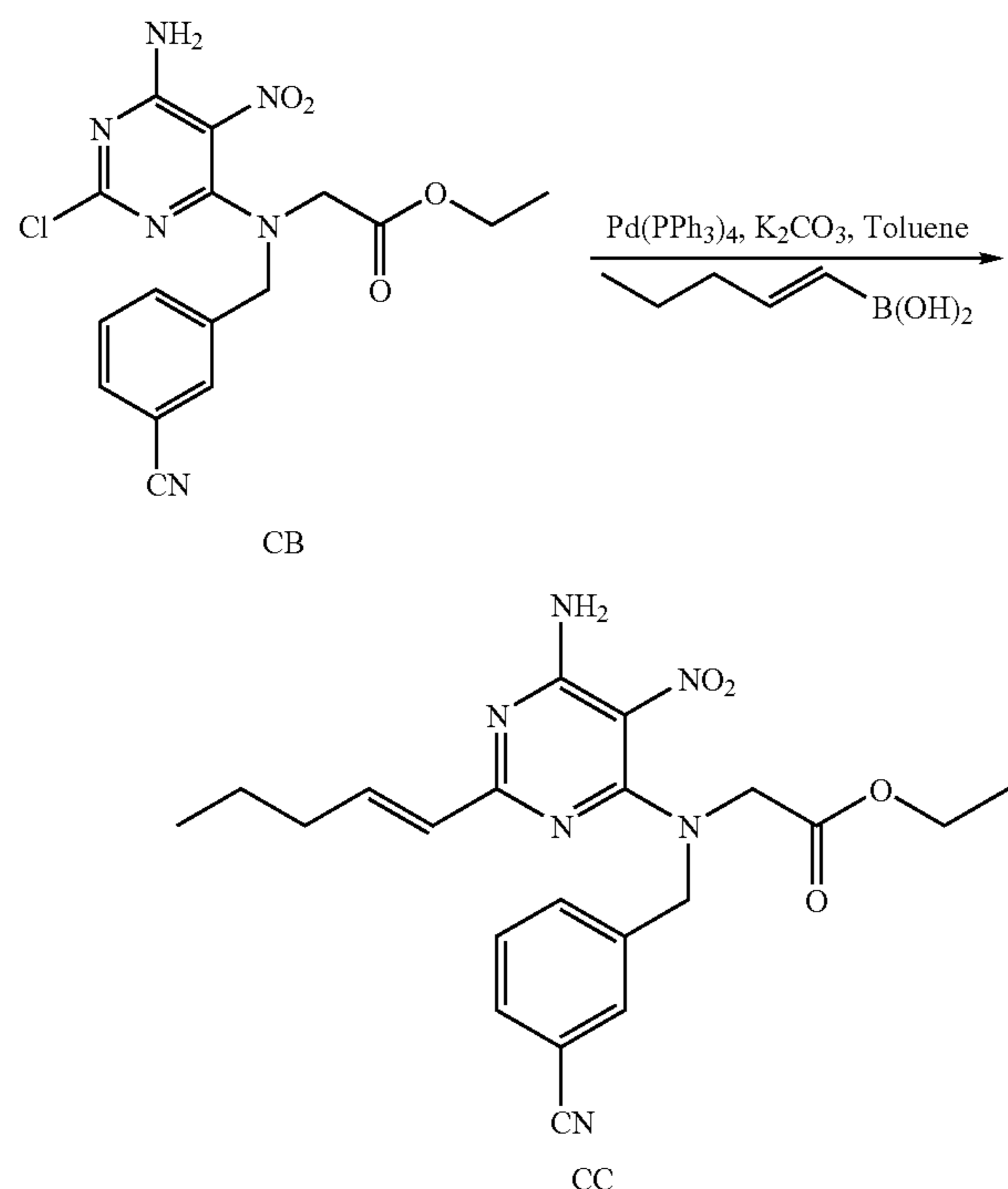
Scheme 50
