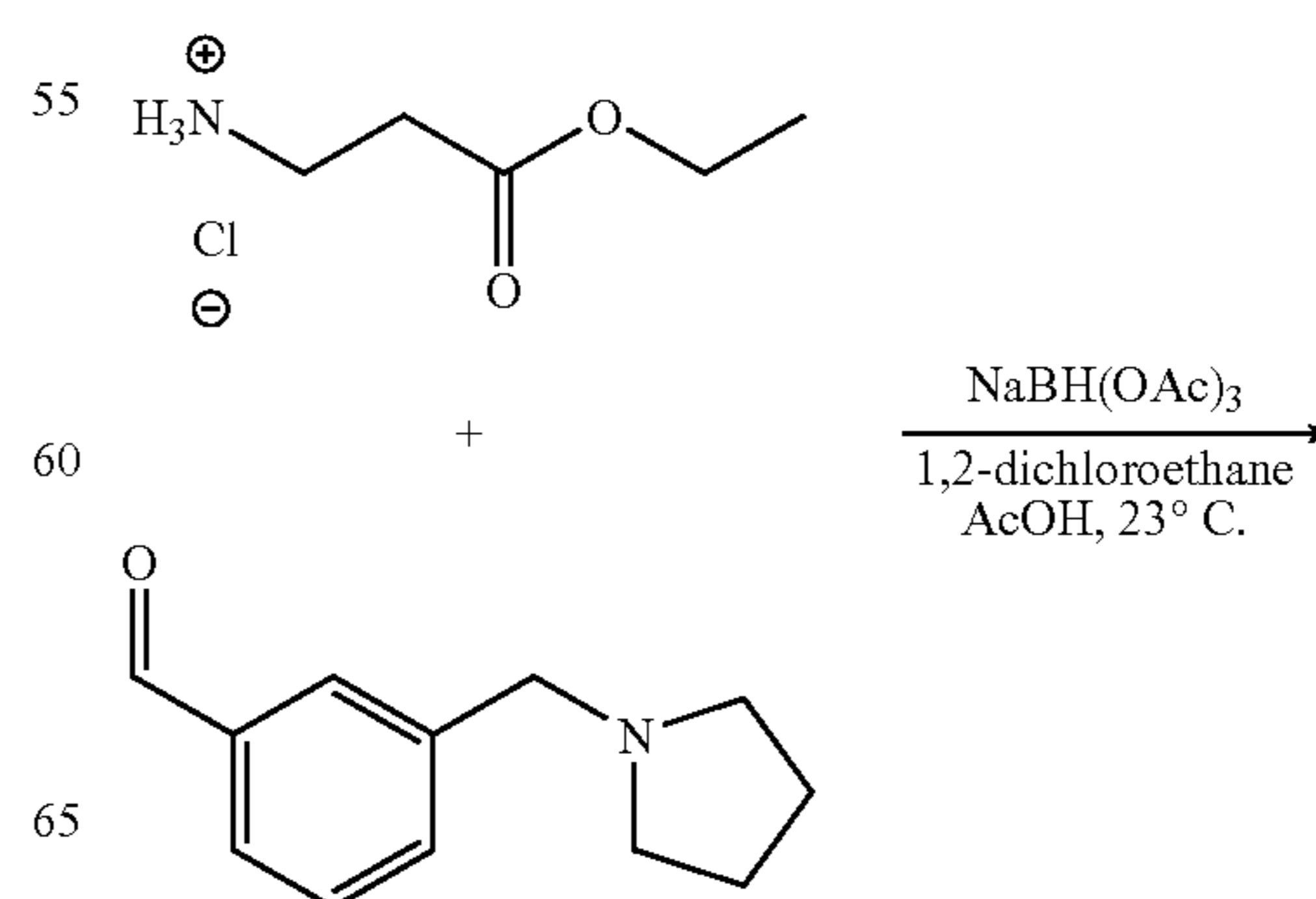
Scheme 33
