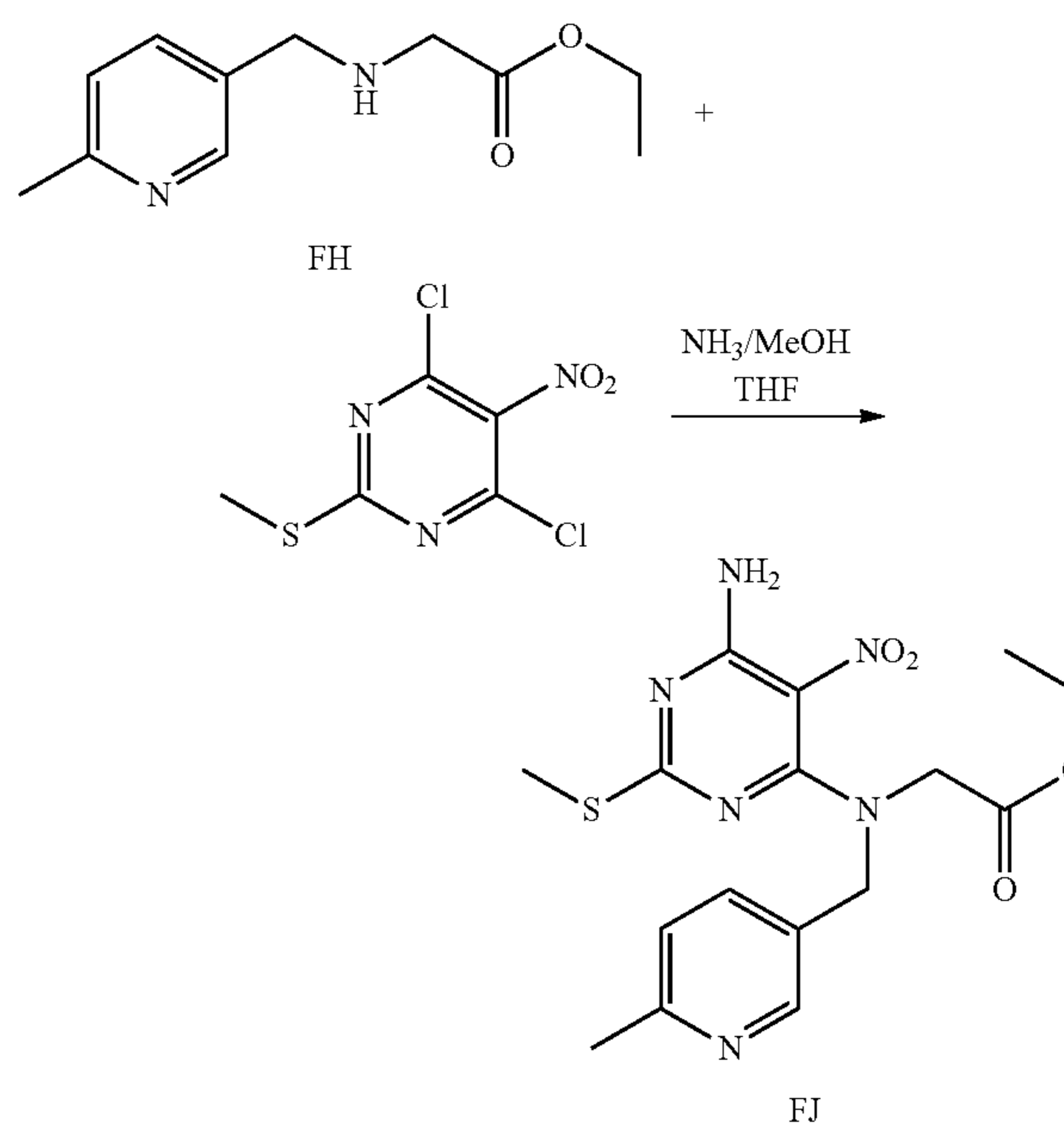
Scheme 98
