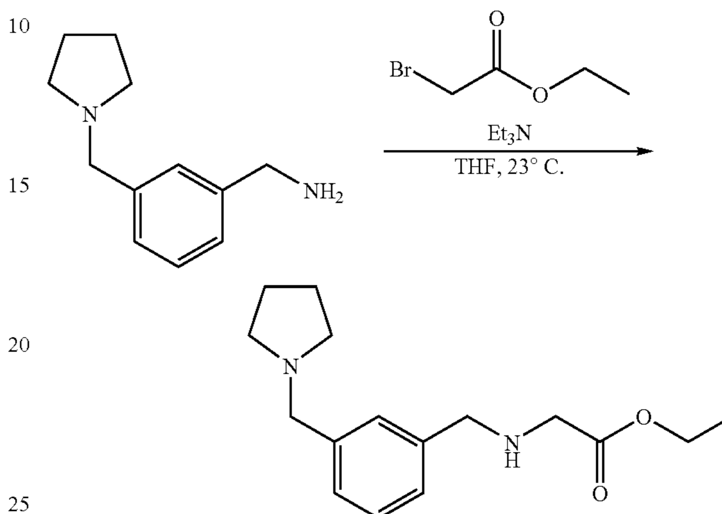
Scheme 6
