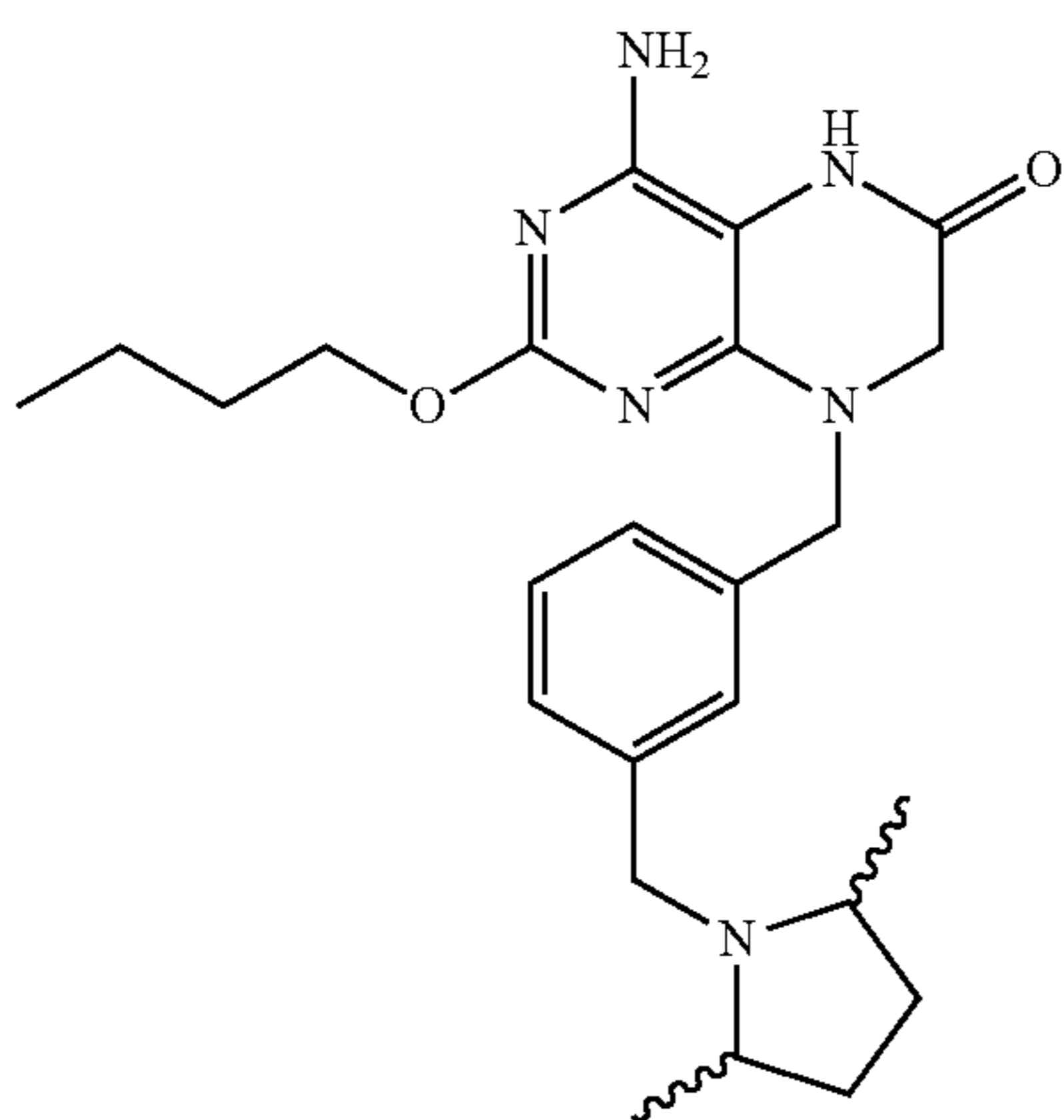
Example 102
