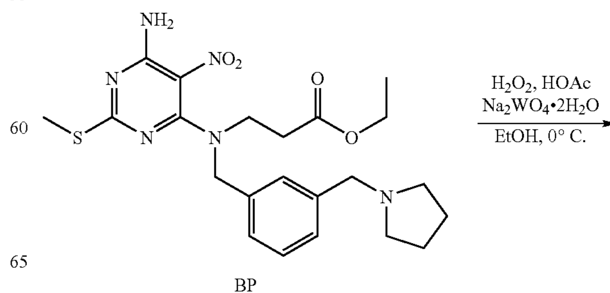
Scheme 36
