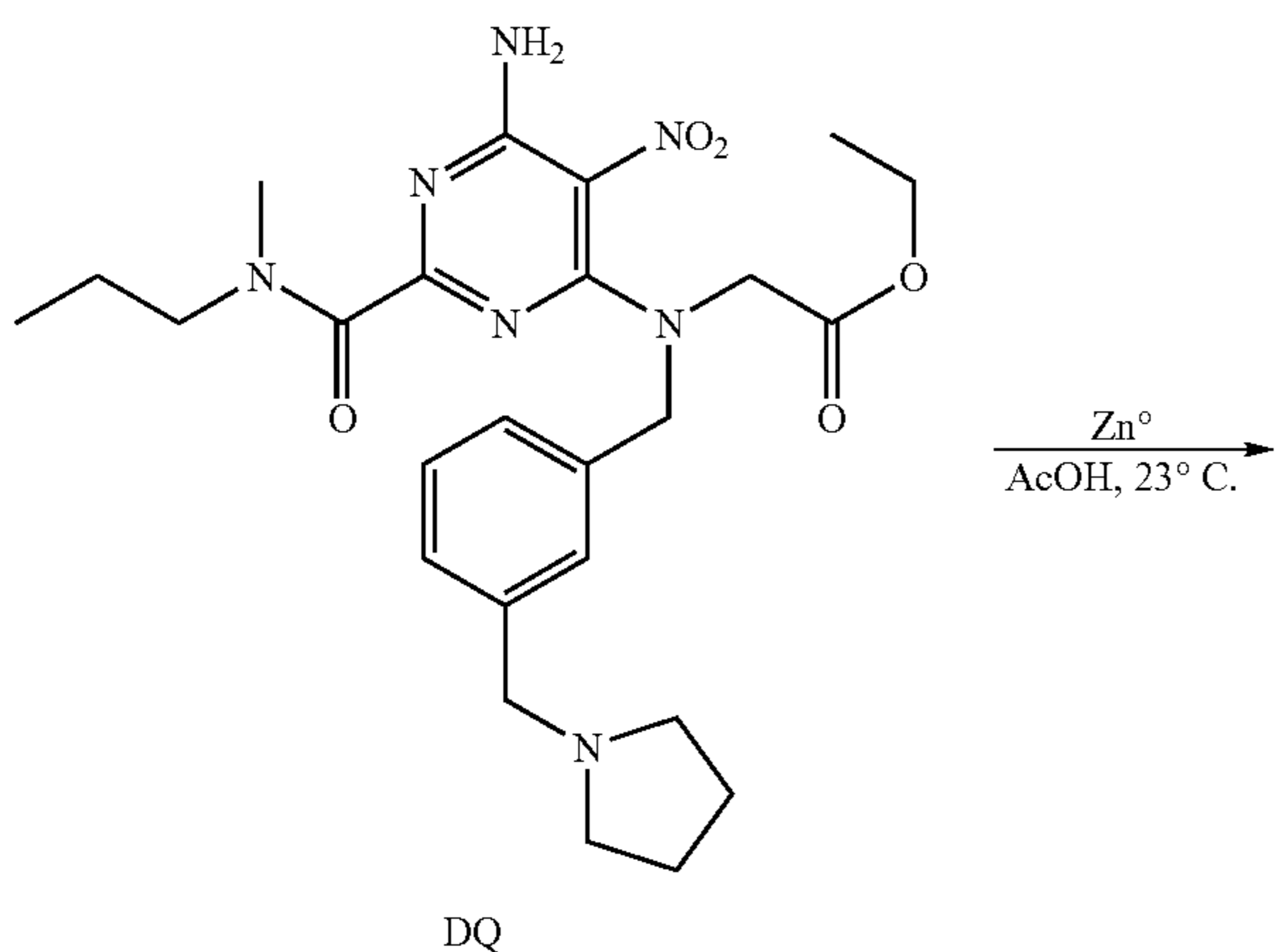
Scheme 84: Example 81
