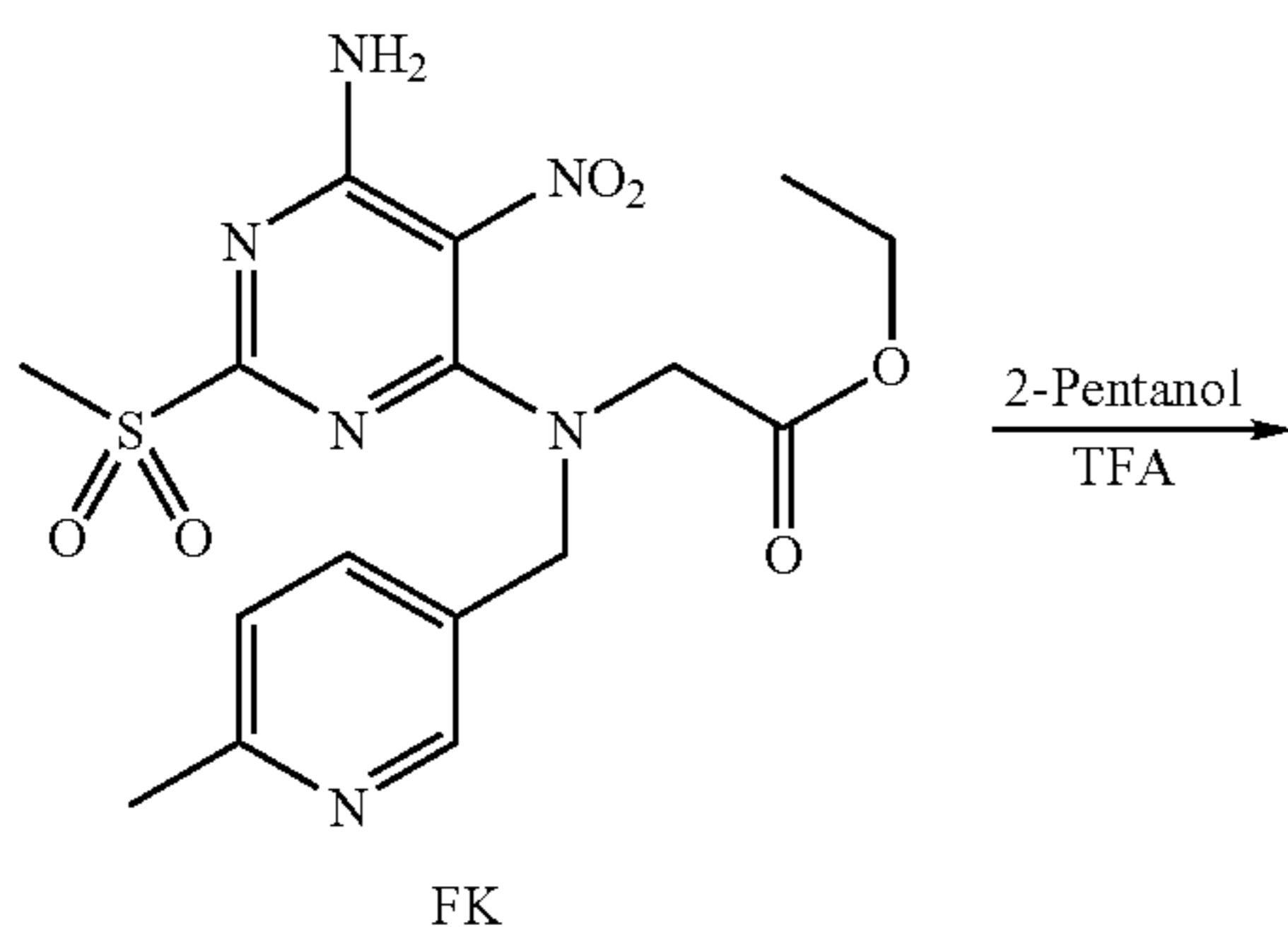
Scheme 100:
