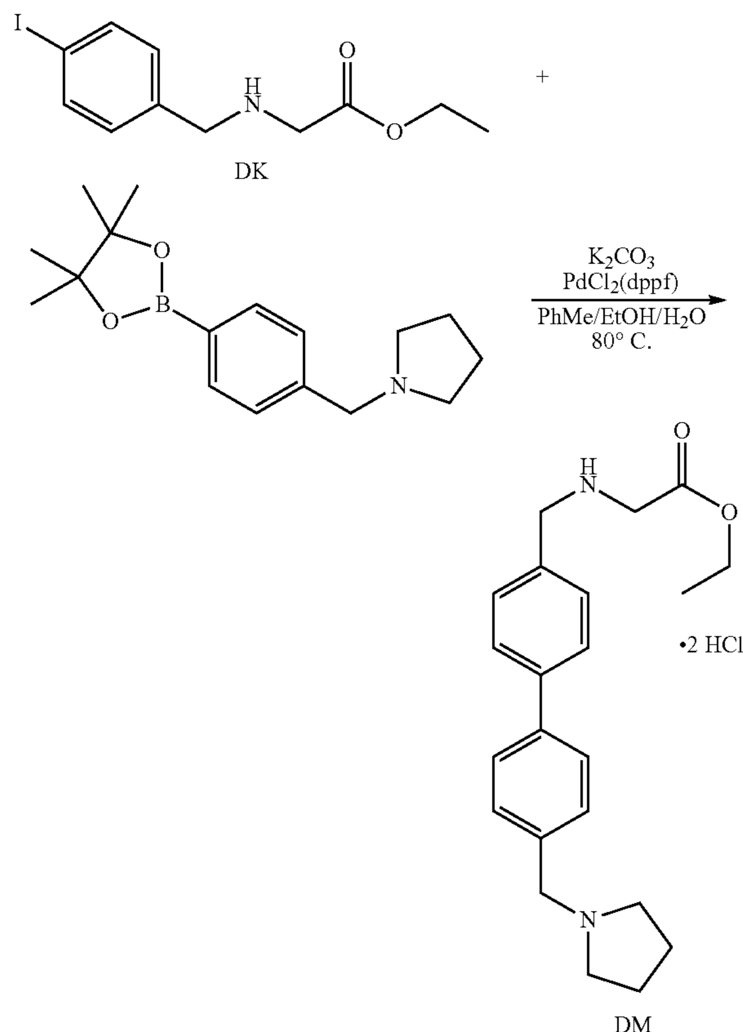
Scheme 79
