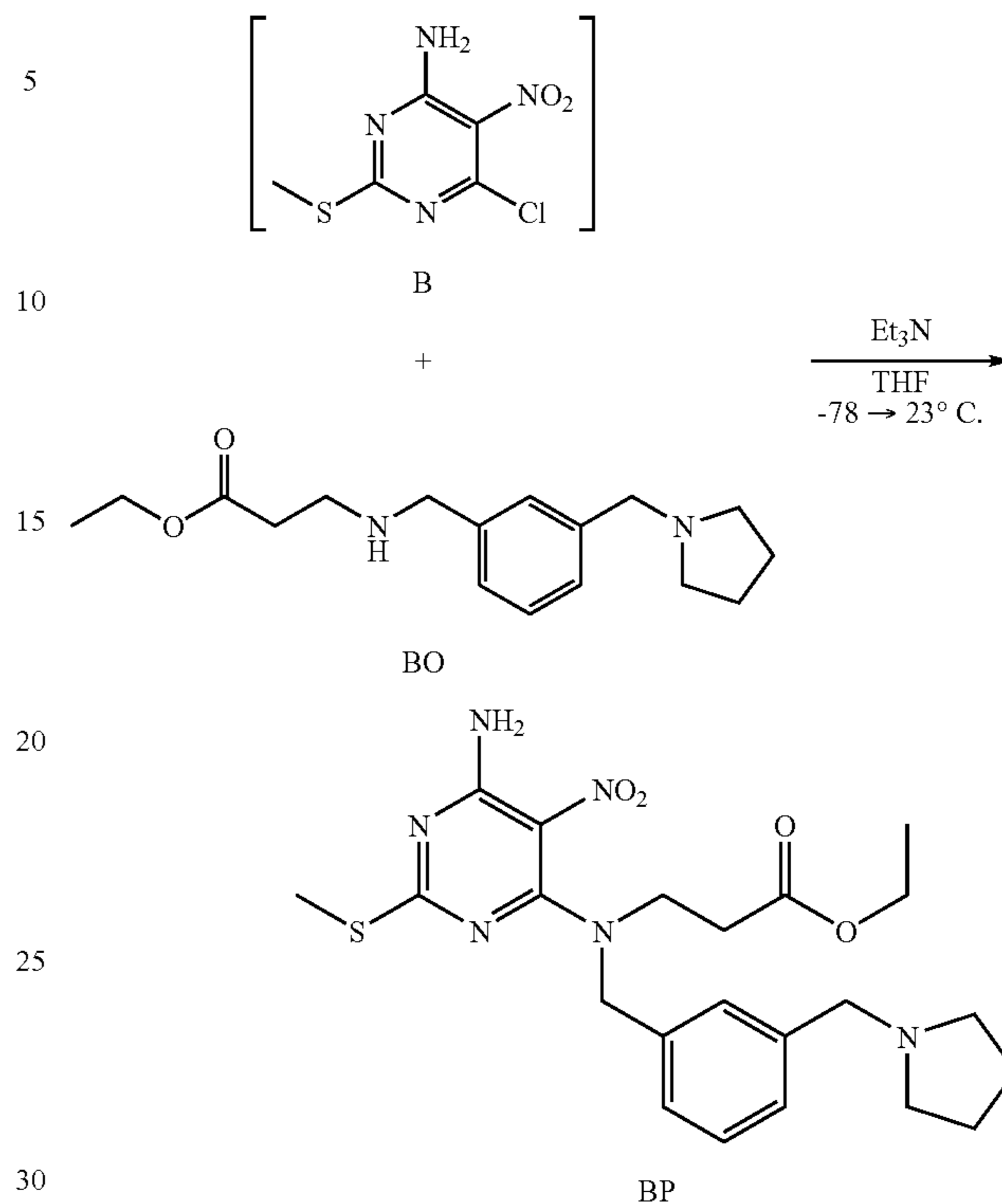
Scheme 35
