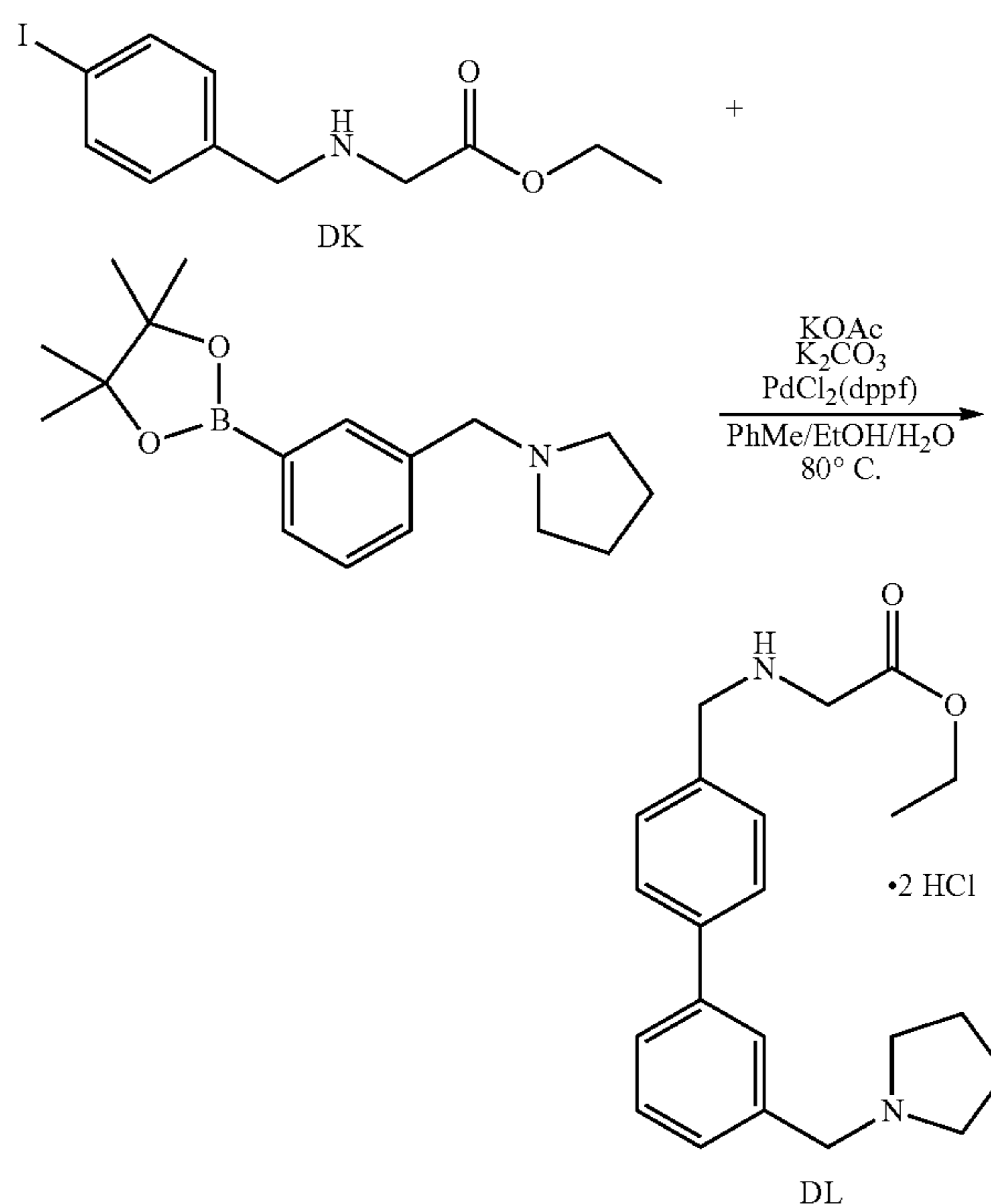
Scheme 78
