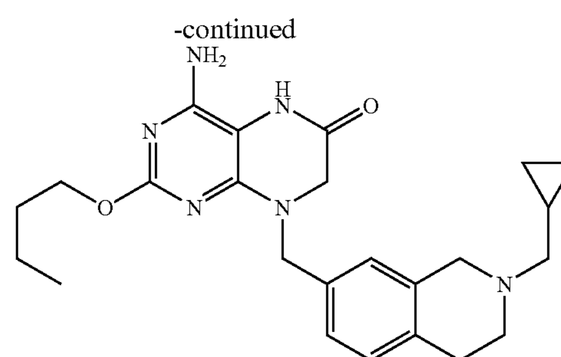
Example 70
