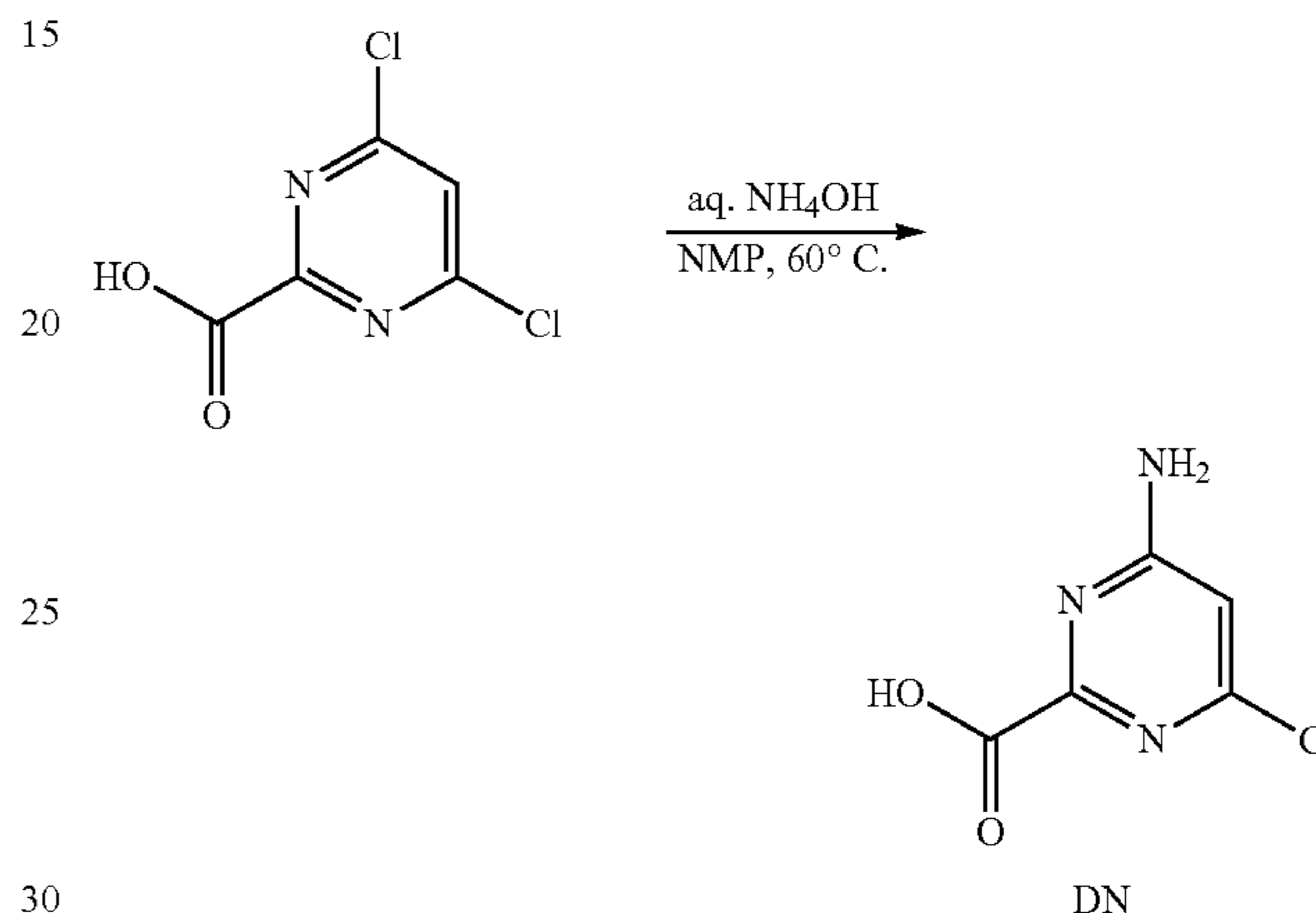
Scheme 80
