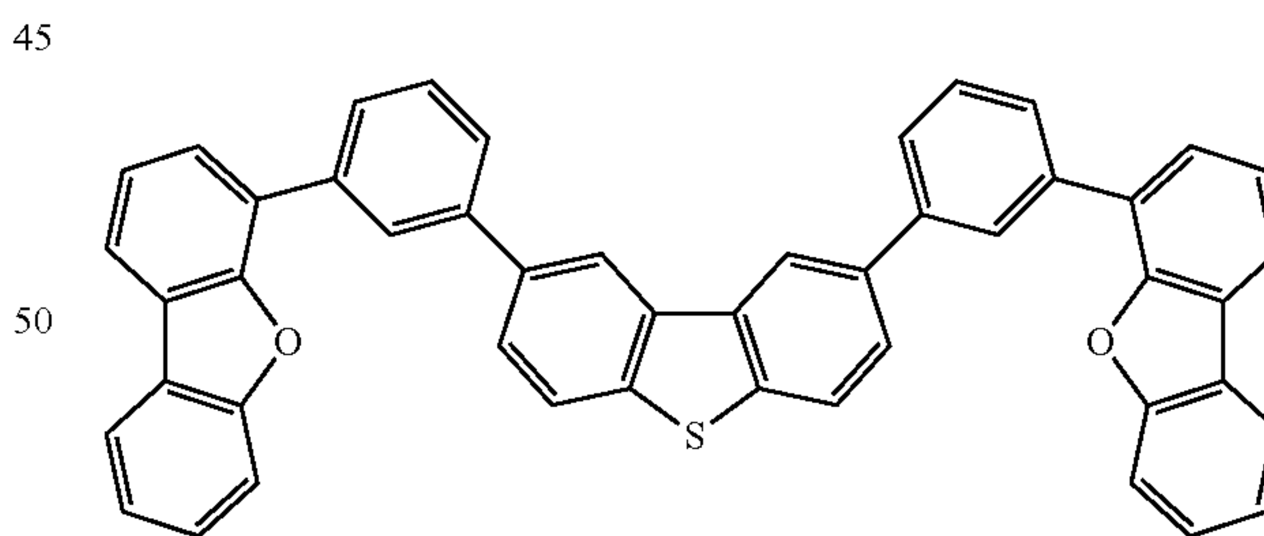
Comparative compound 2
