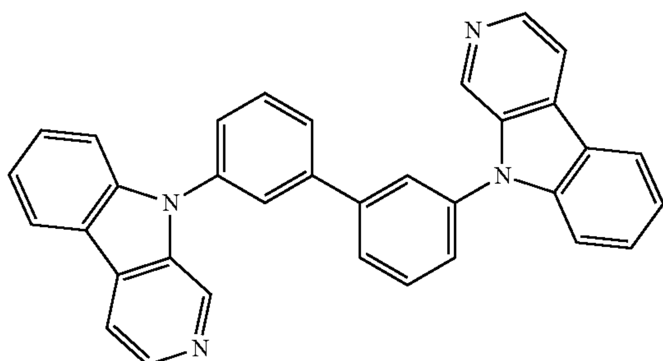
Comparative compound 6
