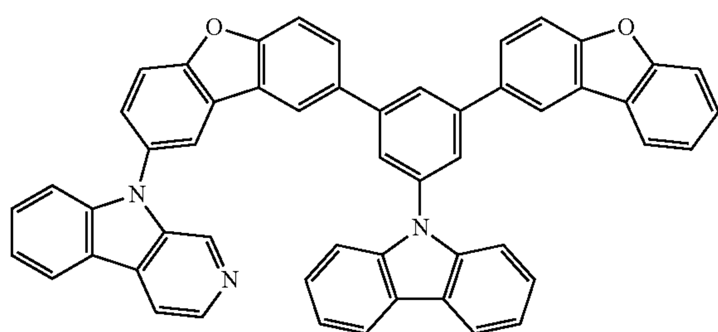
Comparative compound 7
