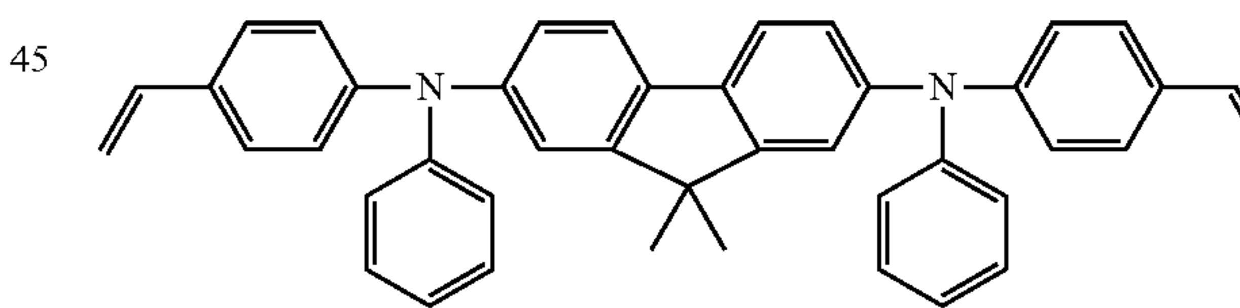
Positive hole transport compound 7
