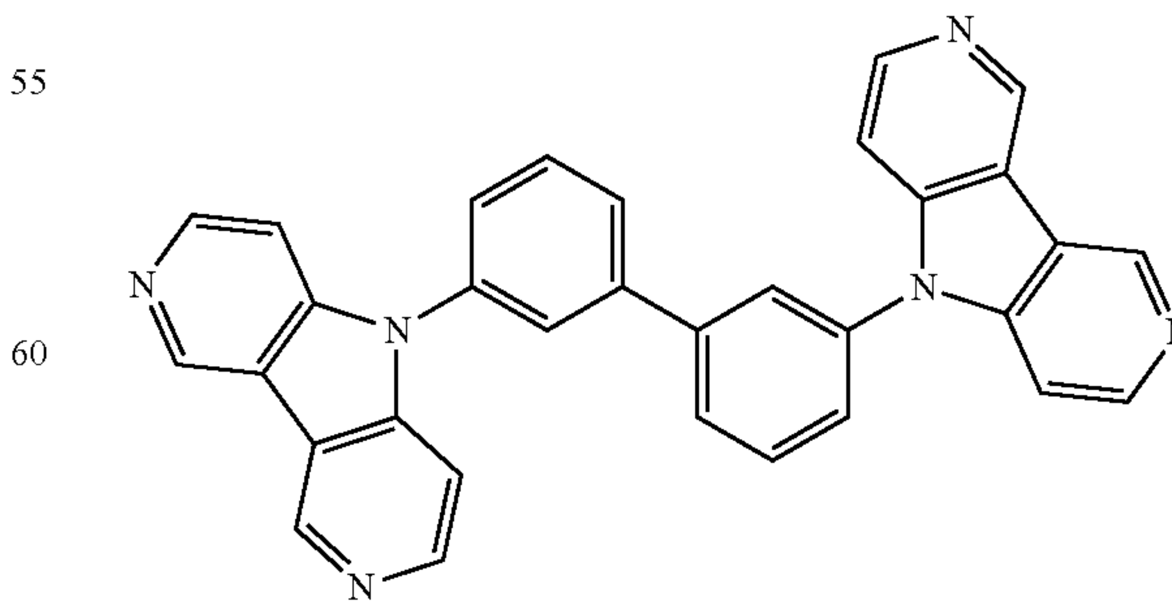
Electron transport compound 1
