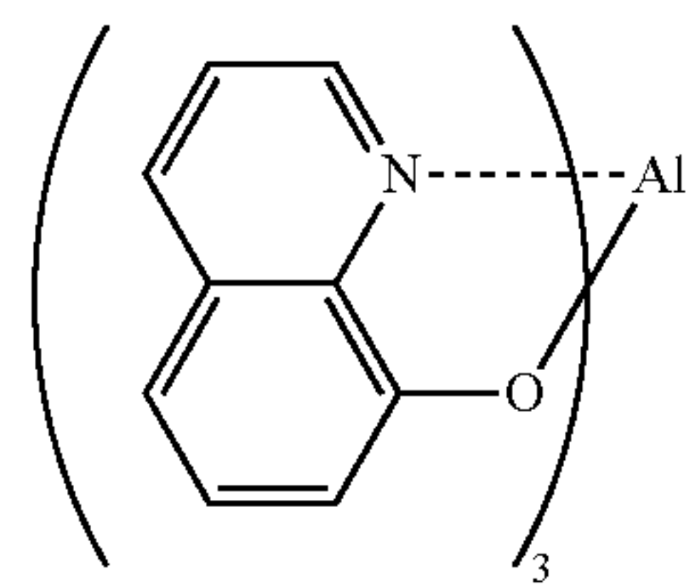
Electron transport compound 5
