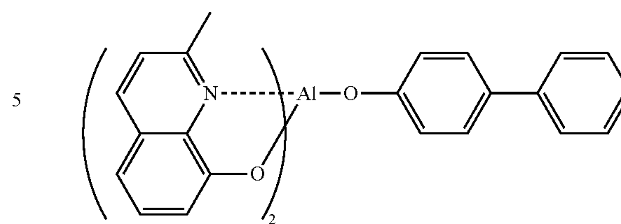
Electron transport compound 6
