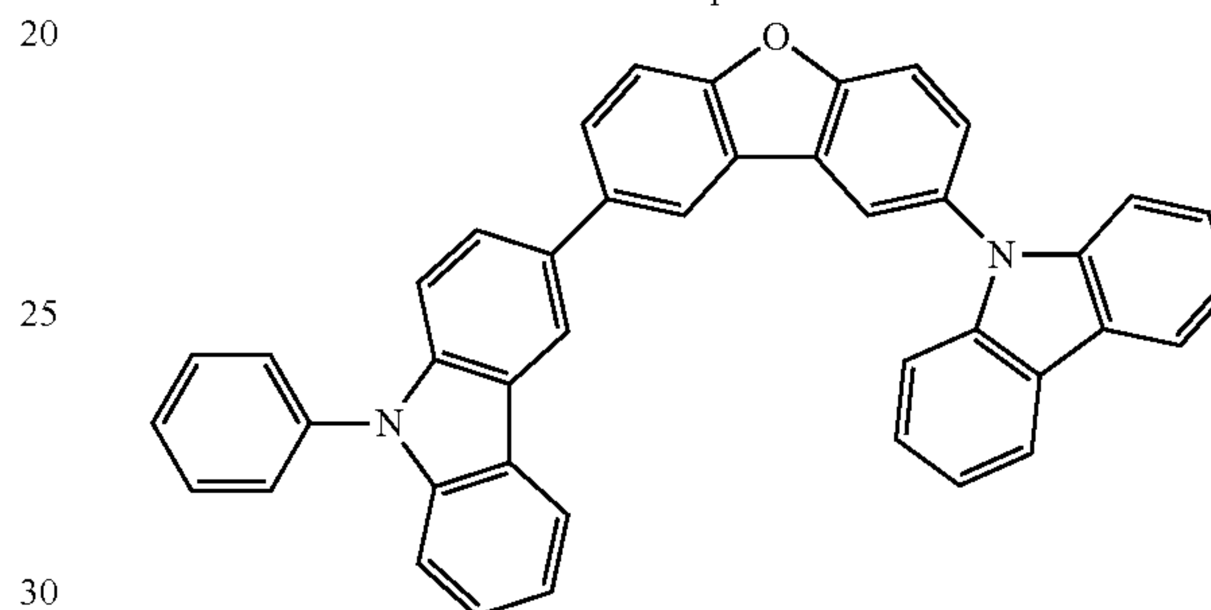
Host compound 2
