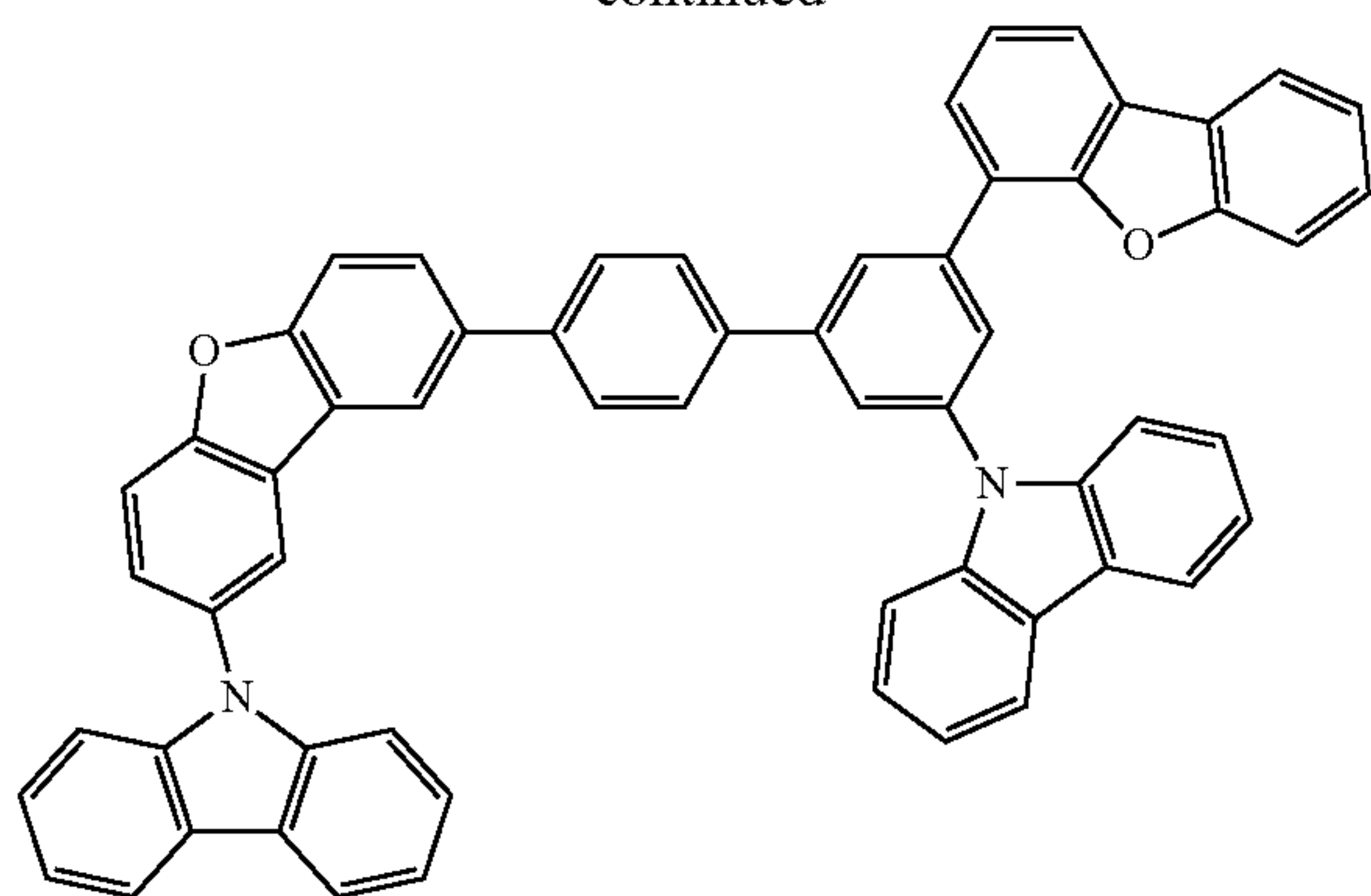
Comparative compound 4
