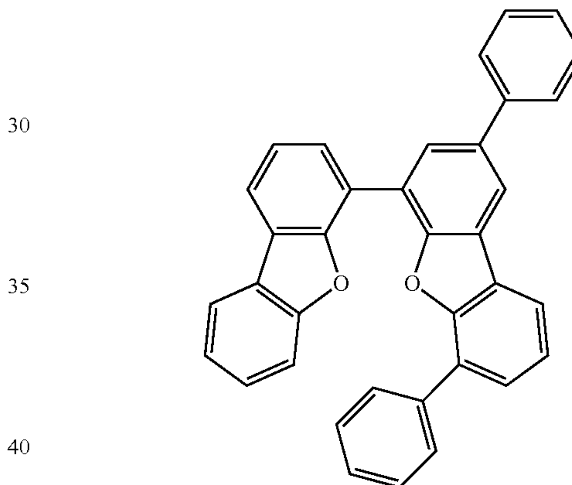
Comparative compound 1
