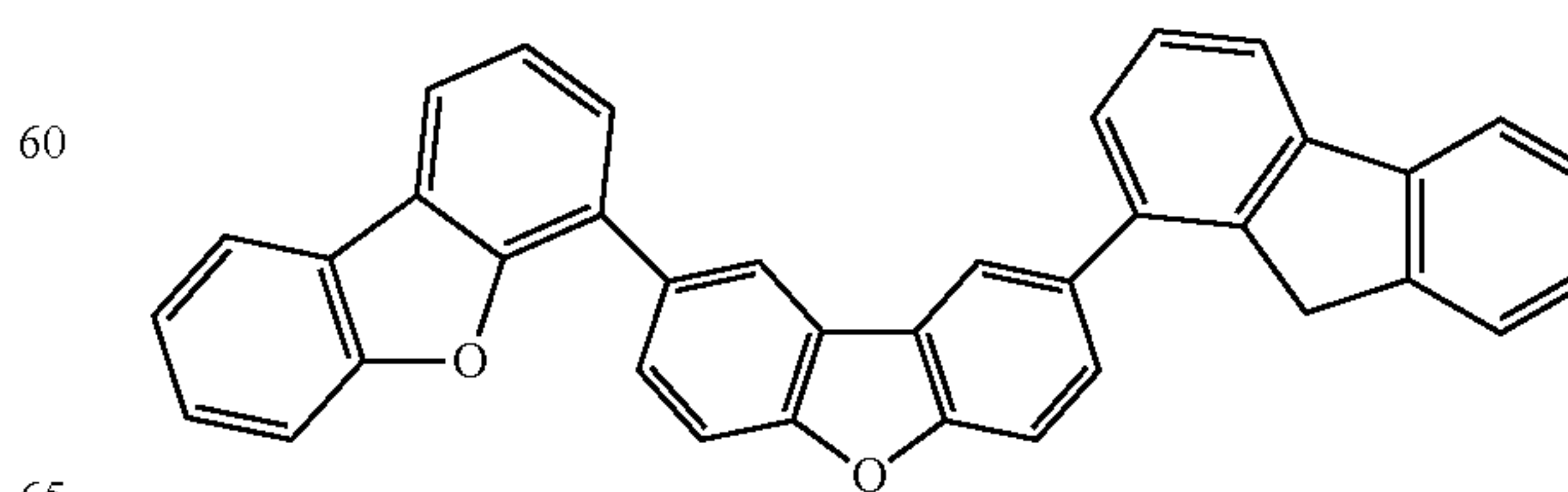
Comparative compound 3
