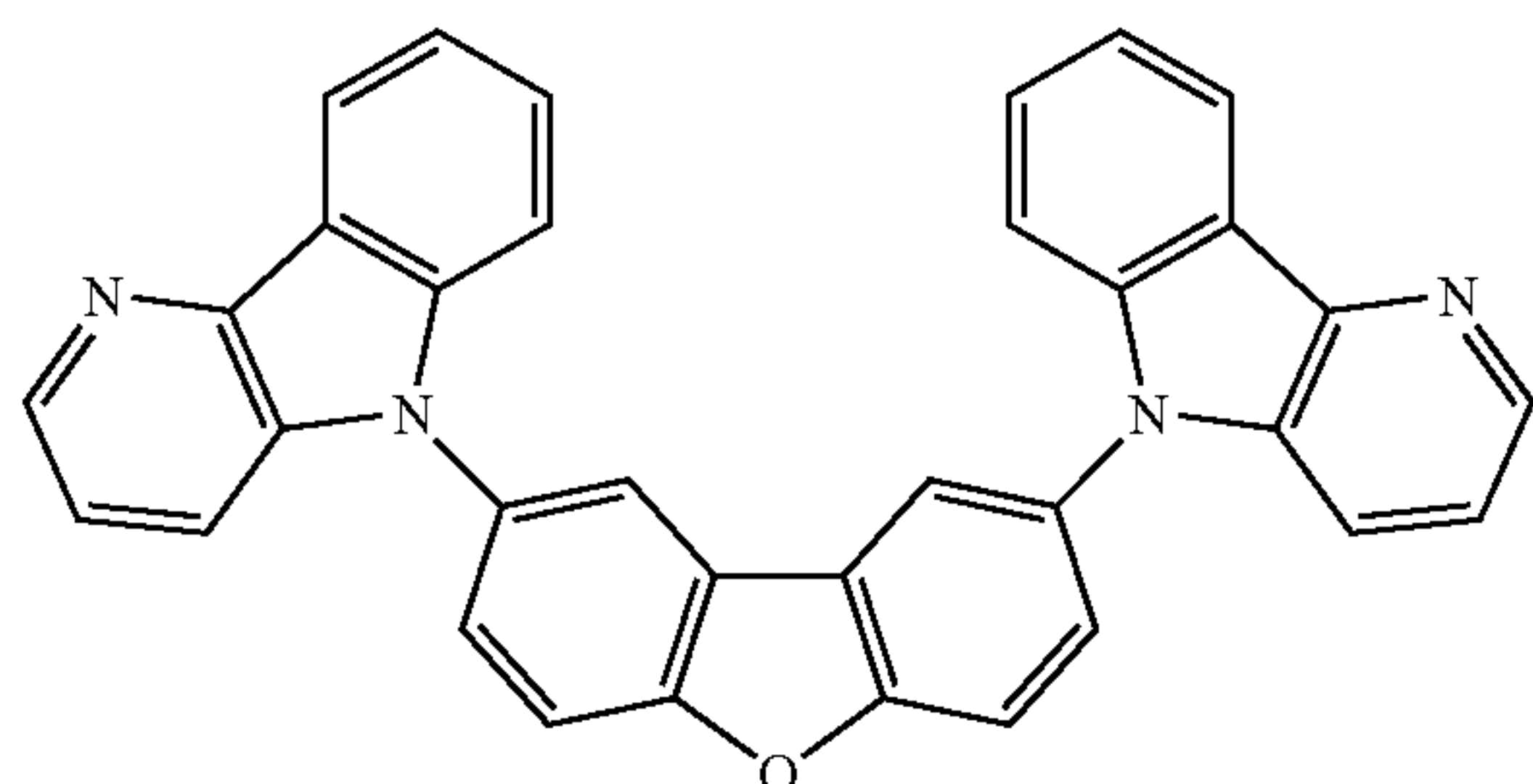
Comparative compound 8
