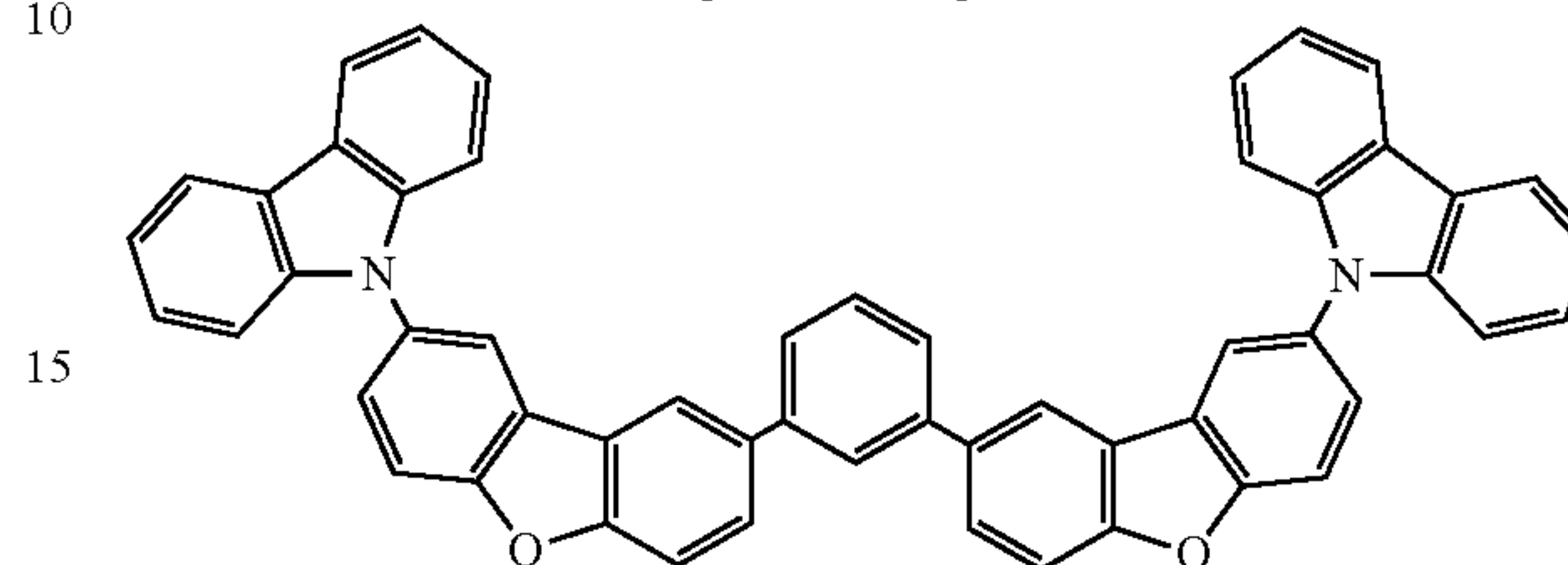
Host compound 1
