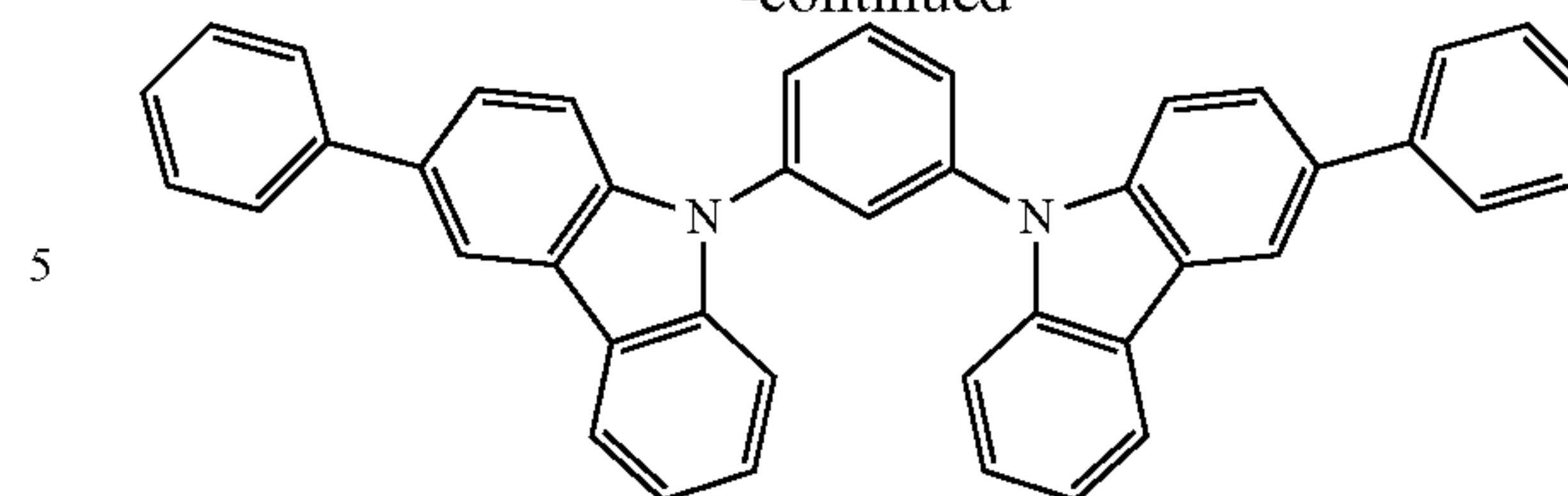
Comparative compound 9
