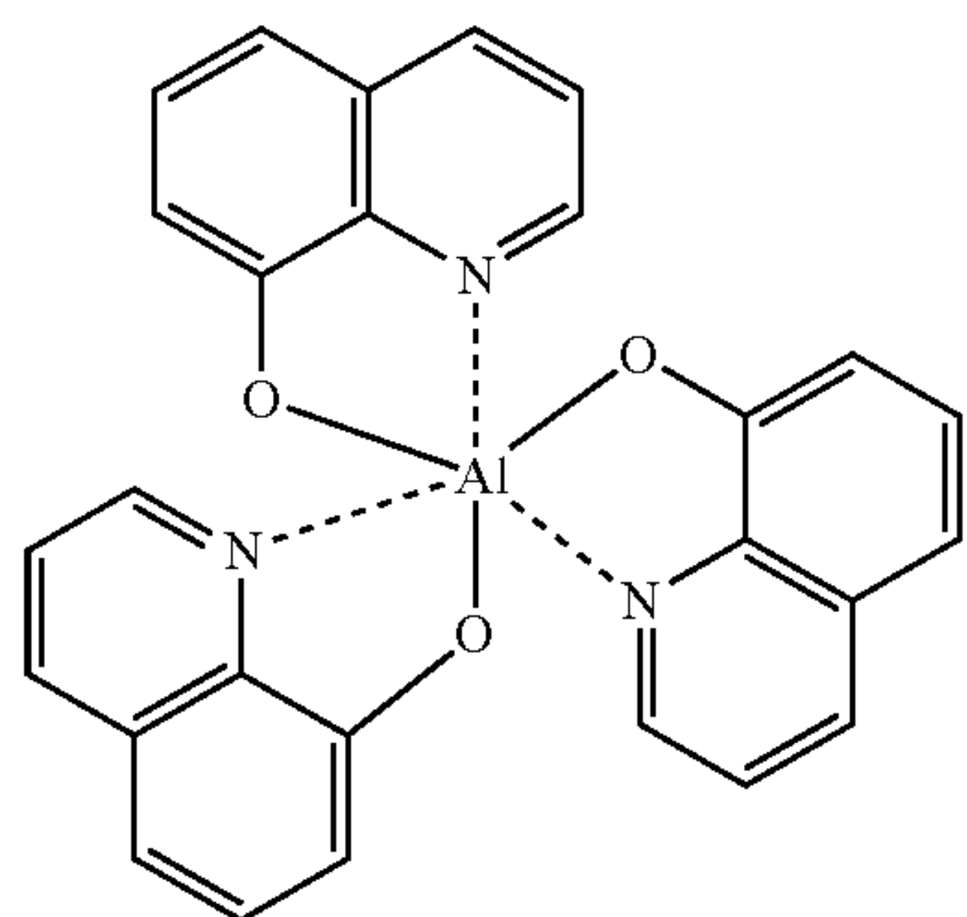
(Alq 3 )
