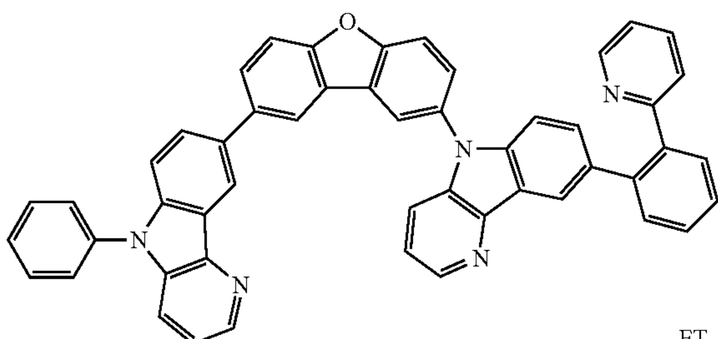
ET-10
