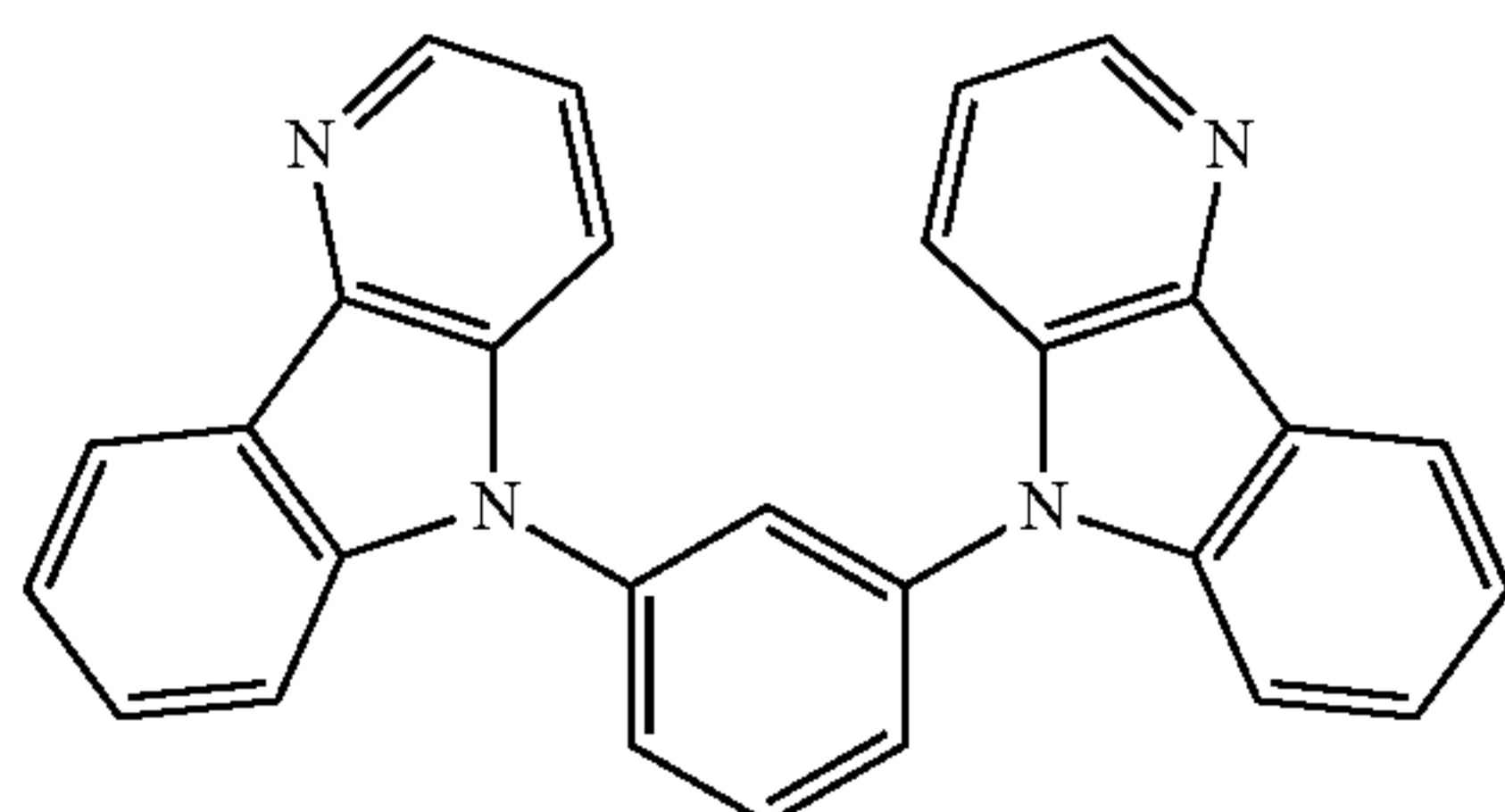
Comparative compound 5
