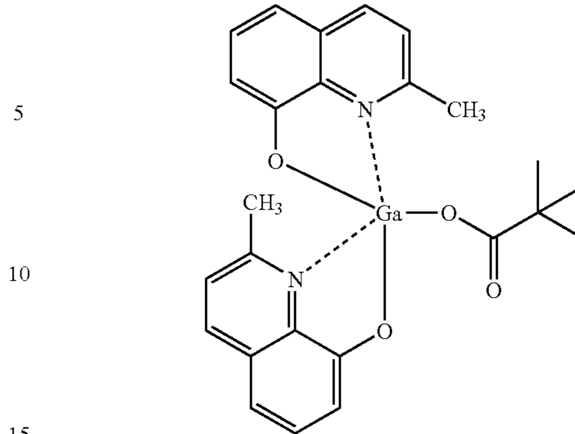
Gaq'2OPiv
