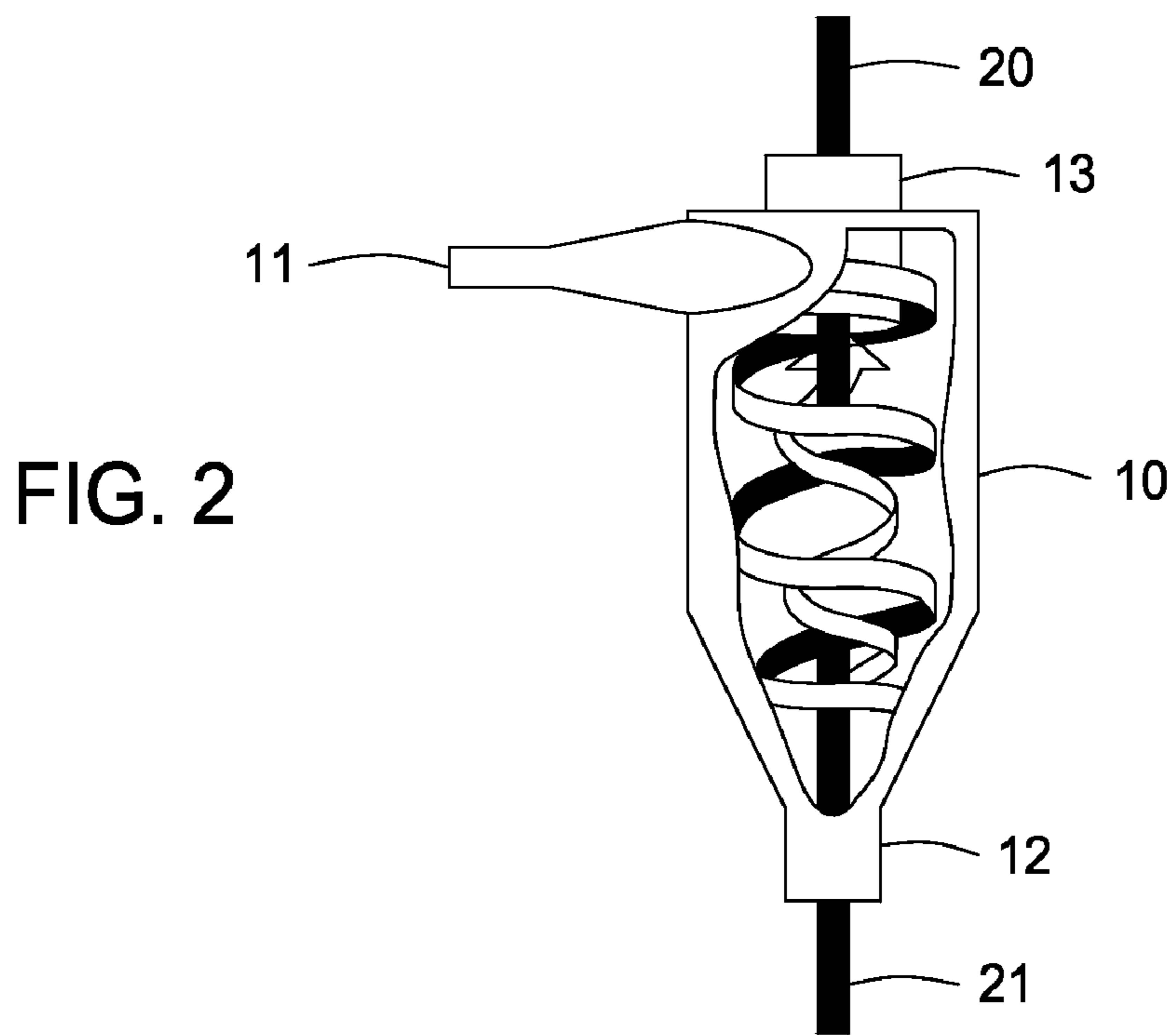
Carbon Arc in Cyclone separator
