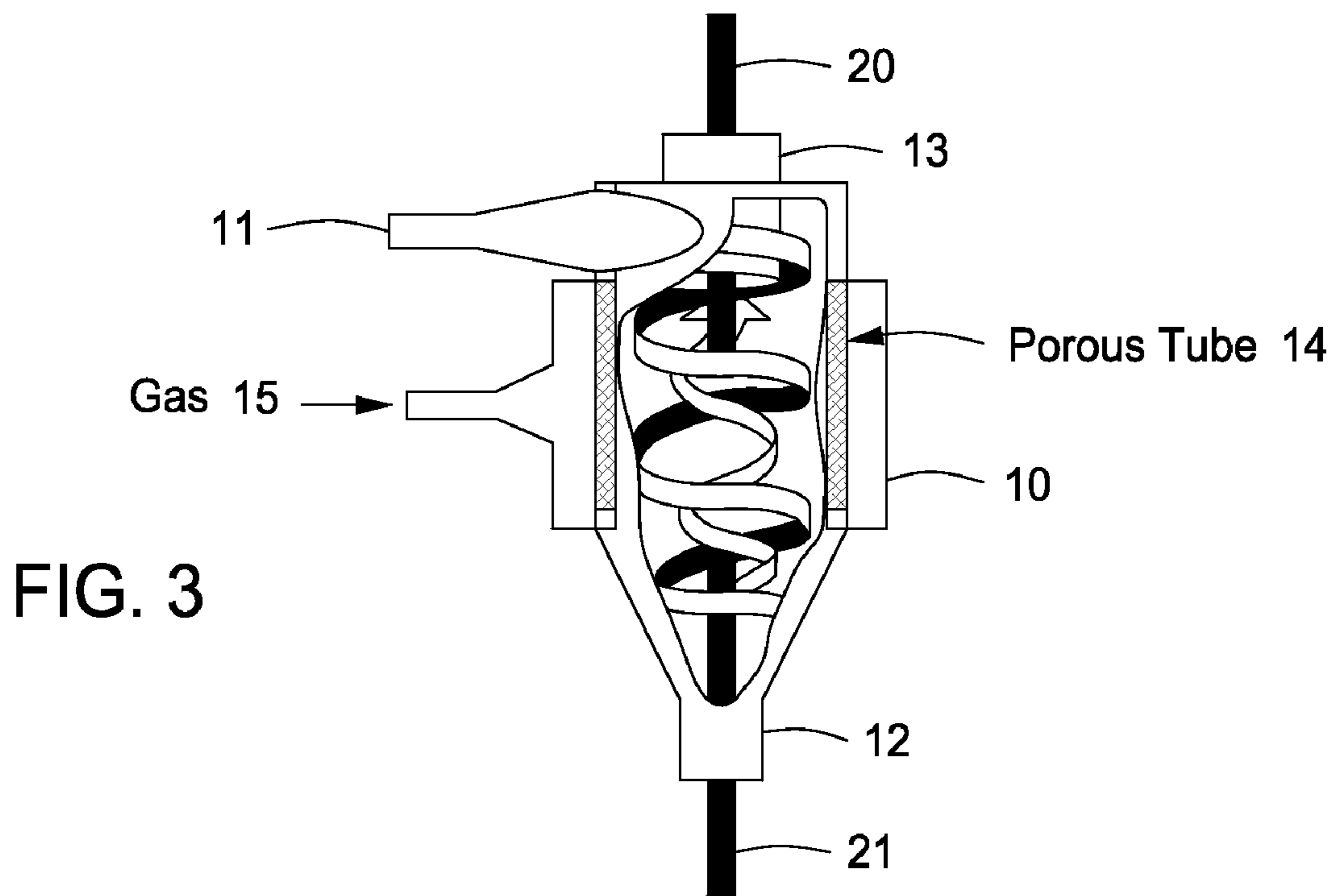
Carbon Arc in Gas-Sparged Hydrocyclone
