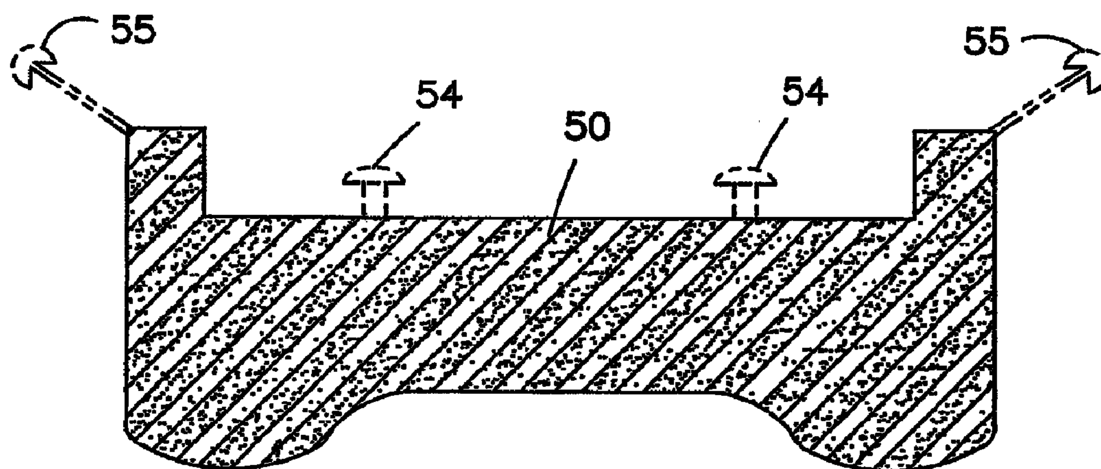
FIG. 2 PRIOR ART
