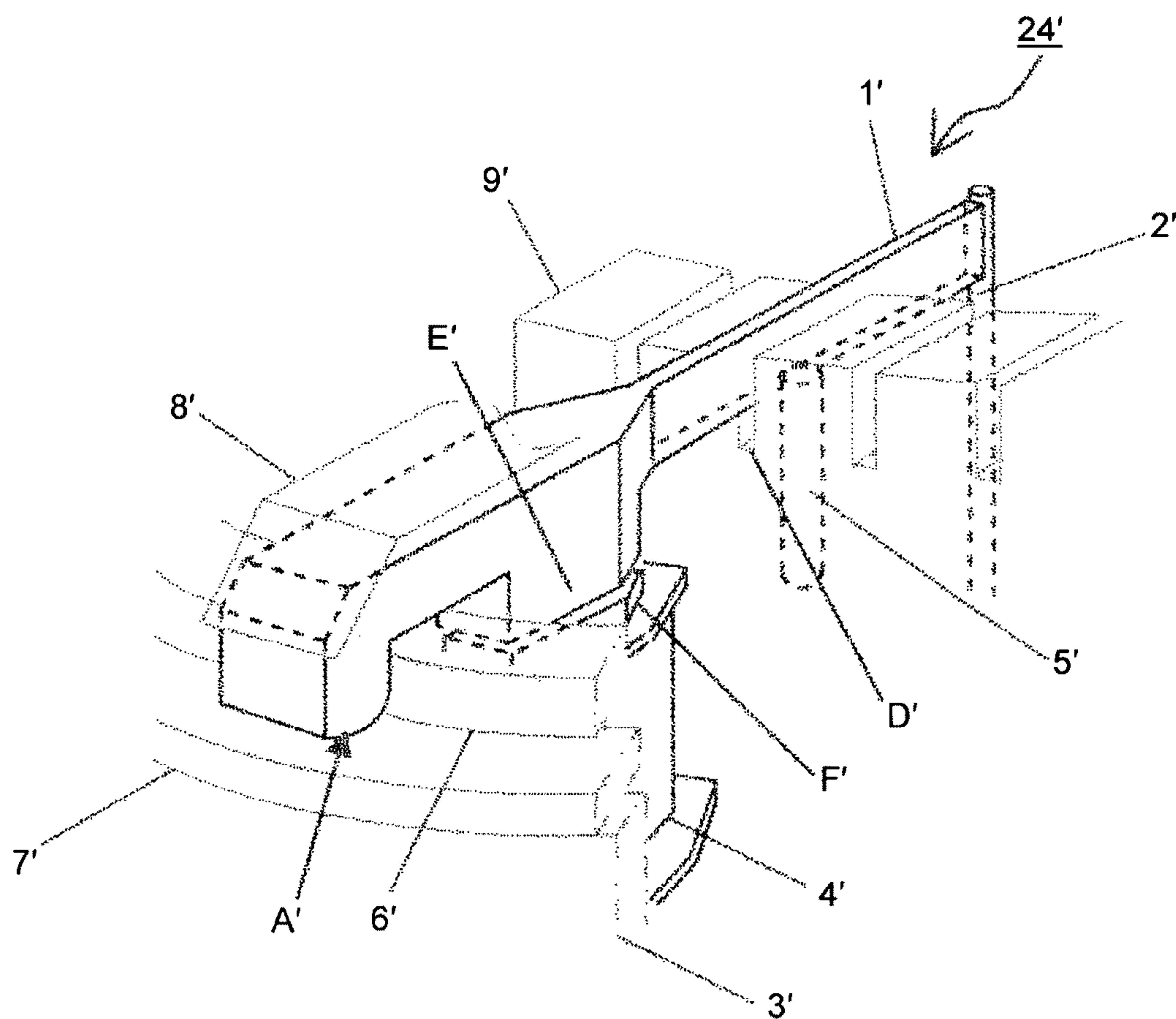
FIG. 13 CONVENTIONAL ART
