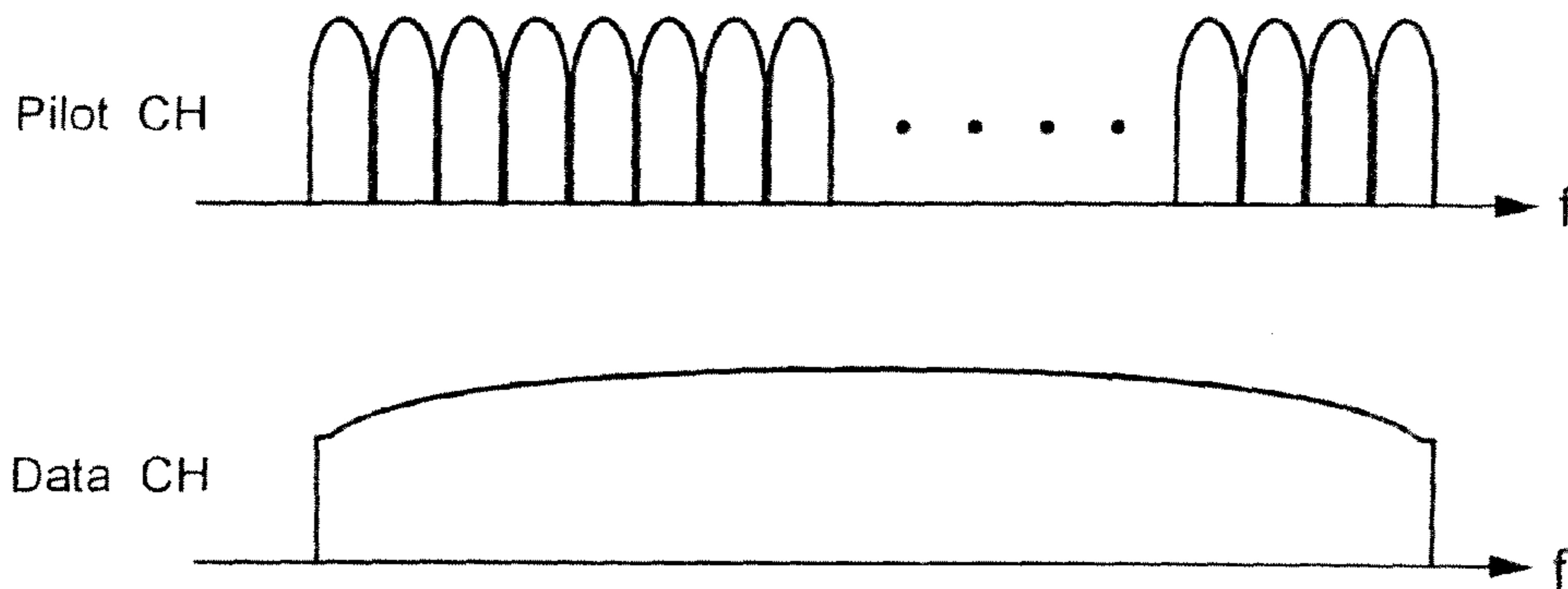
MULTIPLEXING OF Pilot CH AND Data CH ( WHERE FDM pilot AND SRF ( Symbol Repetition Factor = 4 ) )
