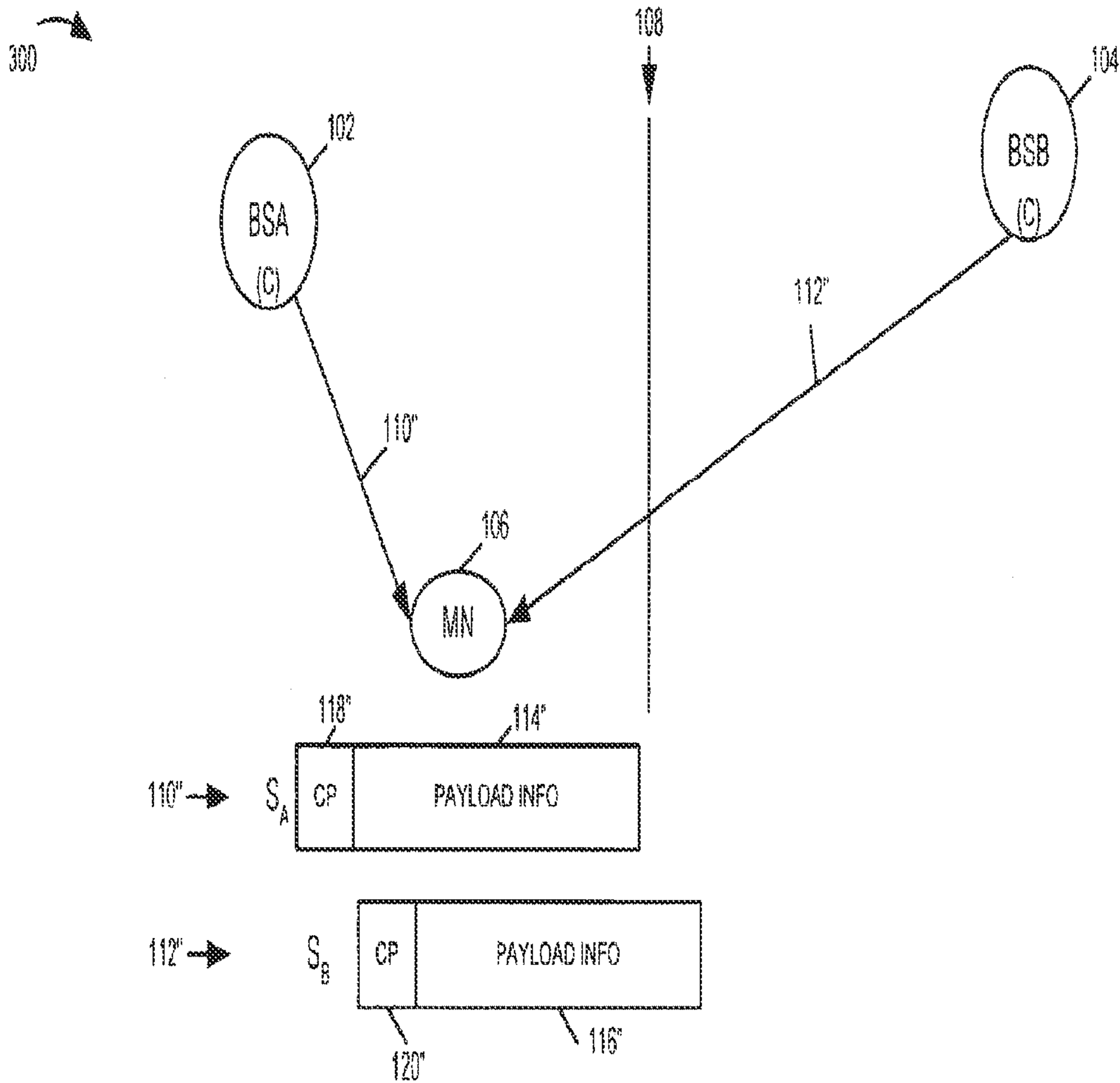
FIGURE 3 PRIOR ART
