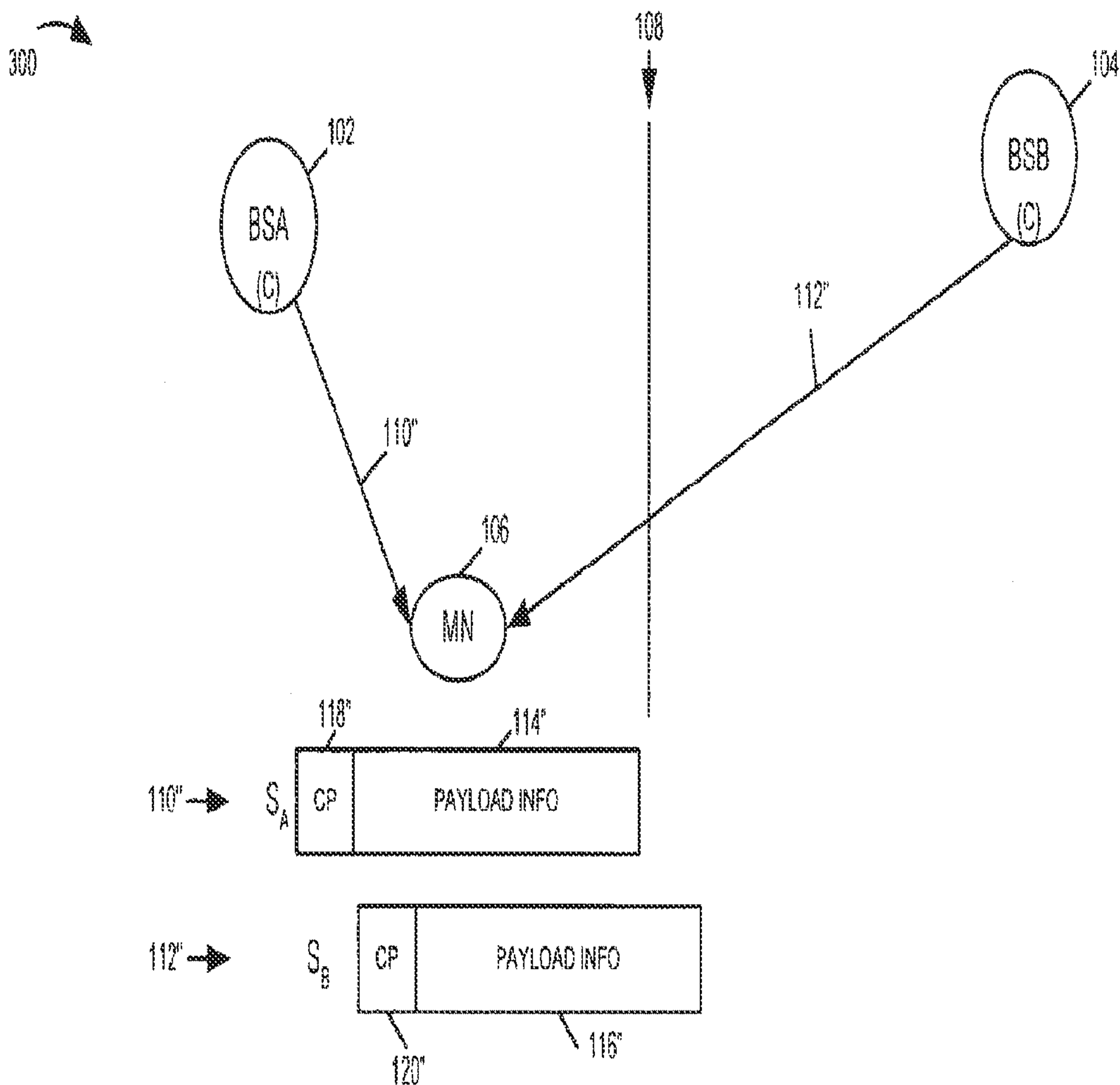
FIGURE 3 PRIOR ART
