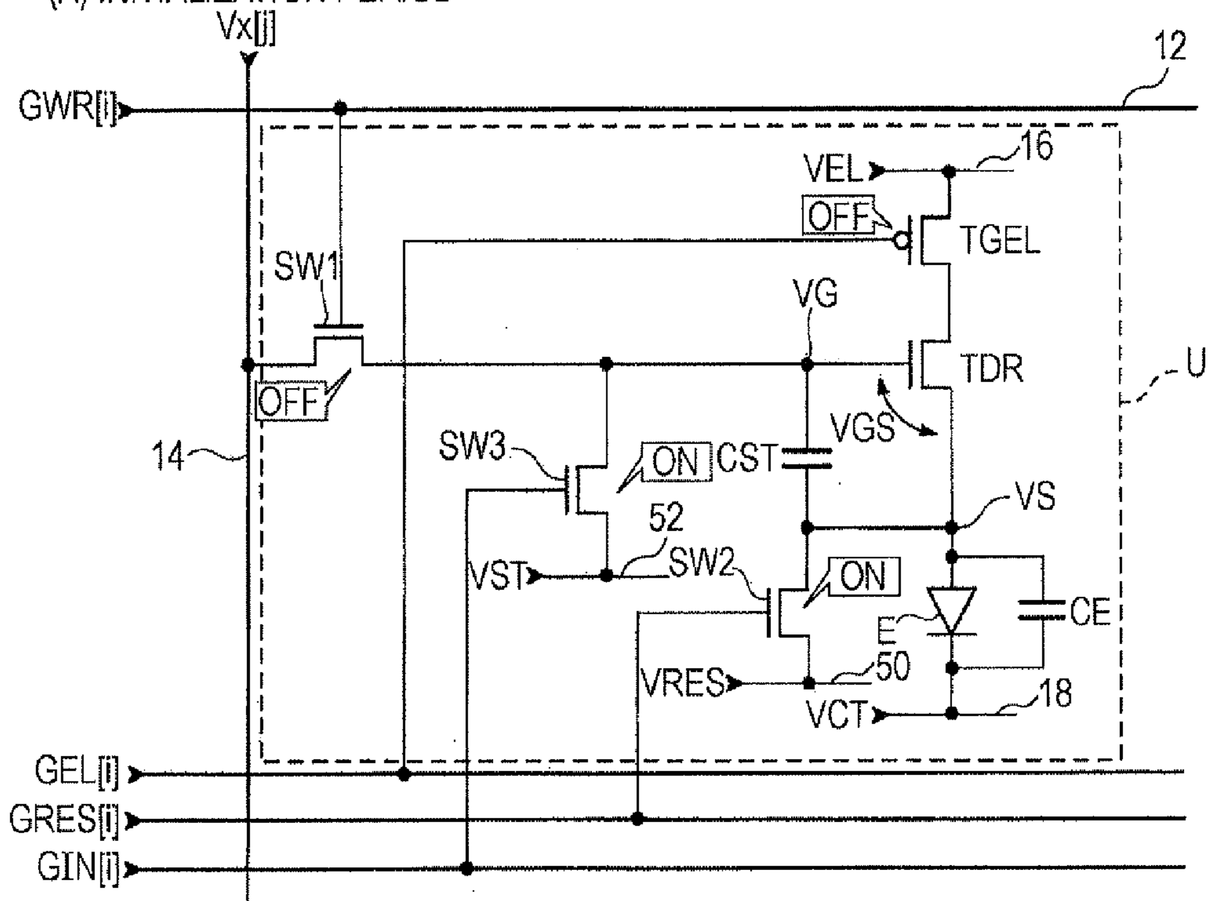
FIG. 6 (A) INITIALIZATION PERIOD
