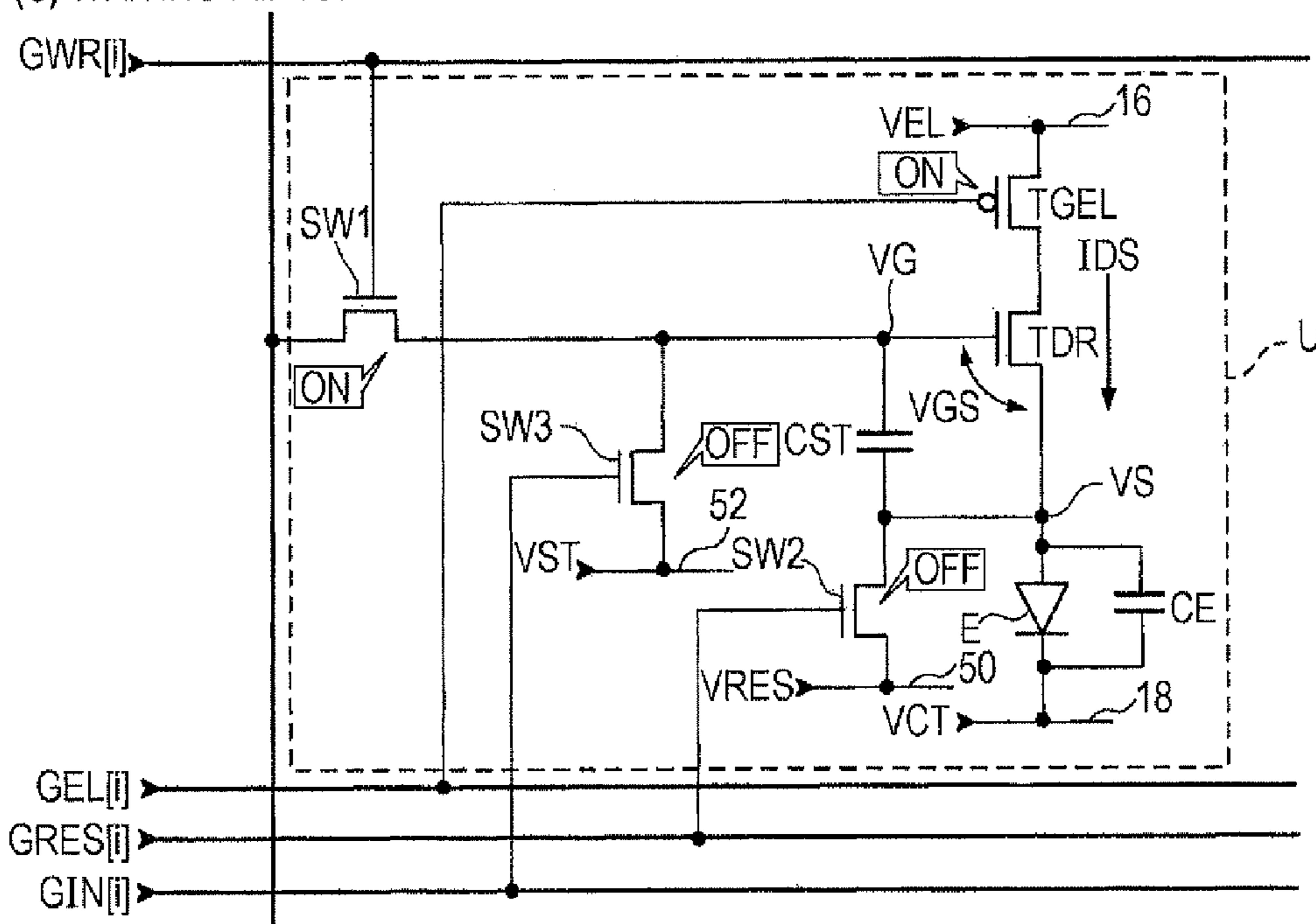
FIG. 8 (C) WRITING PERIOD
