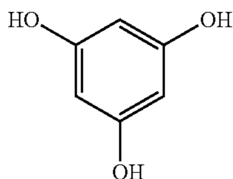
1,3,5-Trihydroxyl-benzene
