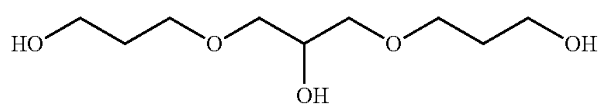
1,3-Di(hydroxypropoxy)-2-hydroxyl-propane
