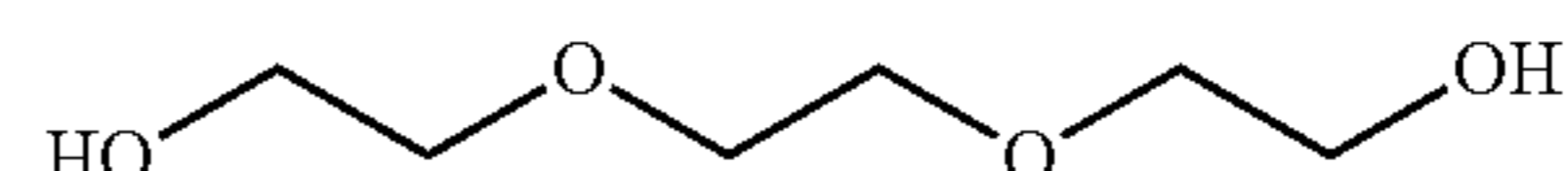
Triethylene glycol
