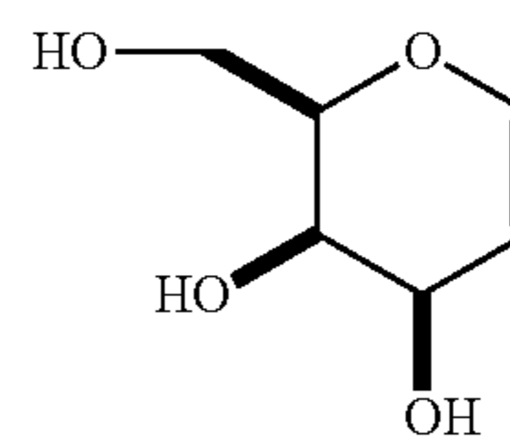
D-Galactool
