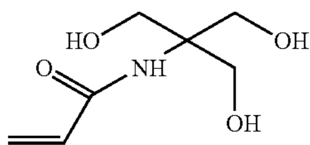
N-[Tris(hydroxymethyl)methyl]acrylamide
