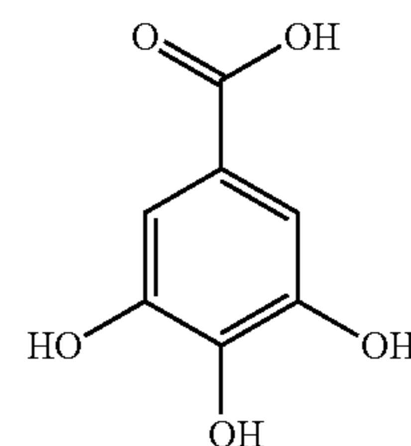
Gallic acid
