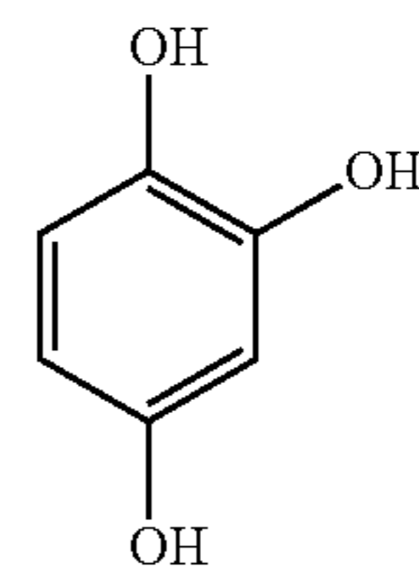
1,2,4-Trihydroxyl-benzene
