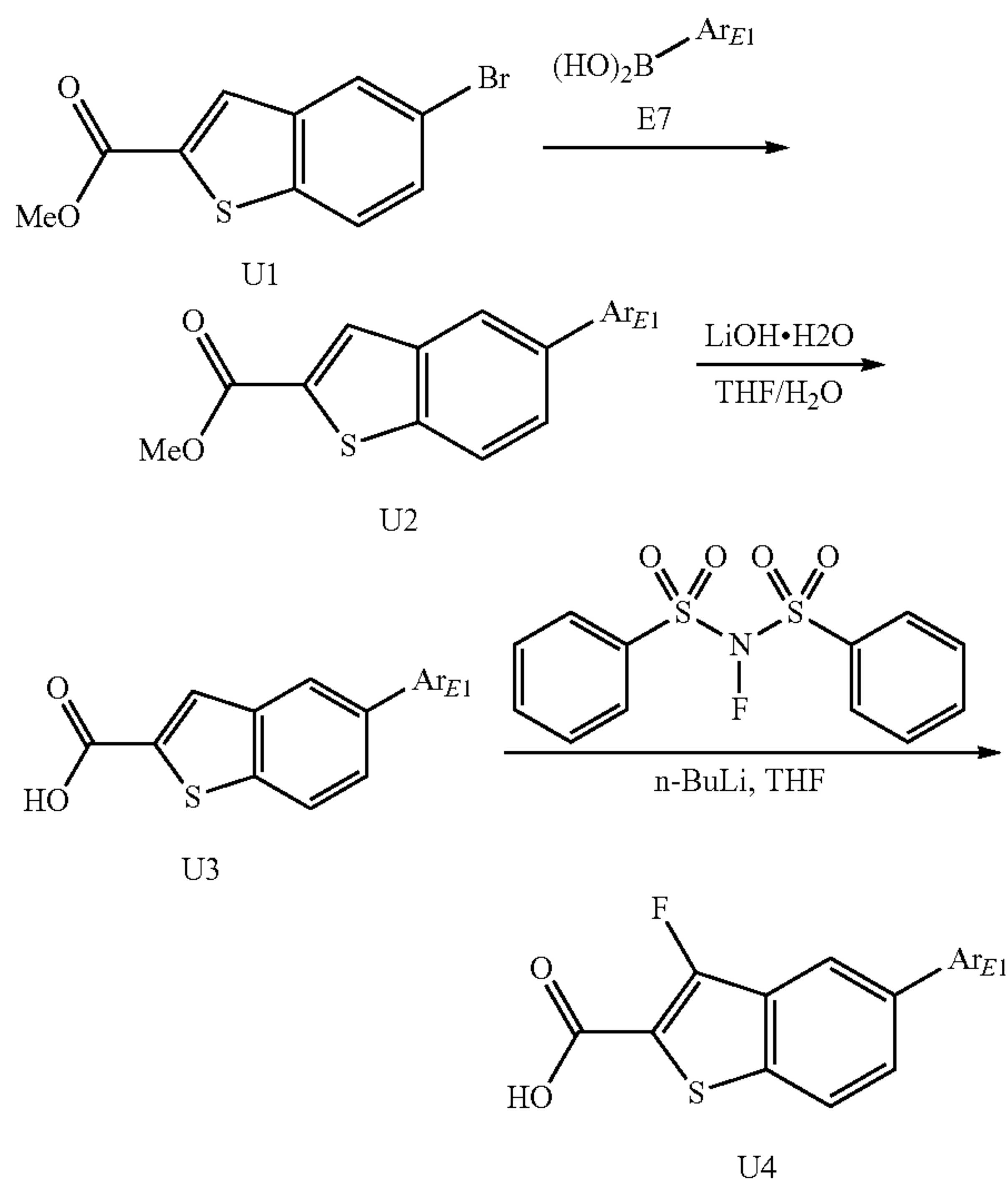
Scheme U
