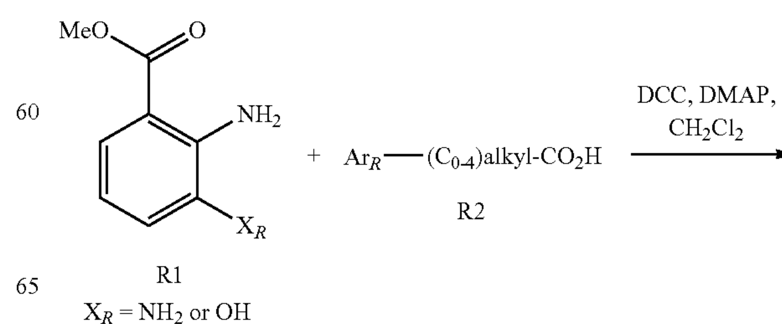
Scheme R
