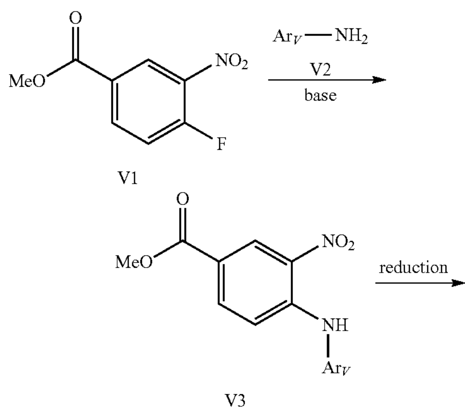
Scheme V
