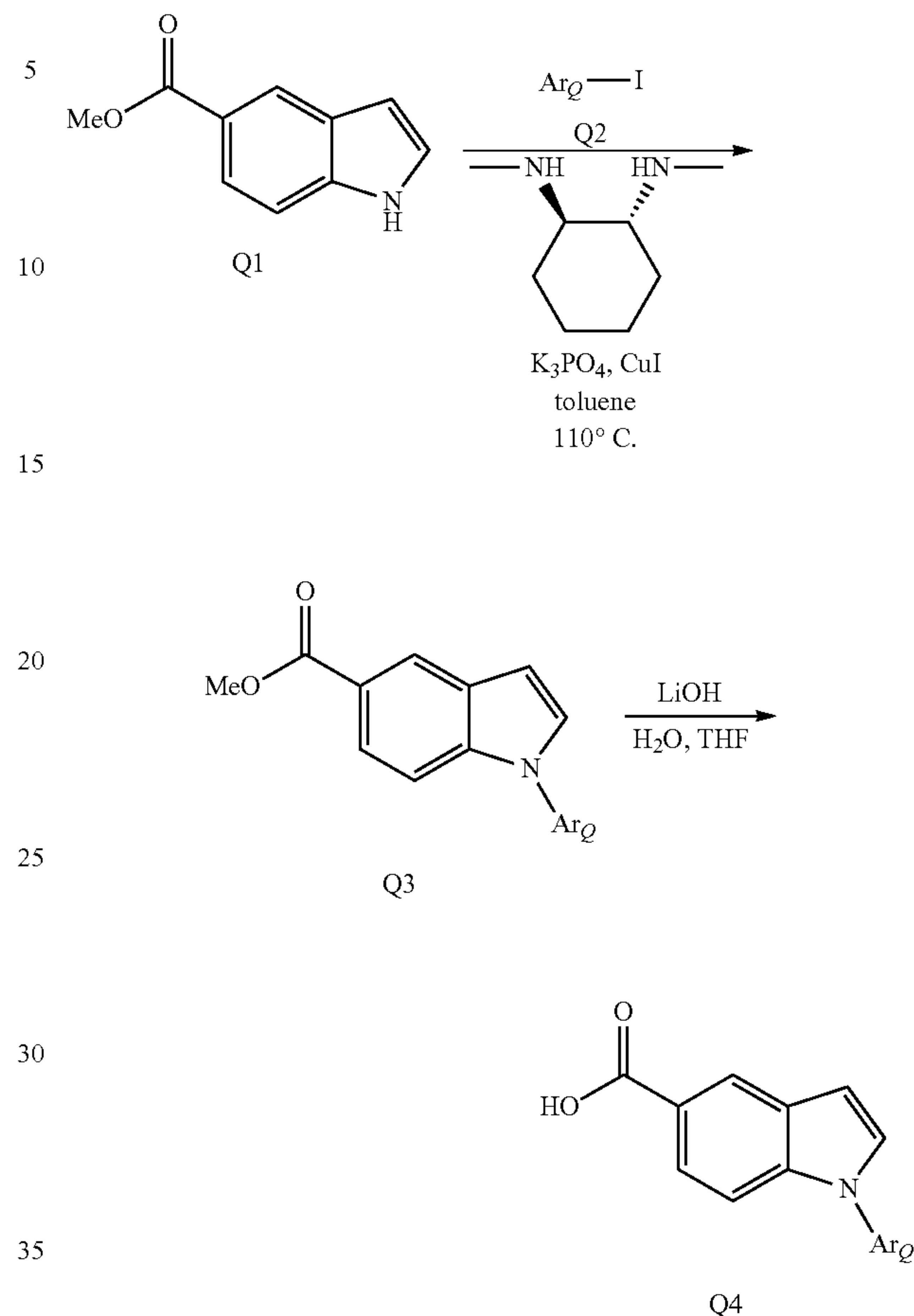
Scheme Q
