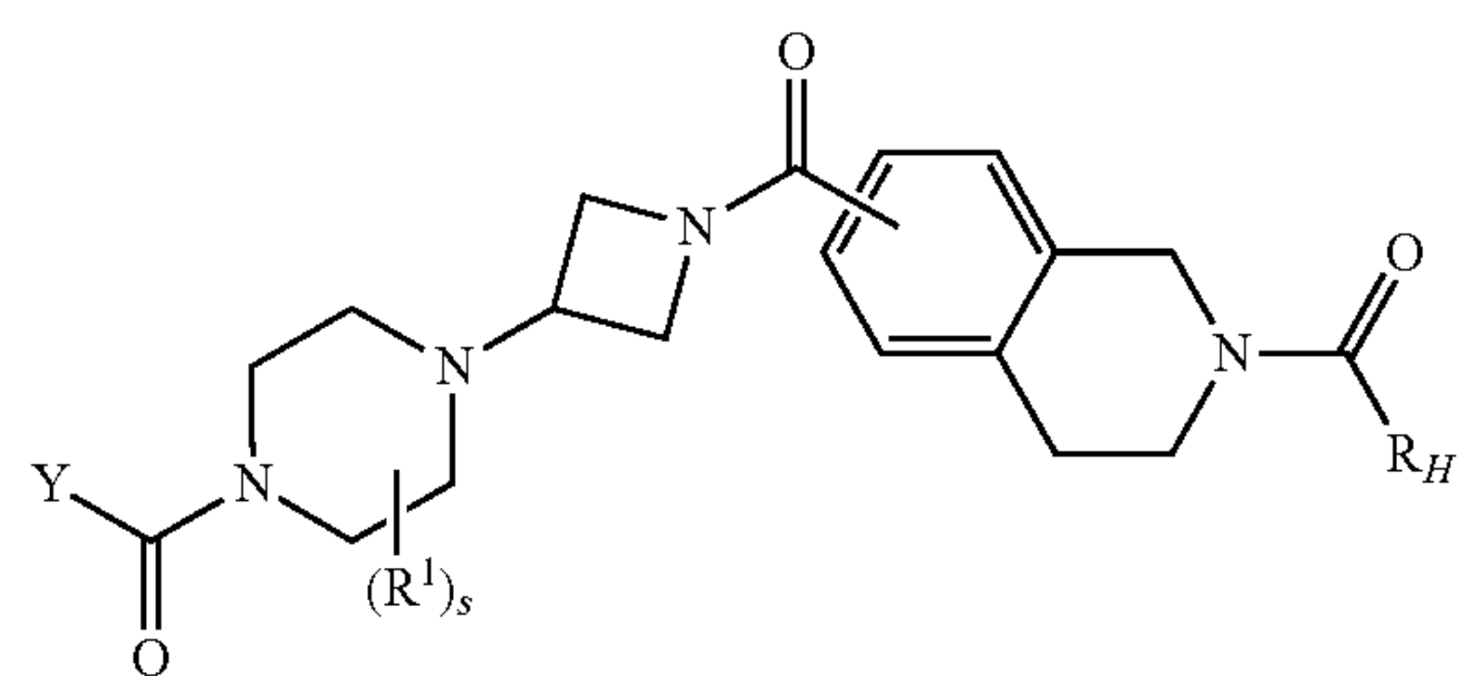
Formula (I)-H3
