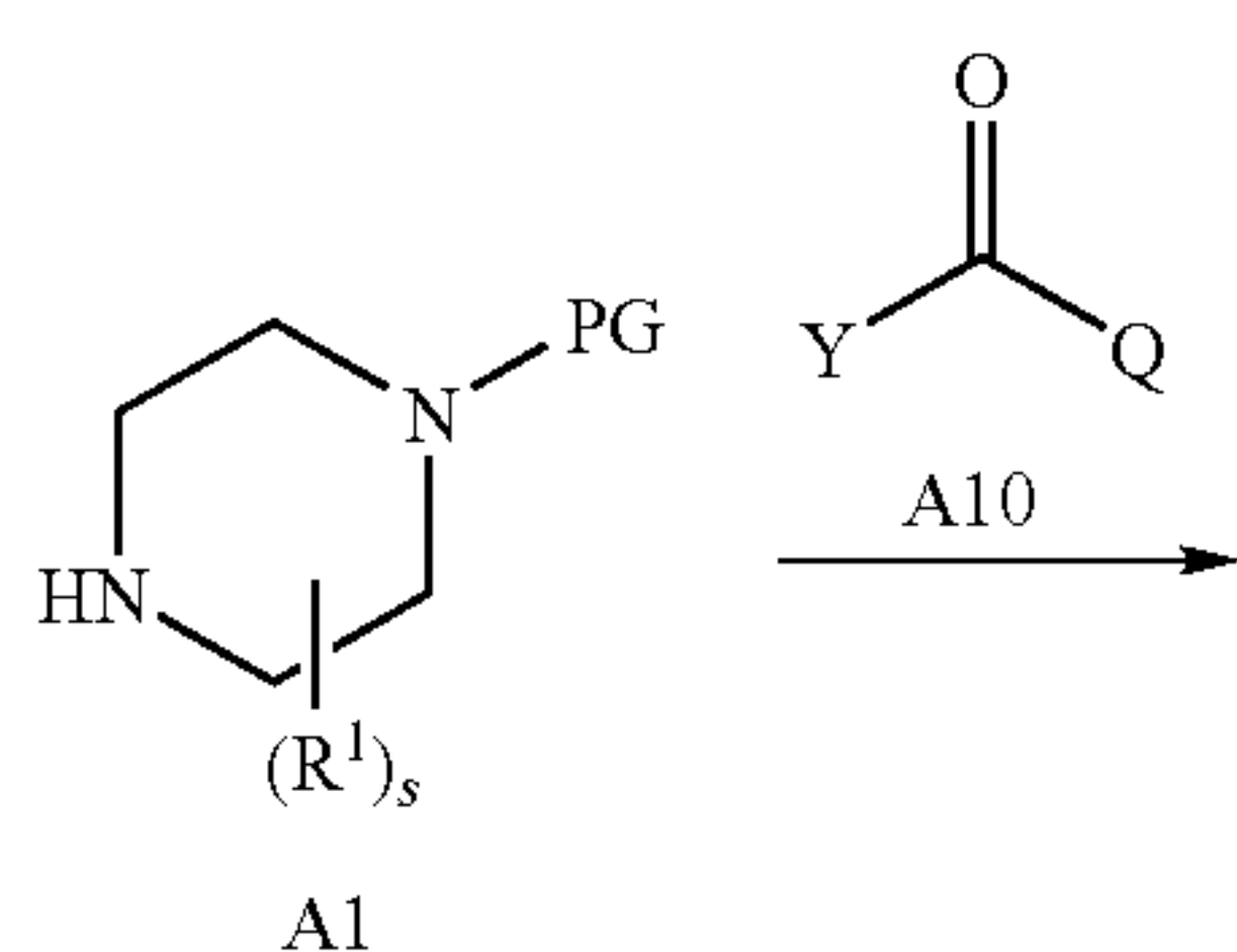
Scheme B
