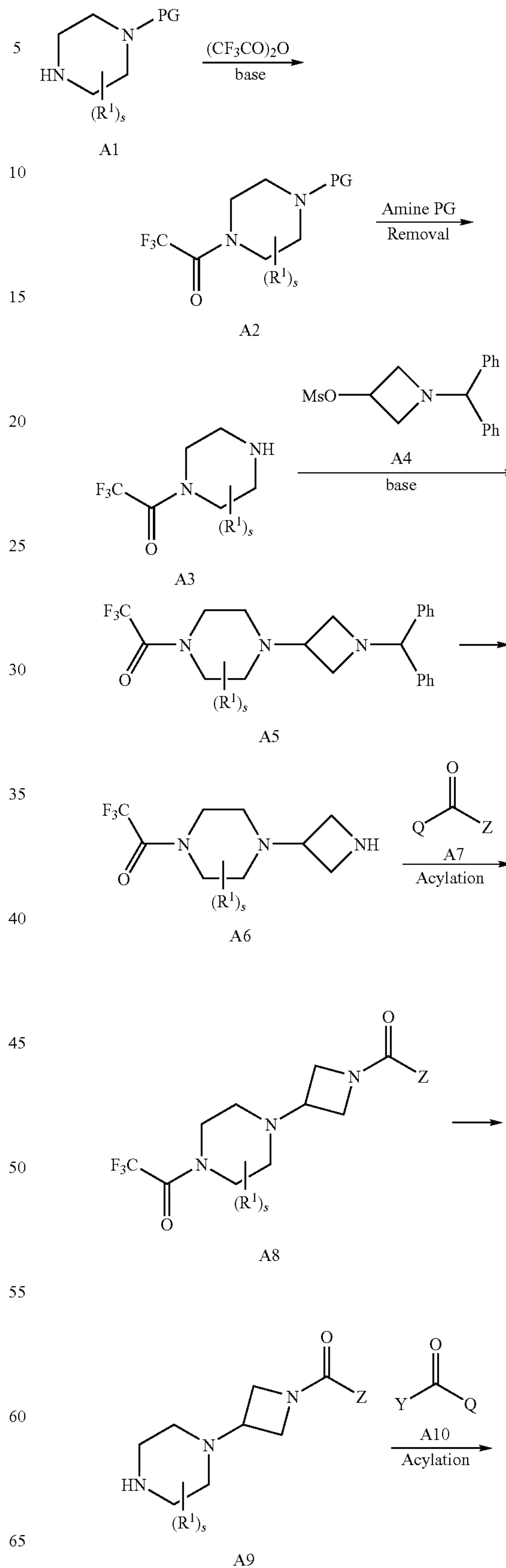
Scheme A
