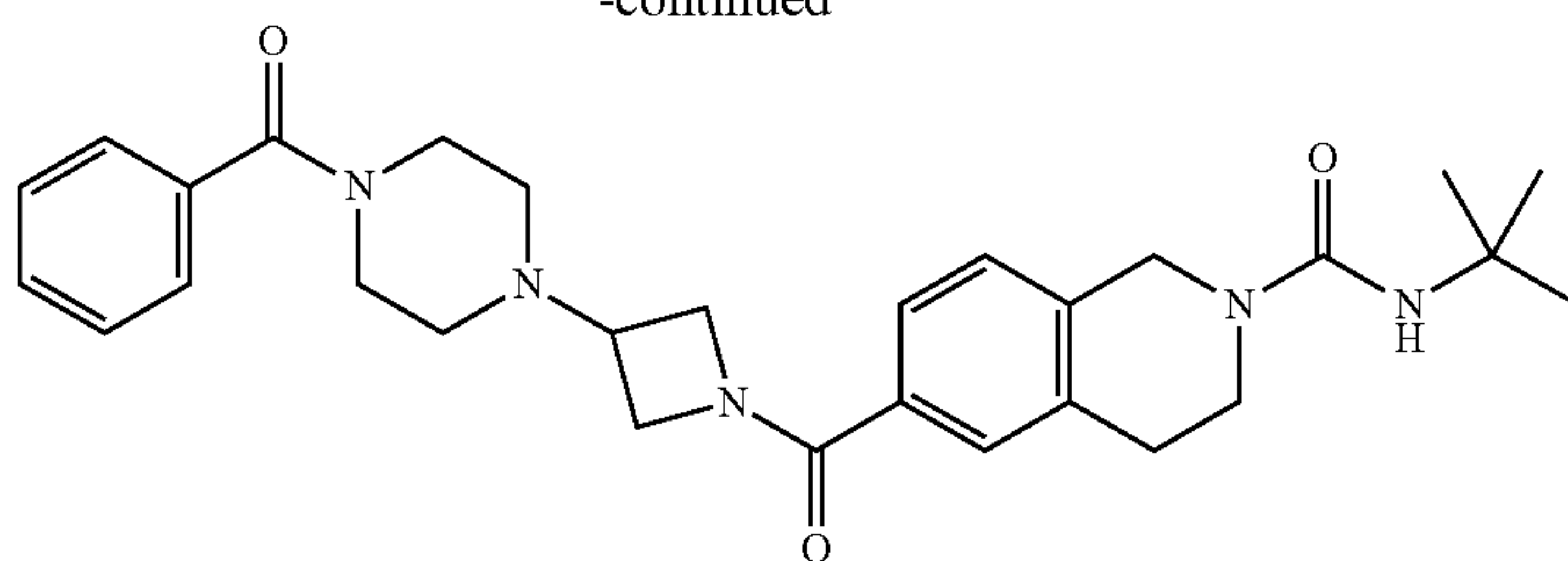
Cpd 356
