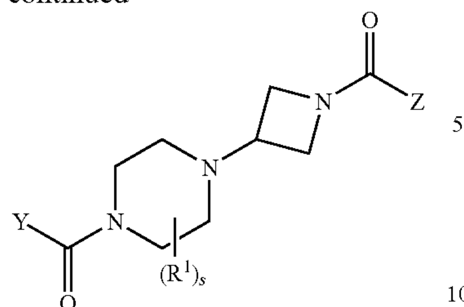
Formula (I)-A
