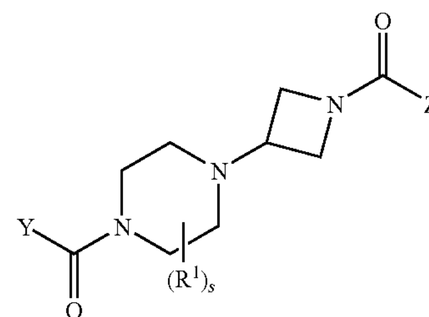
Formula (I)-A
