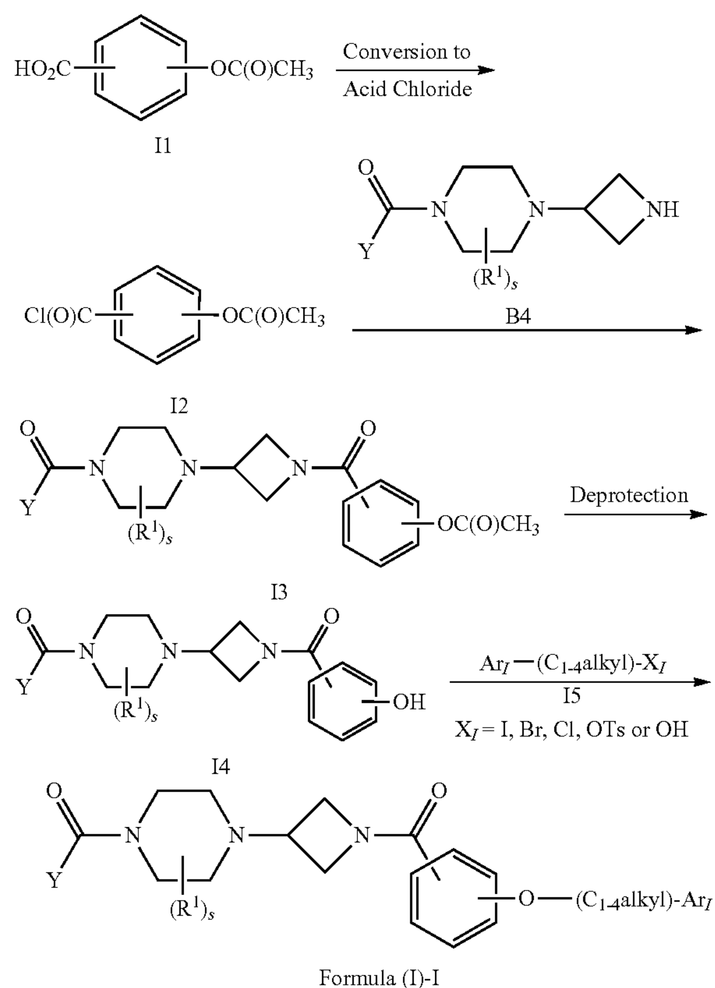
Scheme I
