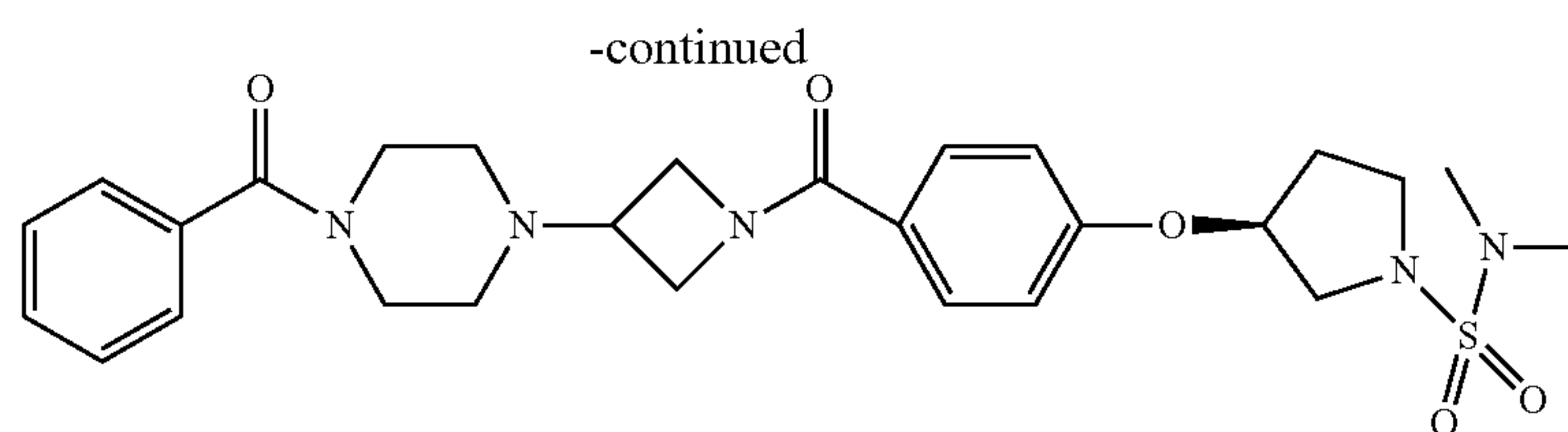
Cpd 439
