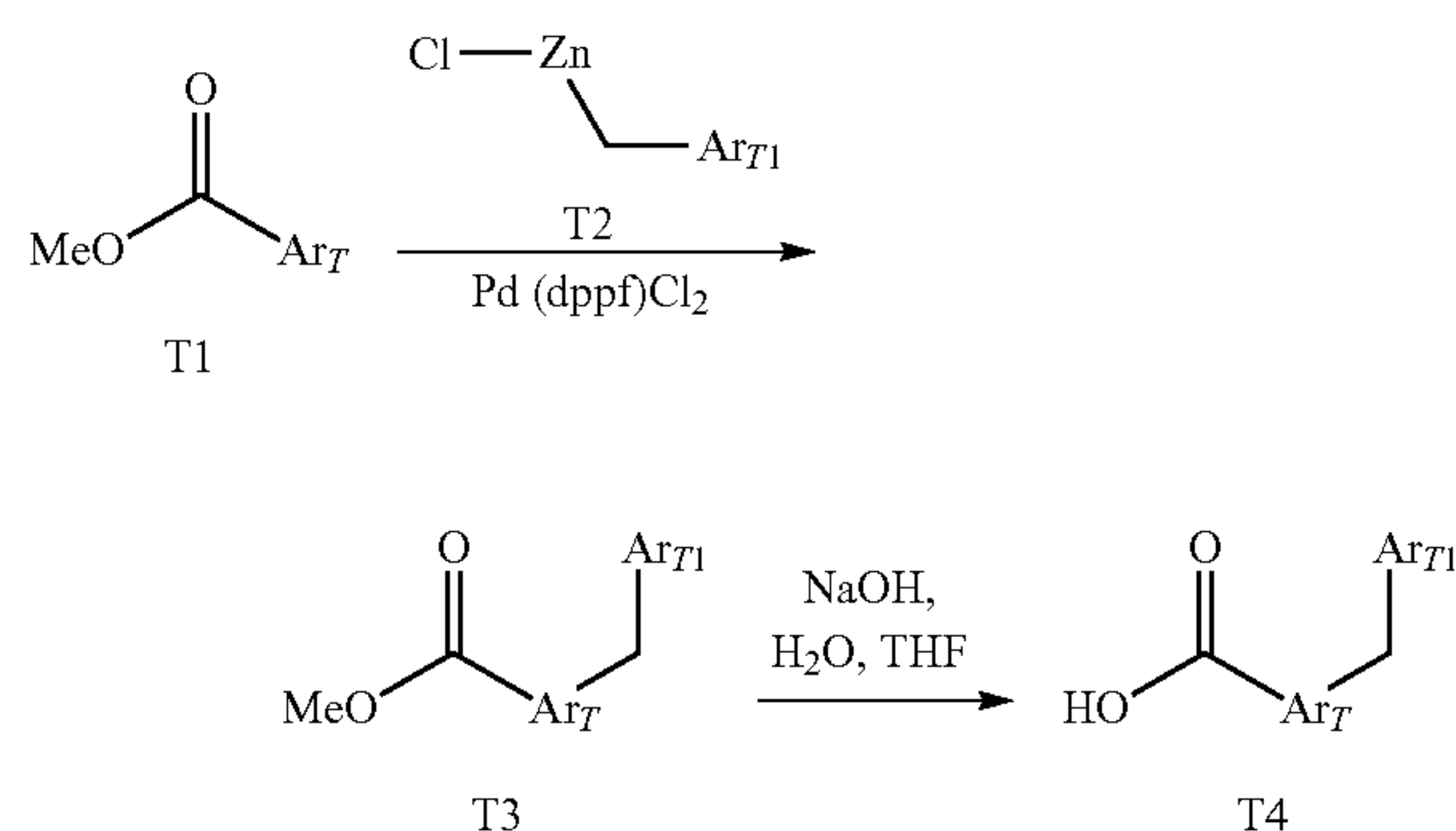
Scheme T
