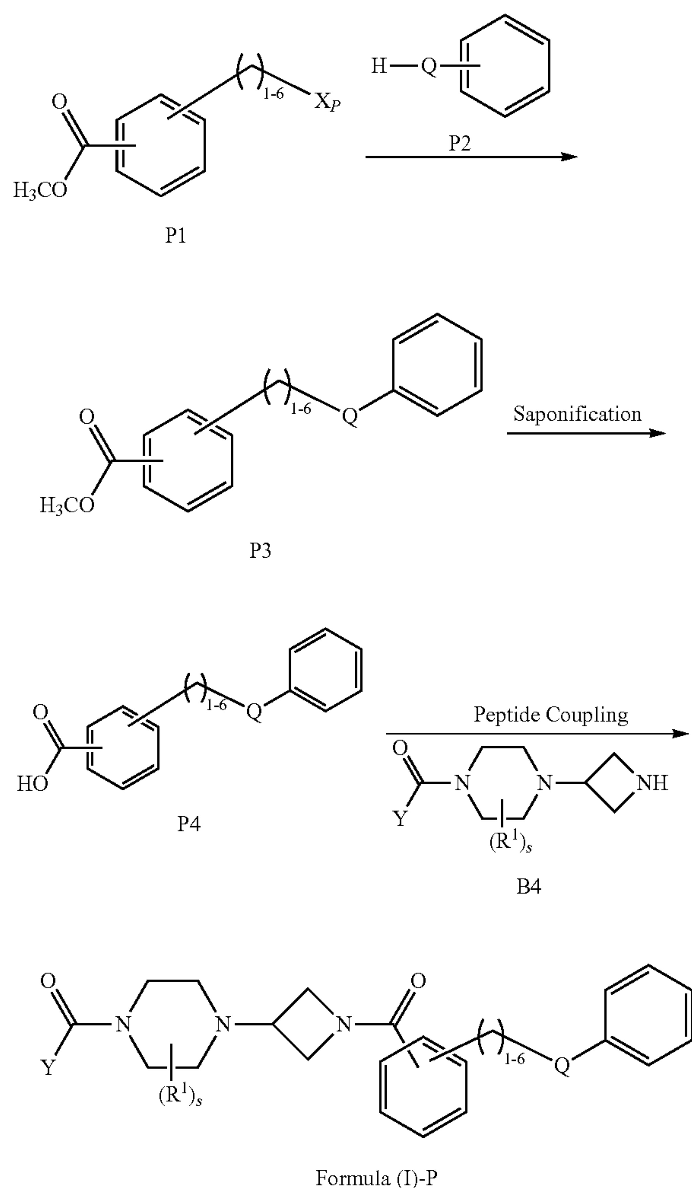
Scheme P
