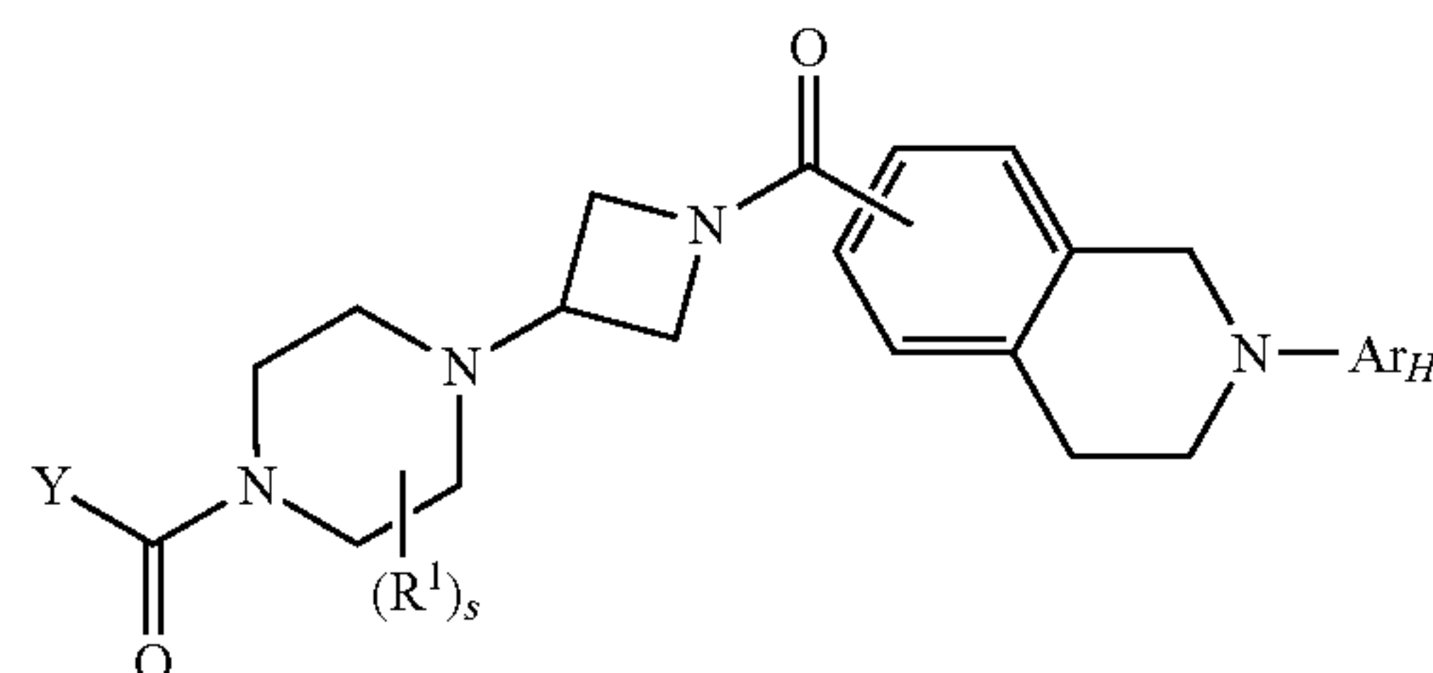
Formula (I)-H4
