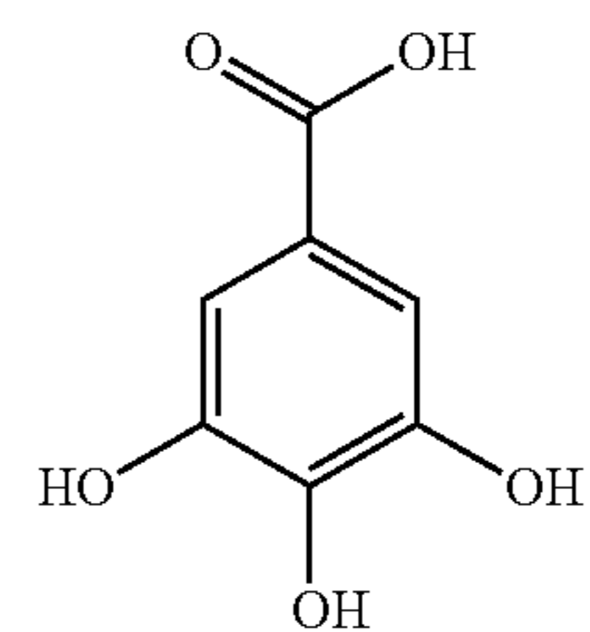
Gallic acid
