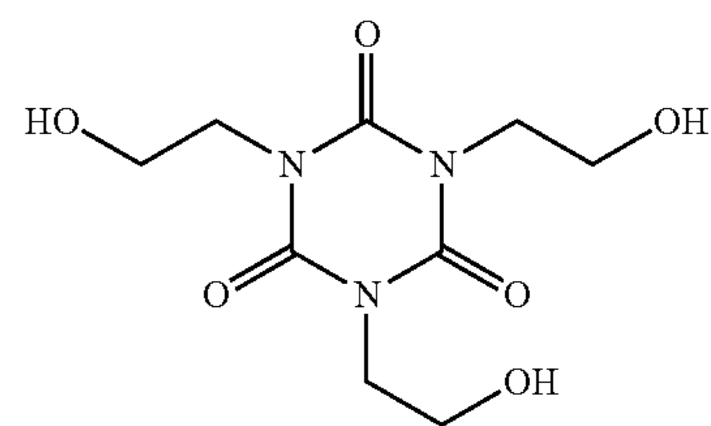
1,3,5-Tris(2-hydroxyethyl)-Cyanuric acid
