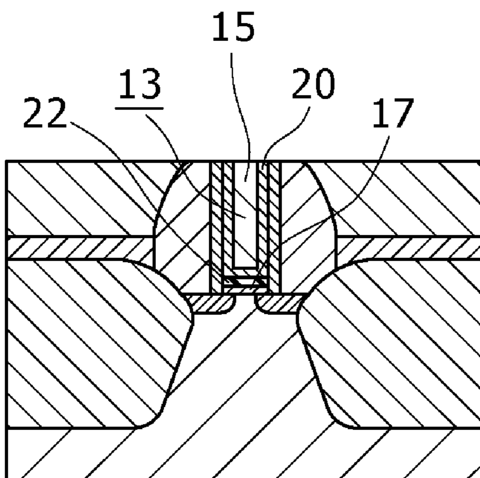
NMOS TRANSISTOR
