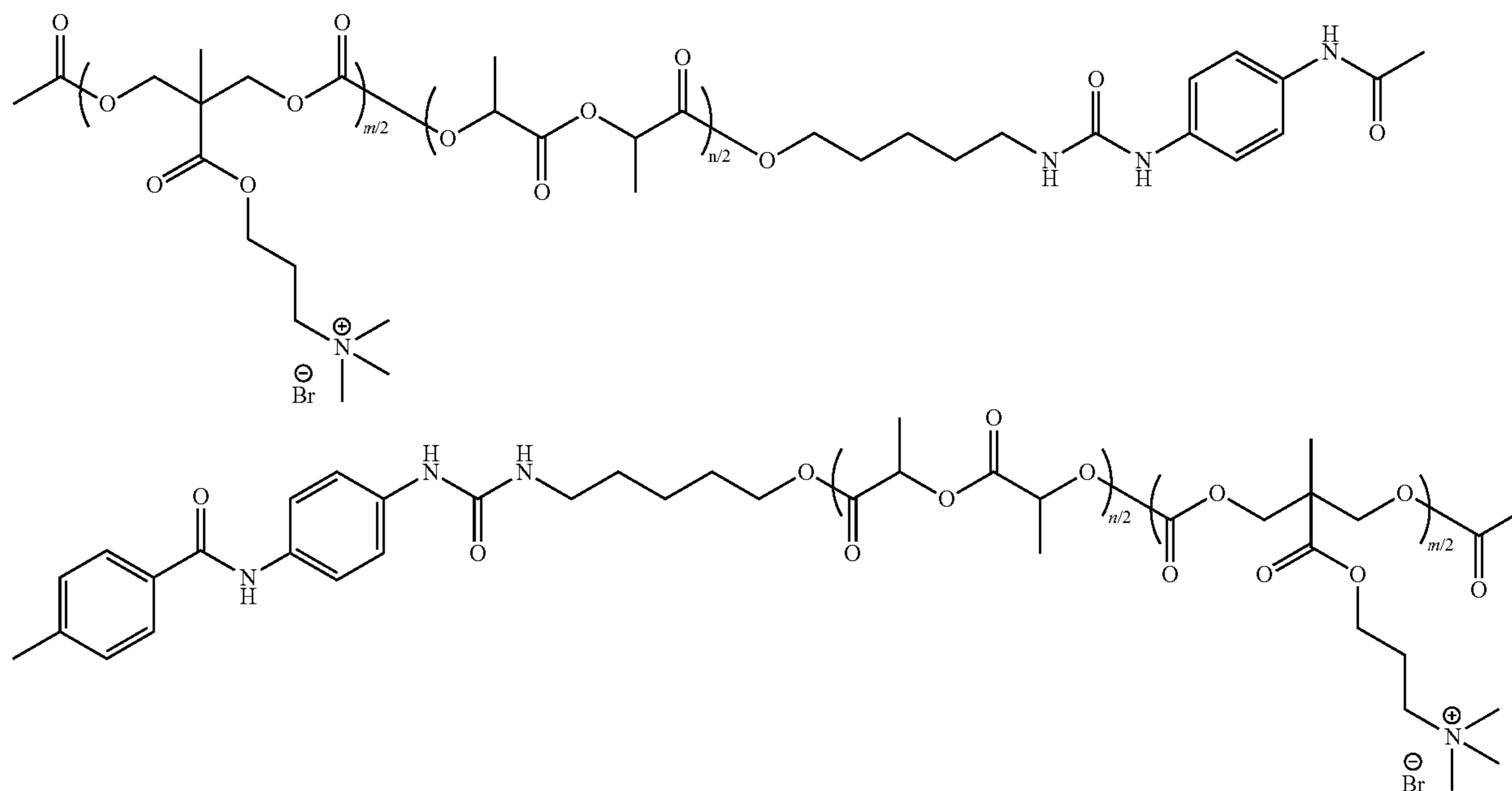
HPUPT-[P(LLA) n/2 -b-P(MTCOPrBr m/2 *NMe 3 )Ac] 2
