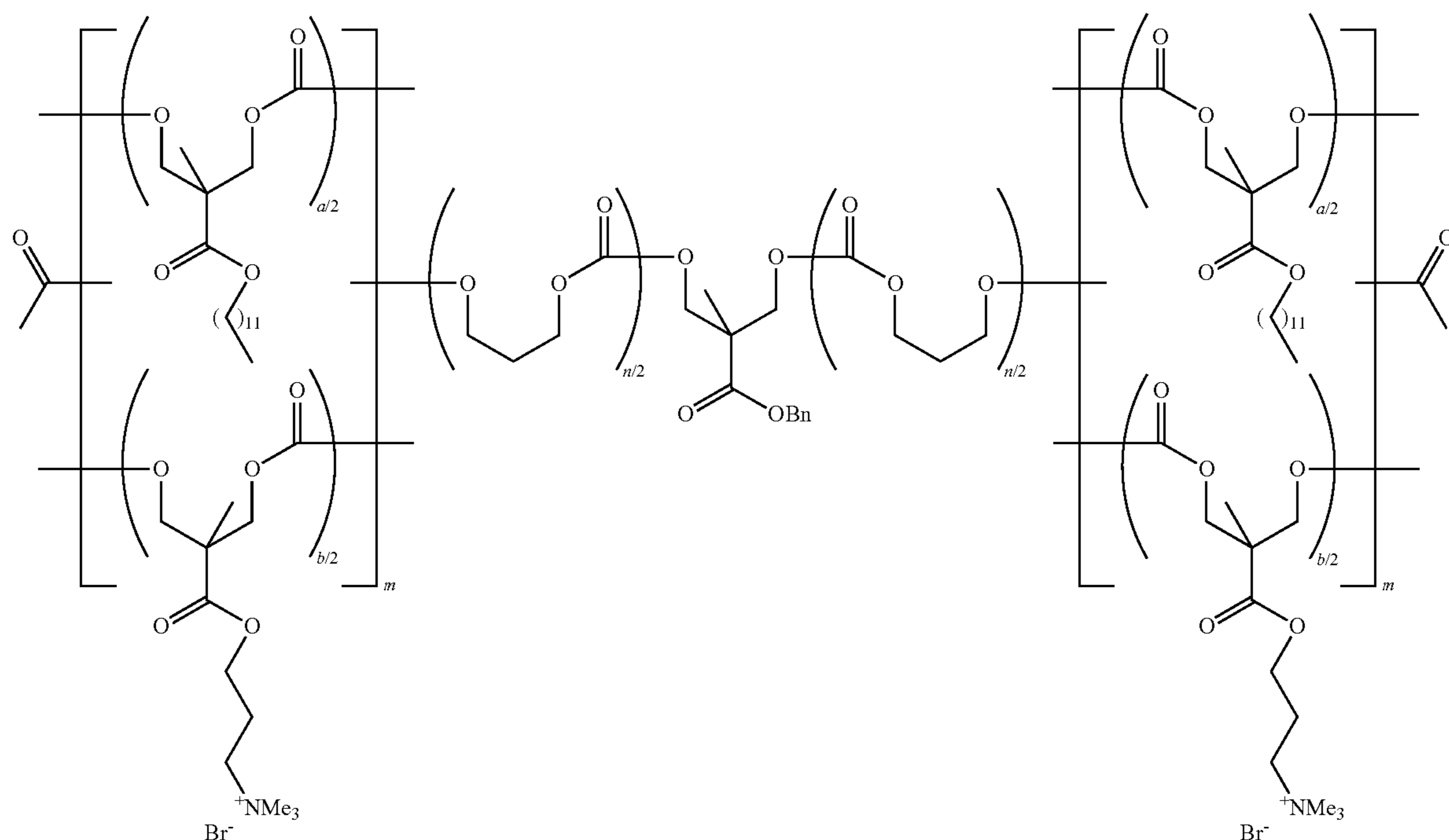
BnMPA-[P(TMC)_{n/2}-b-\{P(MTCOPrBr_{b/2}^*NMe_3-r-MTCOC12_{a/2})_m\}_2]
