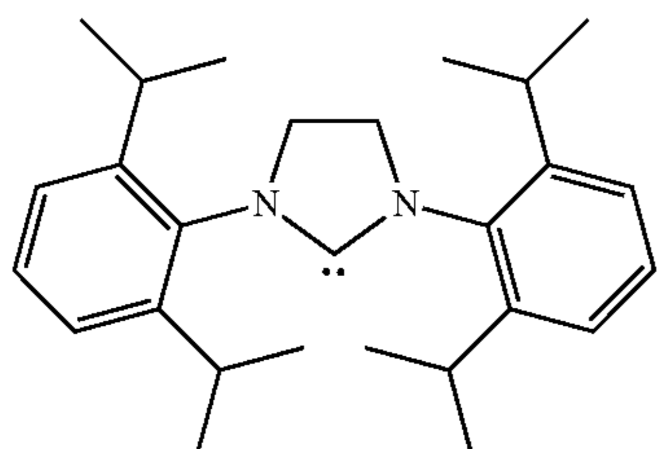
1,3-Bis(2,6-di-i-propylphenyl)-4,5-dihydroimidazol-2-ylidene (Im-8)
