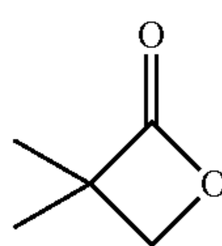
Pivalolactone (PVL)
