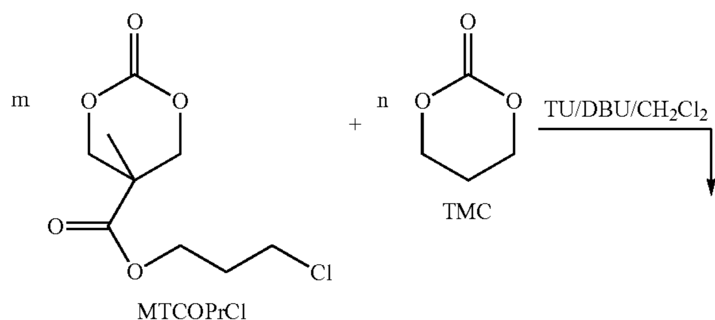
Scheme 2.
