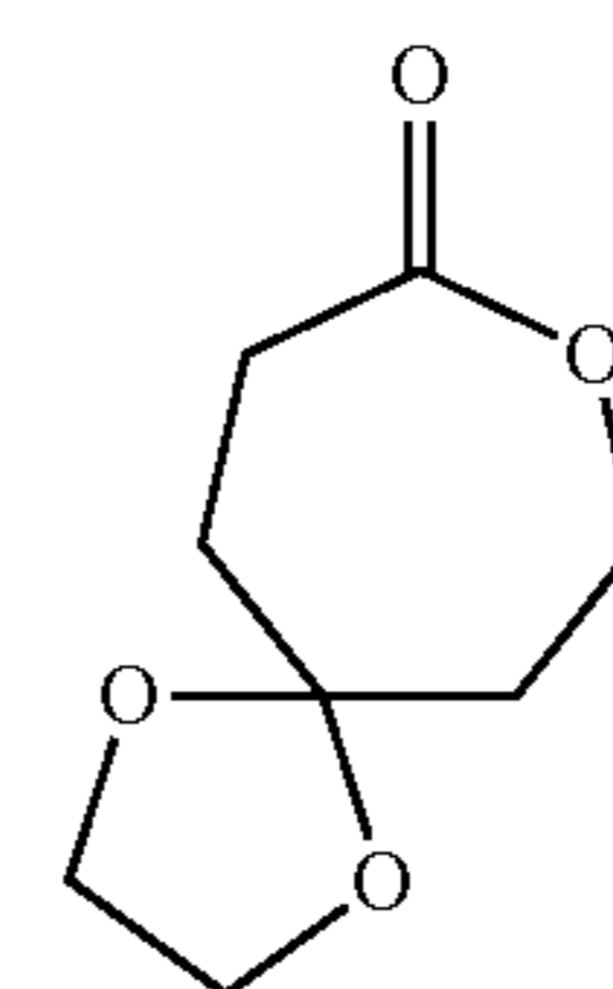
1,4,8-Trioxa(4,6)spiro-9-undecane (TOSUO)
