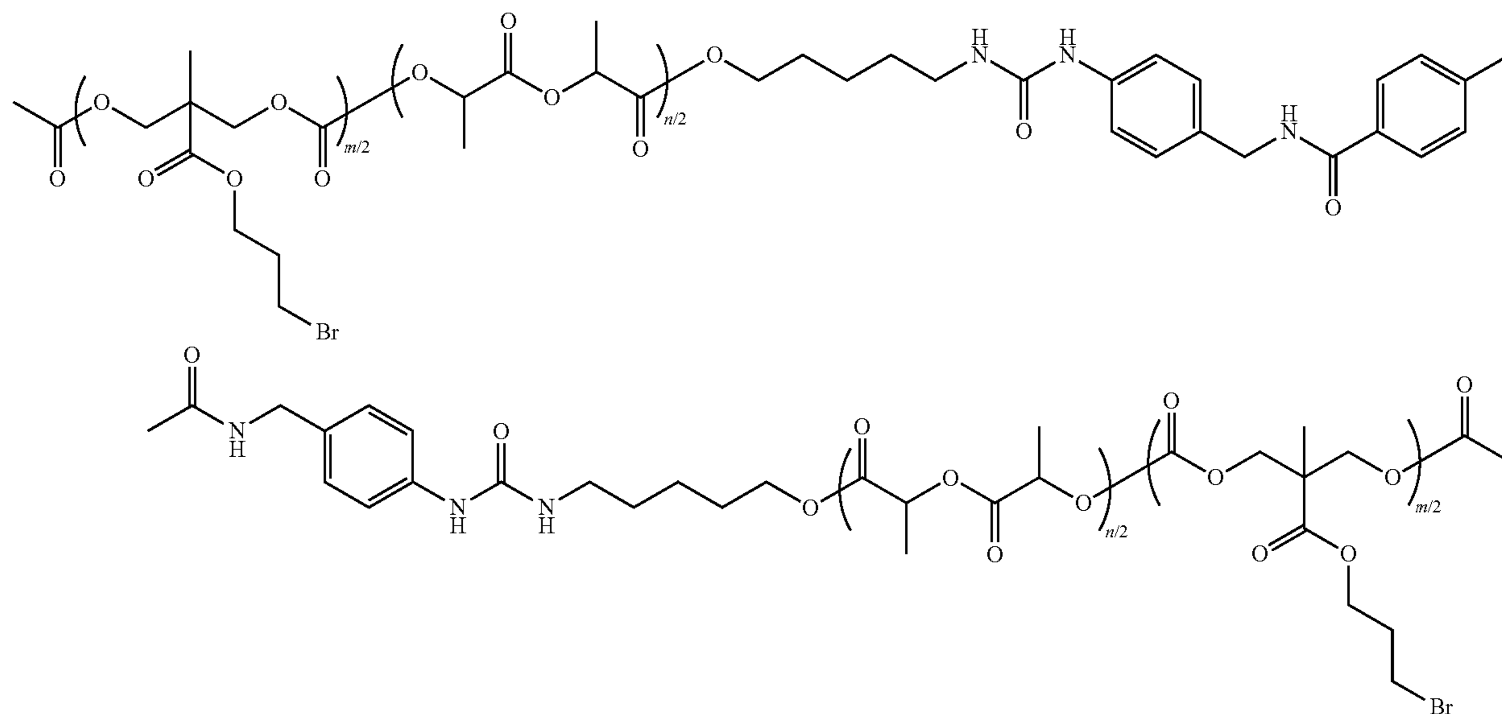
H HPUBT-[P(LLA) n/2 -b-P(MTCOPrBr) m/2 Ac] 2
