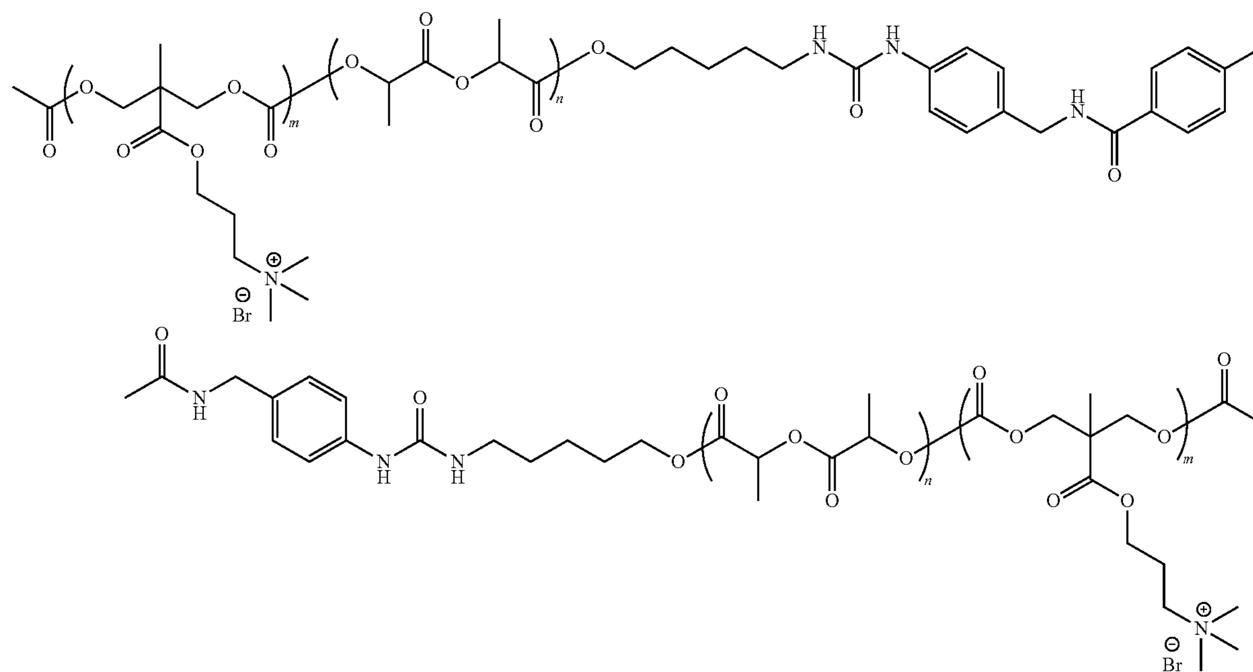
HPUBT-[P(LLA) n/2 -b-P(MTCOPrBr m/2 *NMe 3 )Ac] 2
