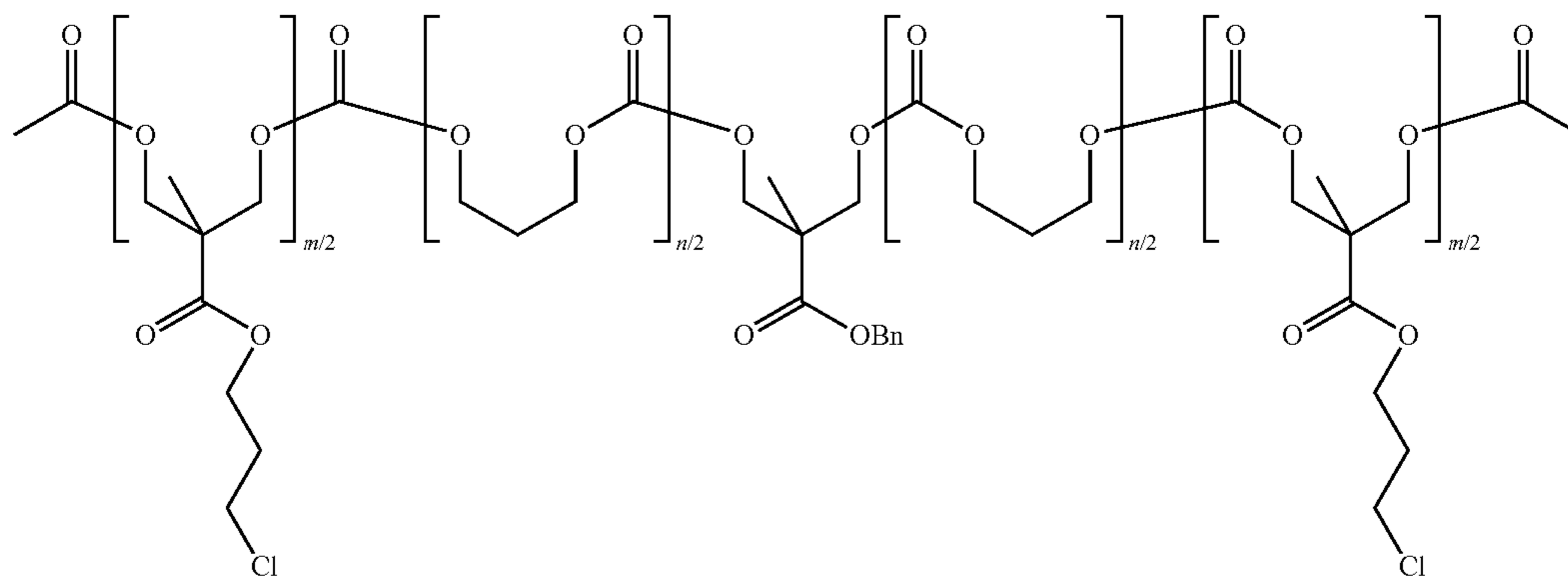
BnMPA-[P(TMC) n/2 -b-P(MTCOPrCl) m/2 Ac] 2
