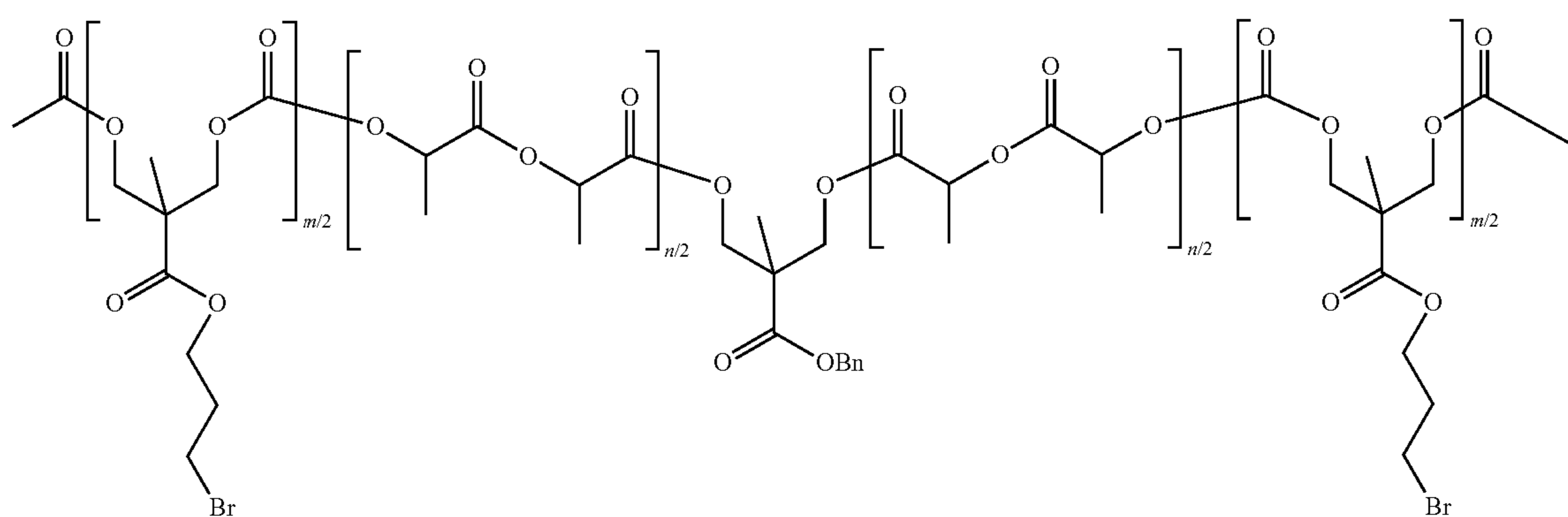
BnMPA-[P(LLA) n/2 -b-P(MTCOPrBr) m/2 Ac] 2
