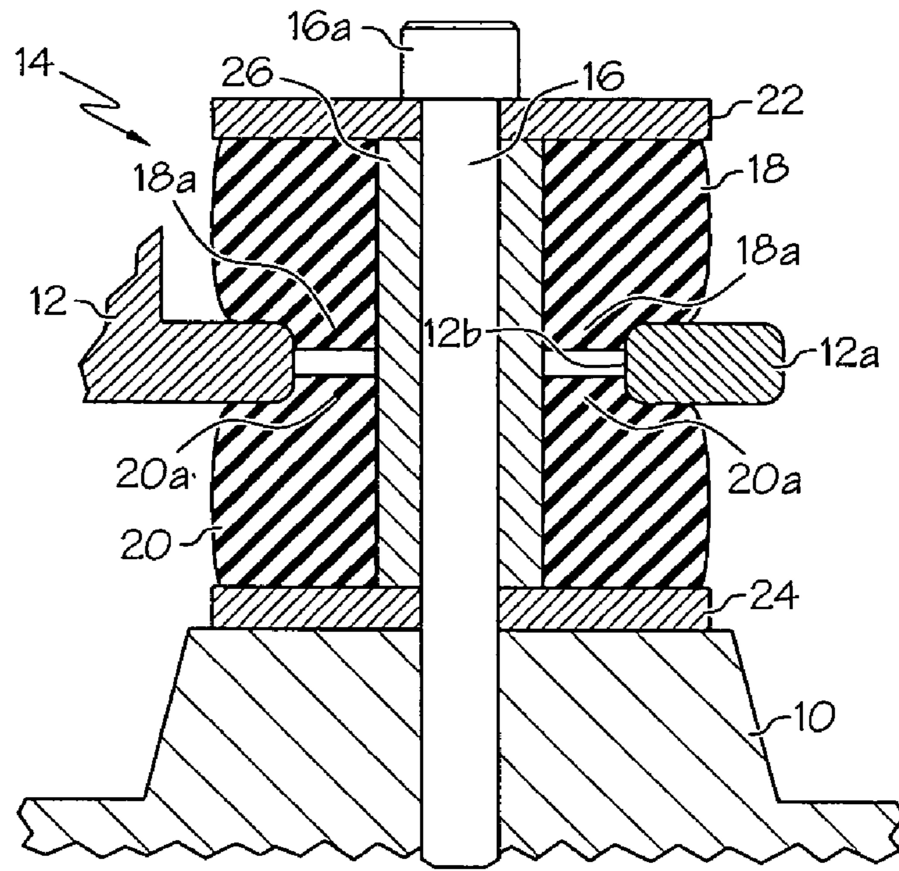
FIG. 1 (PRIOR ART)
