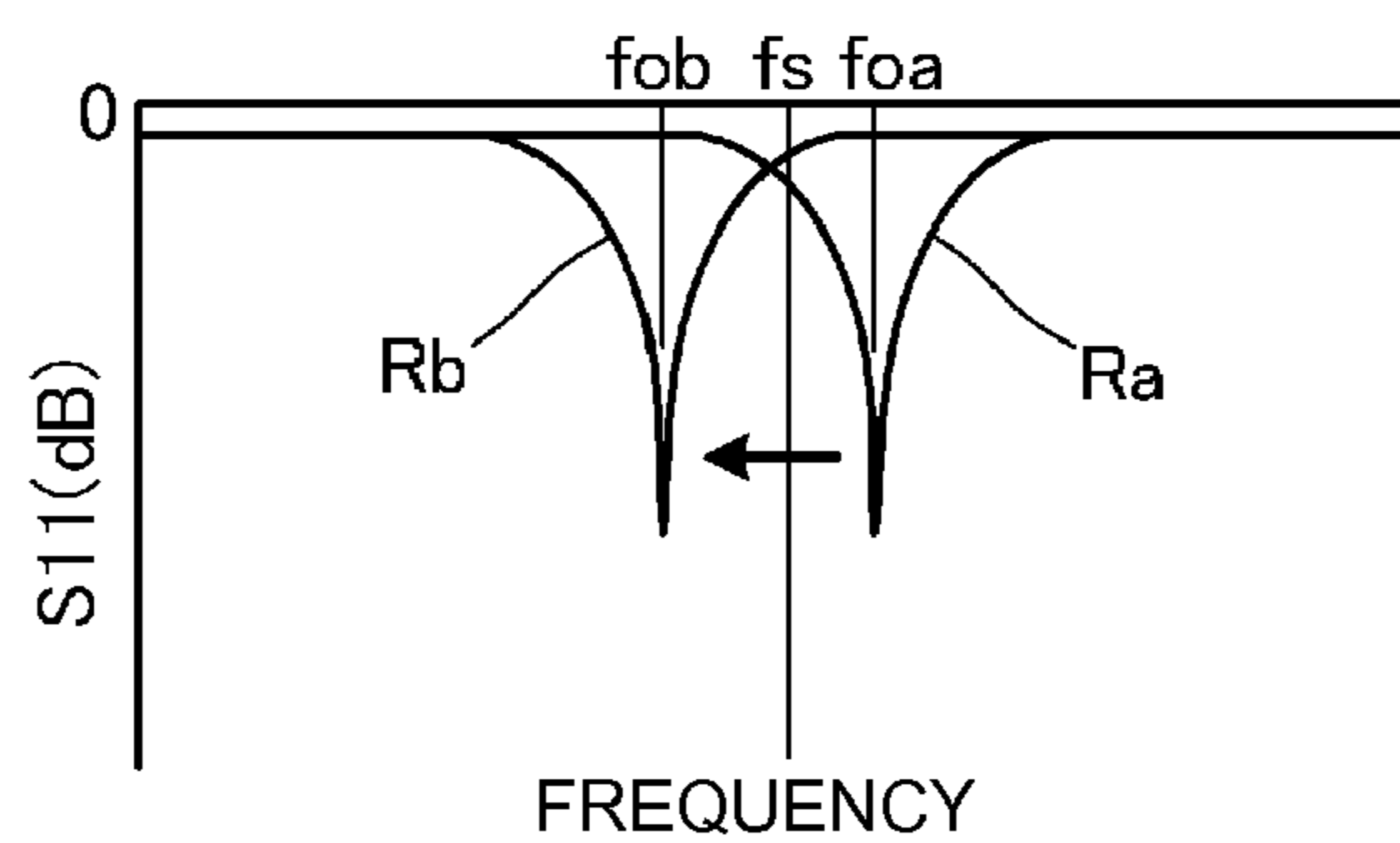
FIG. 2C PRIOR ART
