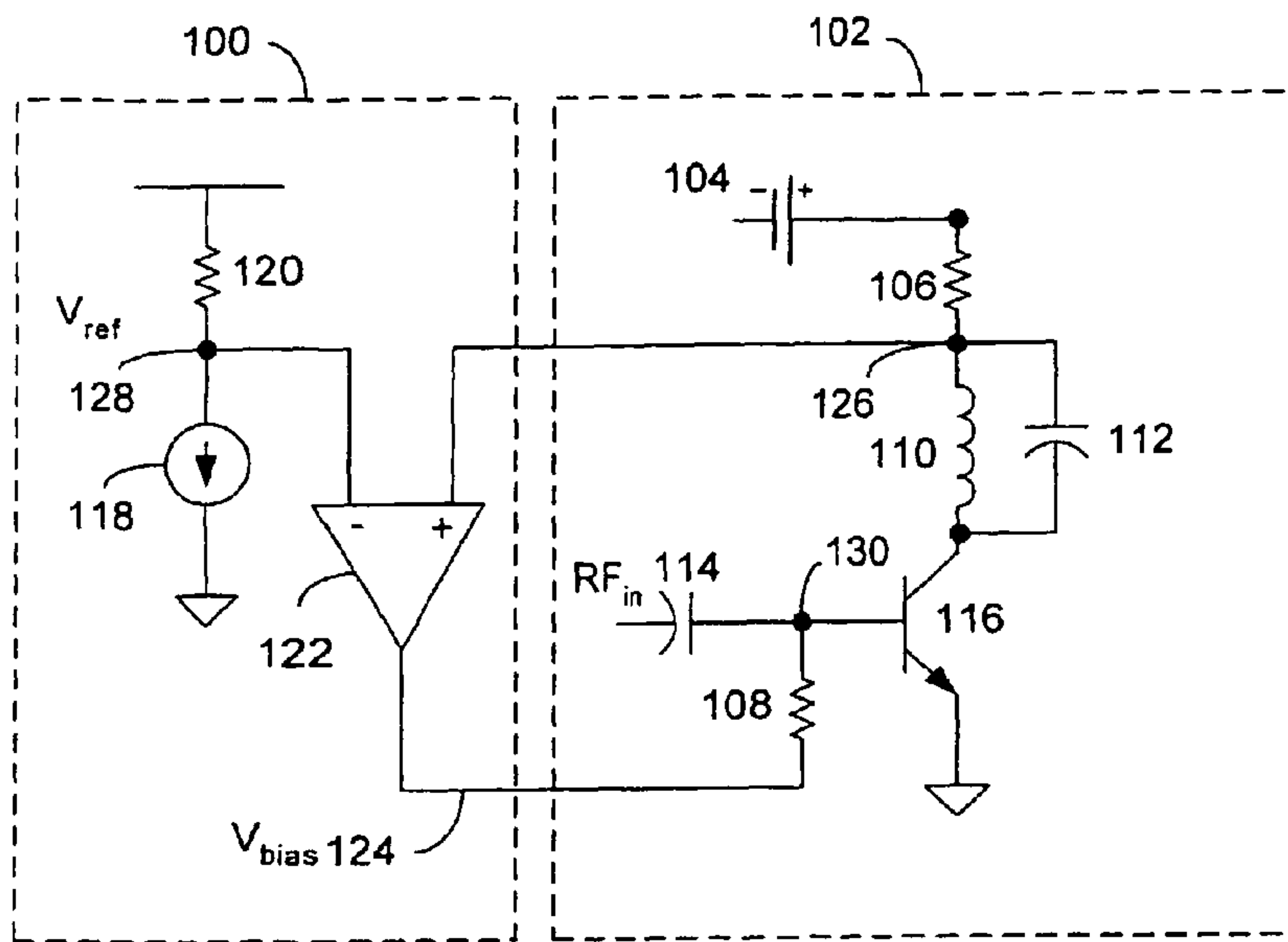
FIG. 1 (PRIOR ART)
