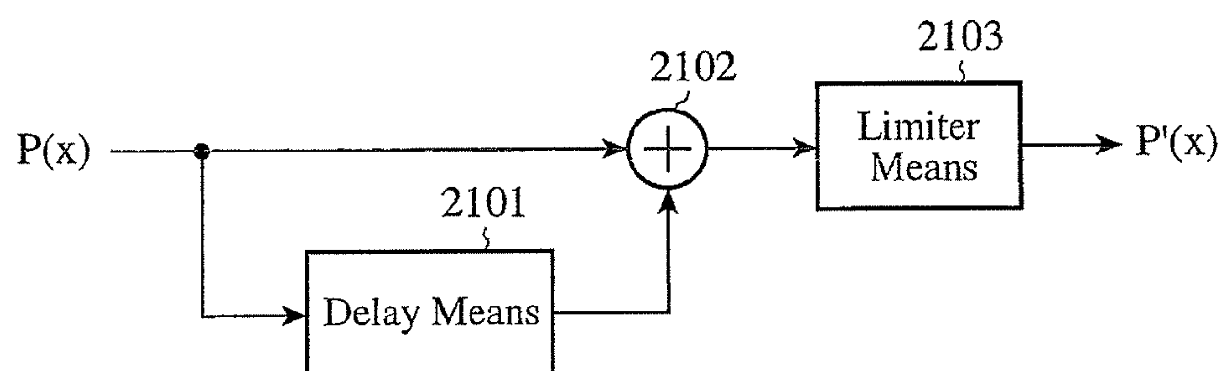
FIG. 21 CONVENTIONAL ART
