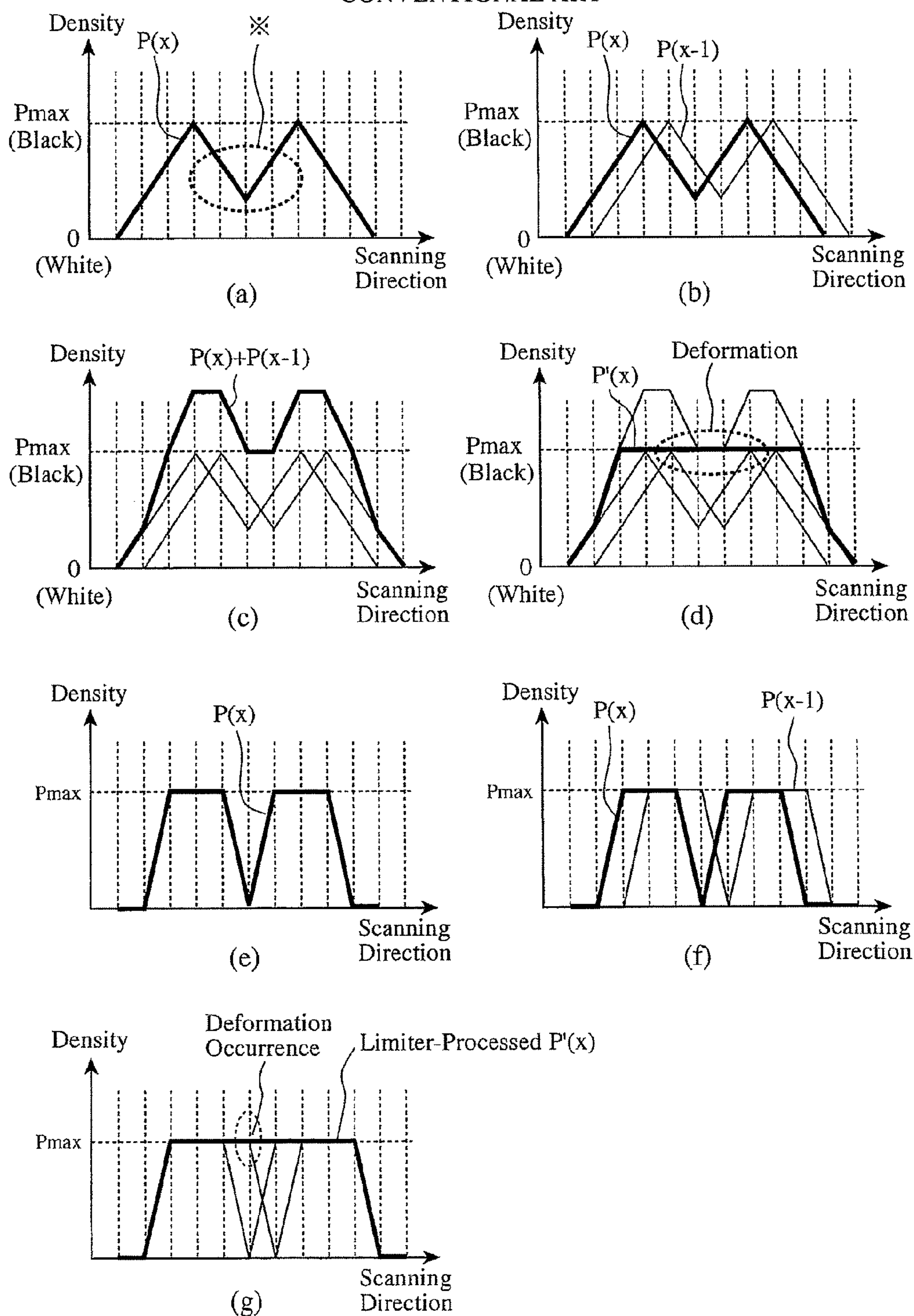
FIG. 22 CONVENTIONAL ART
