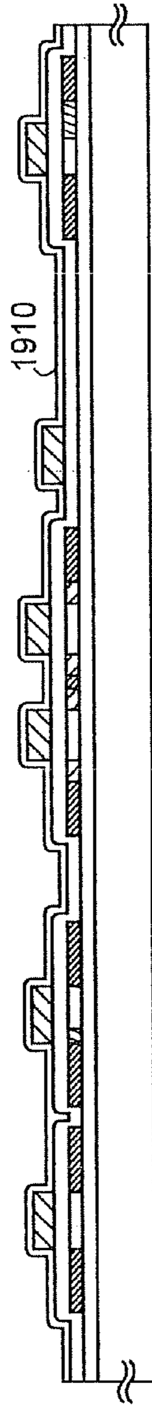
FIG. 19B GETTERING PROCESS AND ACTIVATION PROCESS
