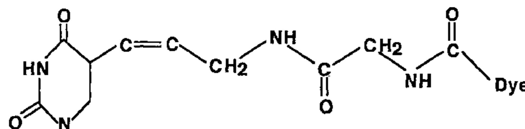
Diglycinyl linker
