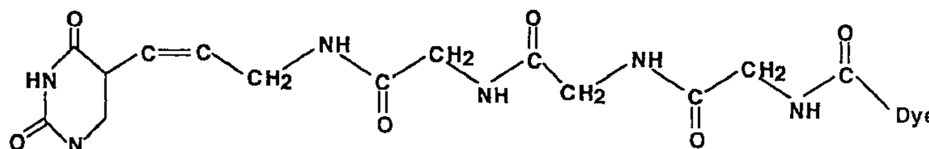
Tetraglycinyl linker
