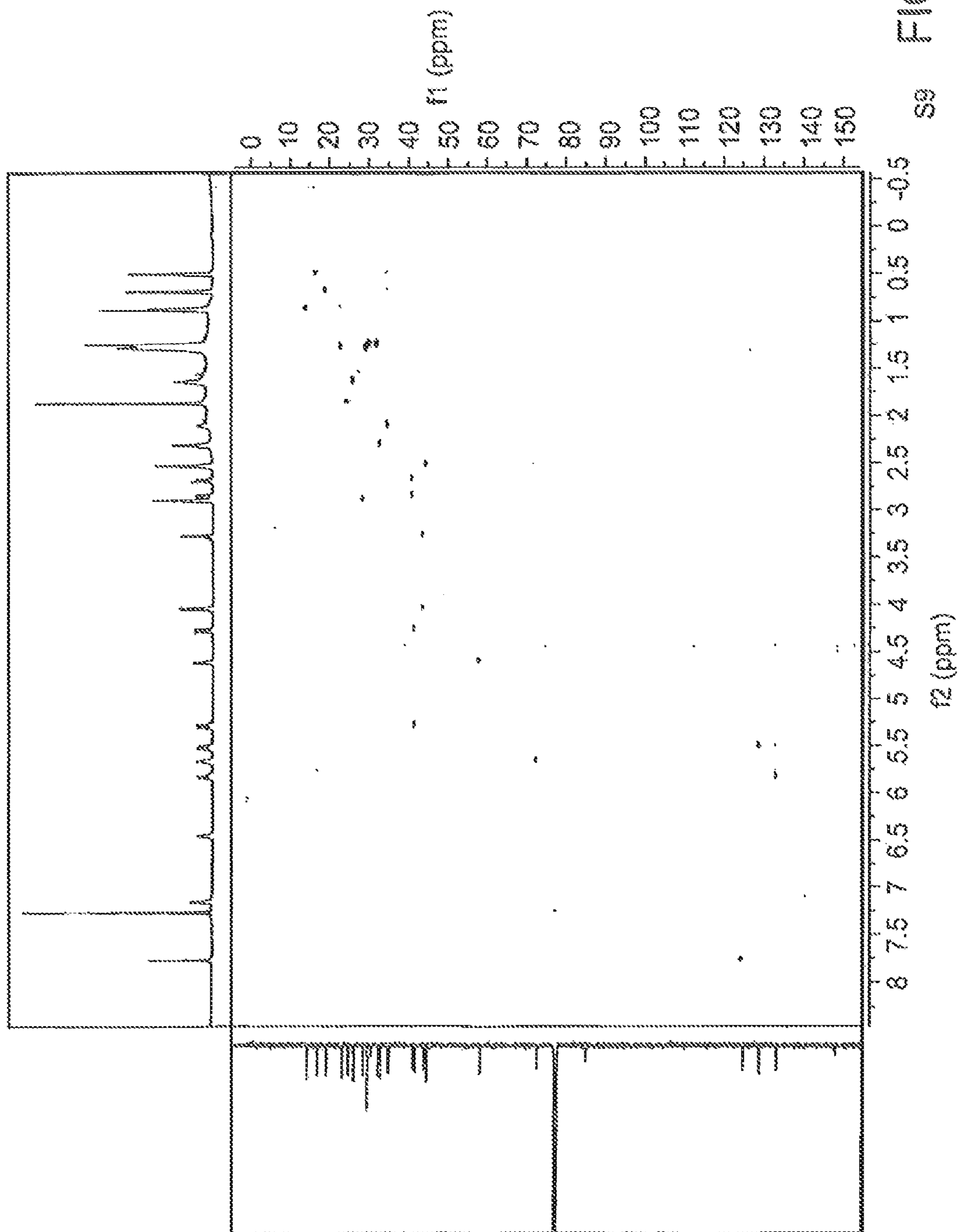
HSQC Spectrum of Largazole (1) in CDCl 3
