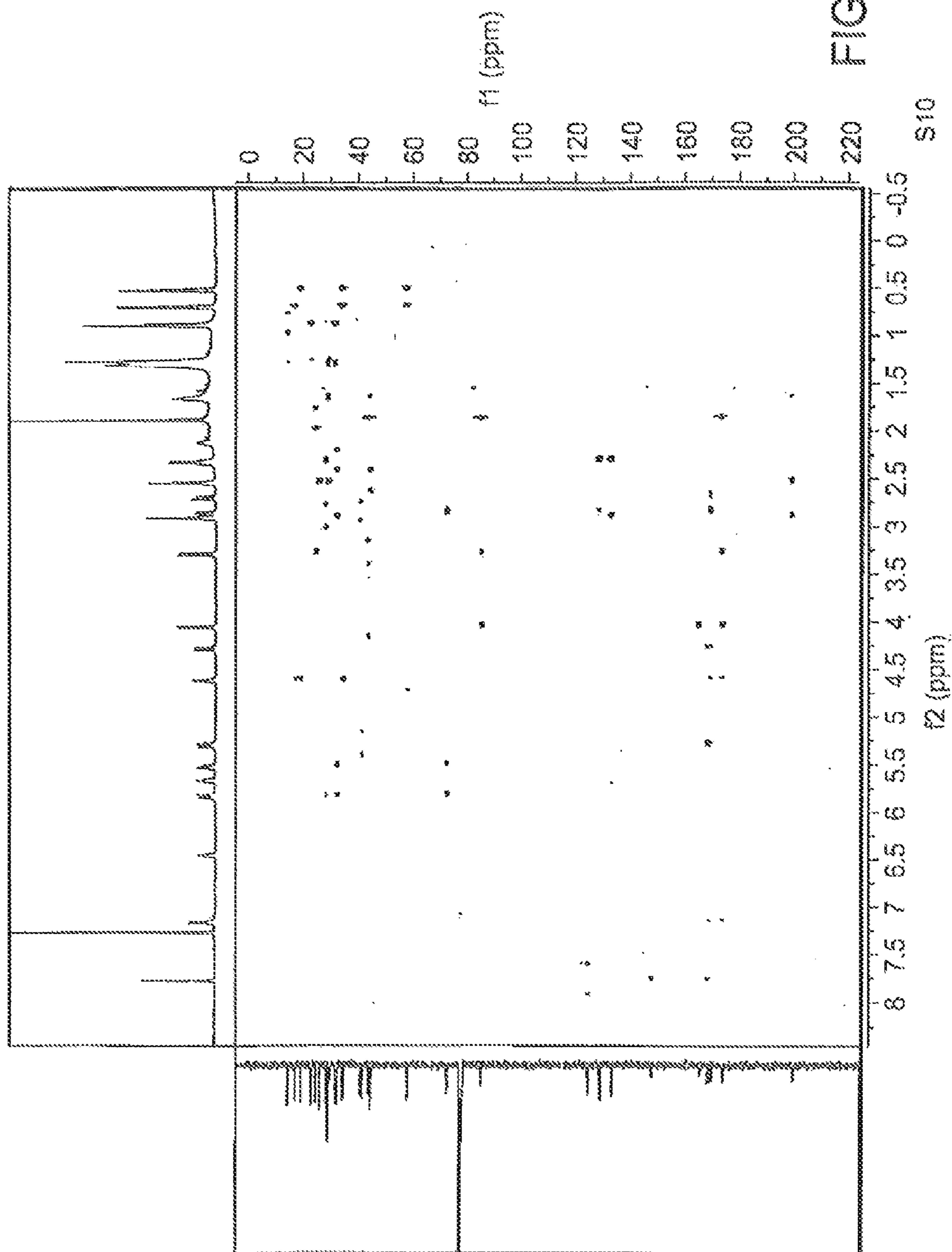
HMBC Spectrum of Largazole (1) in CDCl 3 (optimized for \nu_{ch} = 7 Hz)
