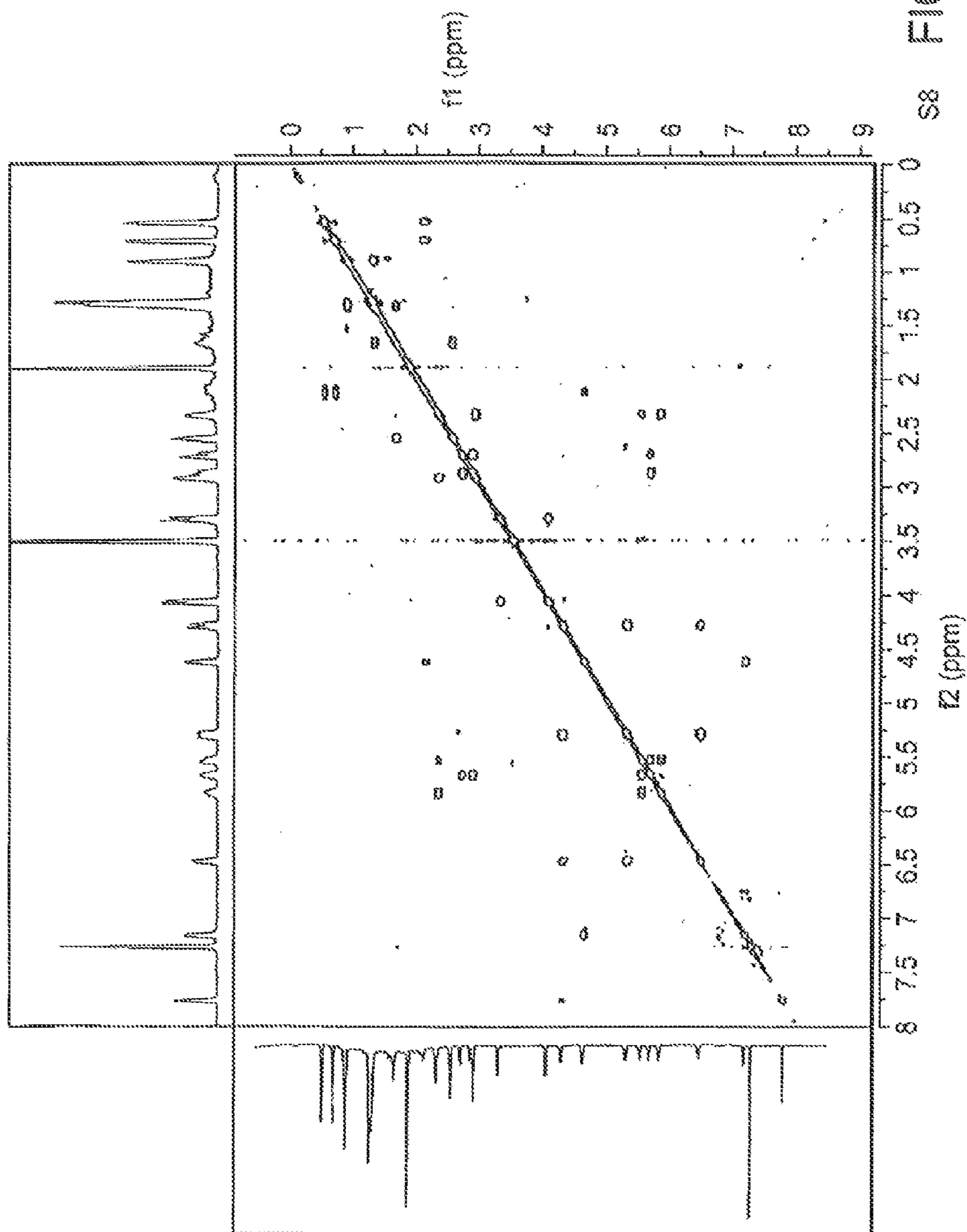
COSY Spectrum of Largazole (1) in CDCl 3
