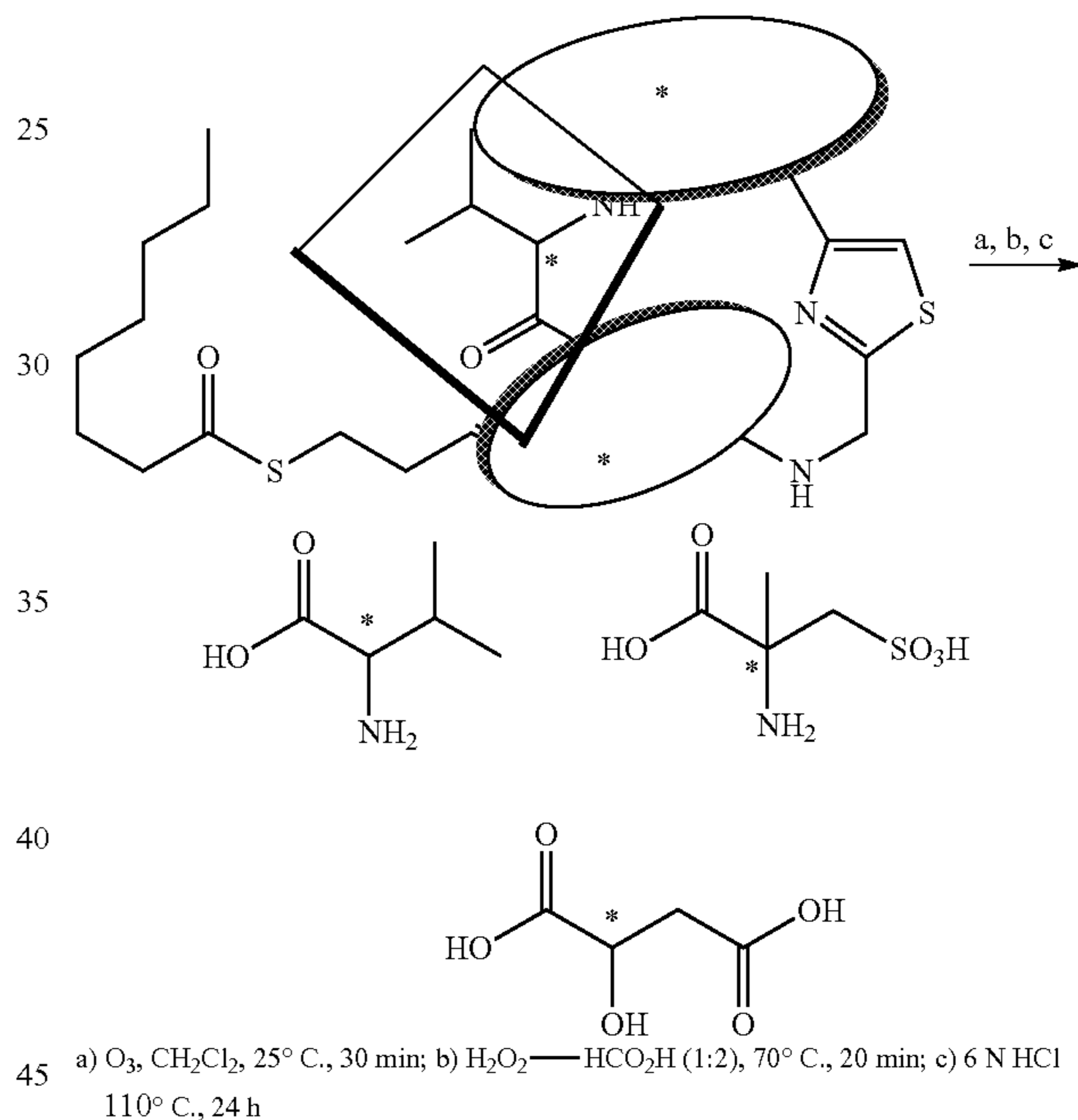
Scheme 1: Degradation strategy to liberate chiral subunits
