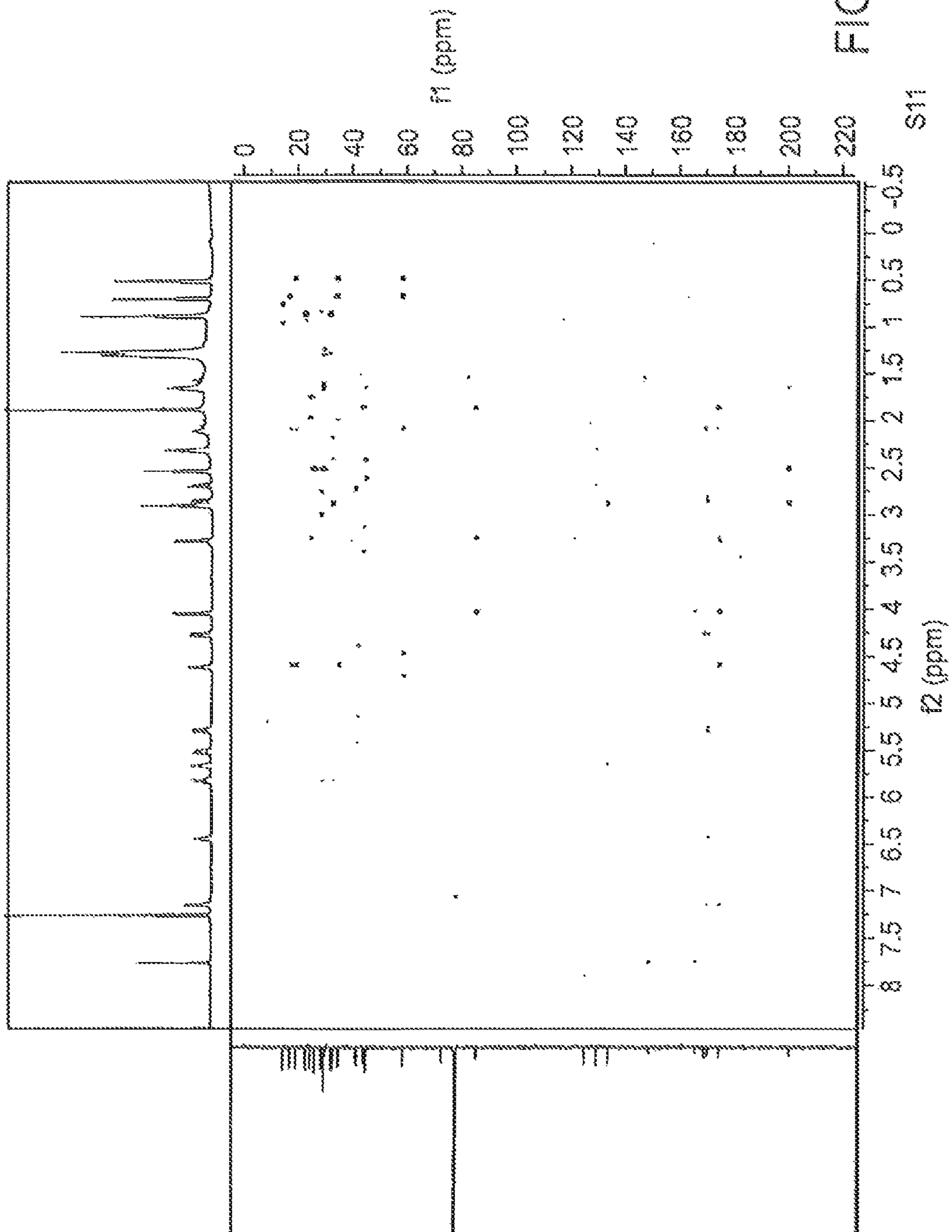
HMBC Spectrum of Largezole (1) in CDCl 3 (optimized for \nu_{\text{ch}} = 3.5 \text{ hz} )
