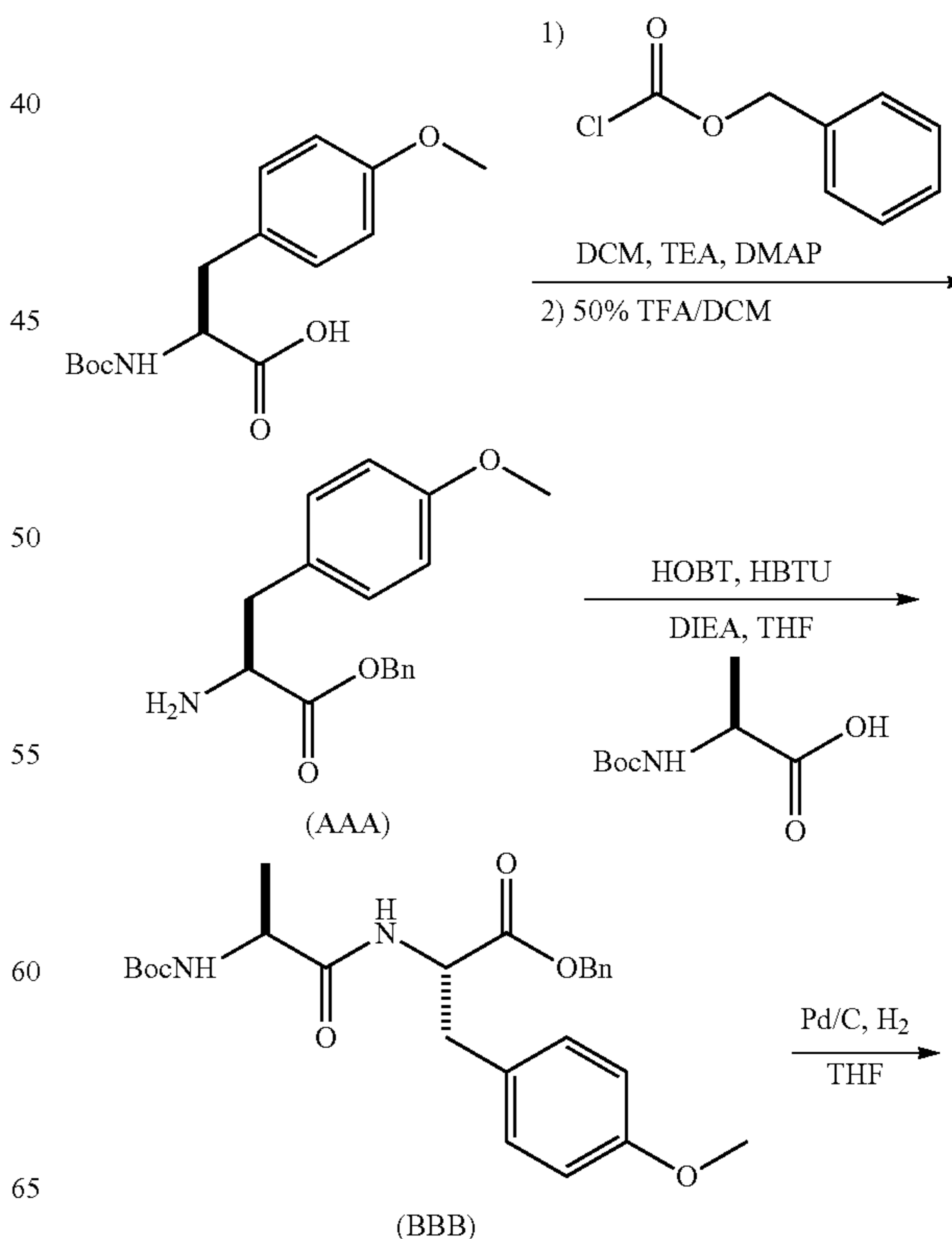
Scheme 14: Synthesis of Example 14
