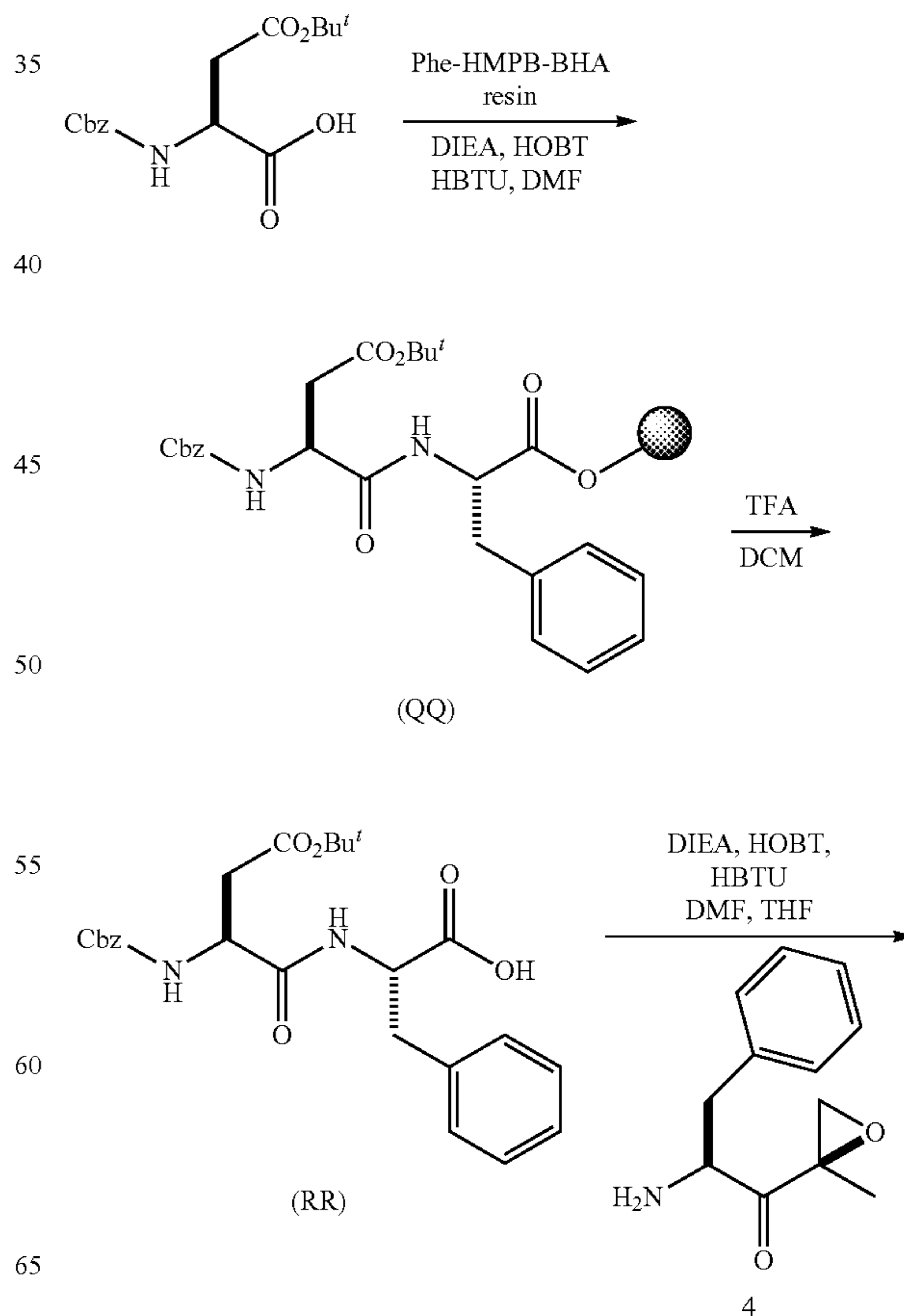
Scheme 10: Synthesis of Example 10
