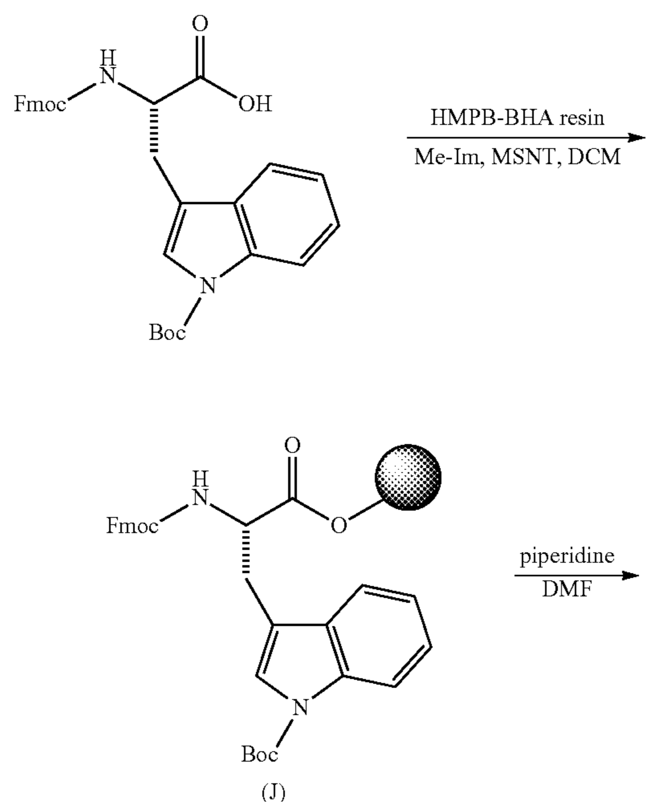
Scheme 2: Synthesis of Example 2
