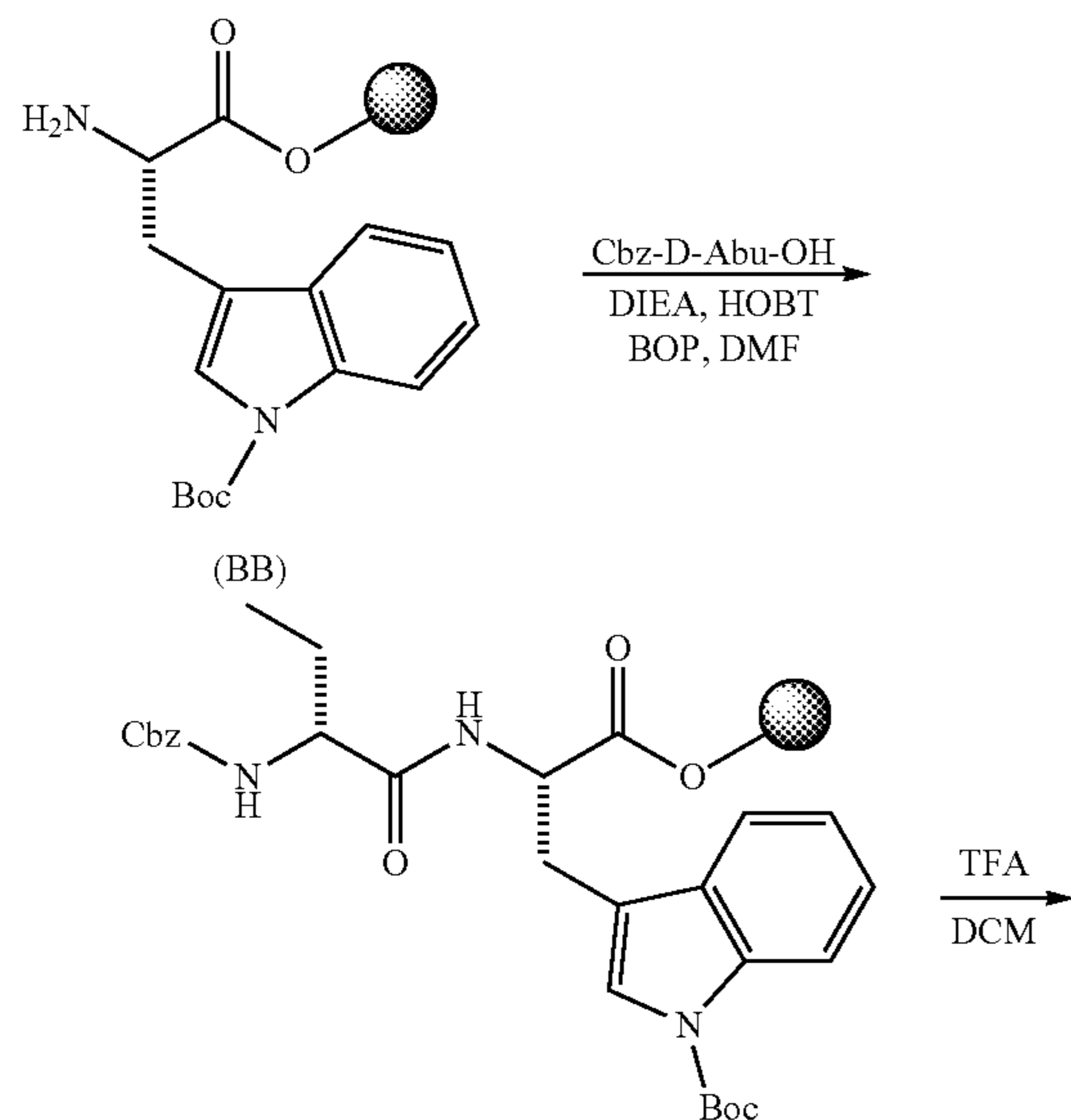
Scheme 5: Synthesis of Example 5
