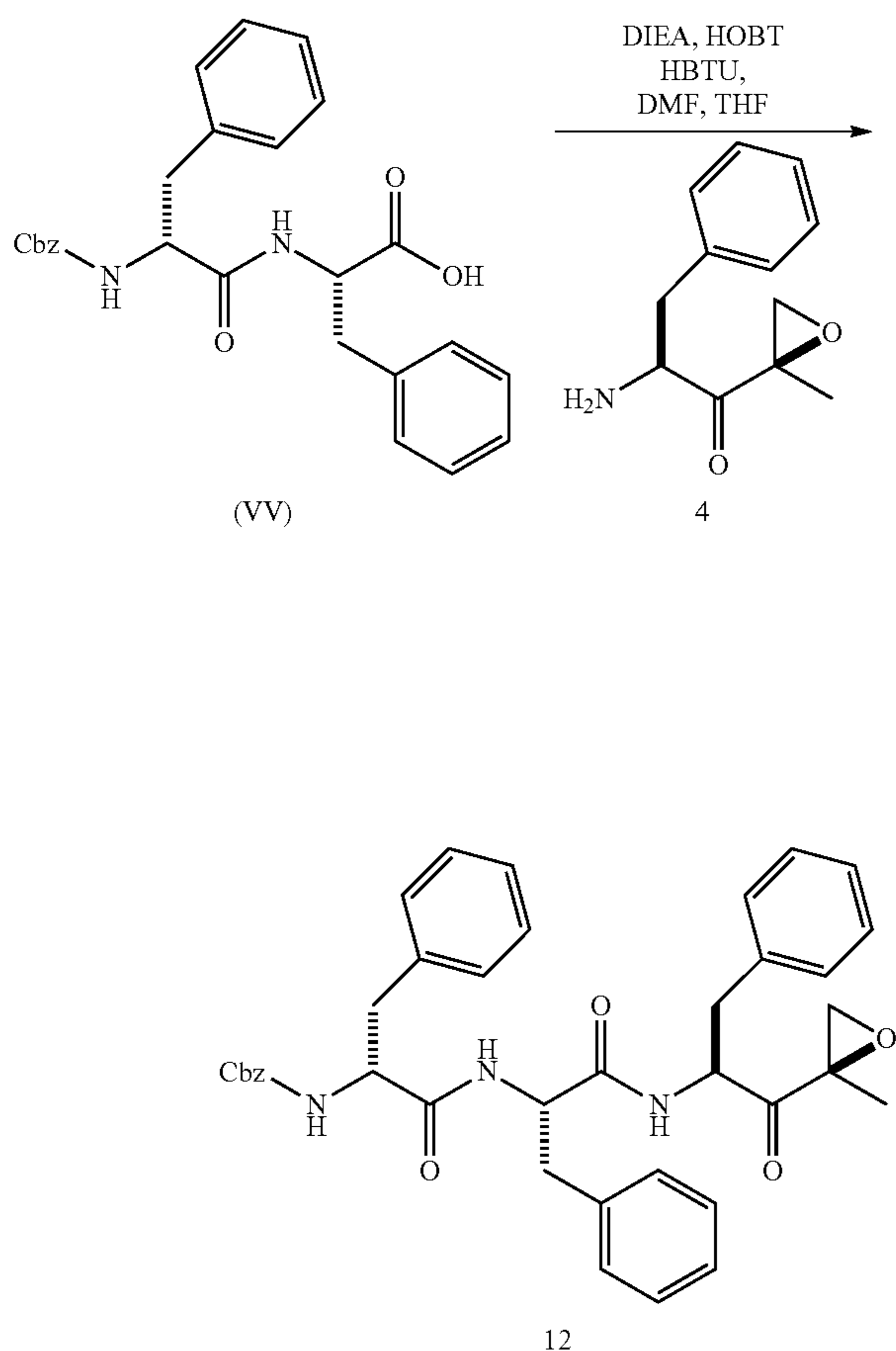
Scheme 12: Synthesis of Example 12
