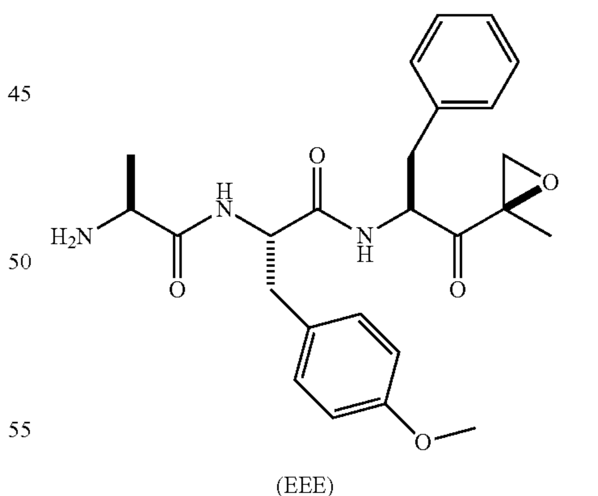
Scheme 16: Synthesis of Example 16
