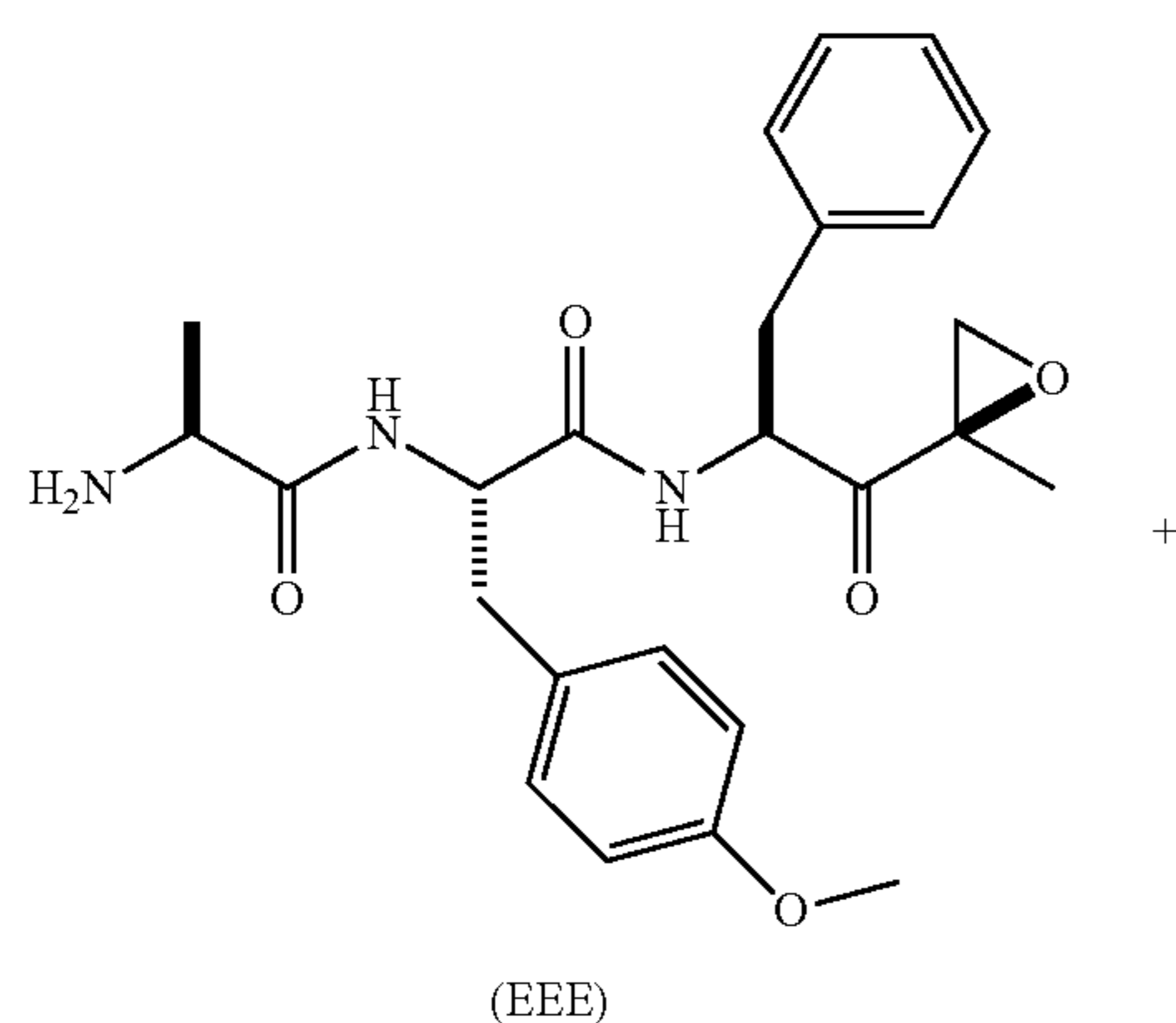
Scheme 15: Synthesis of Example 15
