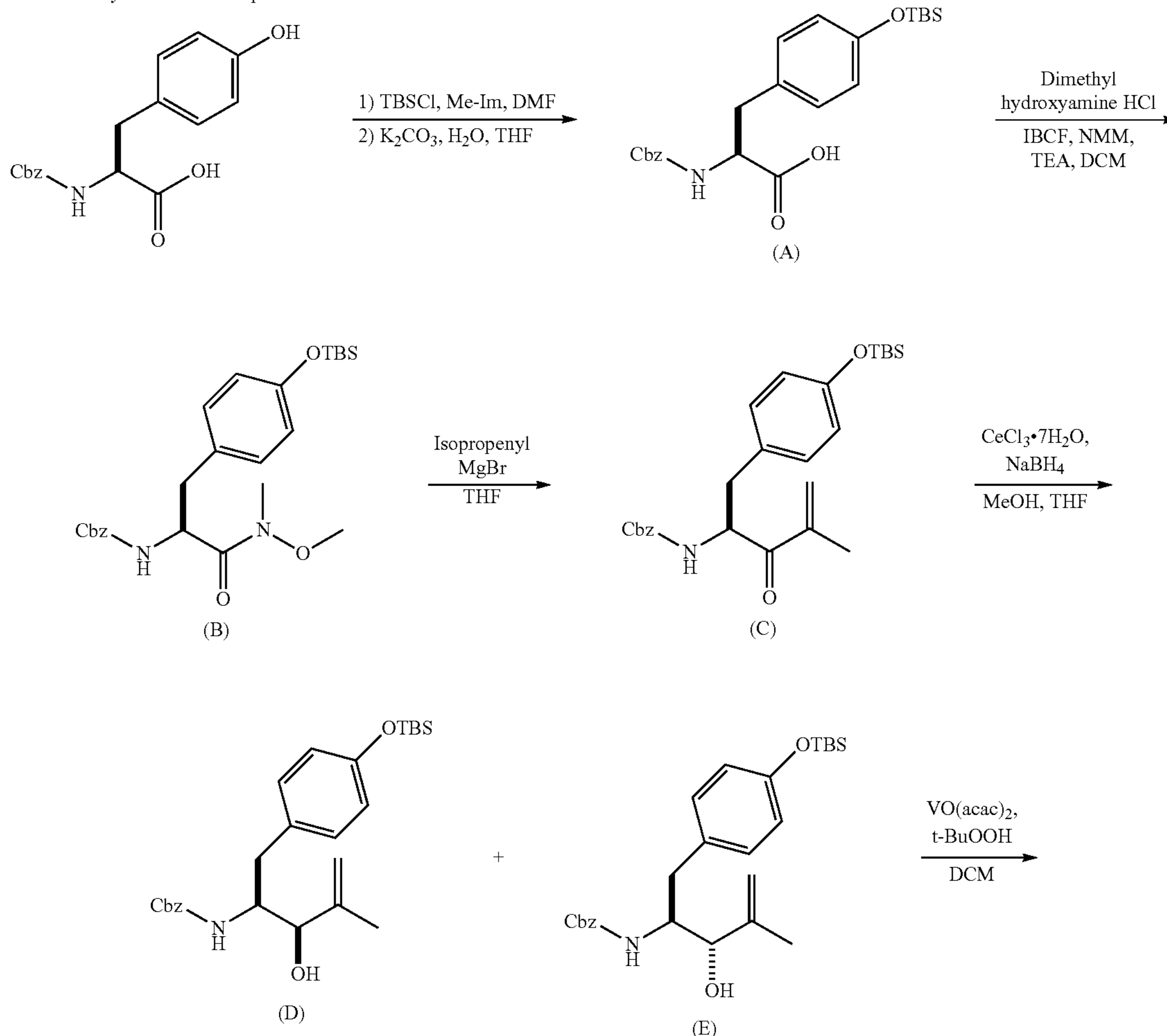
Scheme 1: Synthesis of Example 1
