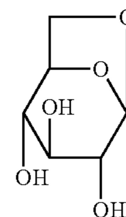
1,6-anhydro-beta-D-Glucose
