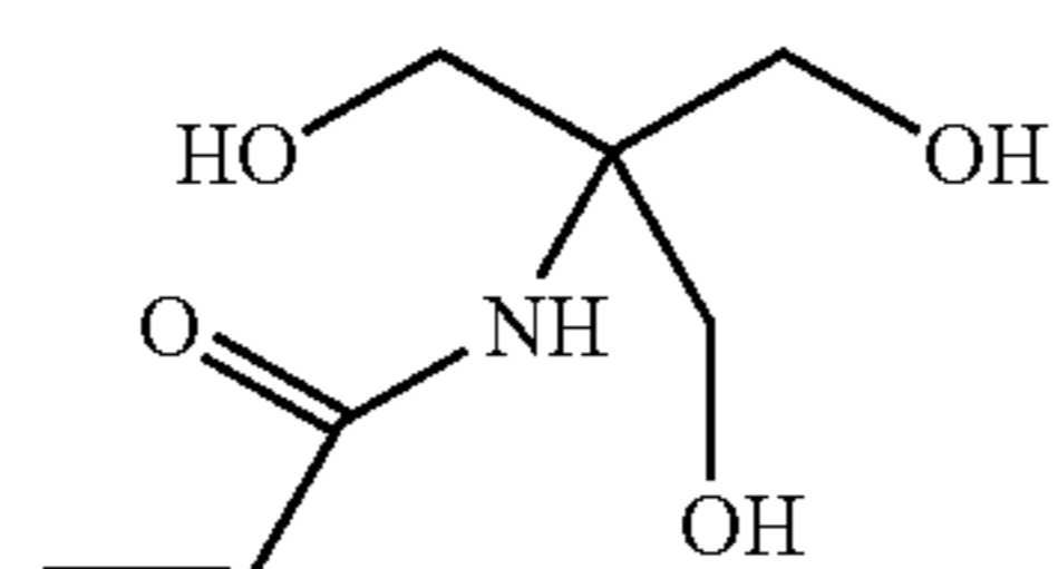
N-[Tris(hydroxymethyl)methyl]acrylamide
