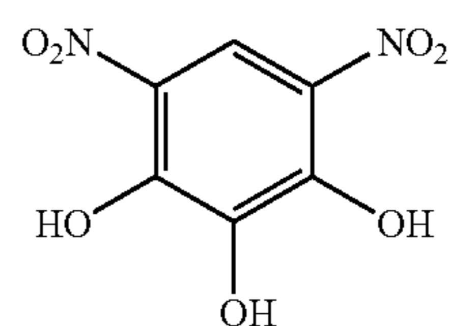
4,6-Nitropyrogallol
