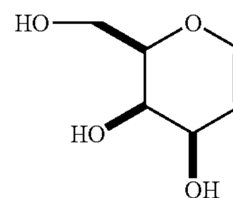
D-Galactool
