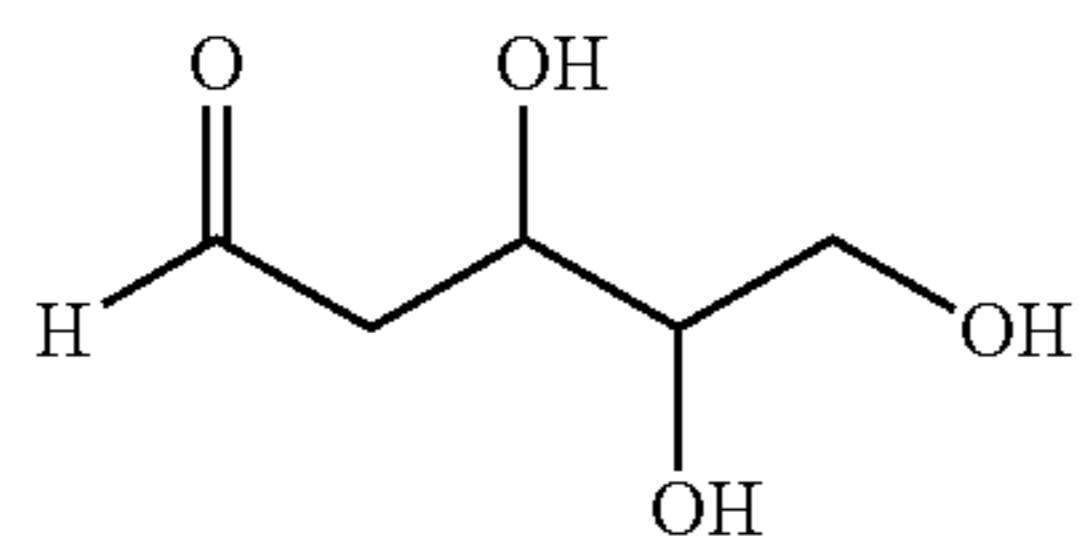
2-Deoxy-D-ribose
