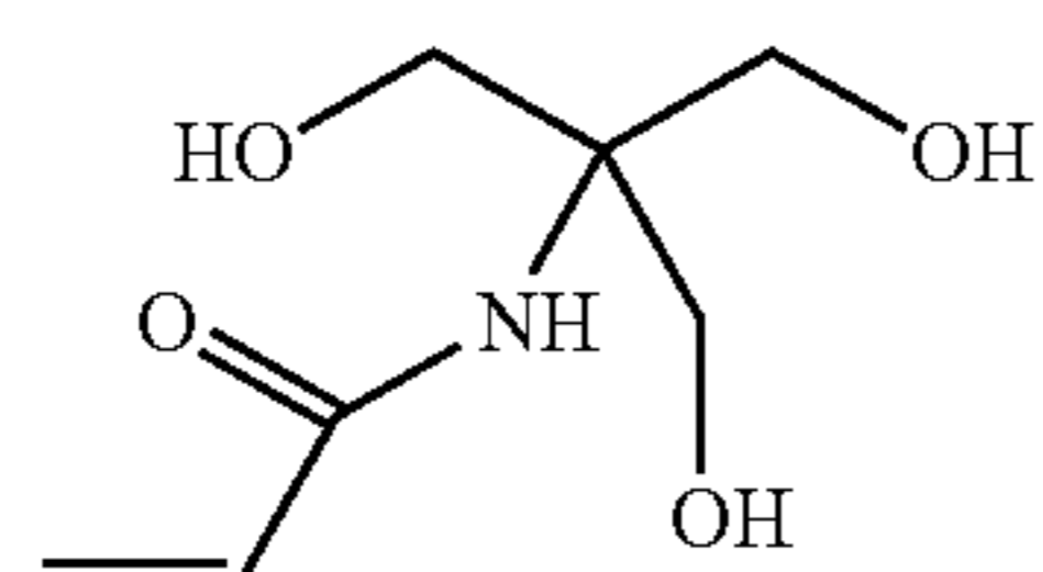
N-[Tris(hydroxymethyl)methyl]acrylamide
