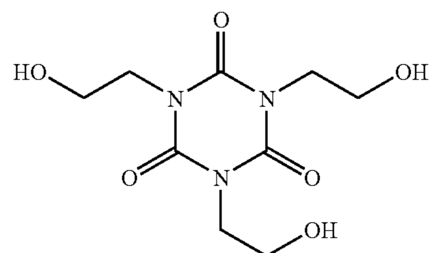
1,3,5-Tris(2-hydroxyethyl)-Cyanuric acid
