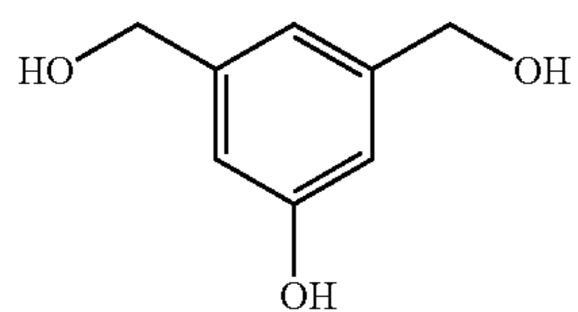
3,5-Di(hydroxymethyl)phenol
