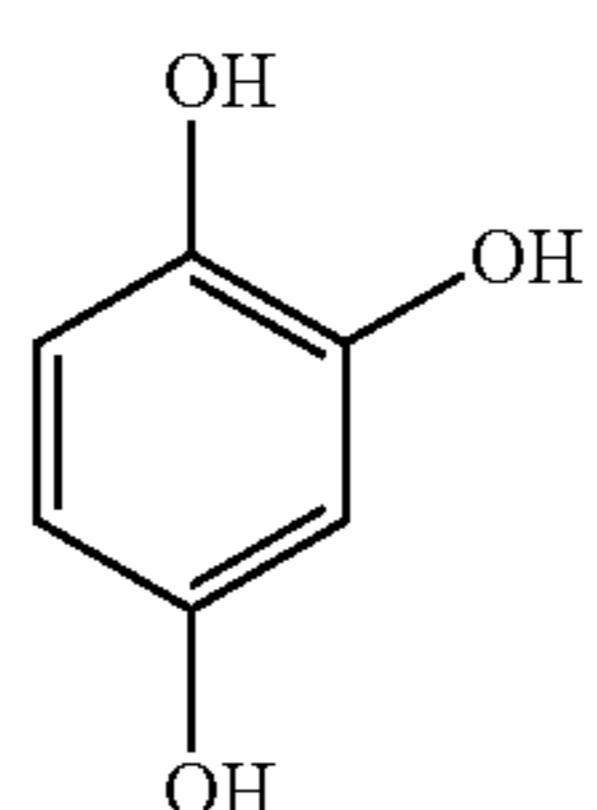
1,2,4-Trihydroxyl-benzene
