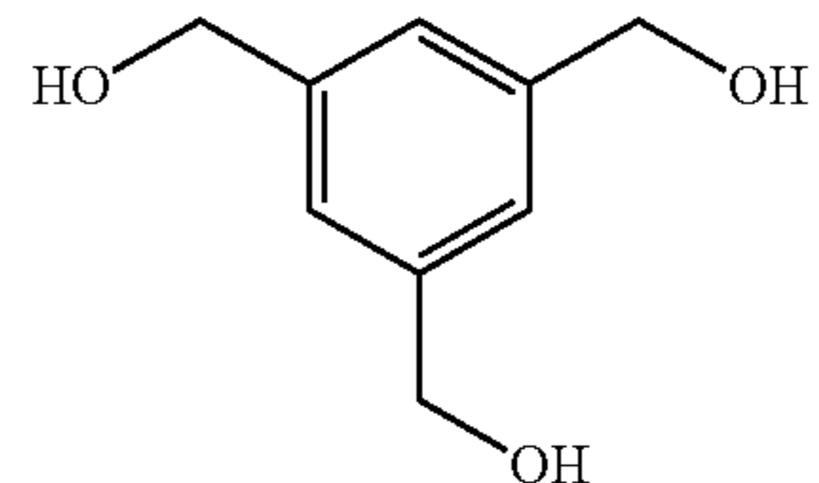
1,3,5-Tri(hydroxymethyl)benzene
