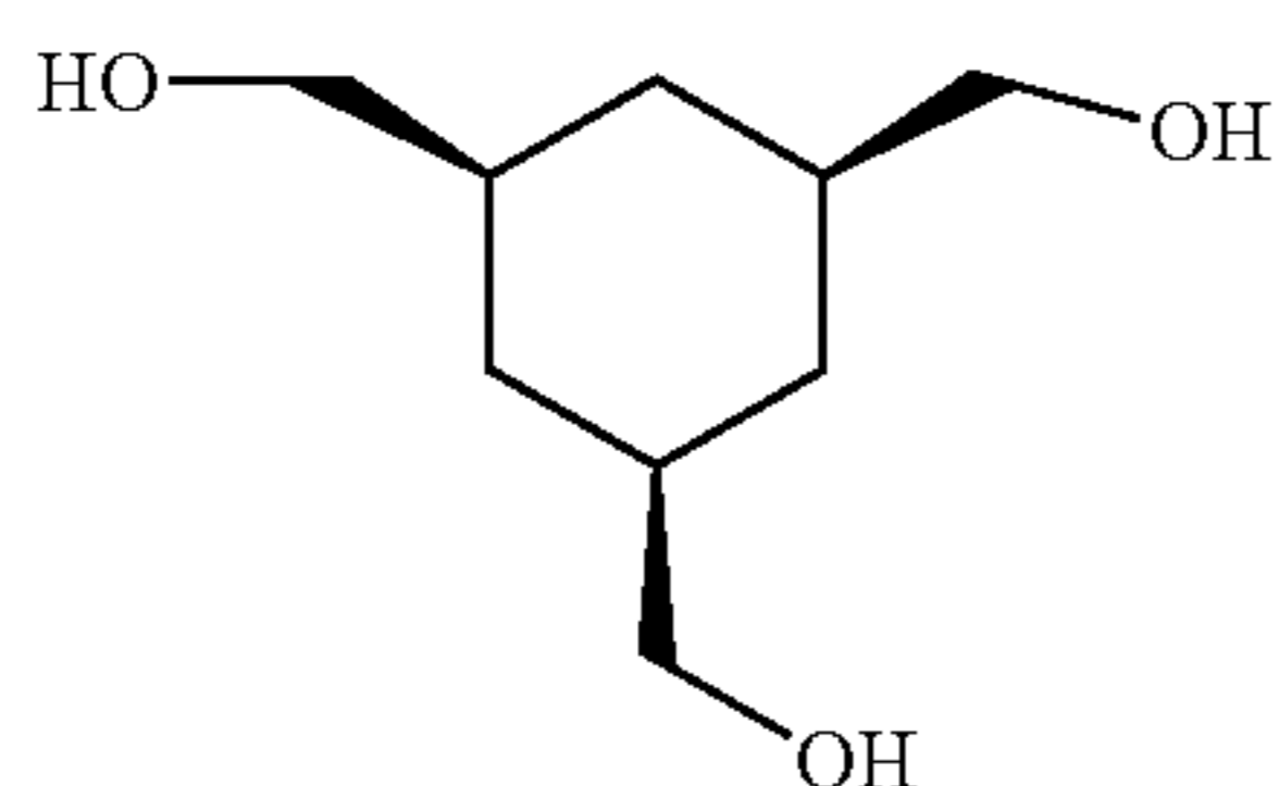
cis-1,3,5-Tri(hydroxymethyl)cyclohexane
