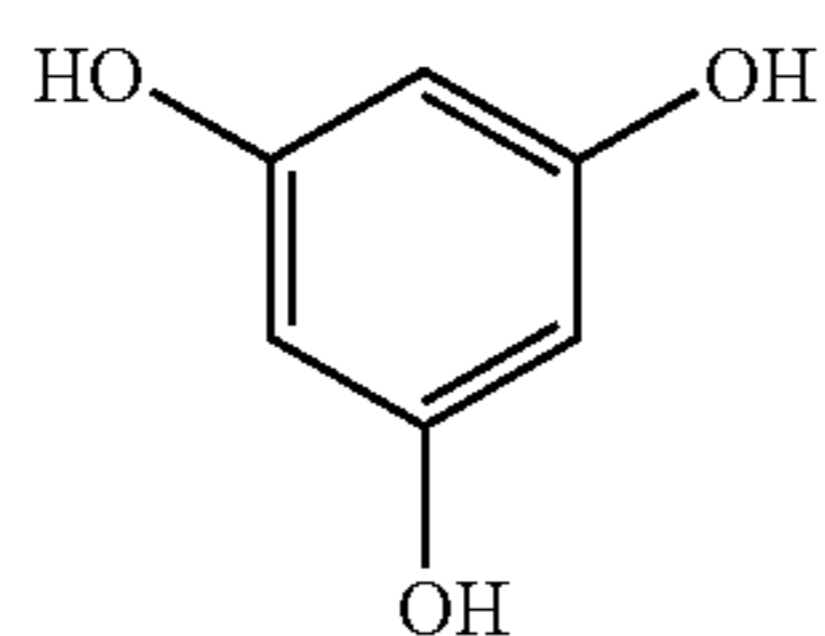
1,3,5-Trihydroxyl-benzene
