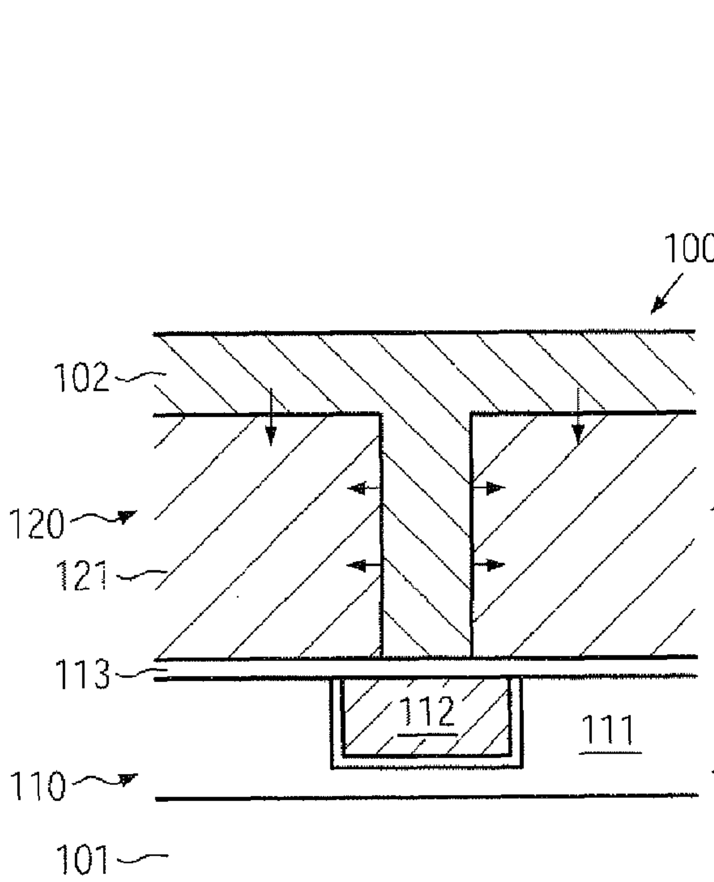
FIG. 1c (prior art)
