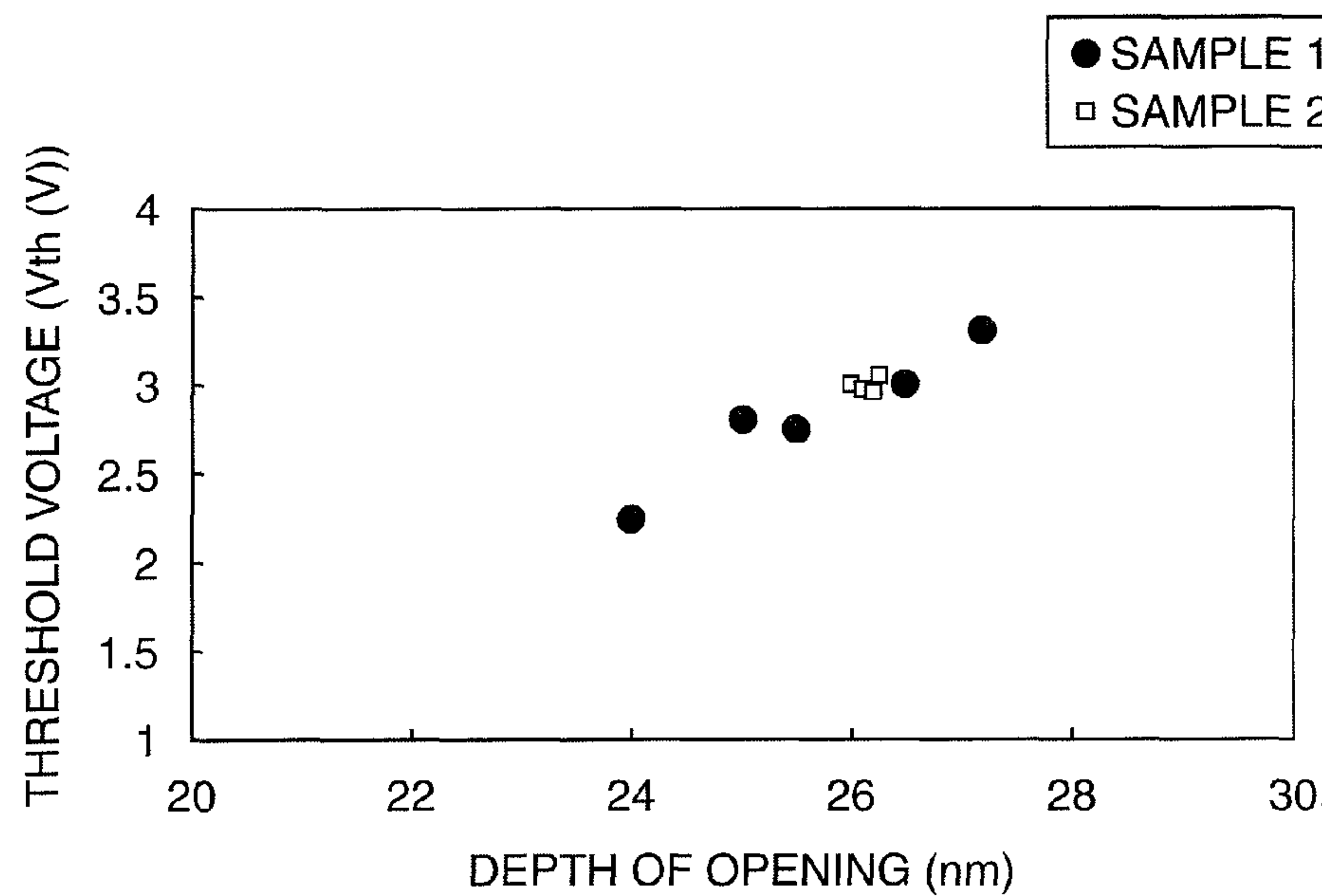
RELATION BETWEEN DEPTH OF ETCHING AND THRESHOLD VOLTAGE
